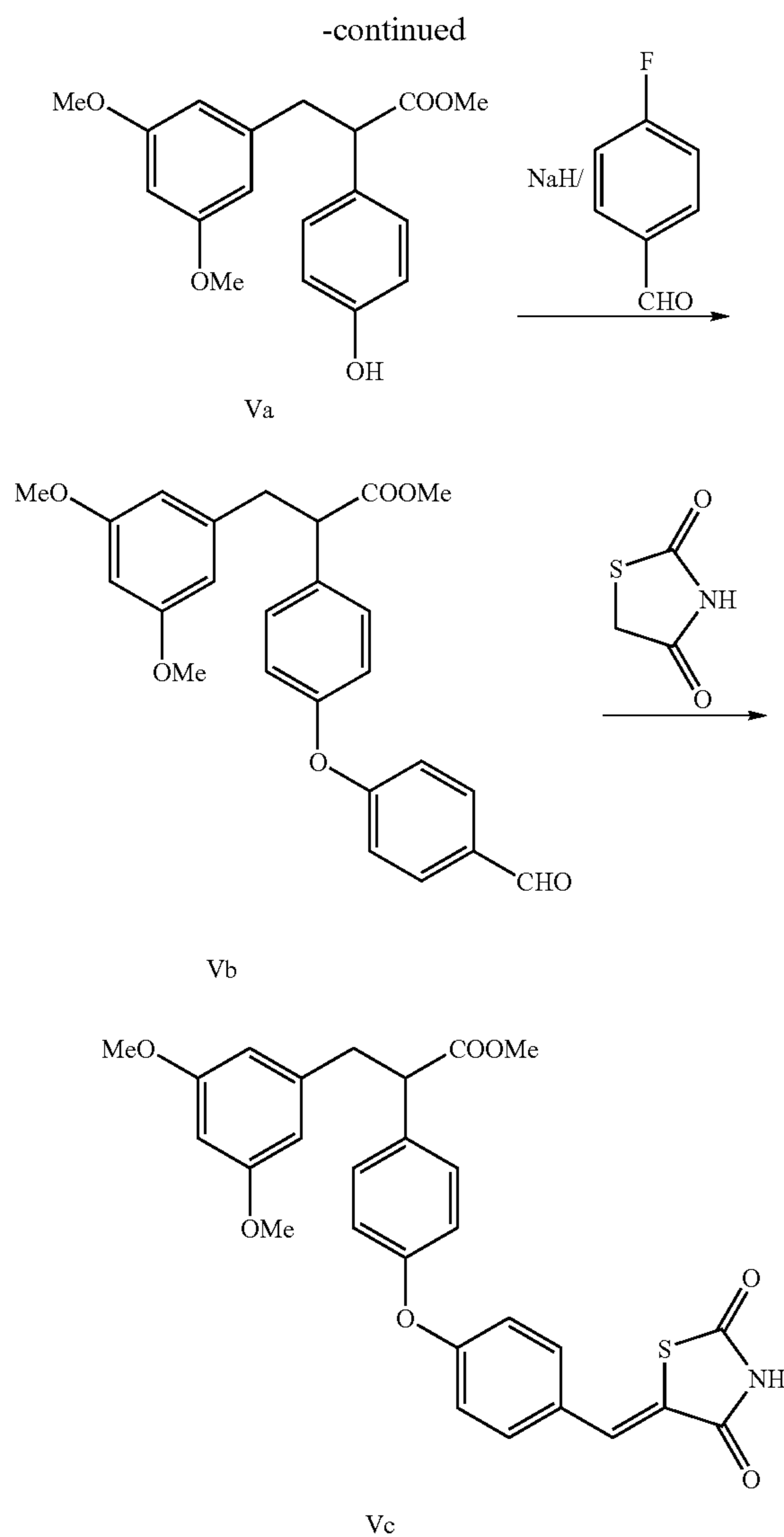
(a) Synthesis of 3-(3,5-Dimethoxy-phenyl)-2-(4-hydroxy-phenyl)-propionic acid methyl ester, (Compound Va)
