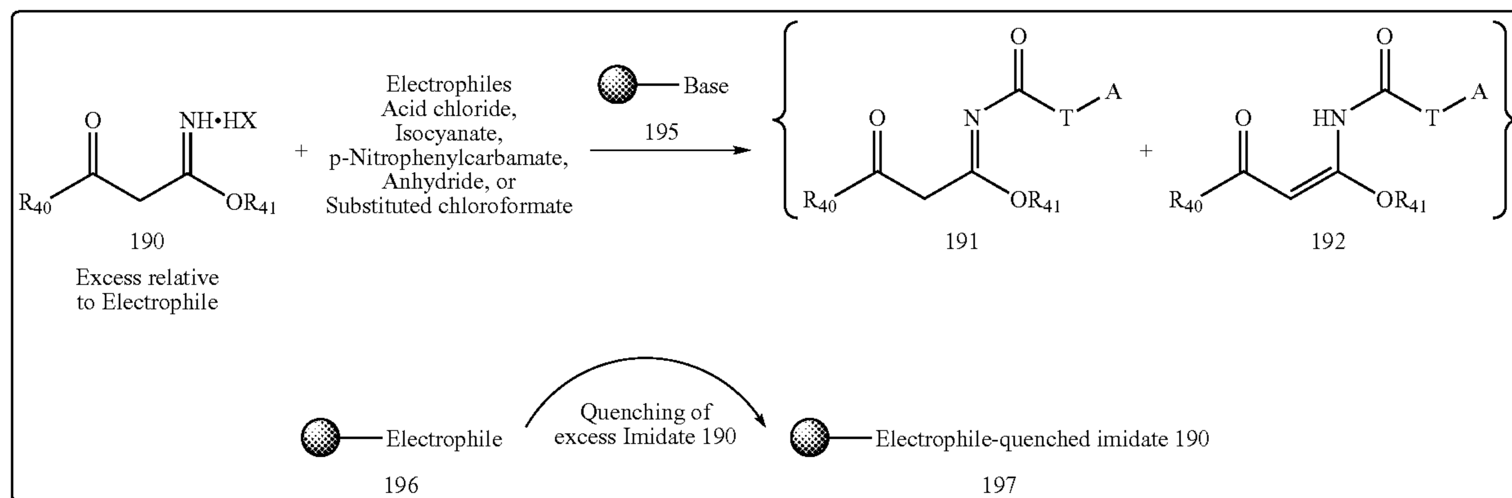
Scheme 36
