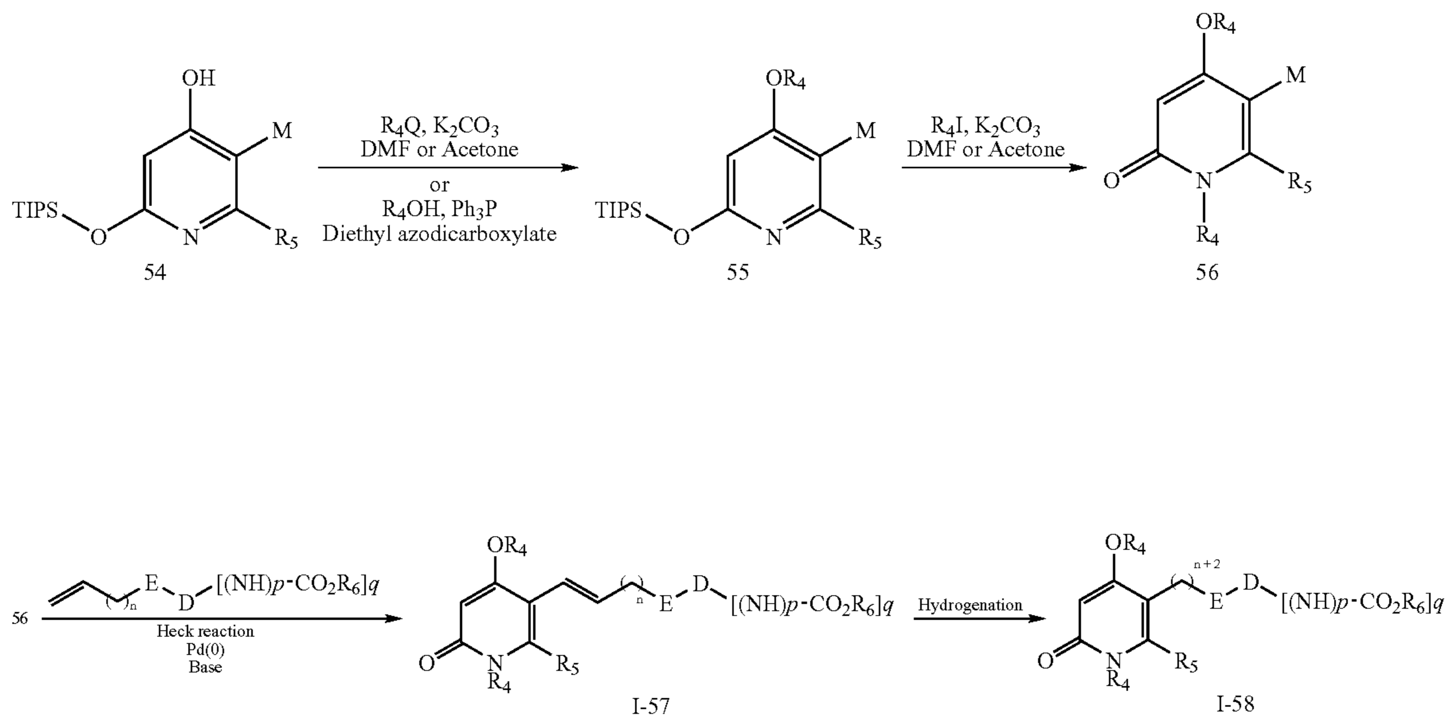
Scheme 10
