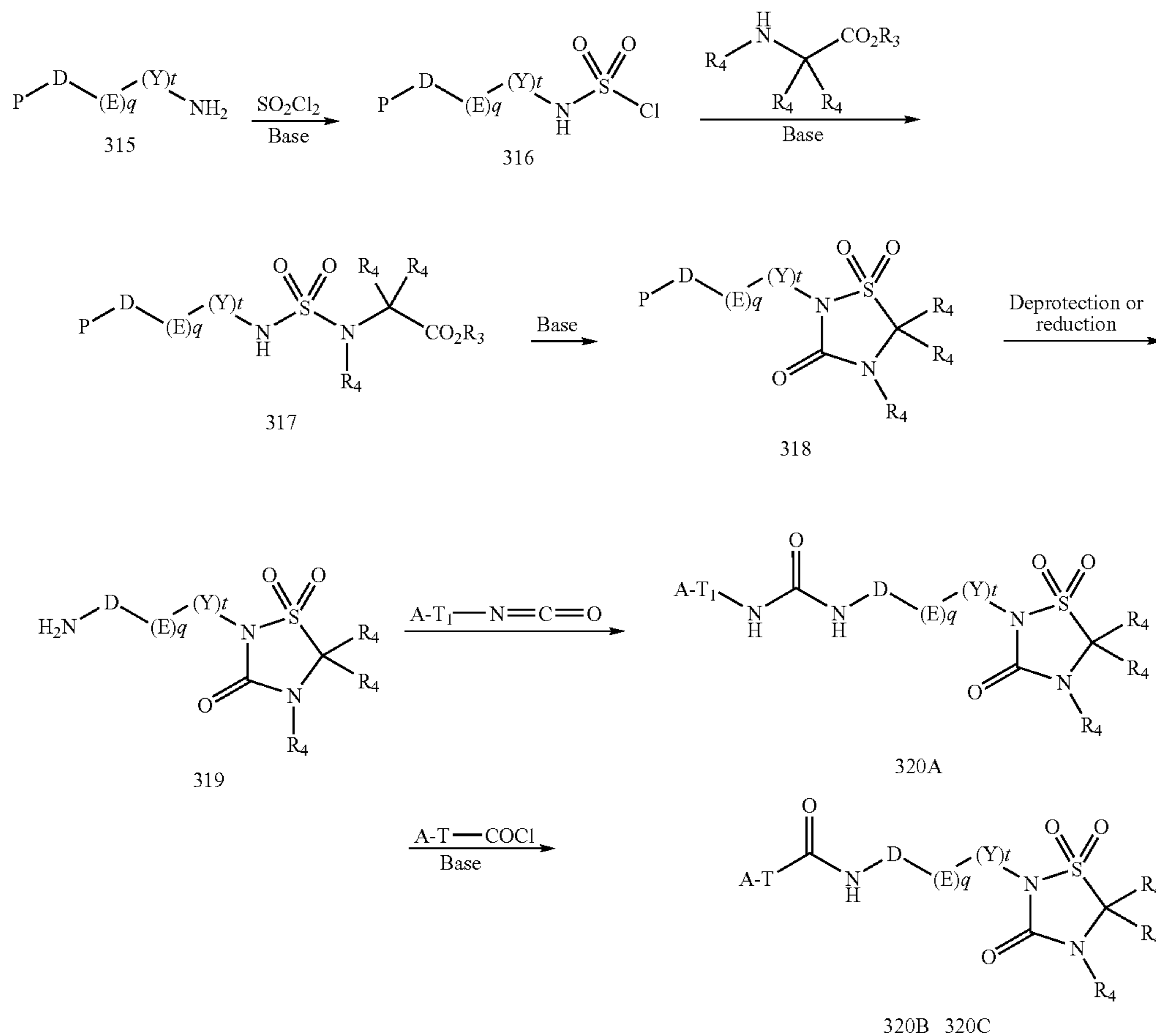
Scheme 57
