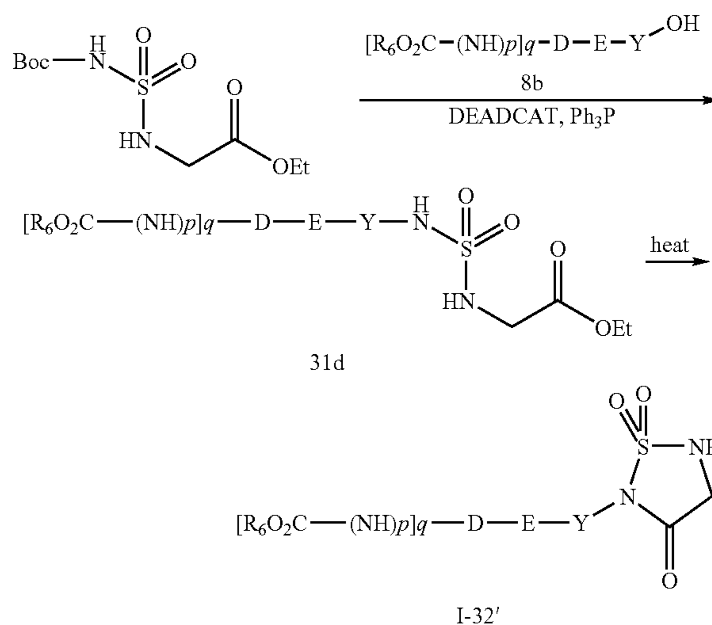
Scheme 5.3
