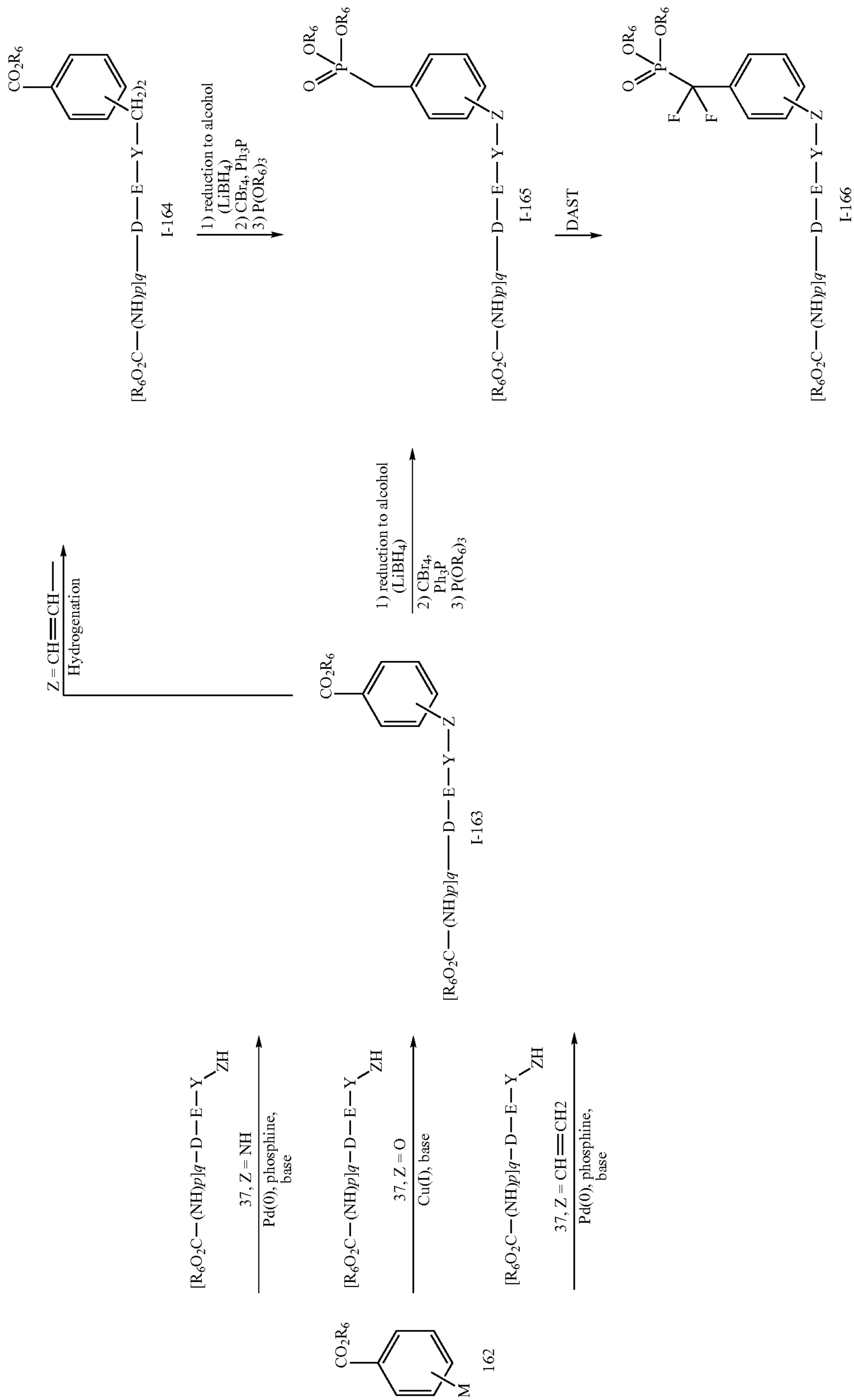
Scheme 26
