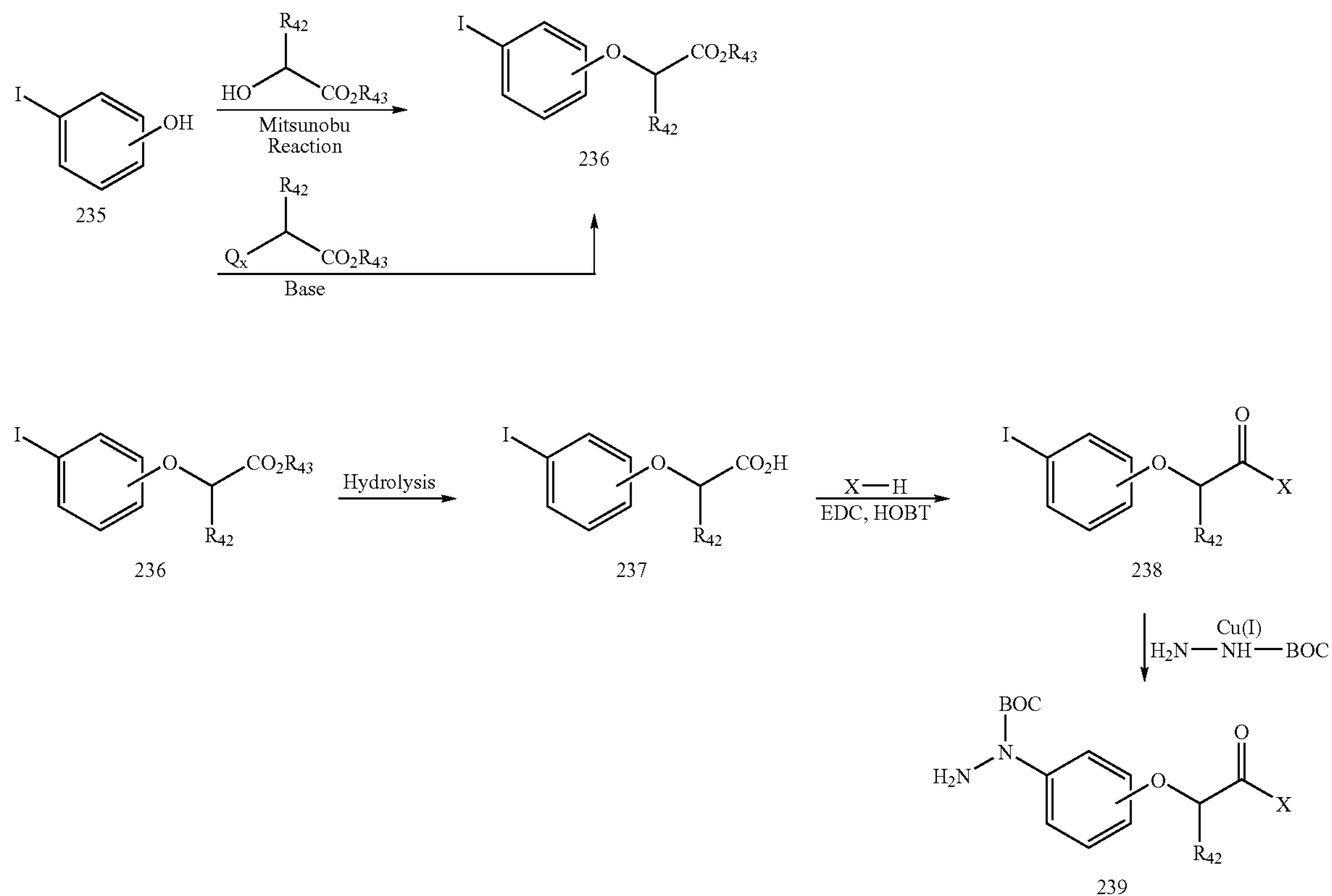
Scheme 43
