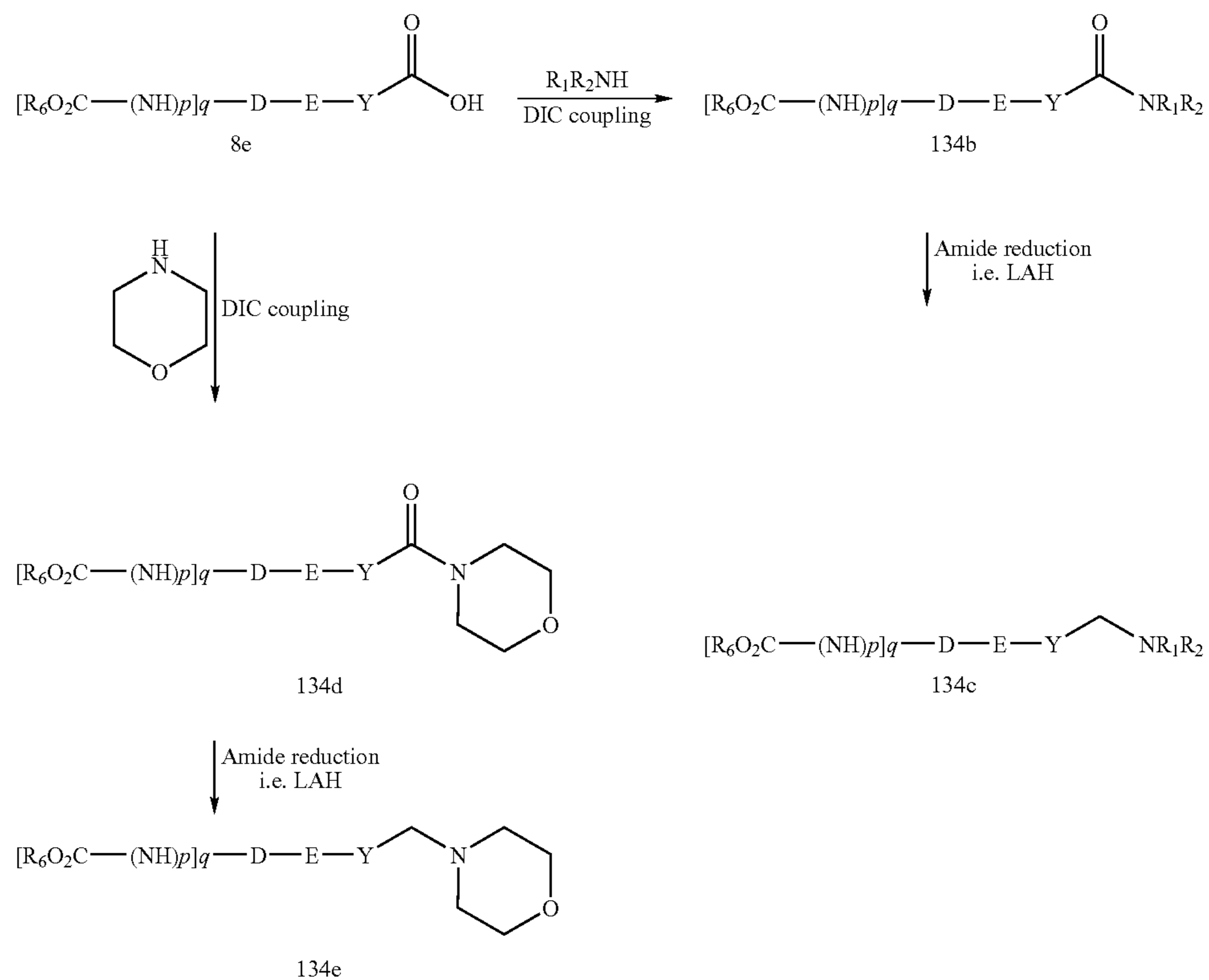
Scheme 21.2
