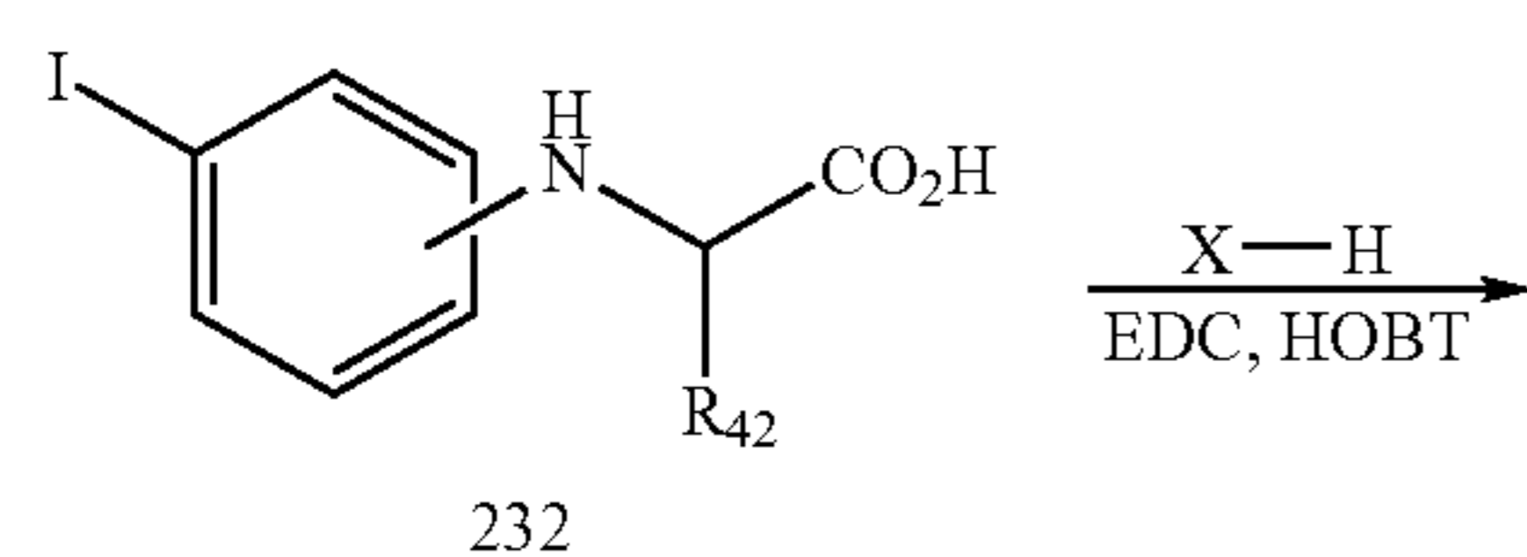
Scheme 44
