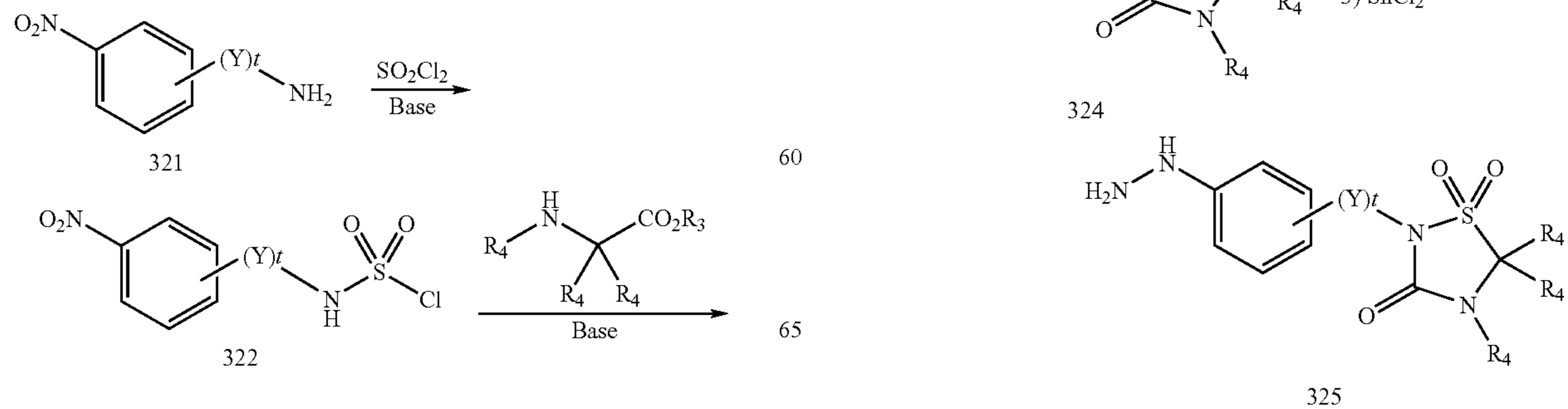
Scheme 58
