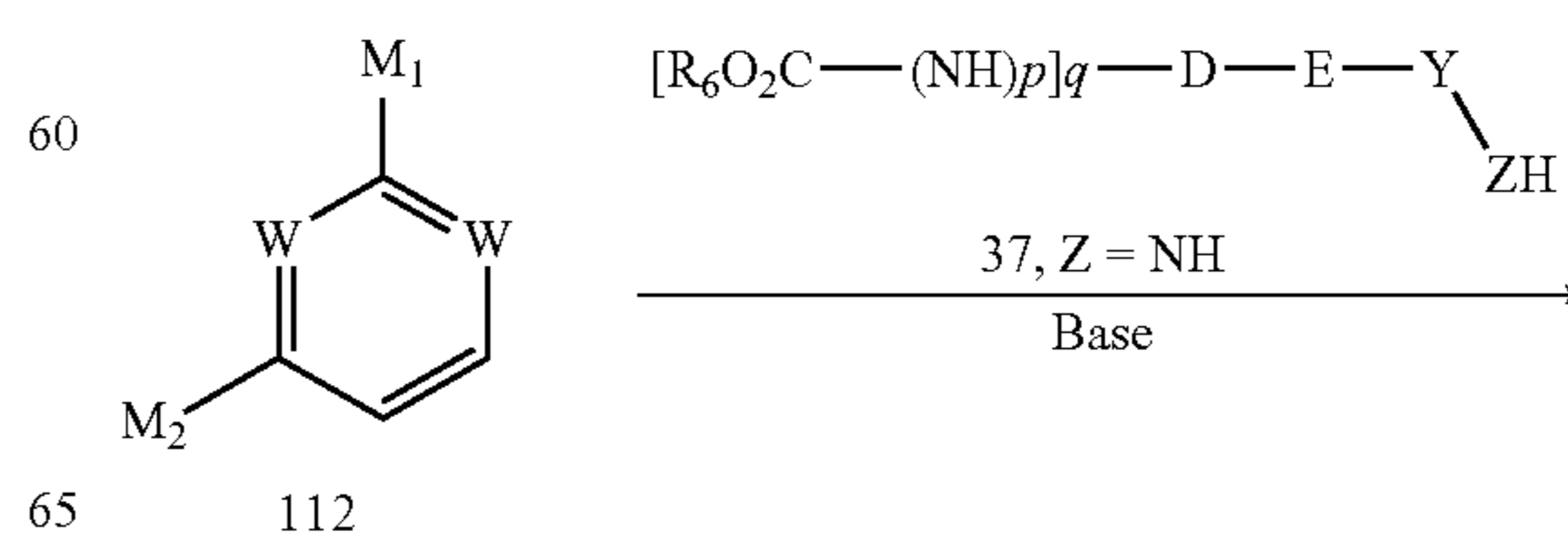
Scheme 19.1
