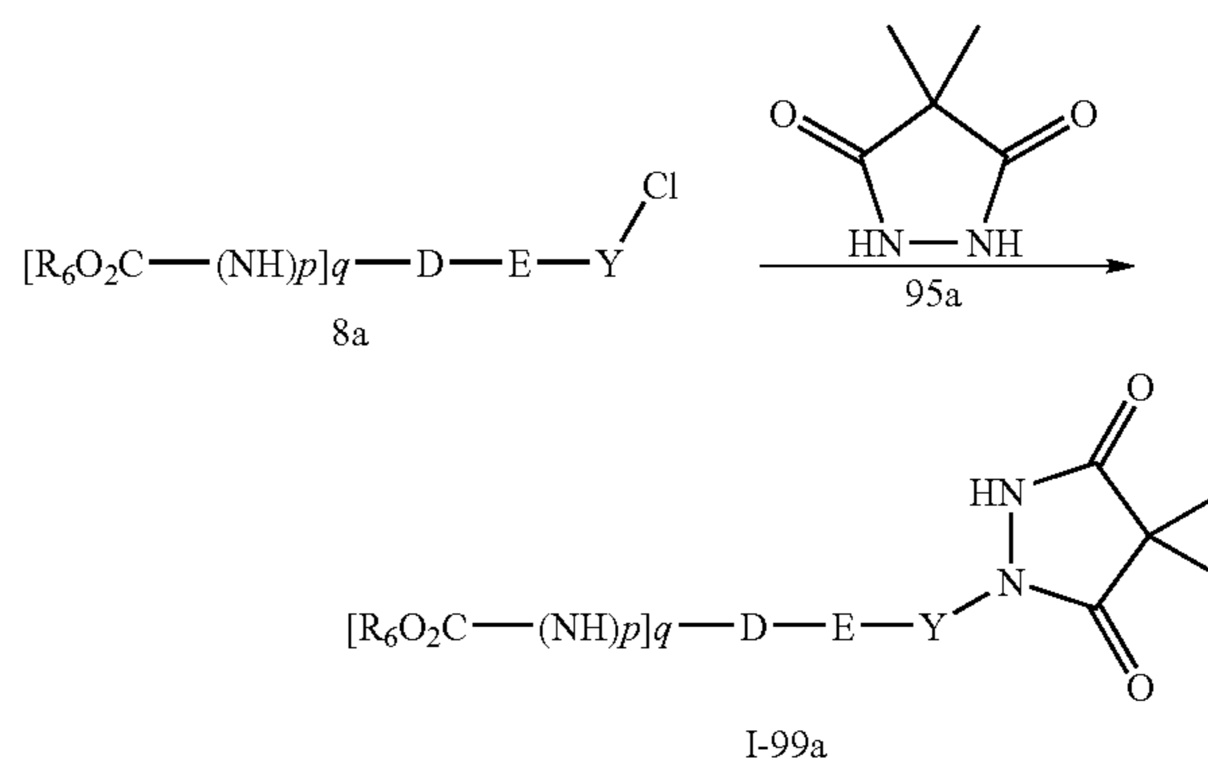
Scheme 16.3
