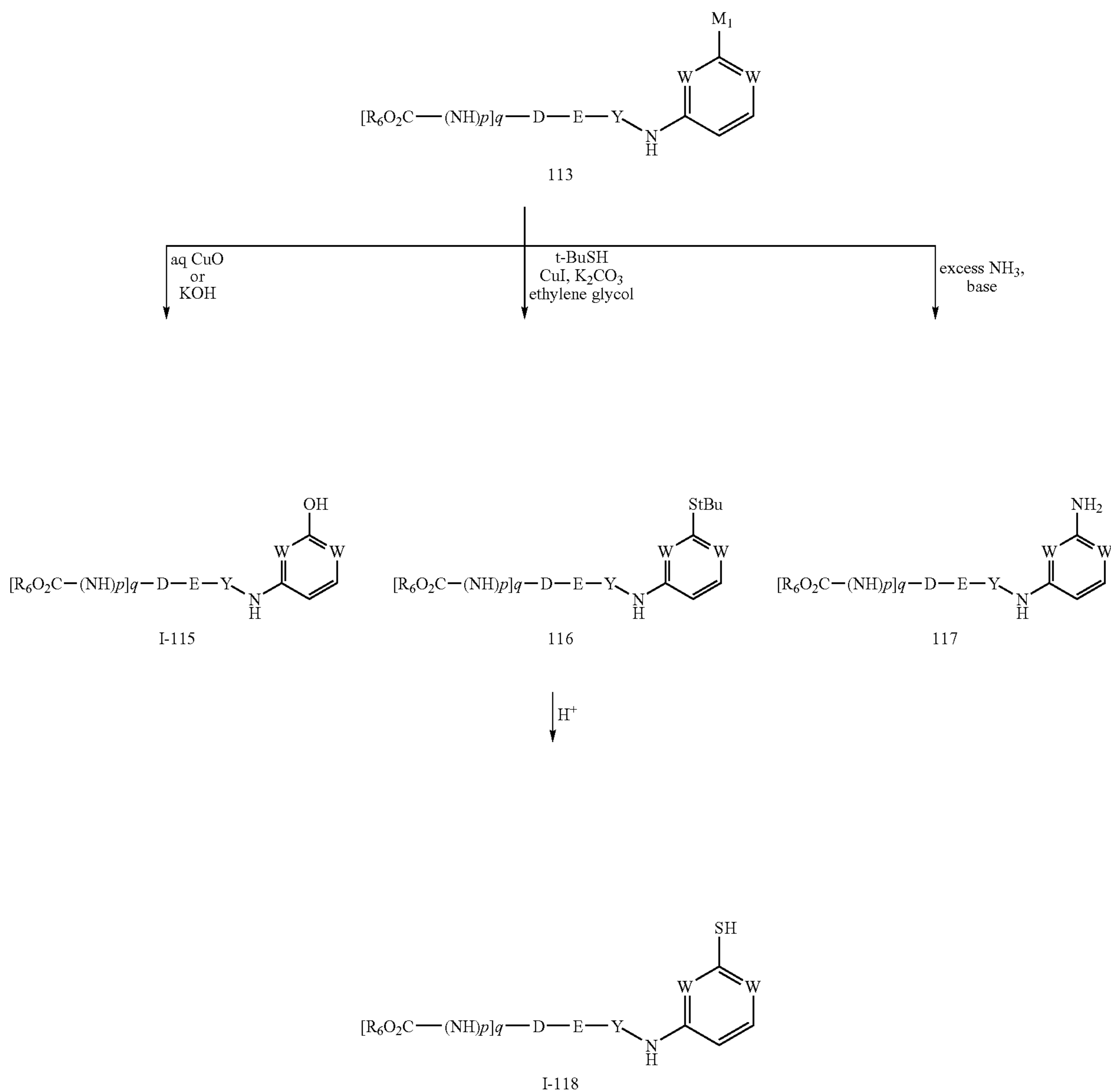
Scheme 19.2
