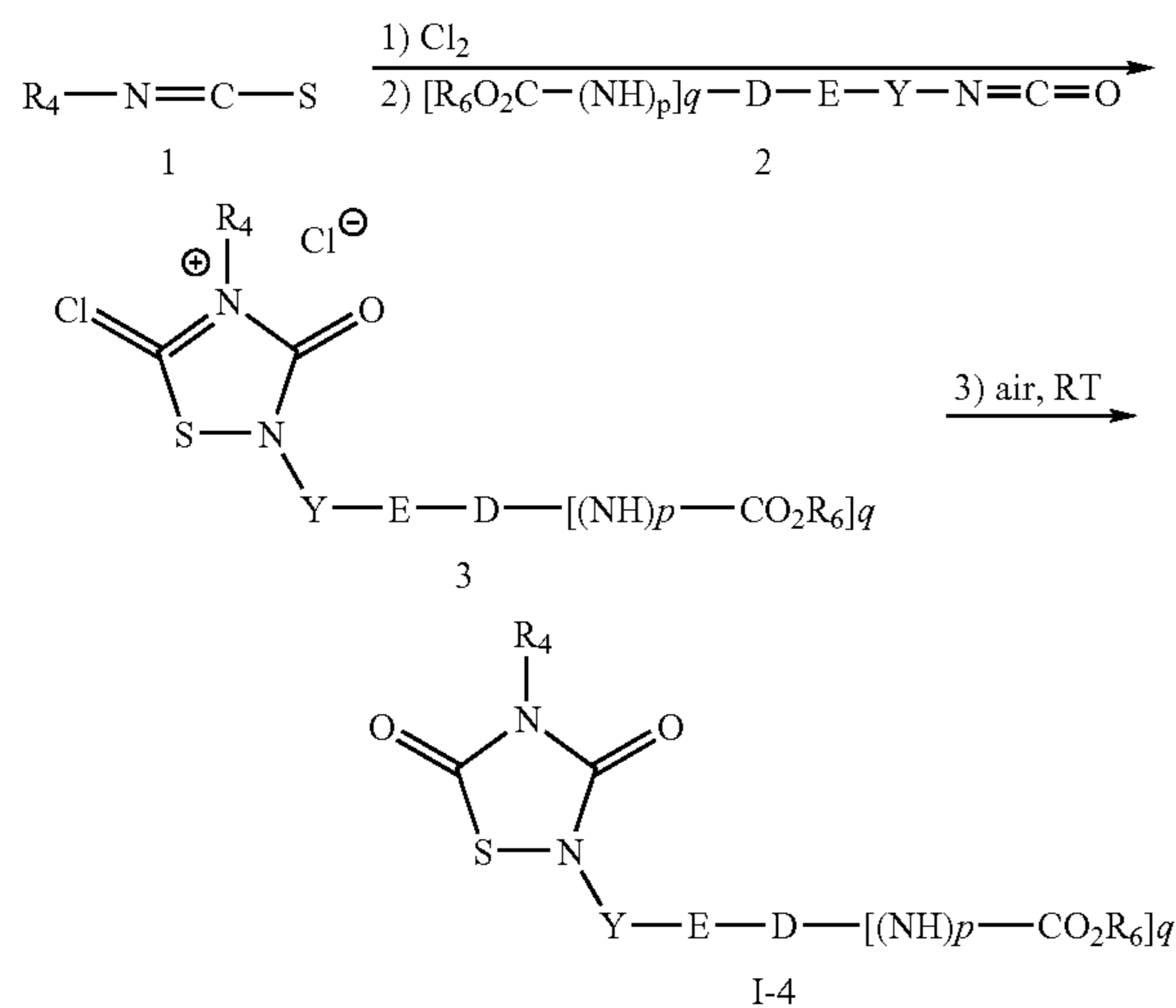
Scheme 1.1
