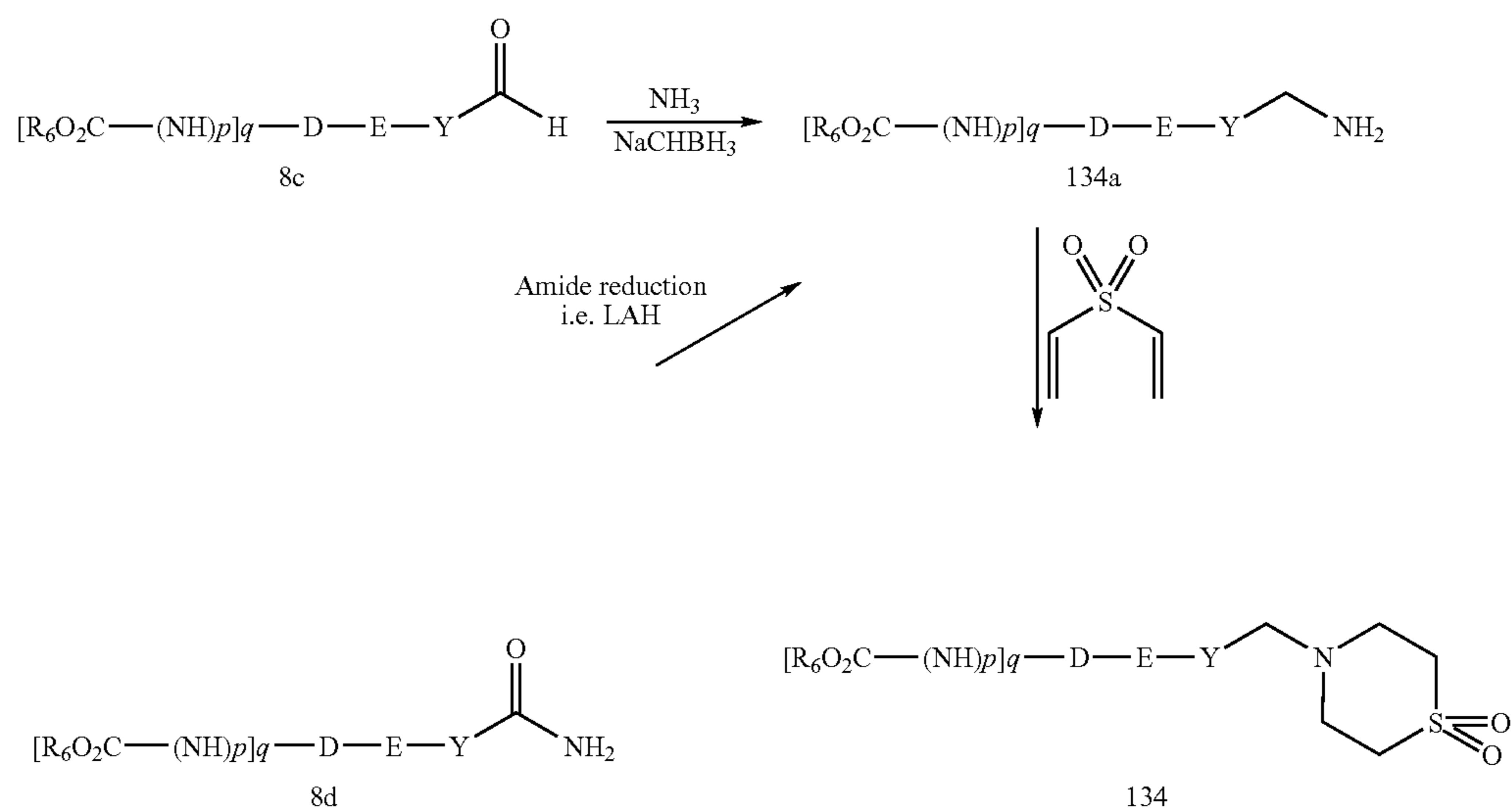
Scheme 21.1
