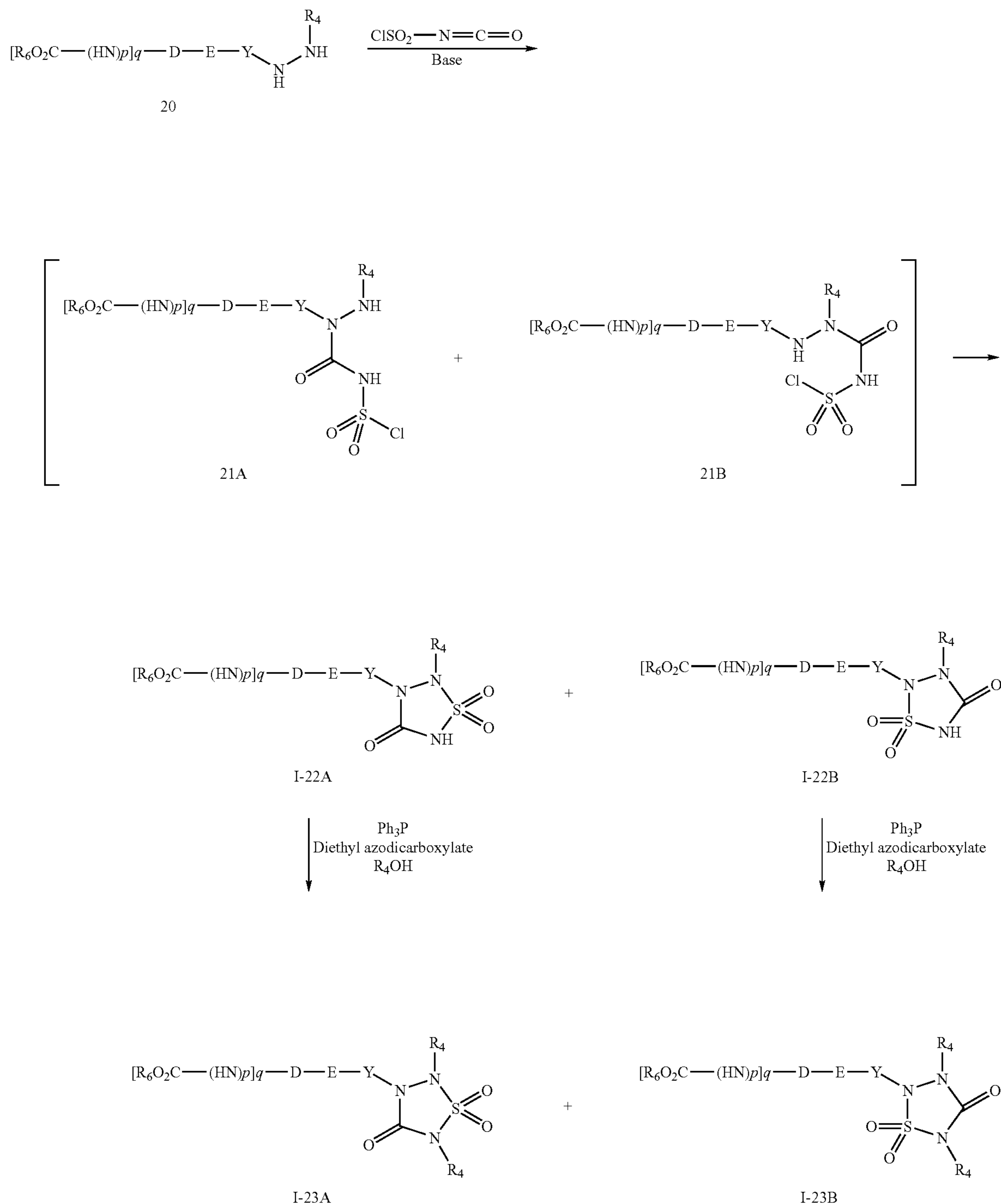
Scheme 3
