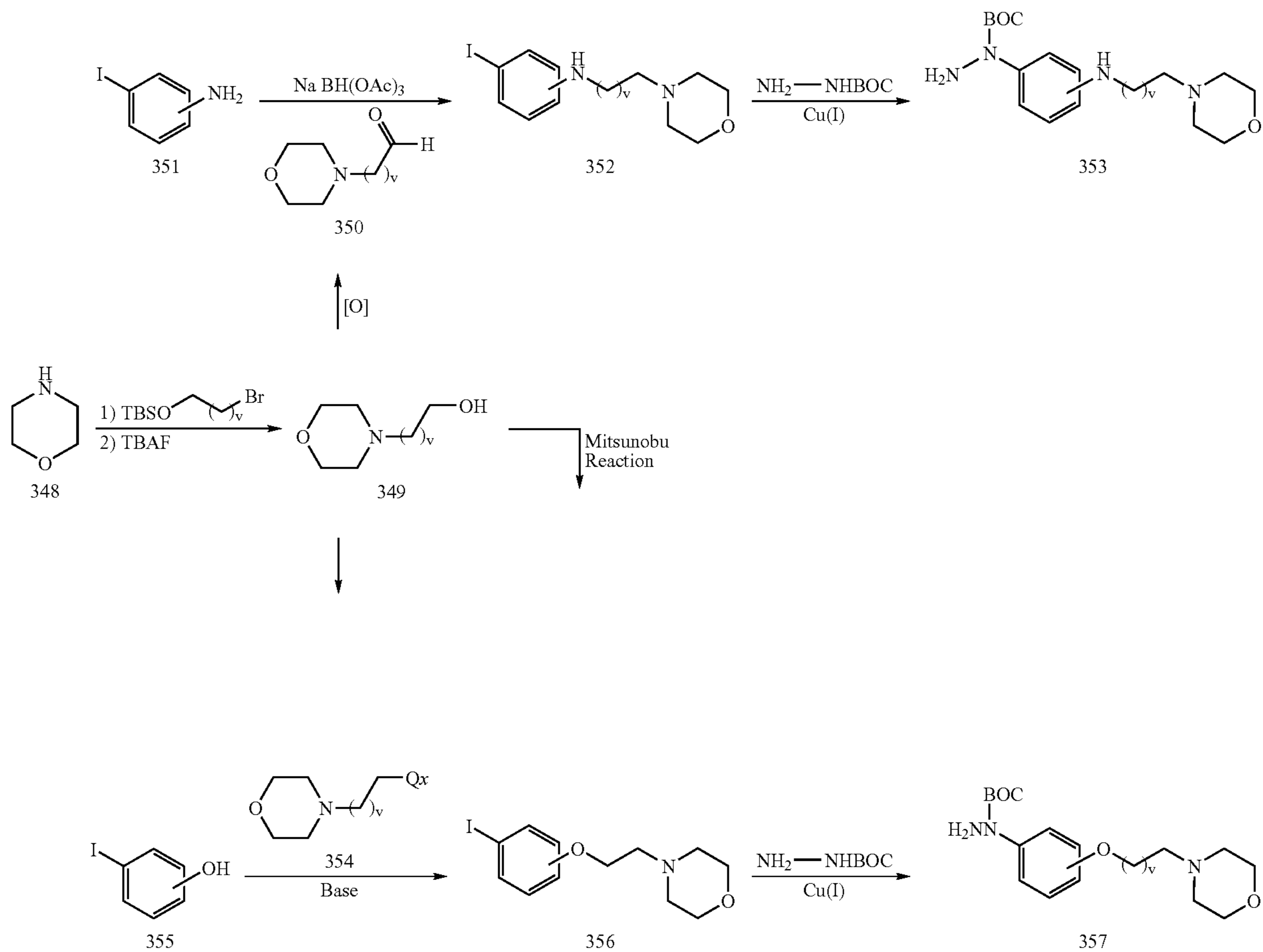
Scheme 63
