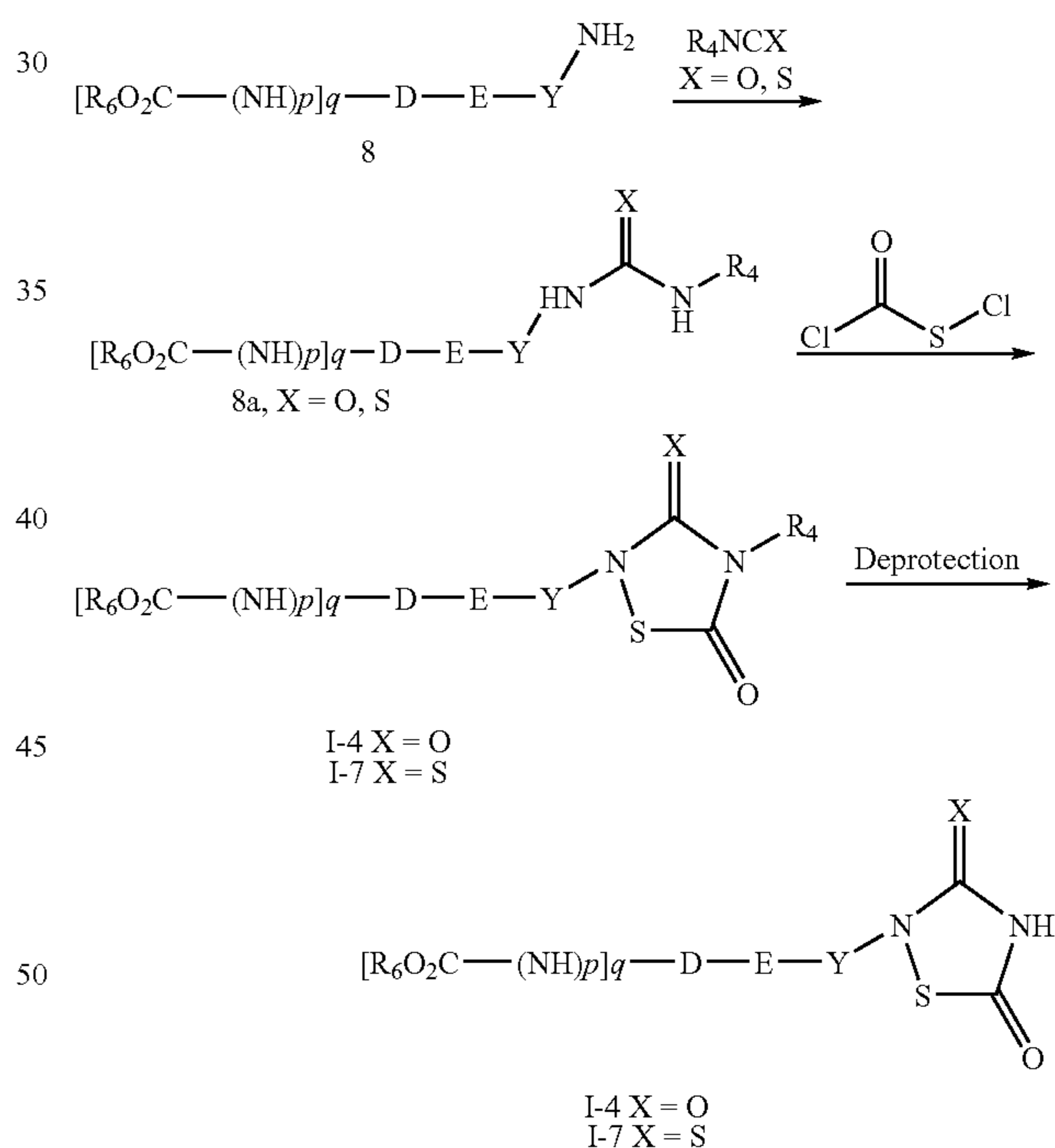
Scheme 1.3
