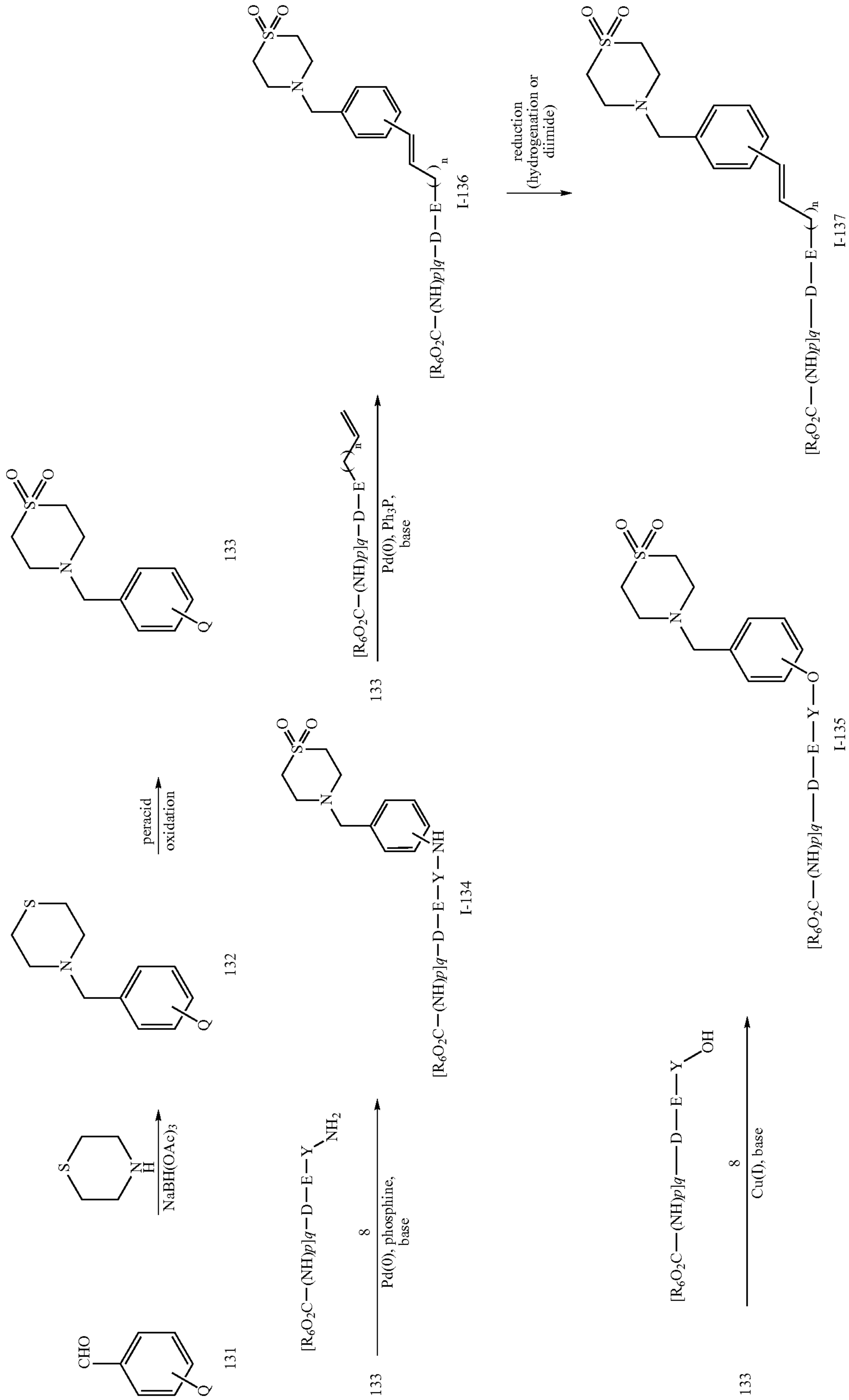
Scheme 21
