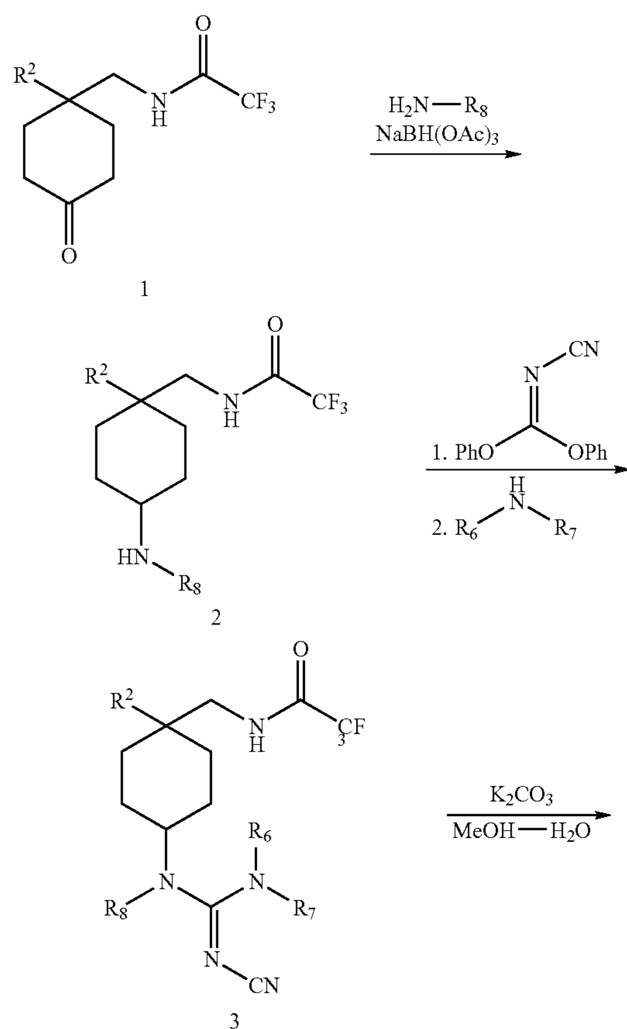
Scheme 3
