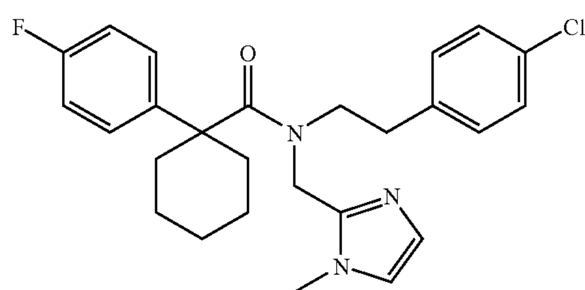
1-(4-fluoro-phenyl)-cyclohexanecarboxylic acid [2-(4-chloro-phenyl)-ethyl]-(1-methyl-1H-imidazol-2-ylmethyl)-amide
