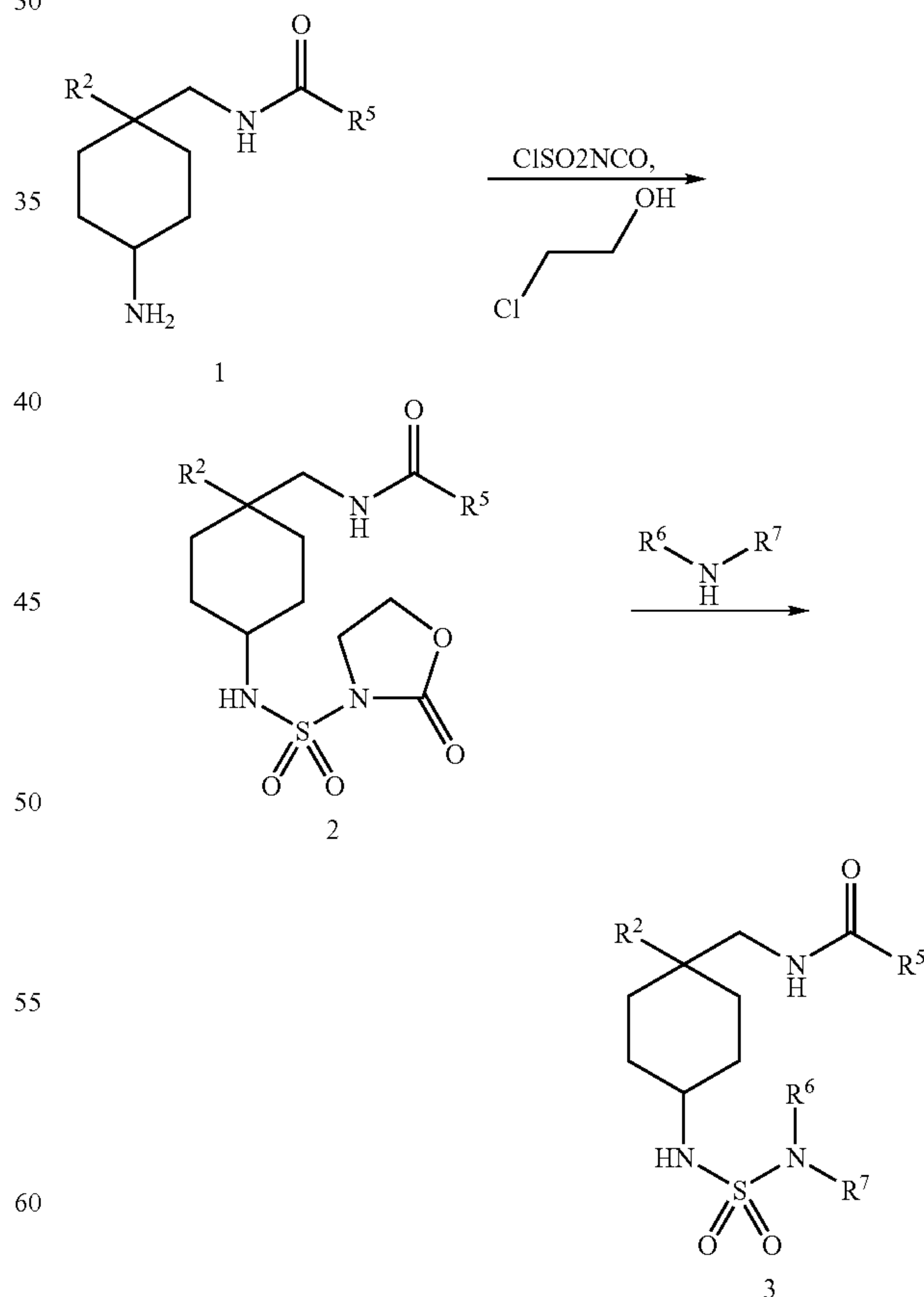
Scheme 4
