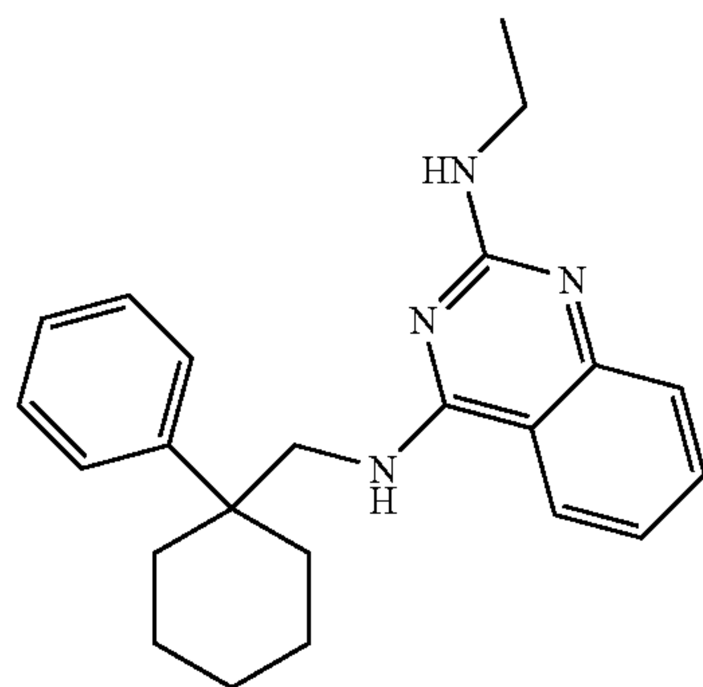
N 2 -ethyl-N 4 -(1-phenyl-cyclohexylmethyl)-quinazoline-2,4-diamine
