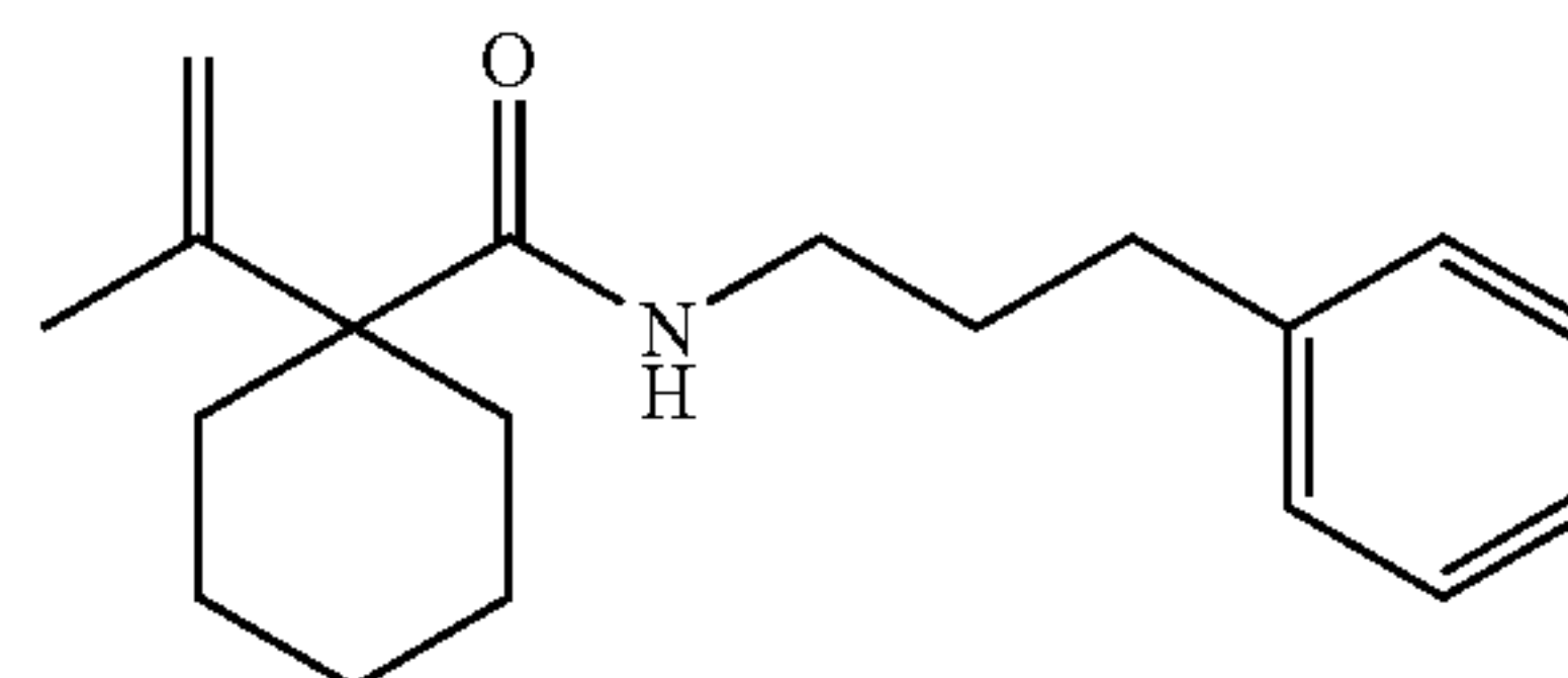
1-Isopropenyl-cyclohexanecarboxylic acid (3-phenyl-propyl)-amide
