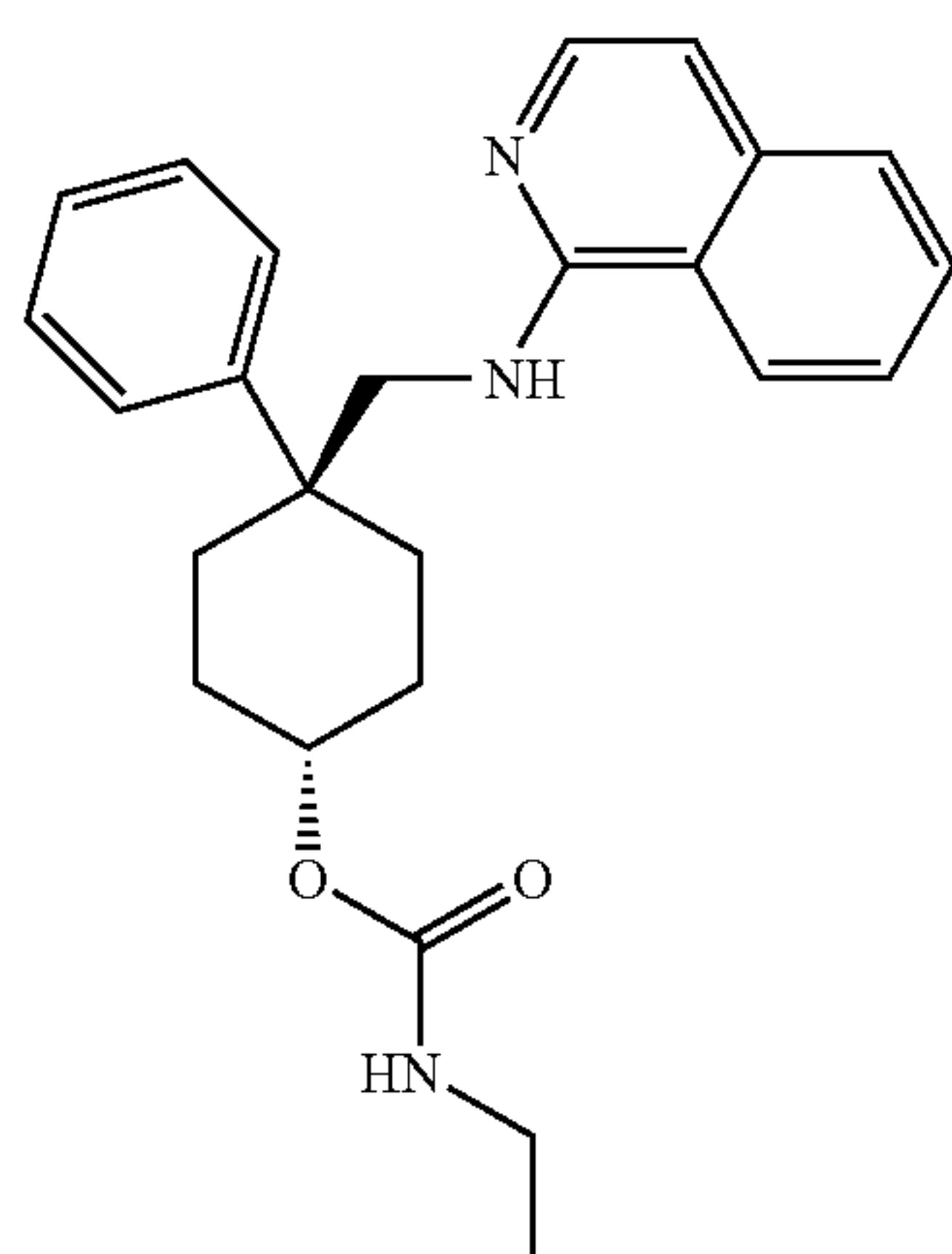
Ethyl-carbamic acid 4-(isoquinolin-1-ylaminomethyl)-4-phenyl-cyclohexyl ester
