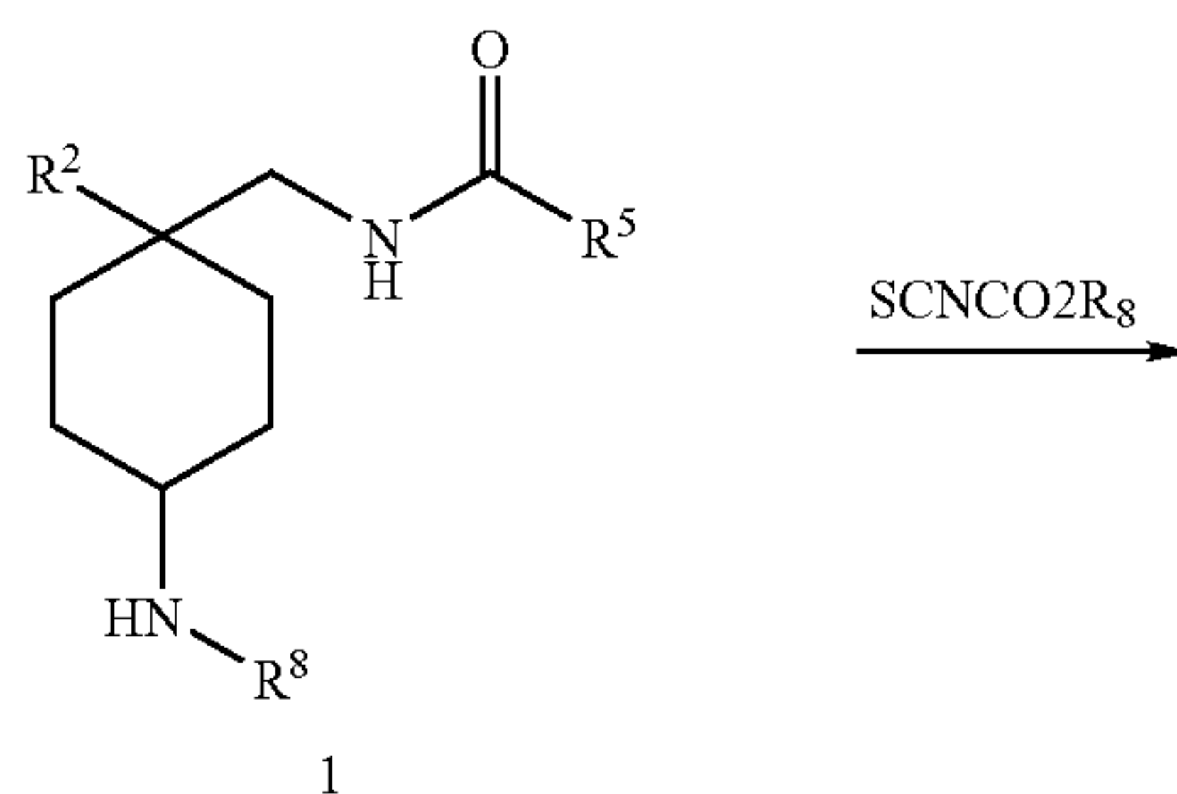
Scheme 5
