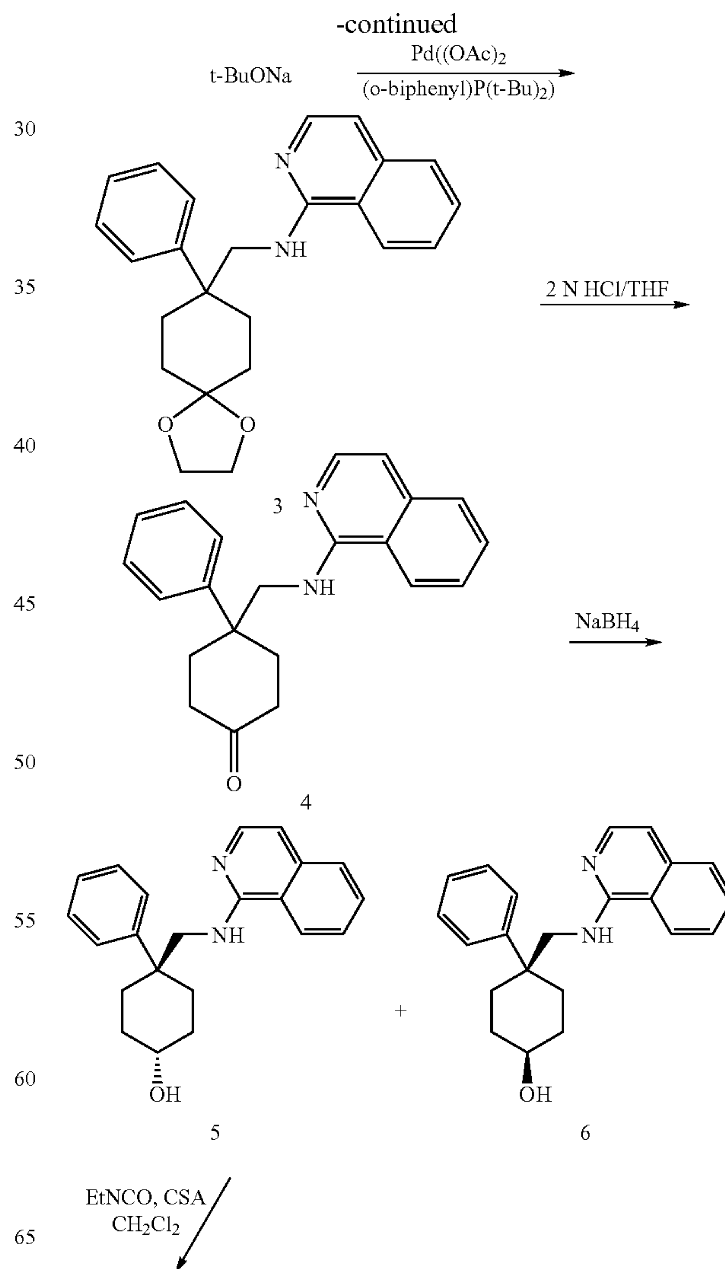
Ethyl-carbamic acid 4-(isoquinolin-1-ylaminomethyl)-4-phenyl-cyclohexyl ester
