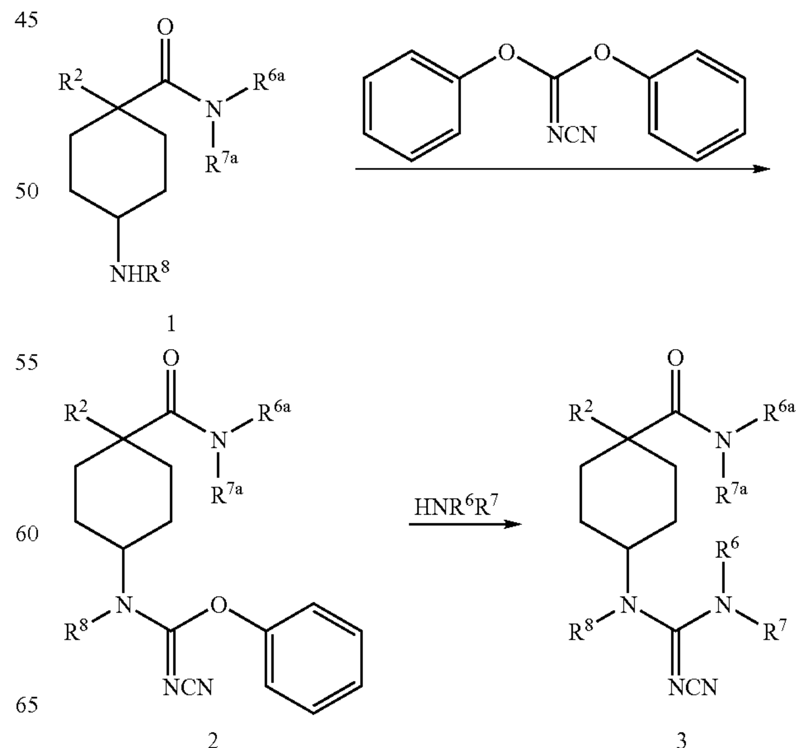
Scheme 19
