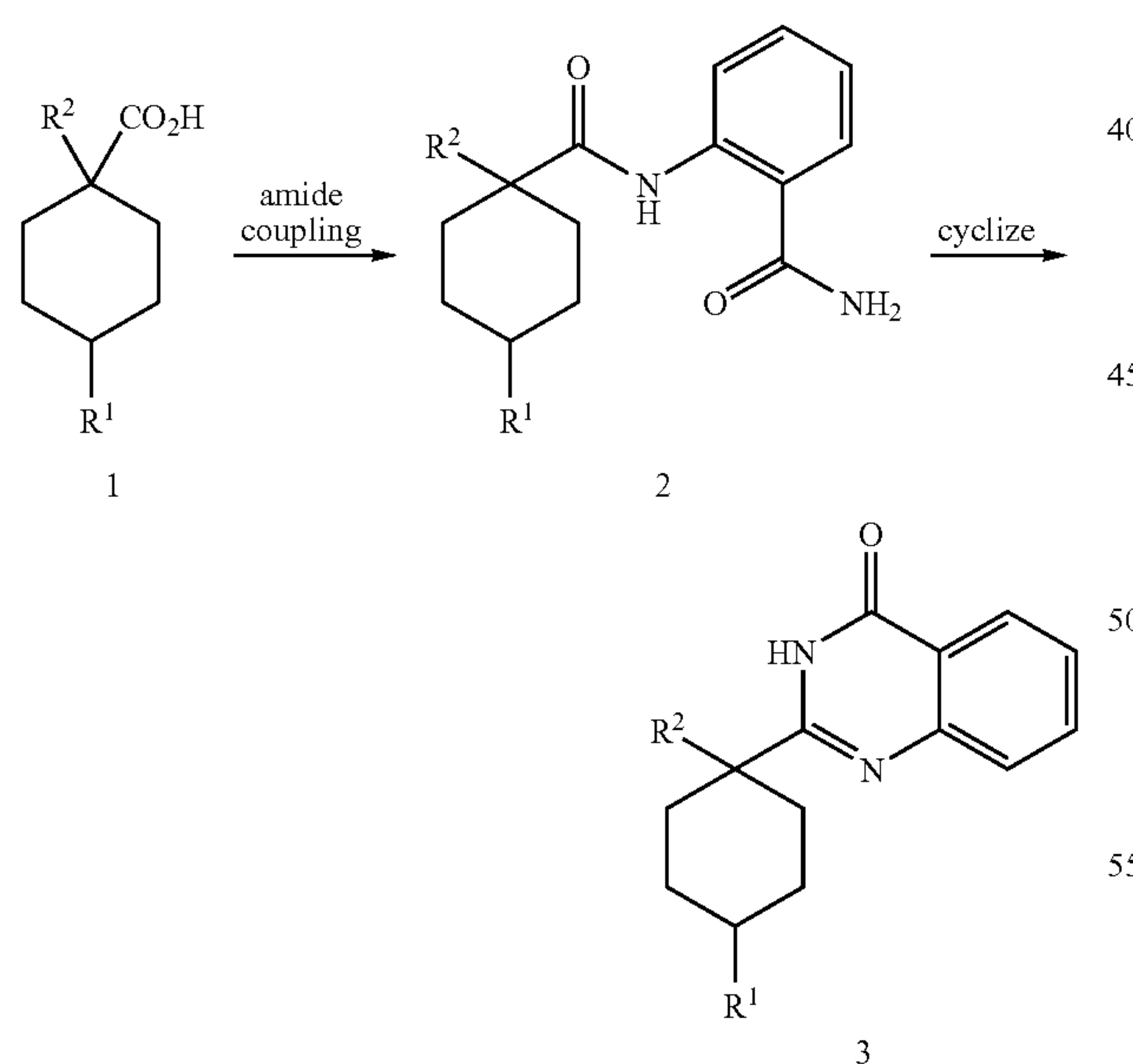
Scheme 14
