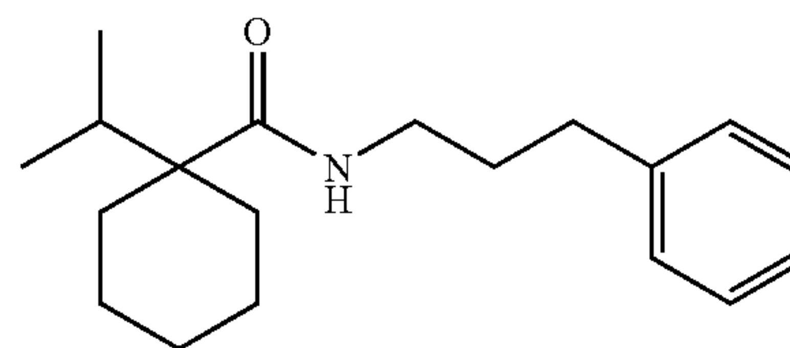
1-Isopropyl-cyclohexanecarboxylic acid (3-phenyl-propyl)-amide
