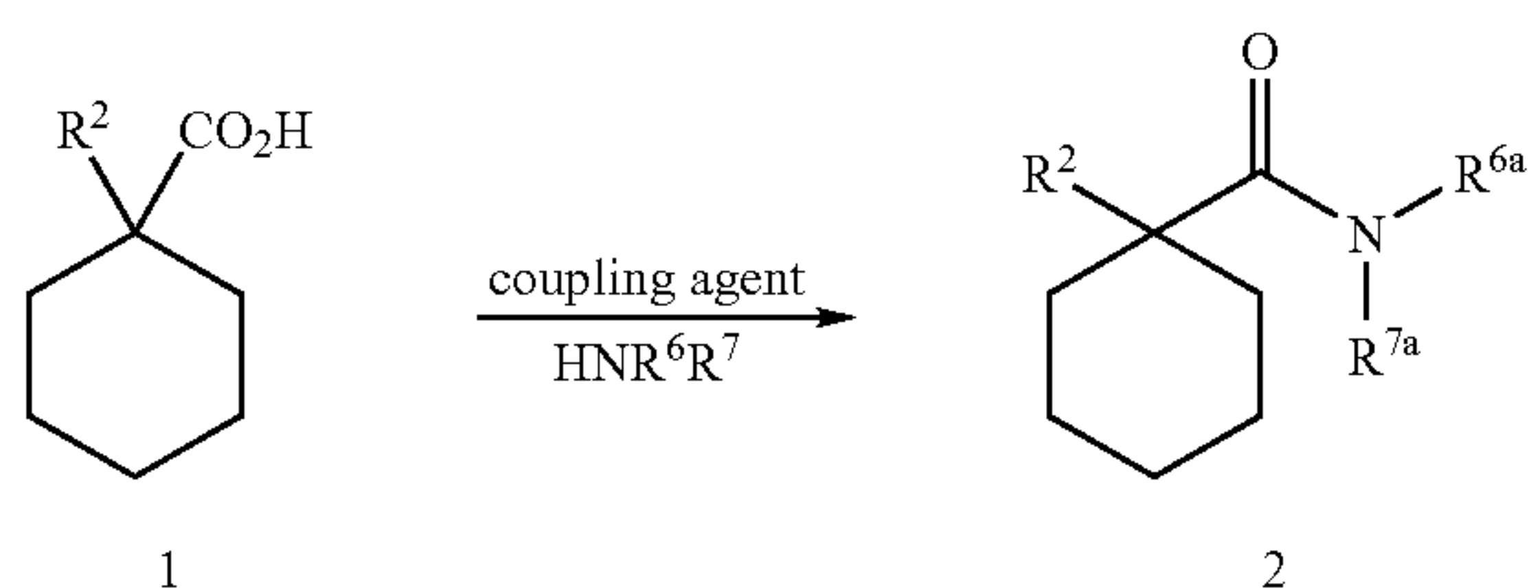
Scheme 11
