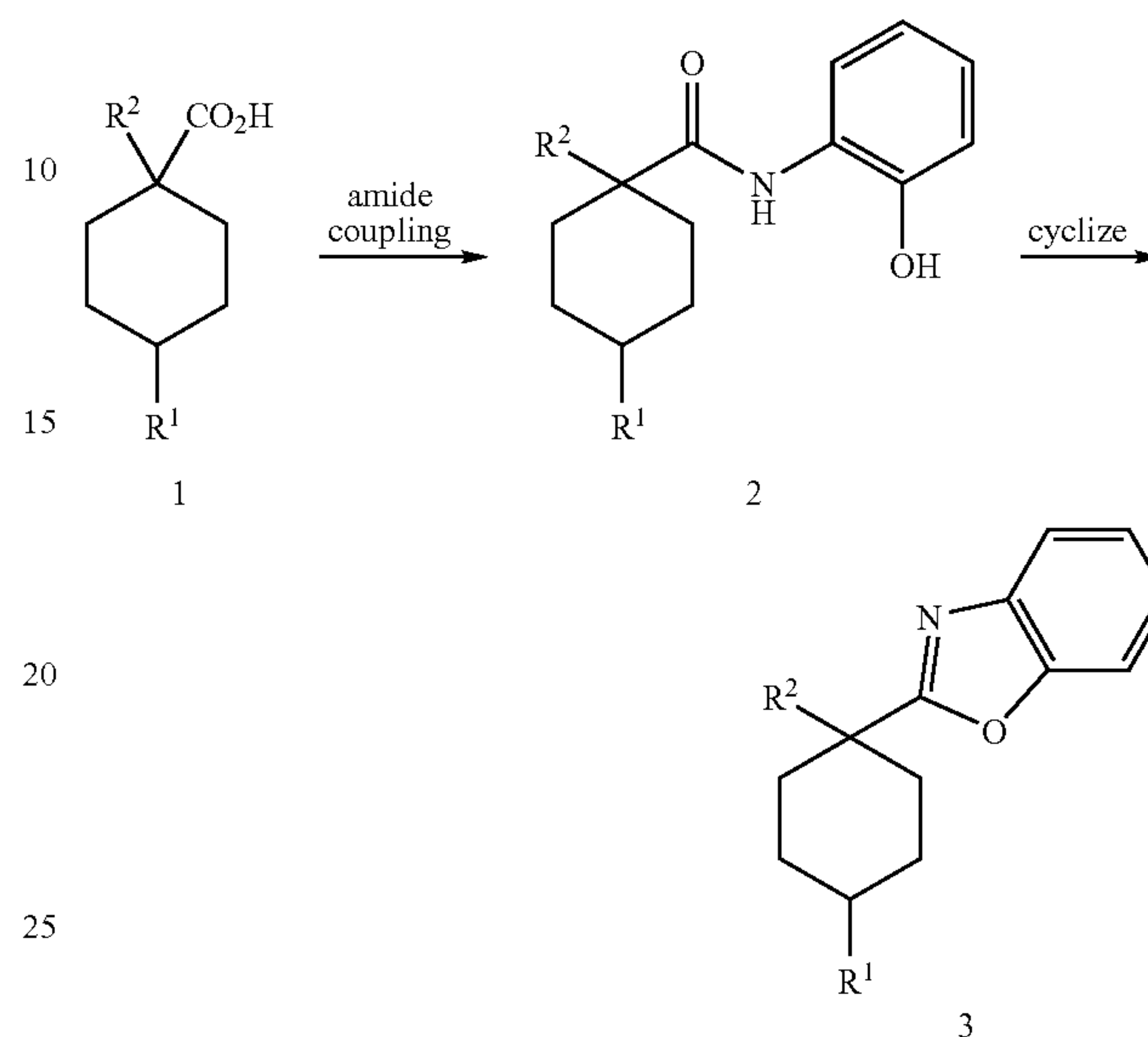
Scheme 15
