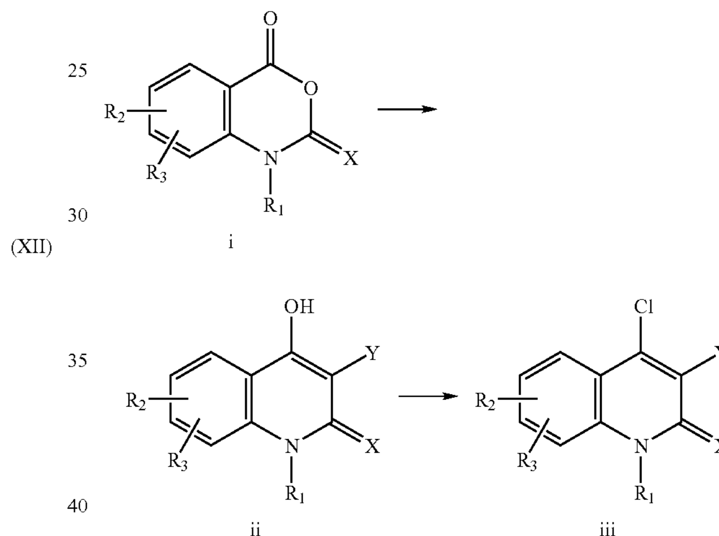
Reaction Scheme 1
