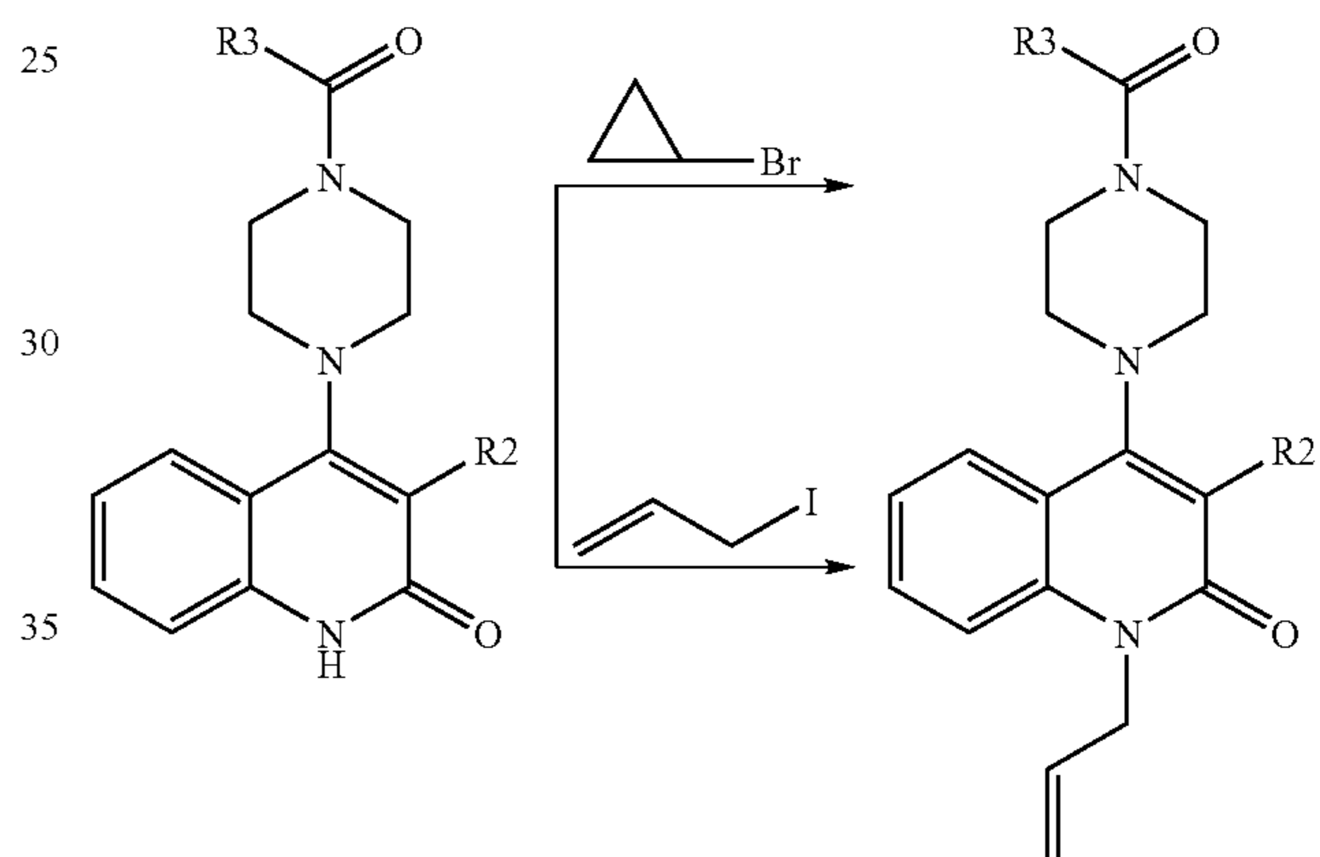
Reaction Scheme 8
