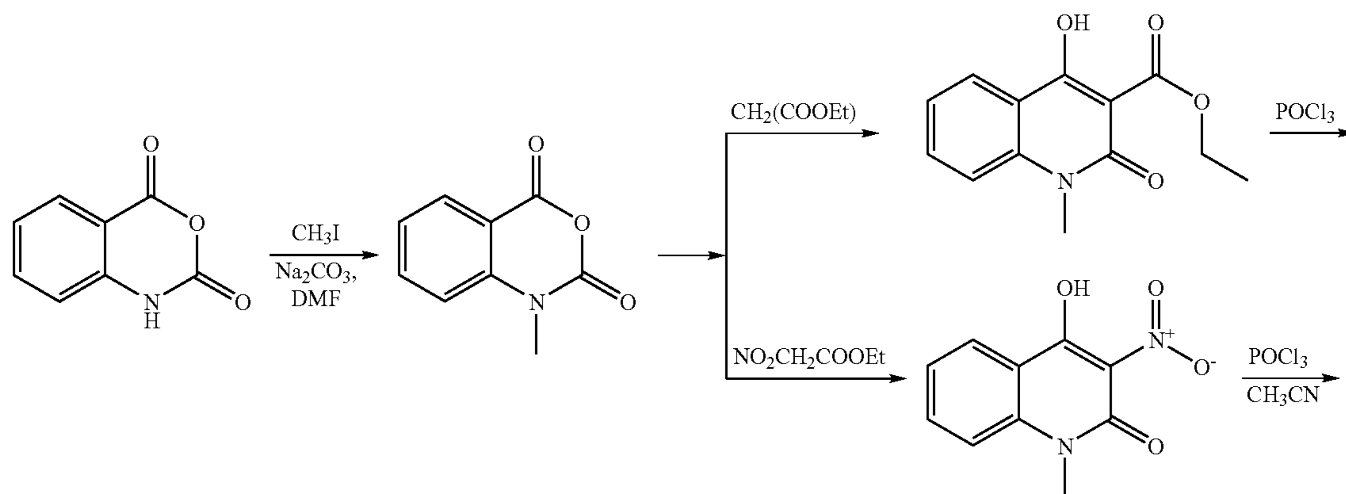
Reaction Scheme 9
