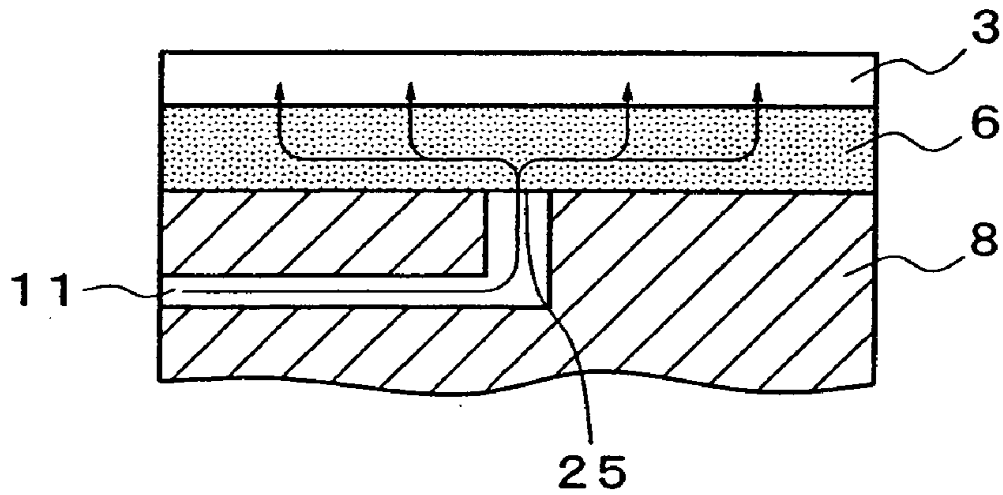
FIG. 8 (PRIOR ART)
