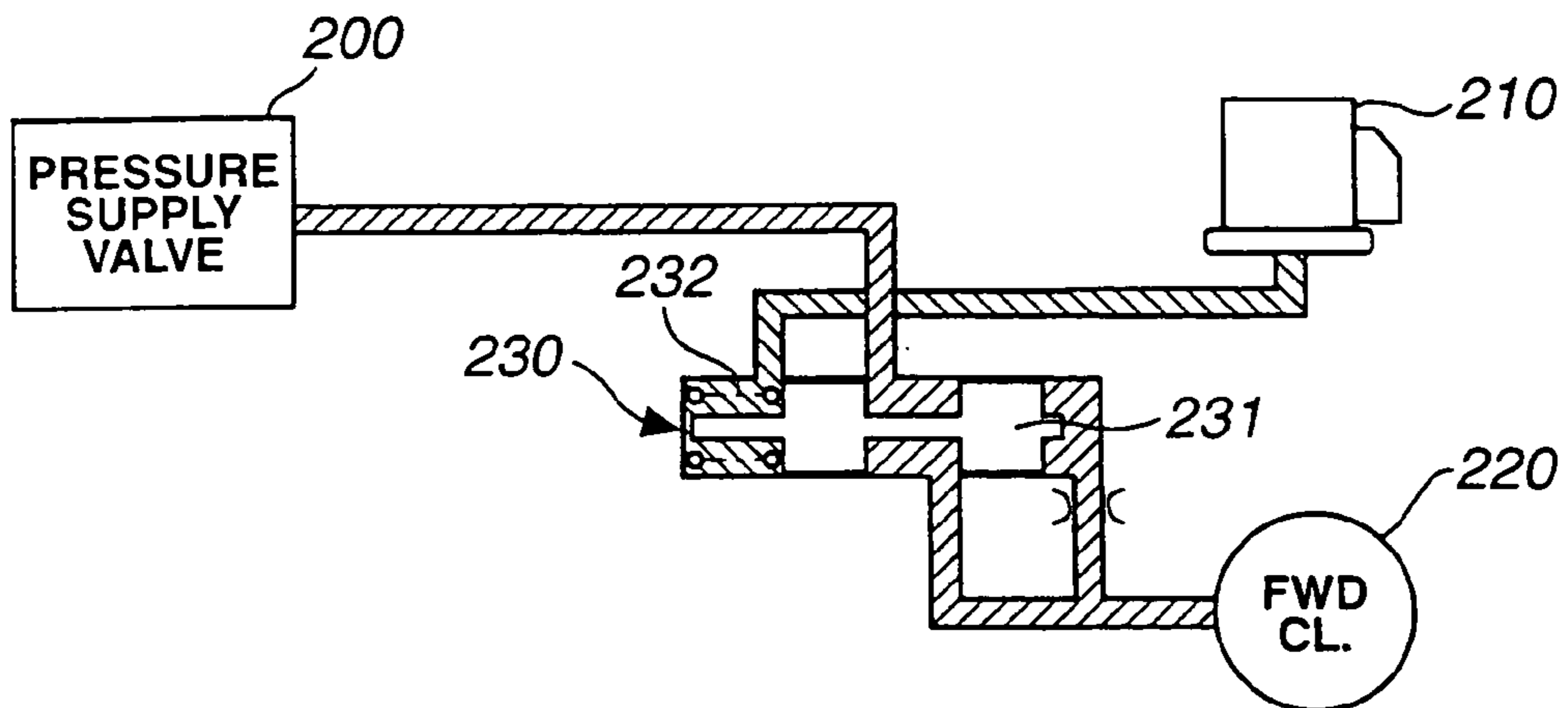
FIG.6 (EARLIER TECHNOLOGY)
