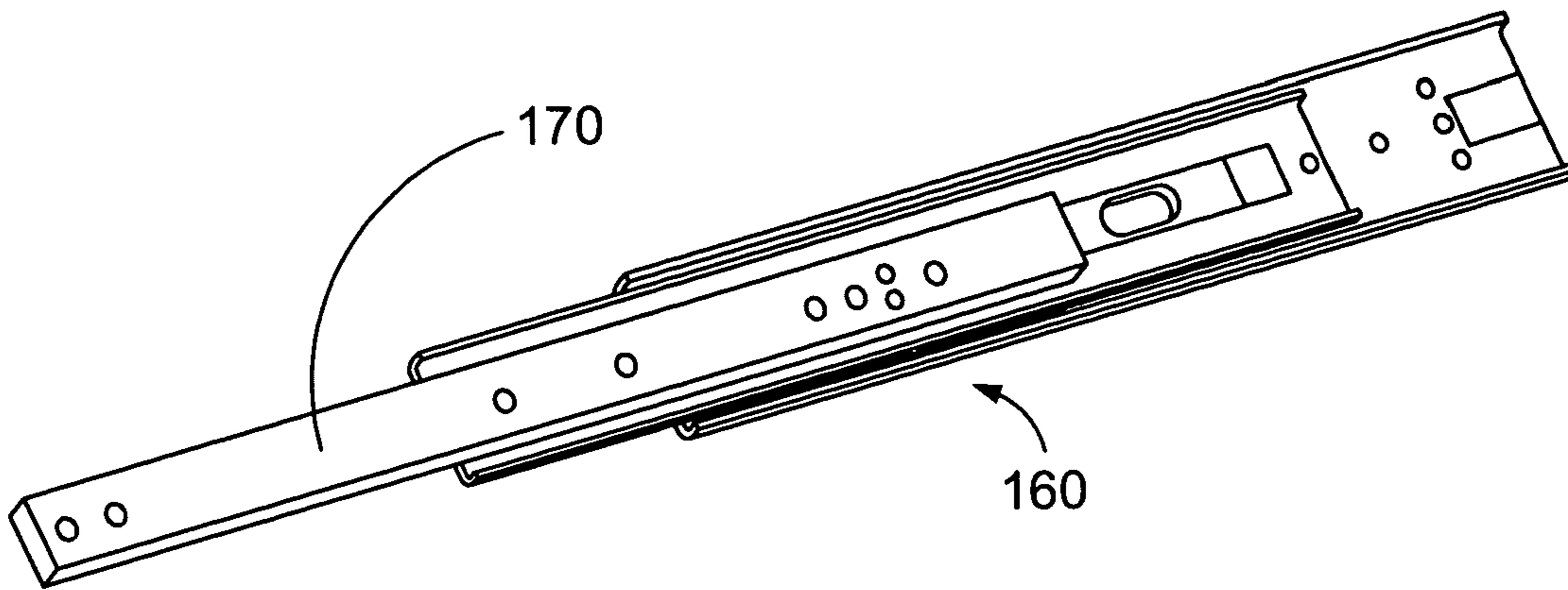
FIG. 3 (Prior Art)
