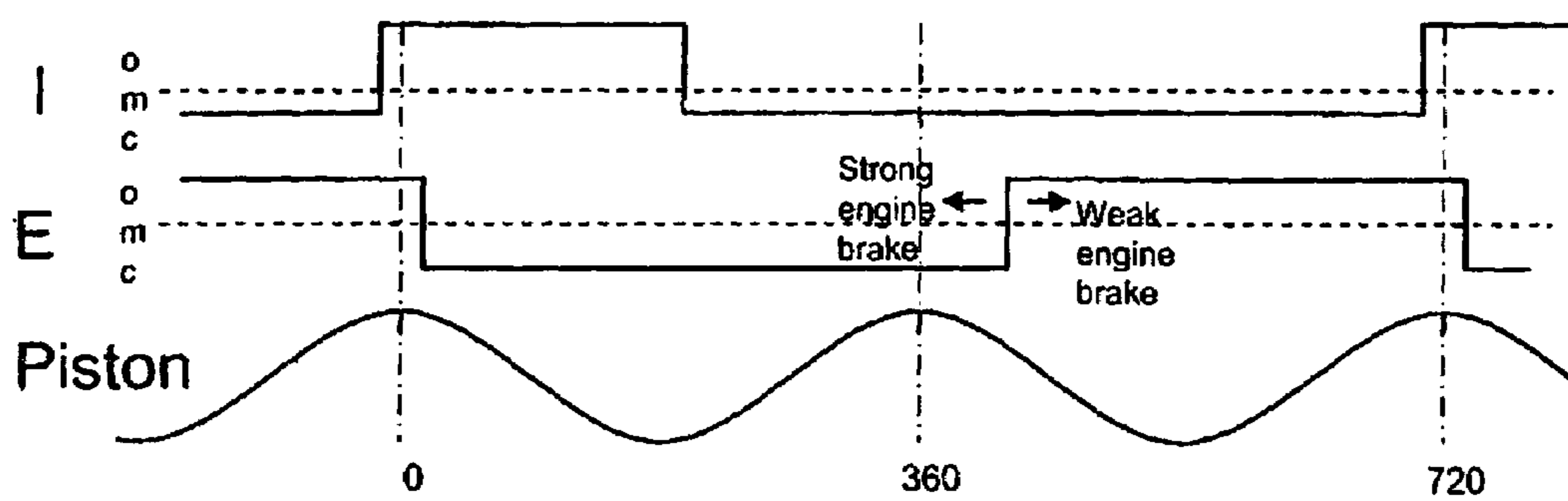
Fig. 20 Prior Art
