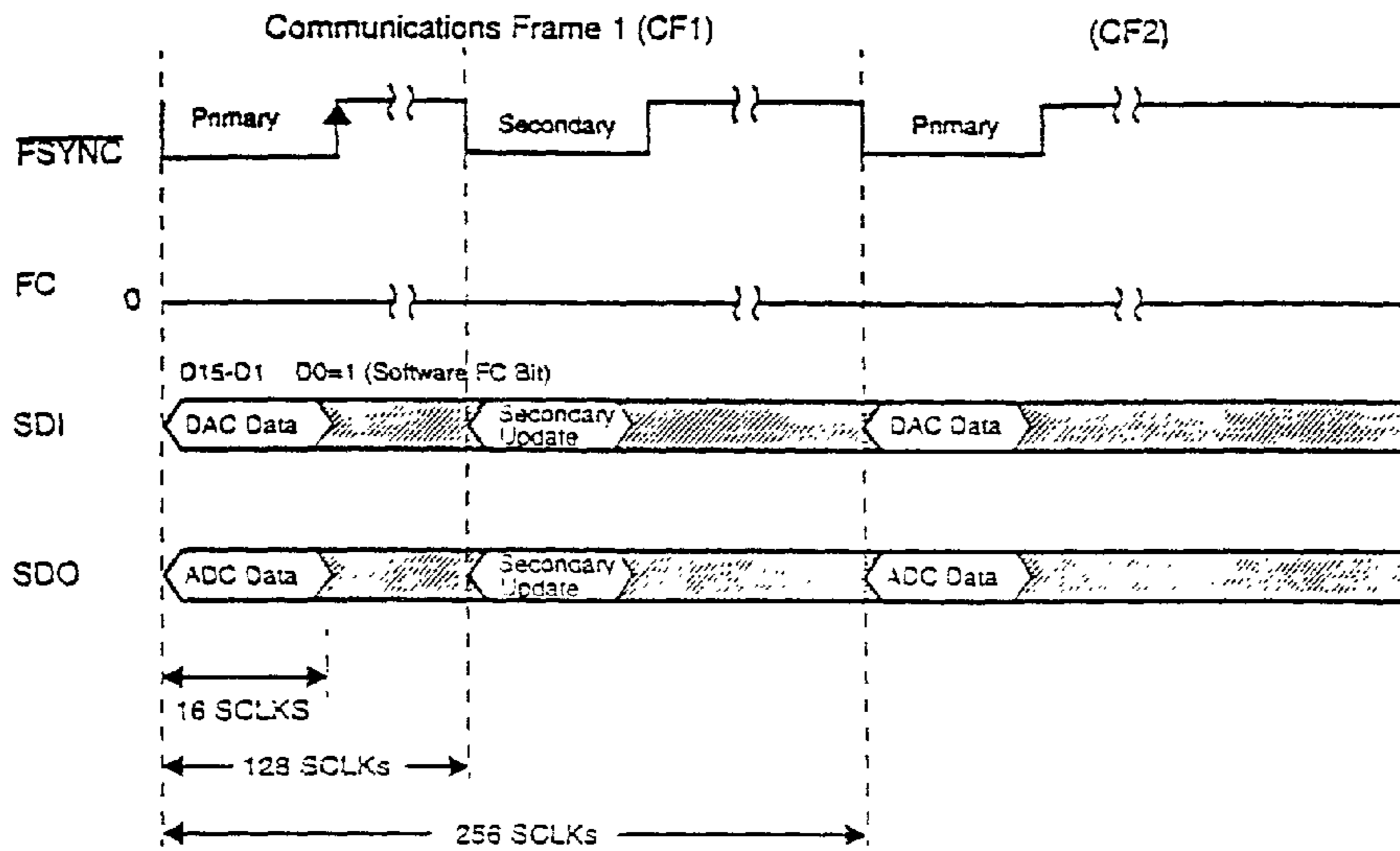
Figure 12. Software FC Secondary Request
