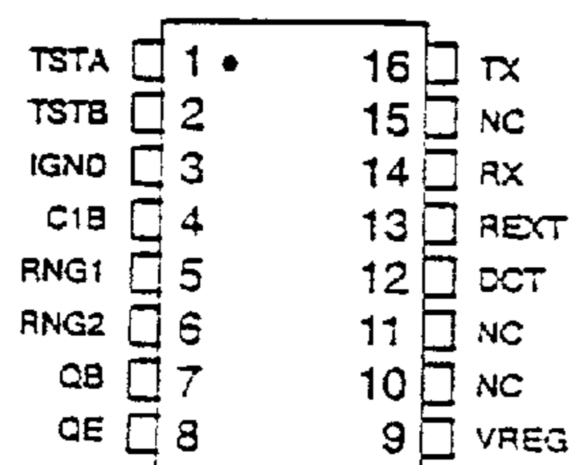
Figure 17. Si3032B Pin Configuration
