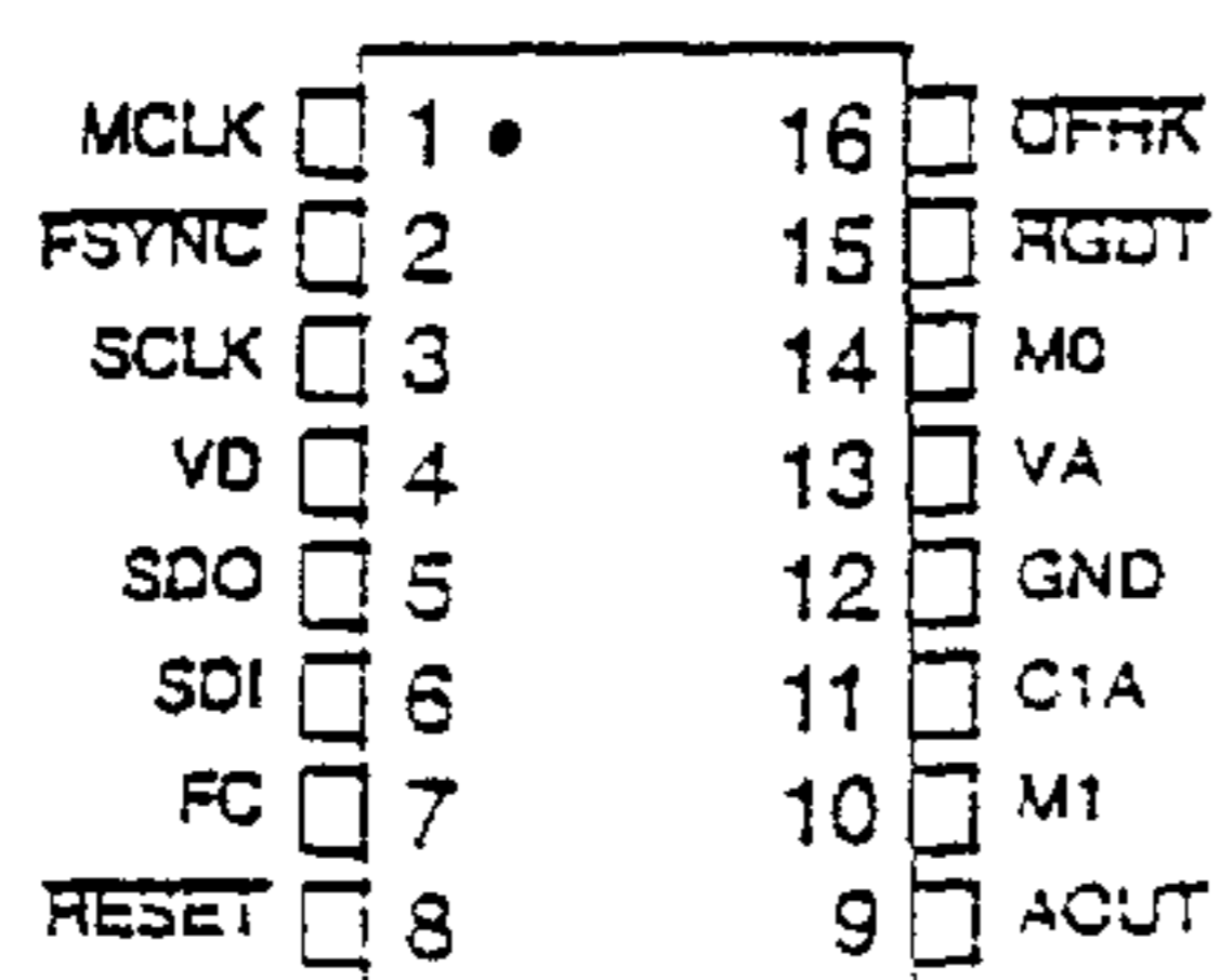
Figure 16. Si3032A Pin Configuration
