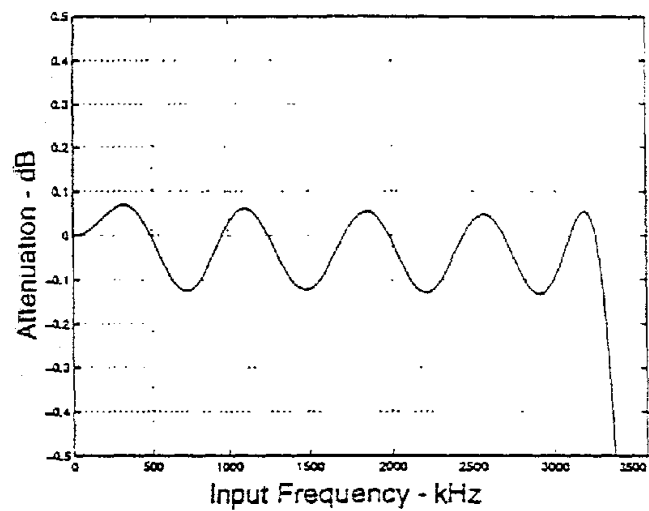
Figure 5. Decimation Filter Passband Ripple
