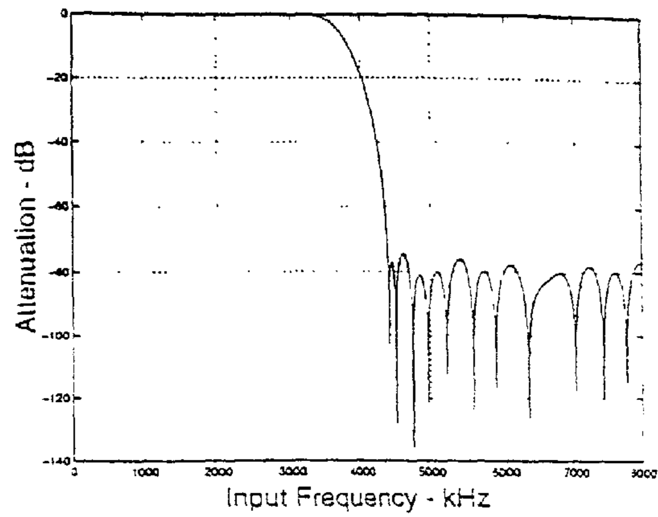
Figure 6. Interpolation Filter Response
