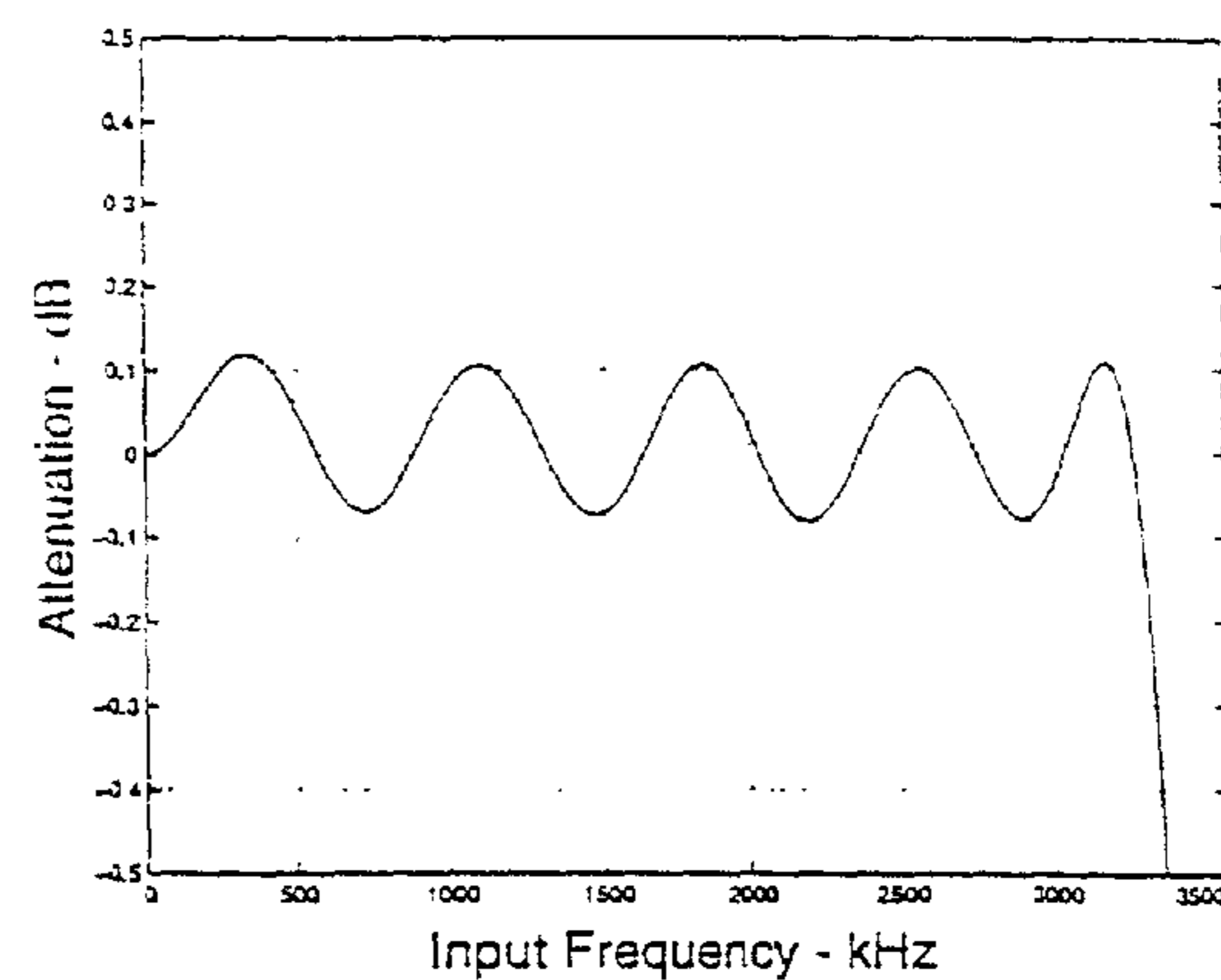
Figure 7. Interpolation Filter Passband Ripple
