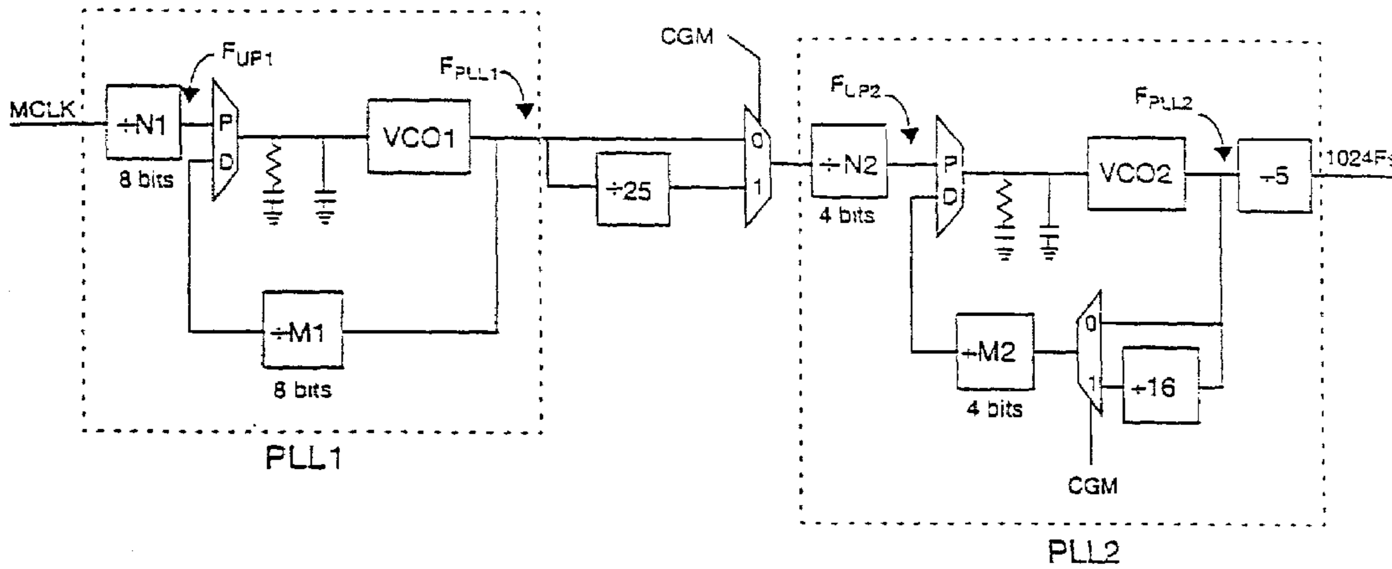
Figure 11. Clock Generation Subsystem
