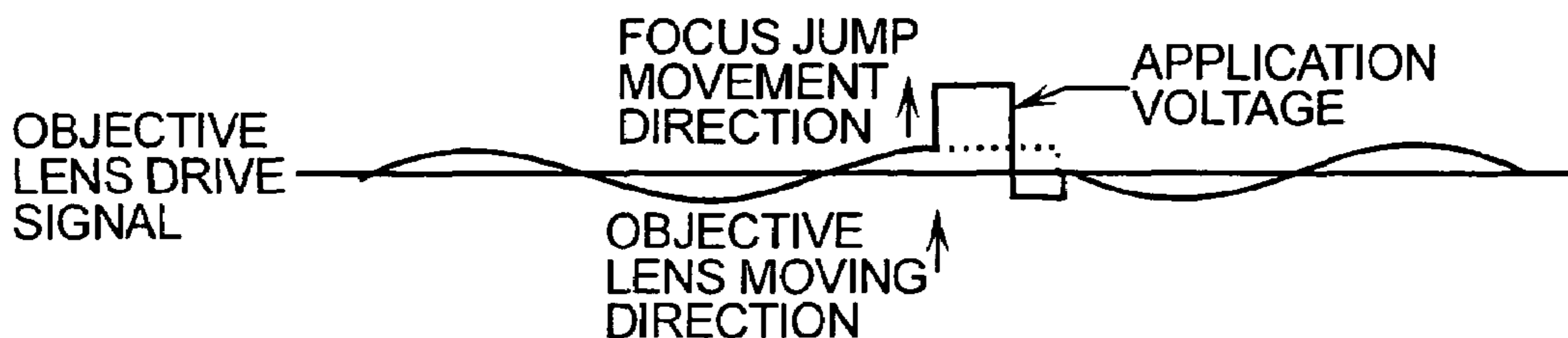
(b) CASE WHERE A VOLTAGE IS APPLIED TO A PEAK OF A SURFACE VIBRATION COMPONENT
