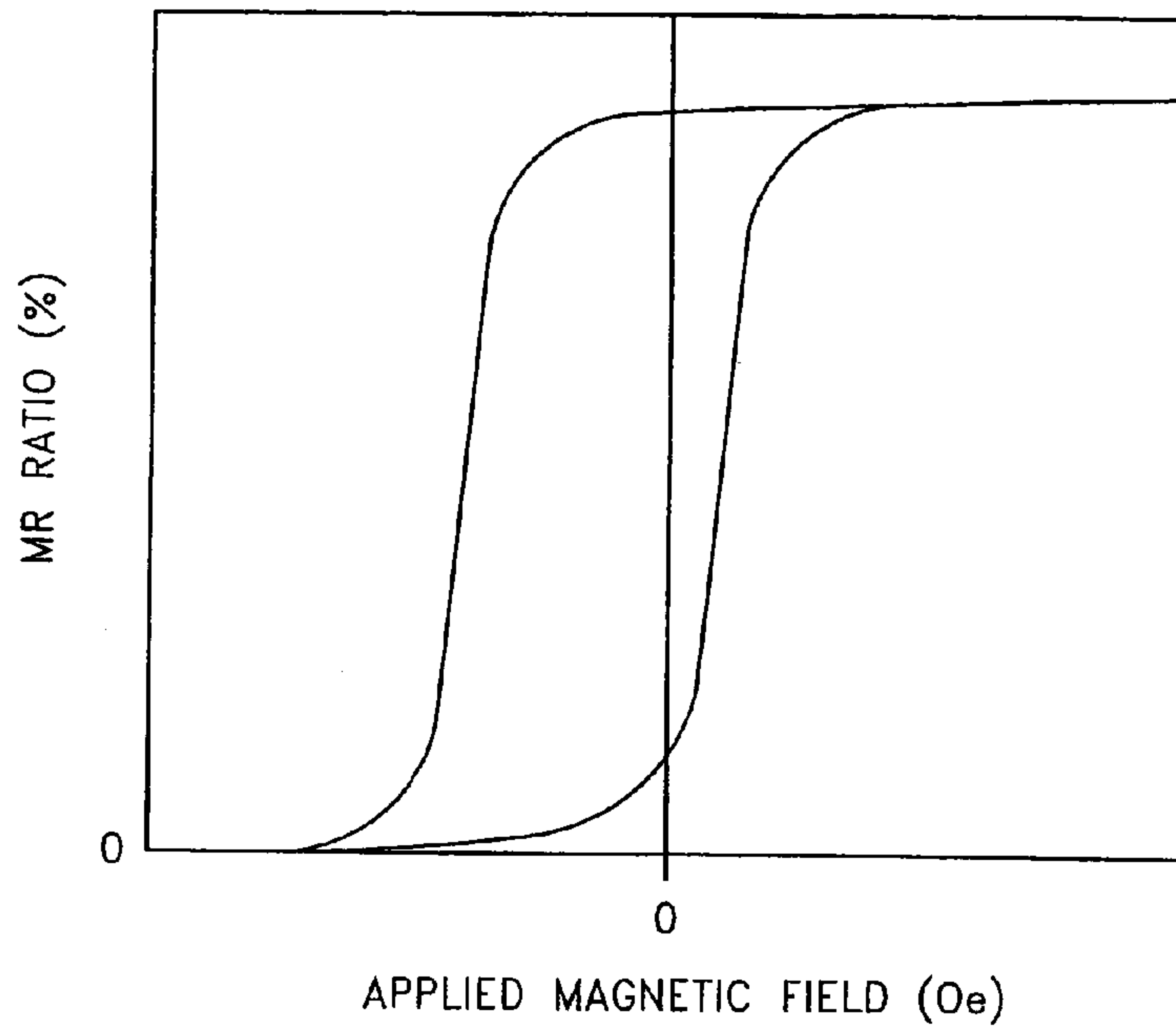
FIG. 1 (PRIOR ART)
