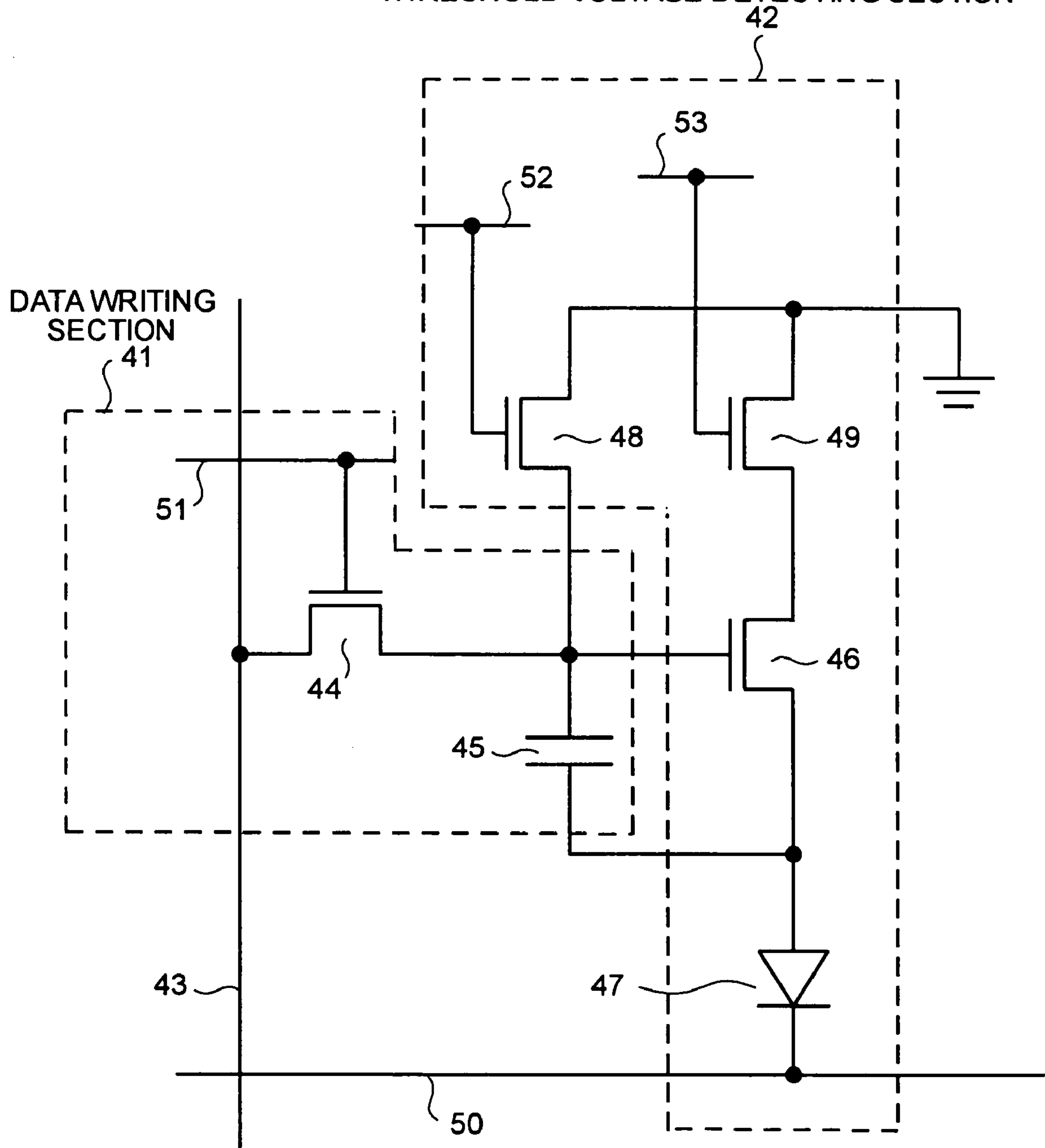
FIG. 17 THRESHOLD VOLTAGE DETECTING SECTION
