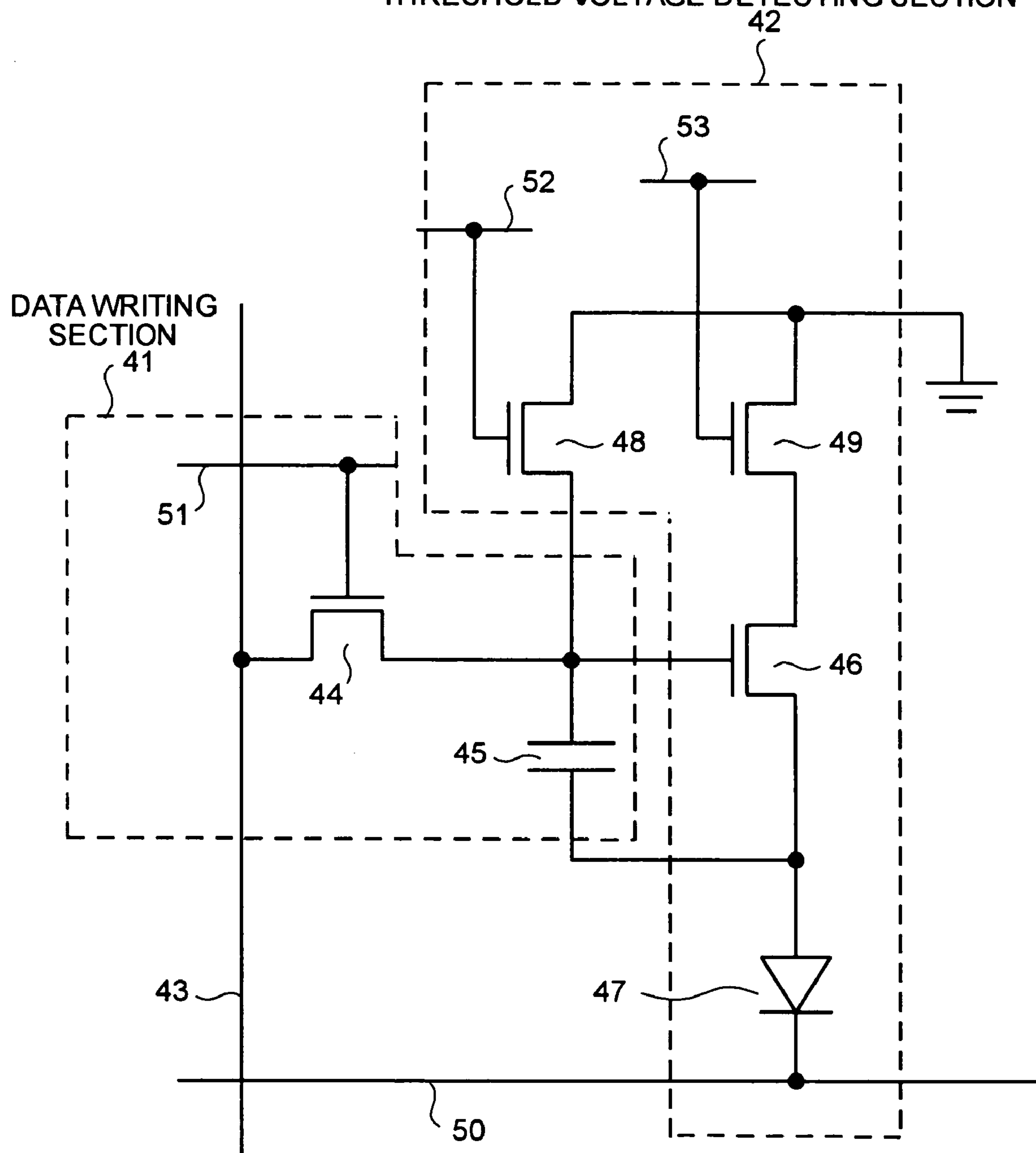
THRESHOLD VOLTAGE DETECTING SECTION
