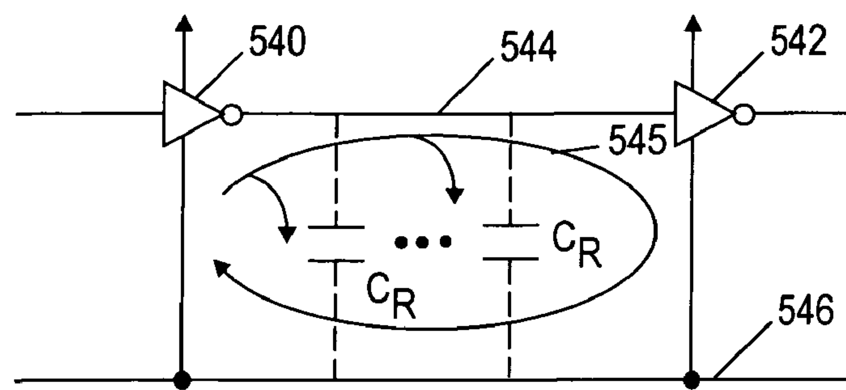
FIG. 7 (PRIOR ART)
