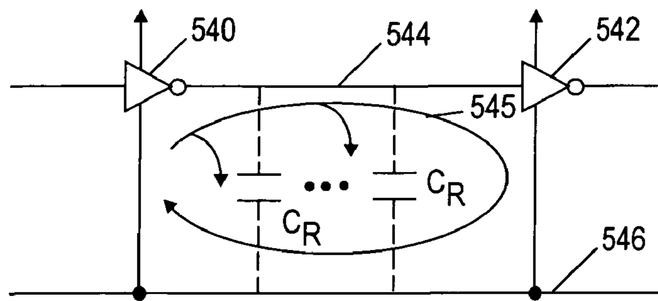
FIG. 7 (PRIOR ART)
