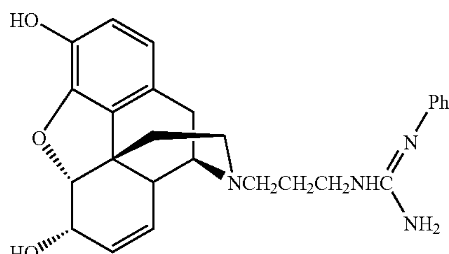
KRS-6-22
