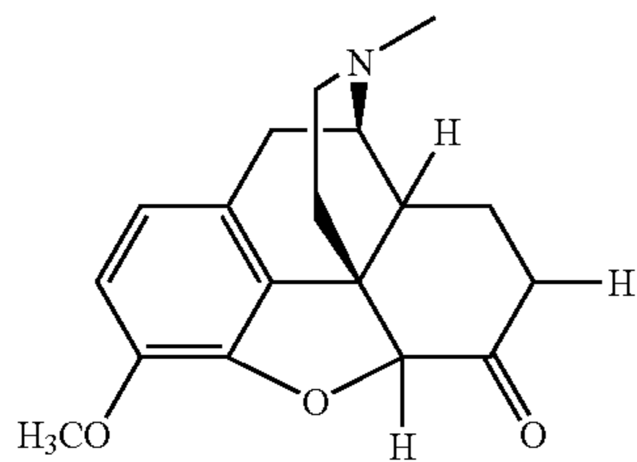
hydrocodone,
