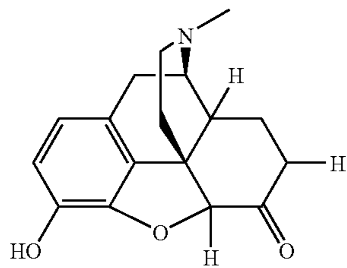
hydromorphone,
