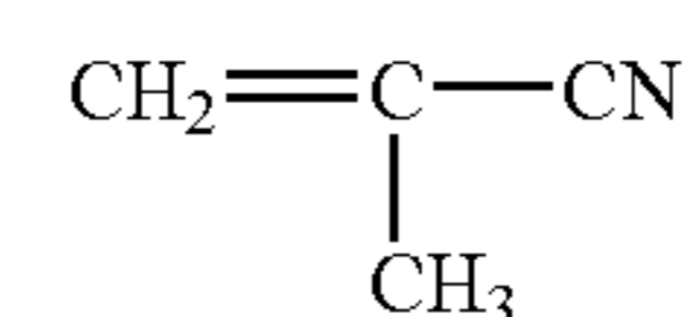
methacrylonitrile
