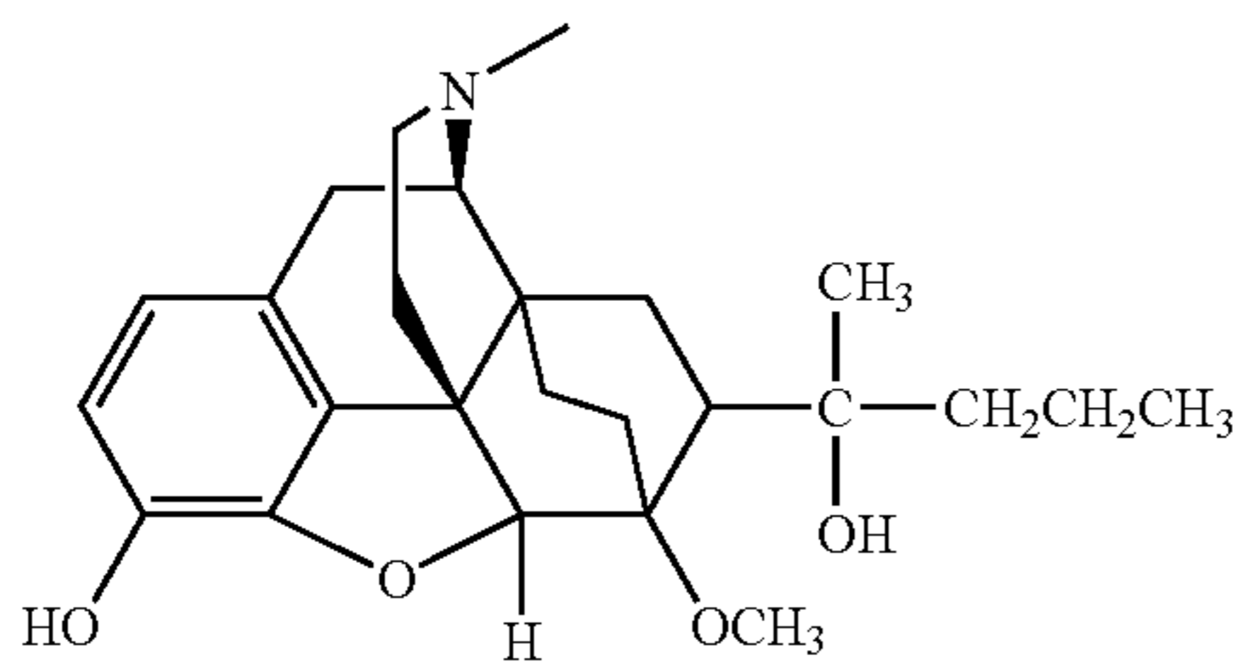
dihydroetorphine, and
