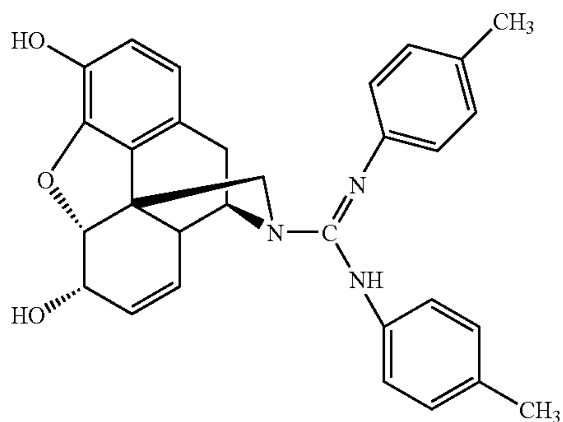
KRS-6-85
