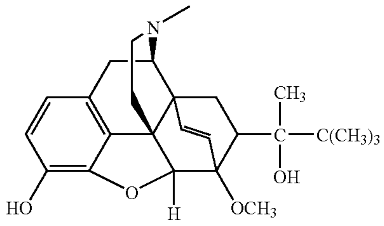
buprenorphine,
