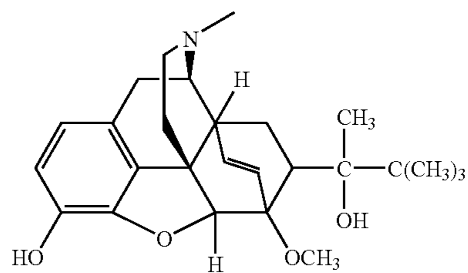
buprenorphine.
