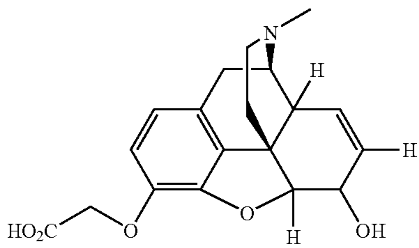
O-carboxymethylmorphine,
