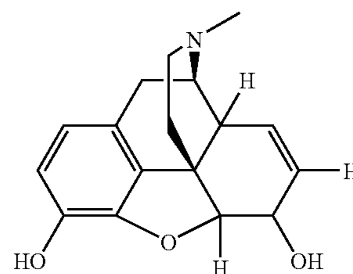
morphine,
