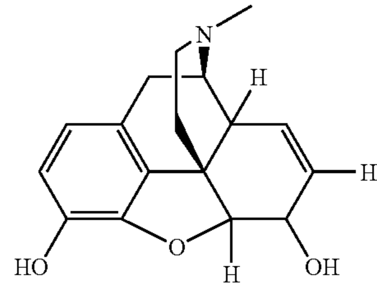
morphine,
