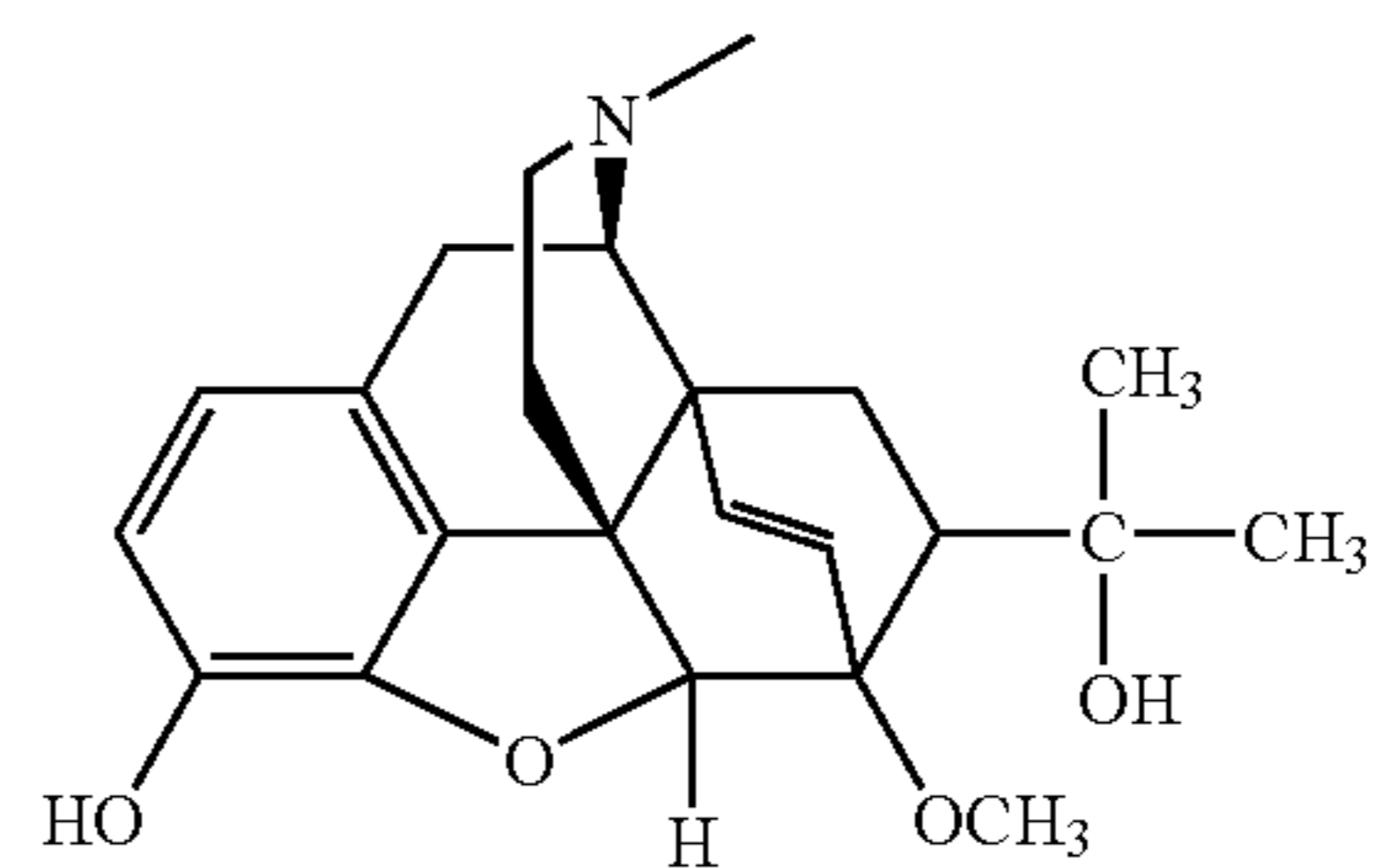
diprenorphine,
