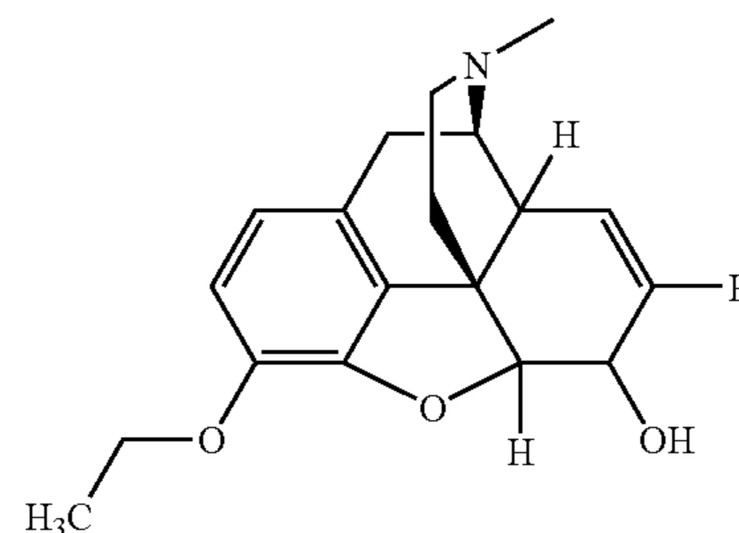
ethylmorphine,
