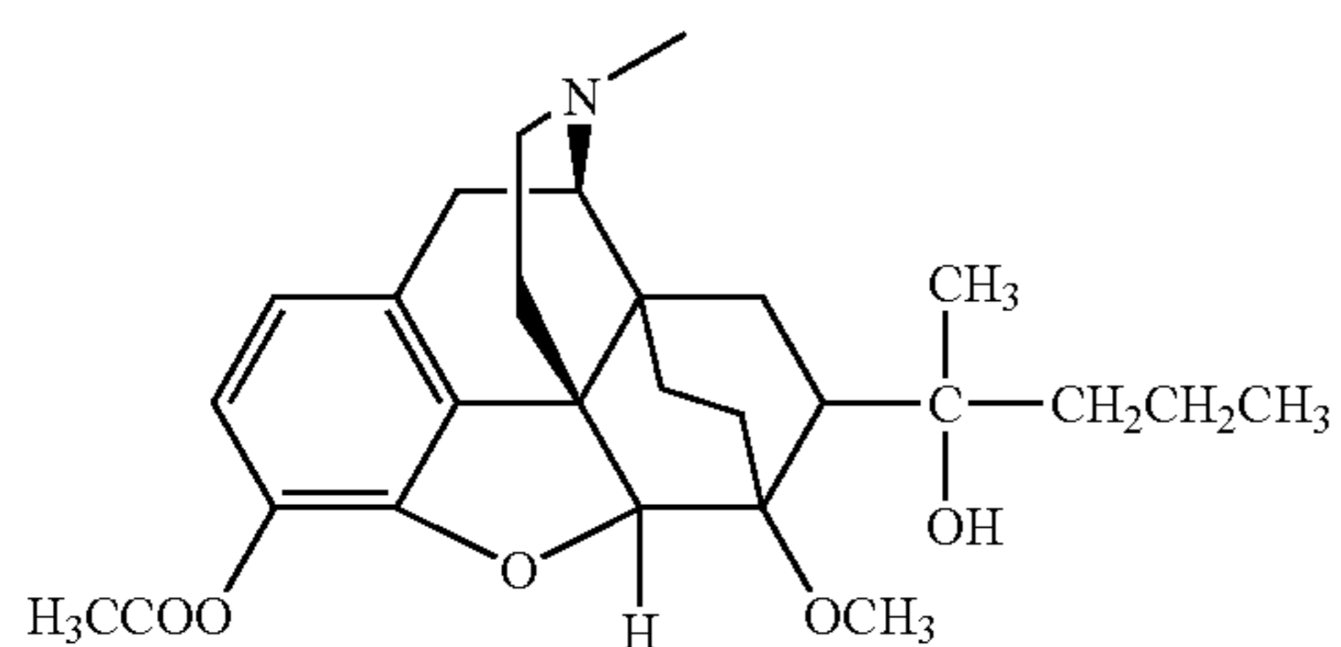
dihydroacetorphine.
