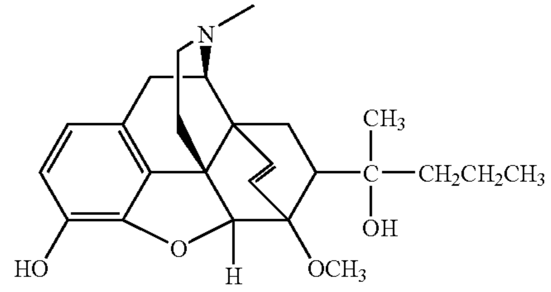
etorphine,
