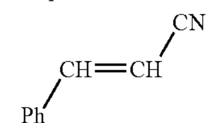
3-phenylacrylonitrile
