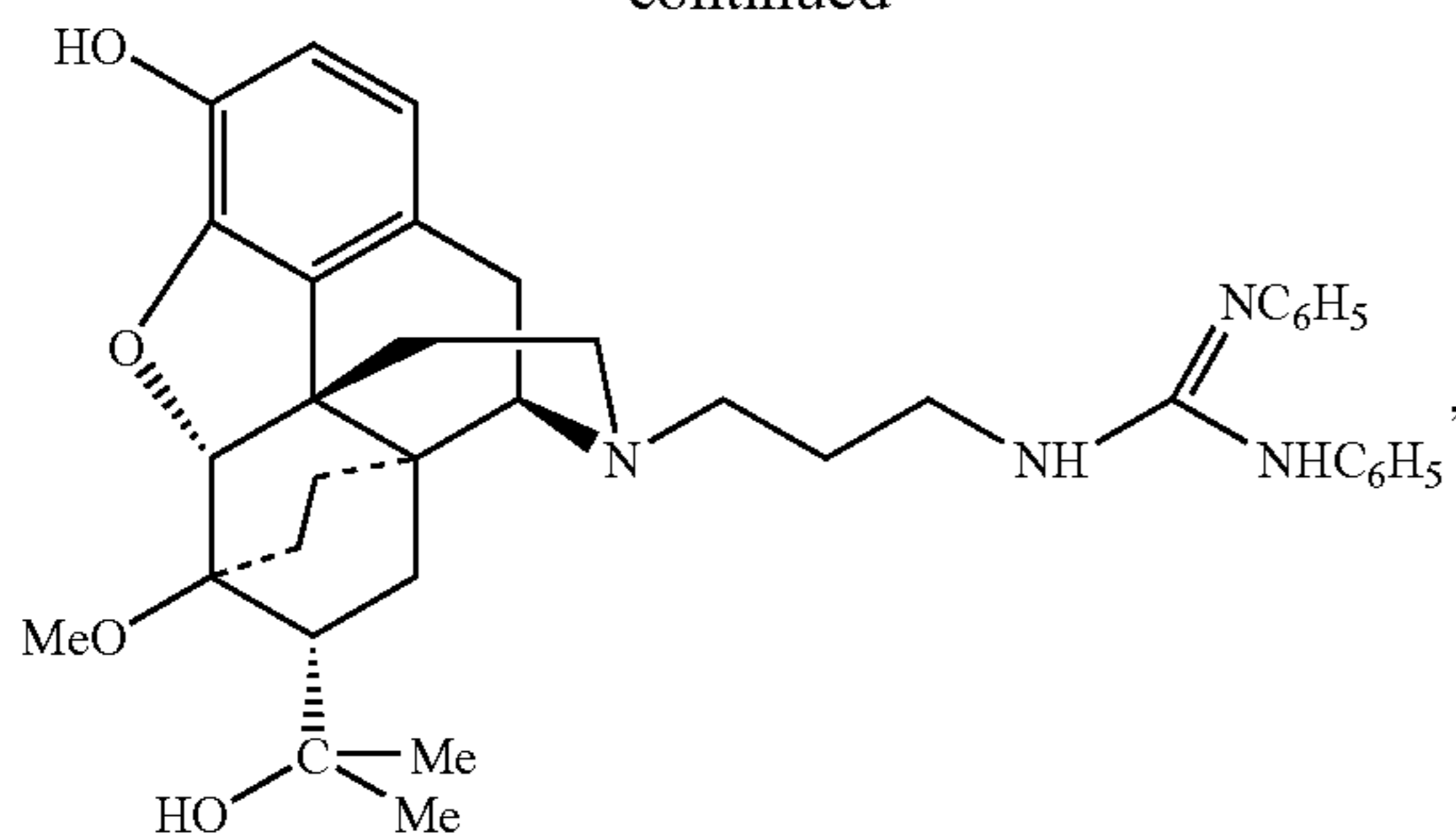
KRS-6-79
