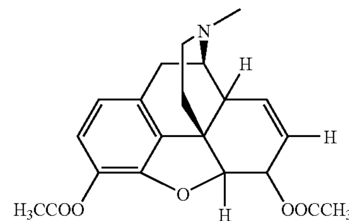
heroin,
