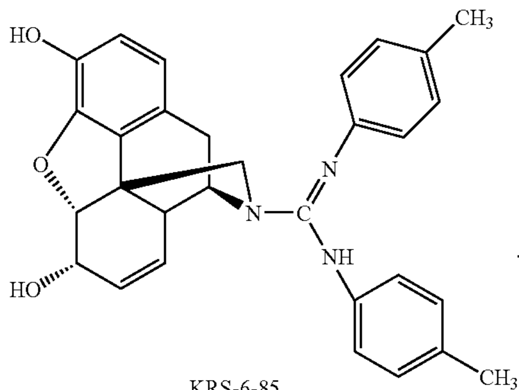
KRS-6-85
