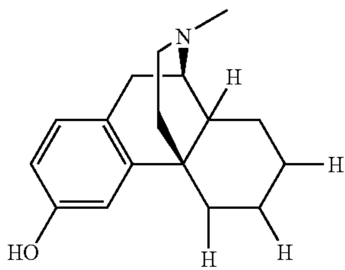
phenomorphan,
