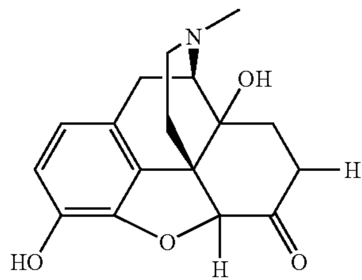
oxymorphone,
