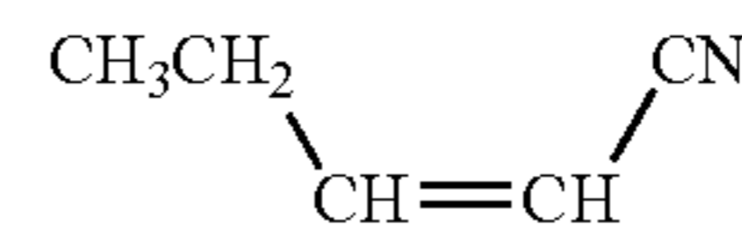
cis-pent-2-ene nitrile
