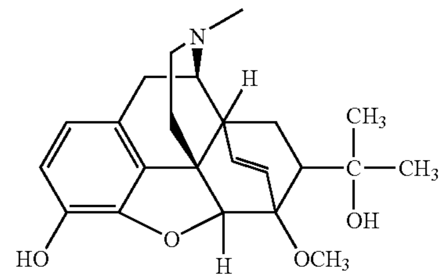
diprenorphine,
