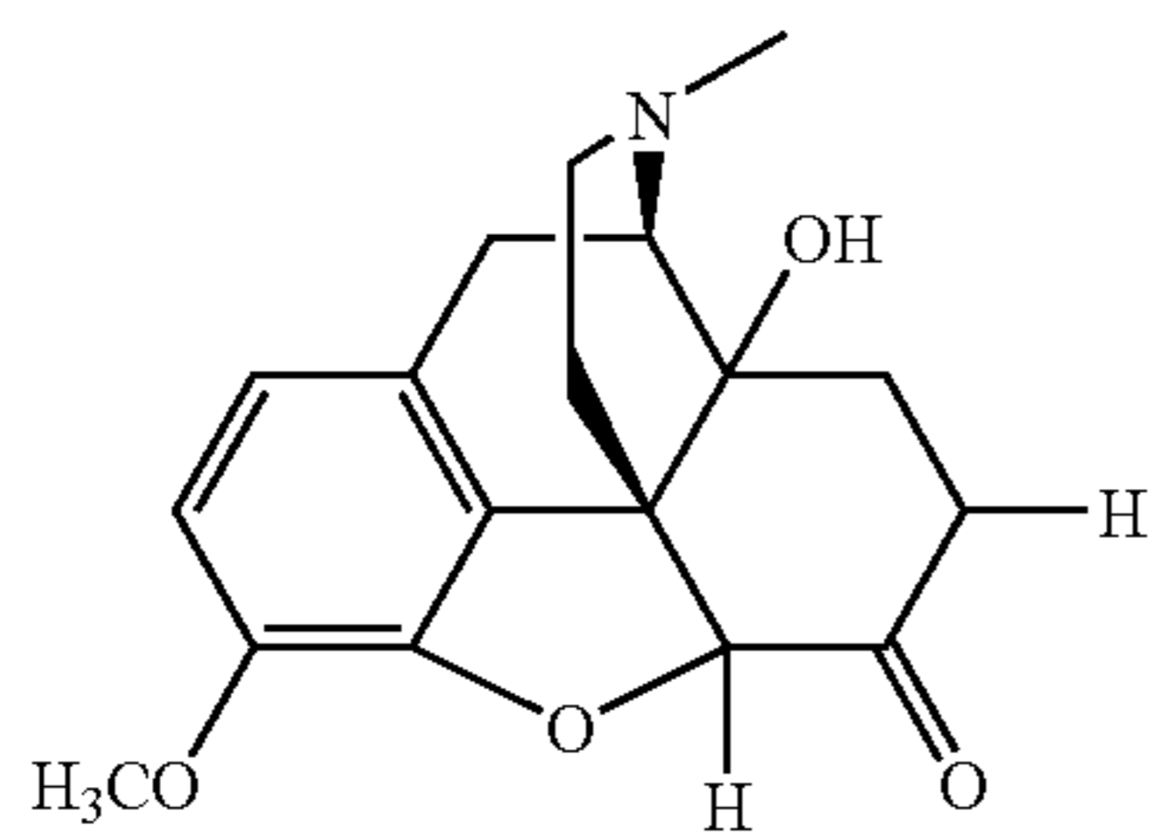
oxycodone,
