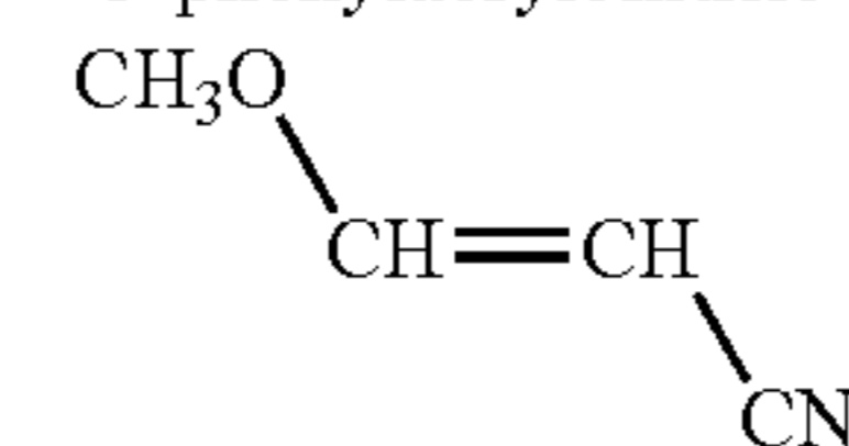
methoxy acrylonitrile
