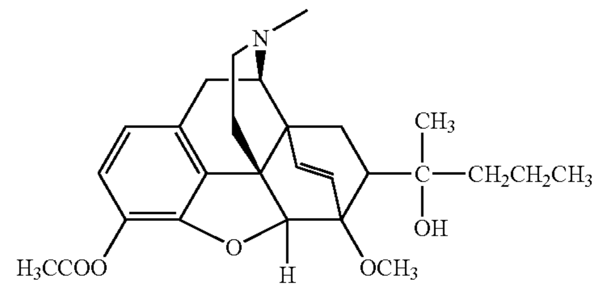
acetorphine,
