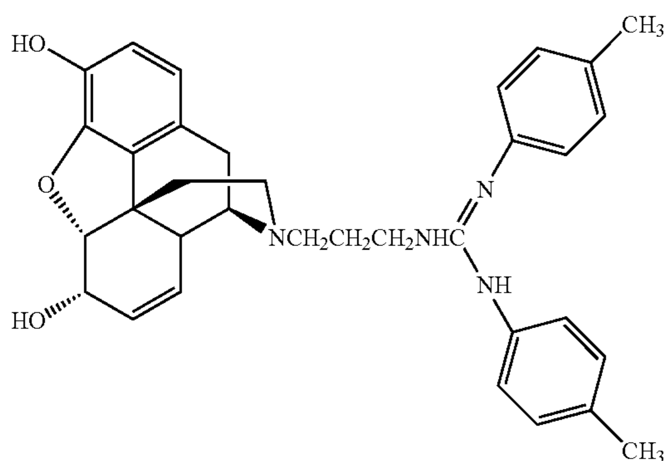
KRS-6-26
