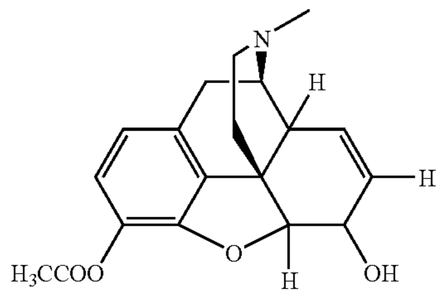
O-acetlmorphine,
