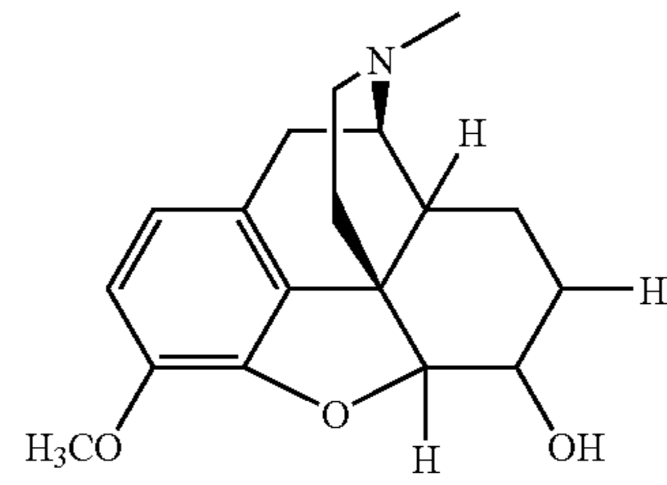
dihydrocodeine,
