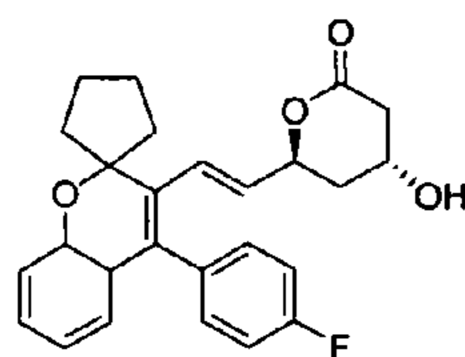
Bervastatin Lactone Figure 6k
