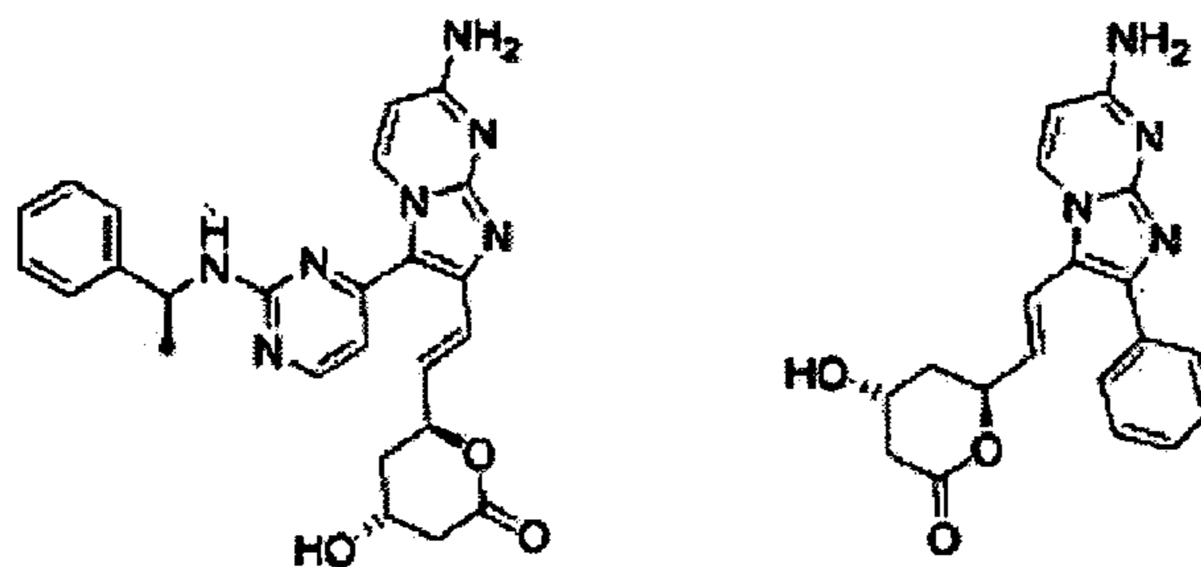
Figure 5d (pyrrolo[2,3- b ]pyrimidines)
