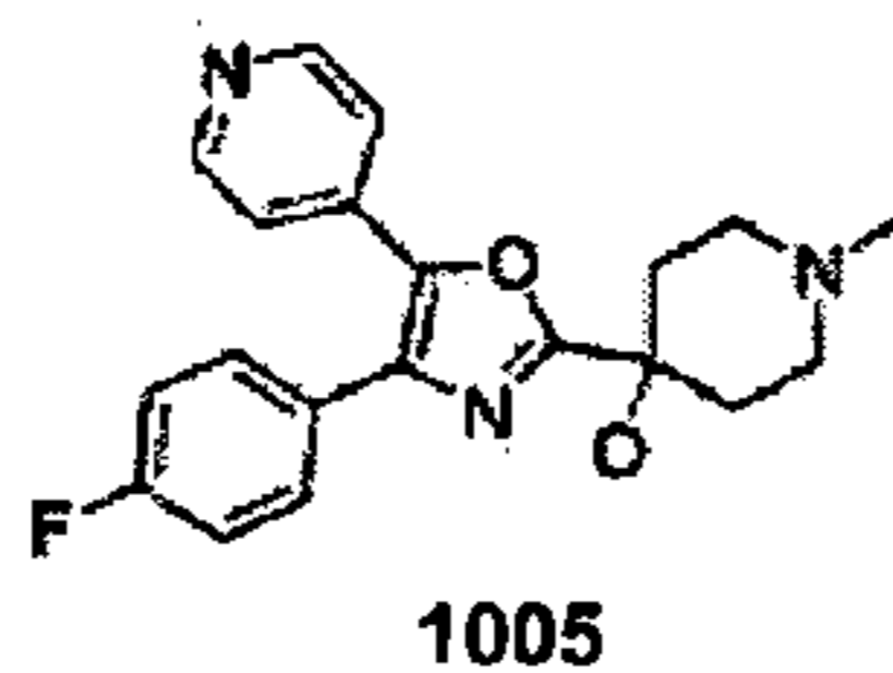
Figure 4b (oxazole)
