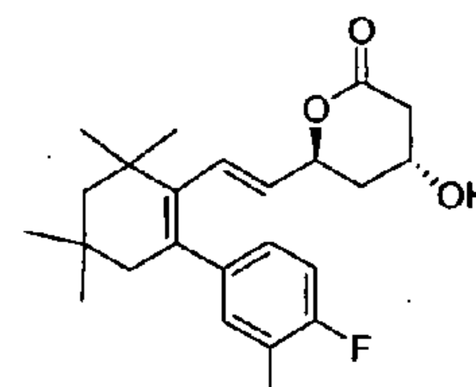
Dalvastatin Lactone Figure 6l
