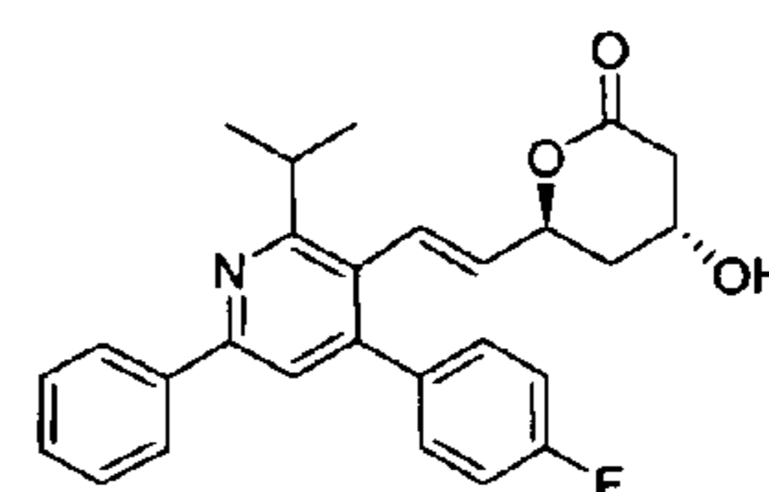
Glenvastatin Lactone Figure 6f
