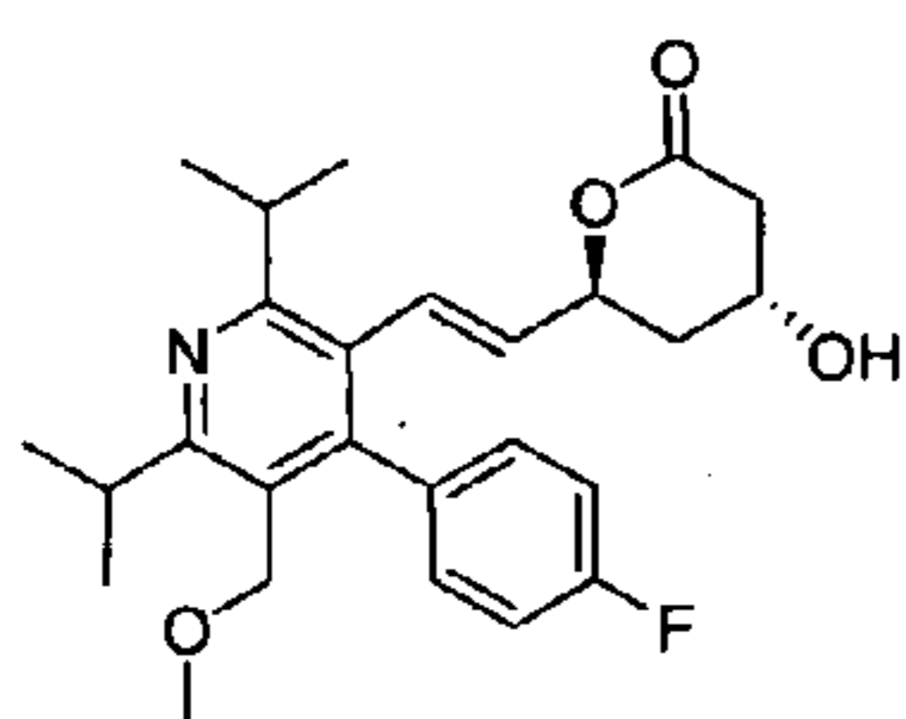
Cerivastatin Lactone Figure 6d
