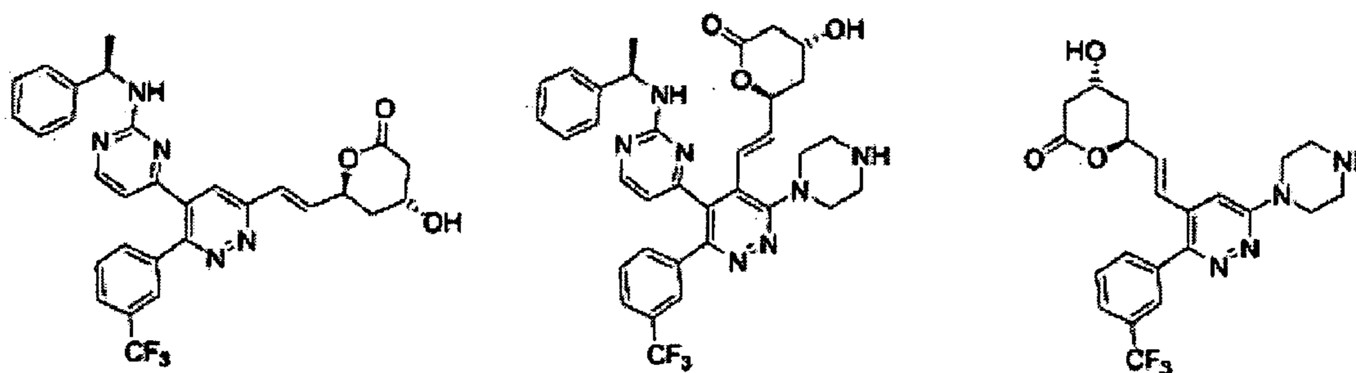
Figure 5f (1,2-pyrazines)
