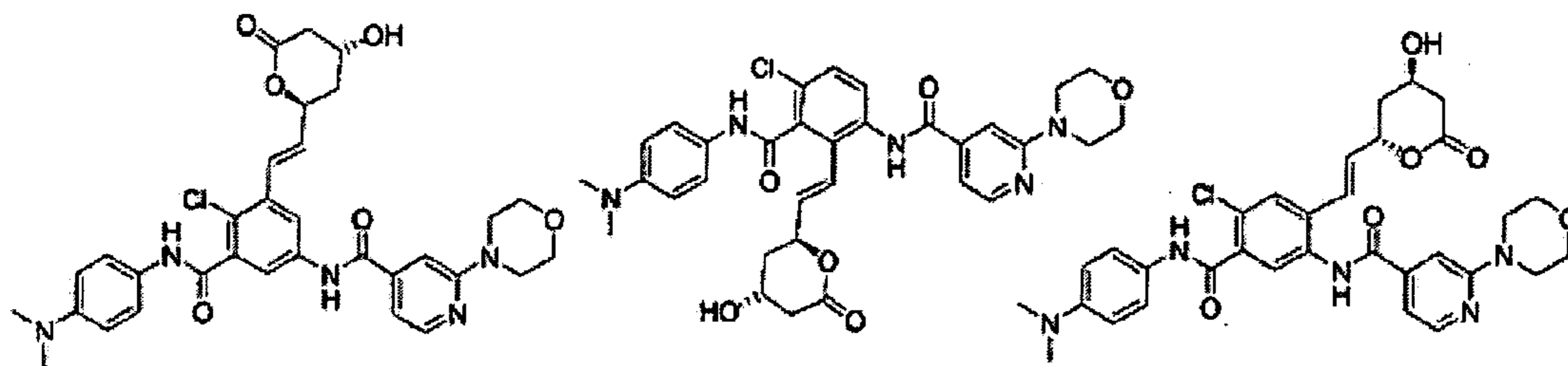
Figure 5i (3-amidobenzamides)
