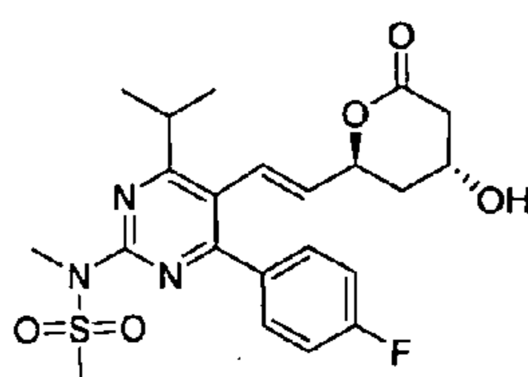
Rosuvastatin Lactone Figure 6e
