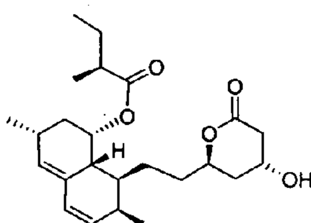
Lovastatin Lactone Figure 6h
