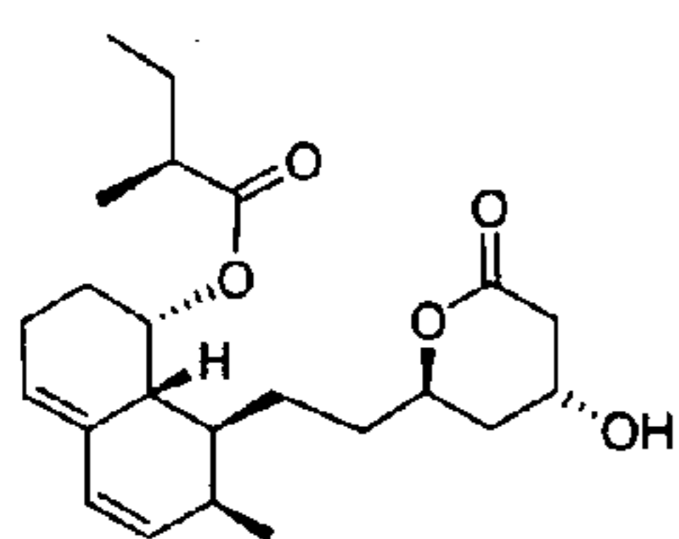
Mevastatin Lactone Figure 6j
