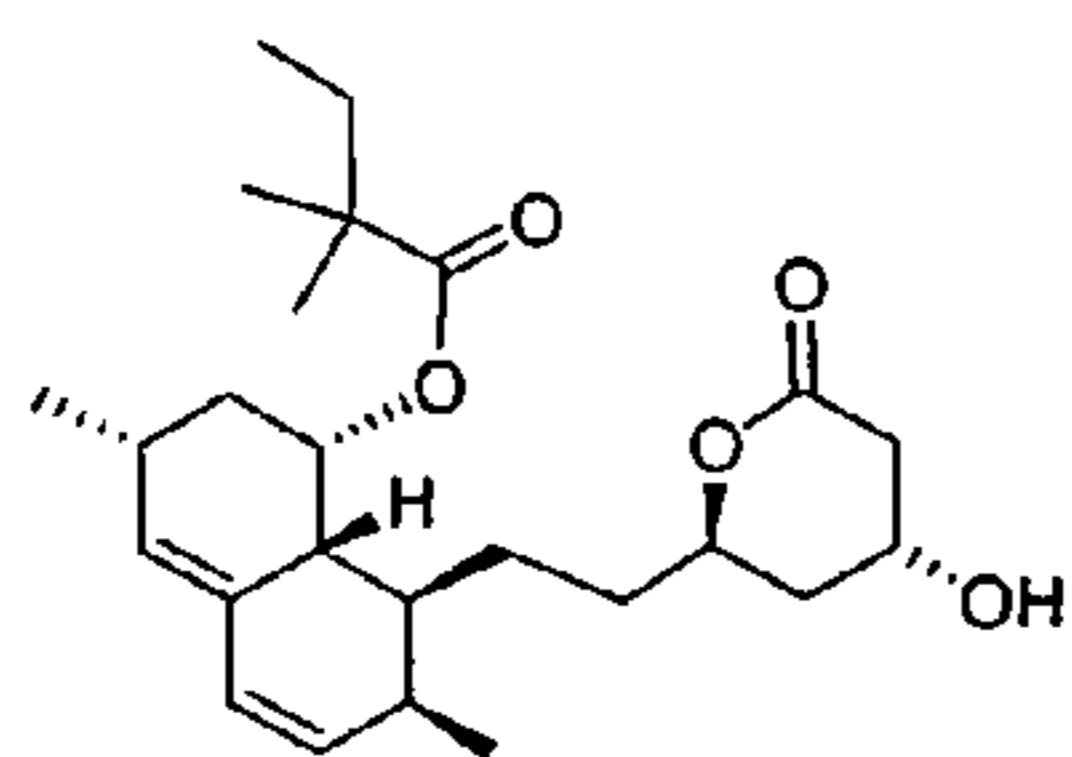
Simvastatin Lactone Figure 6g
