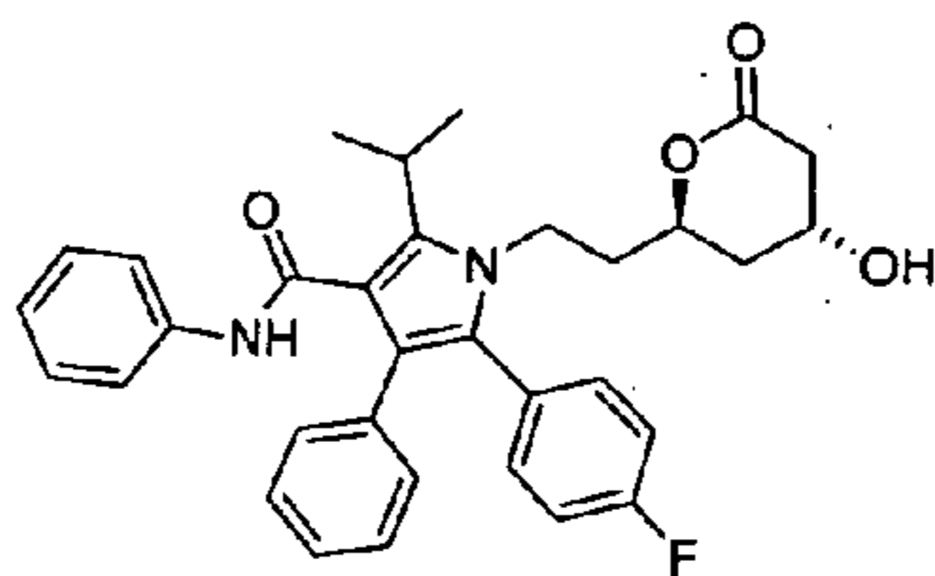
Atorvastatin Lactone Figure 6b
