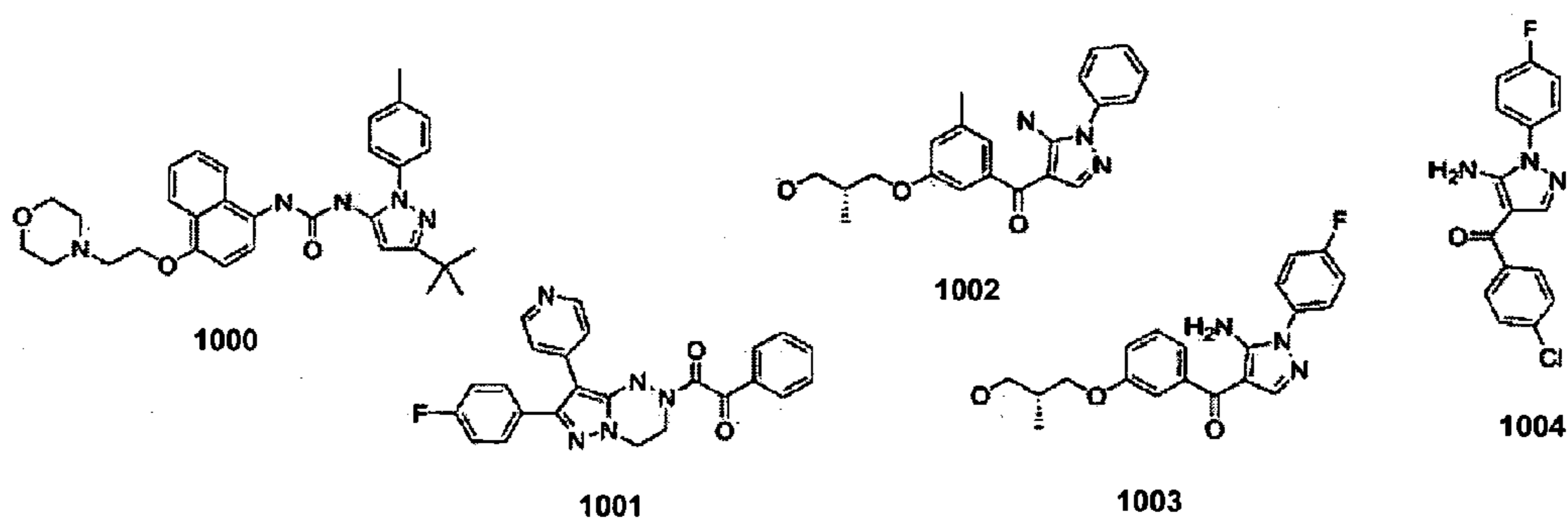
Figure 4a (pyrazoles)
