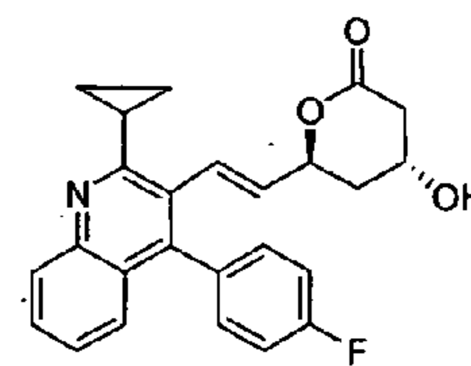
Pitavastatin Lactone Figure 6c
