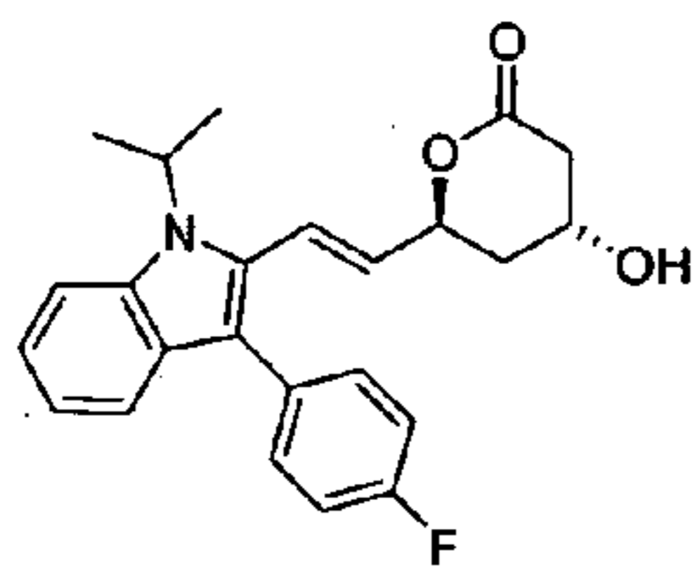
Fluvastatin Lactone Figure 6a
