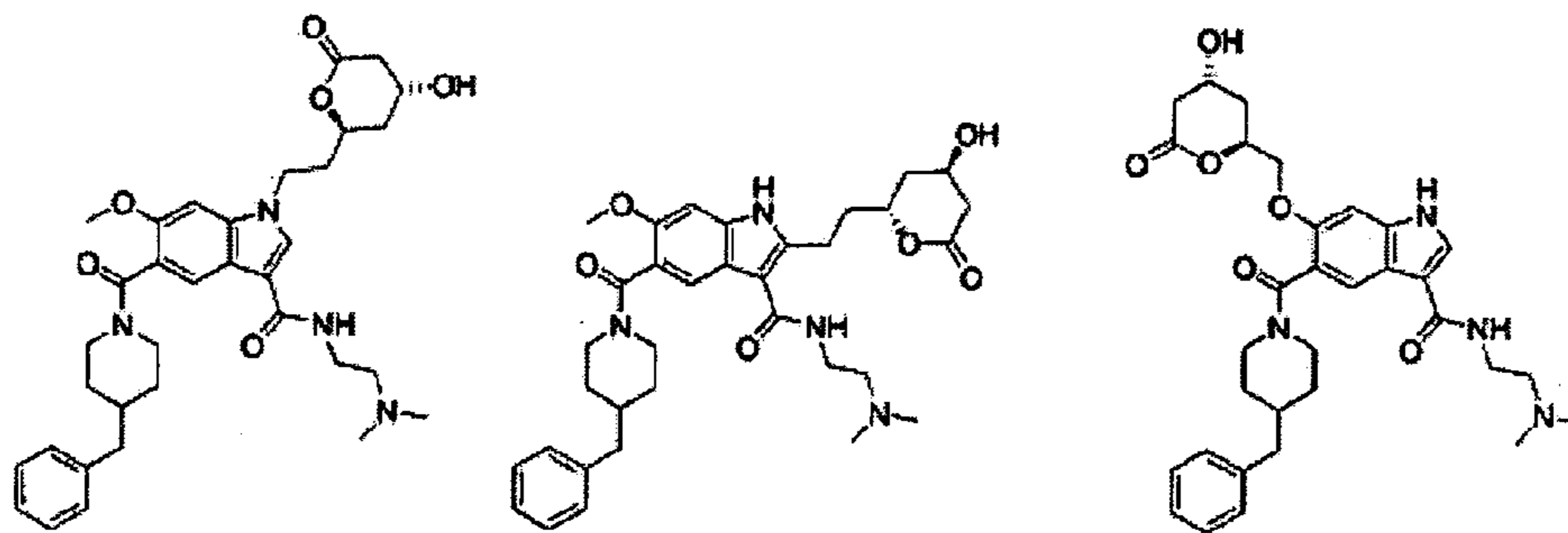
Figure 5l (indoles)
