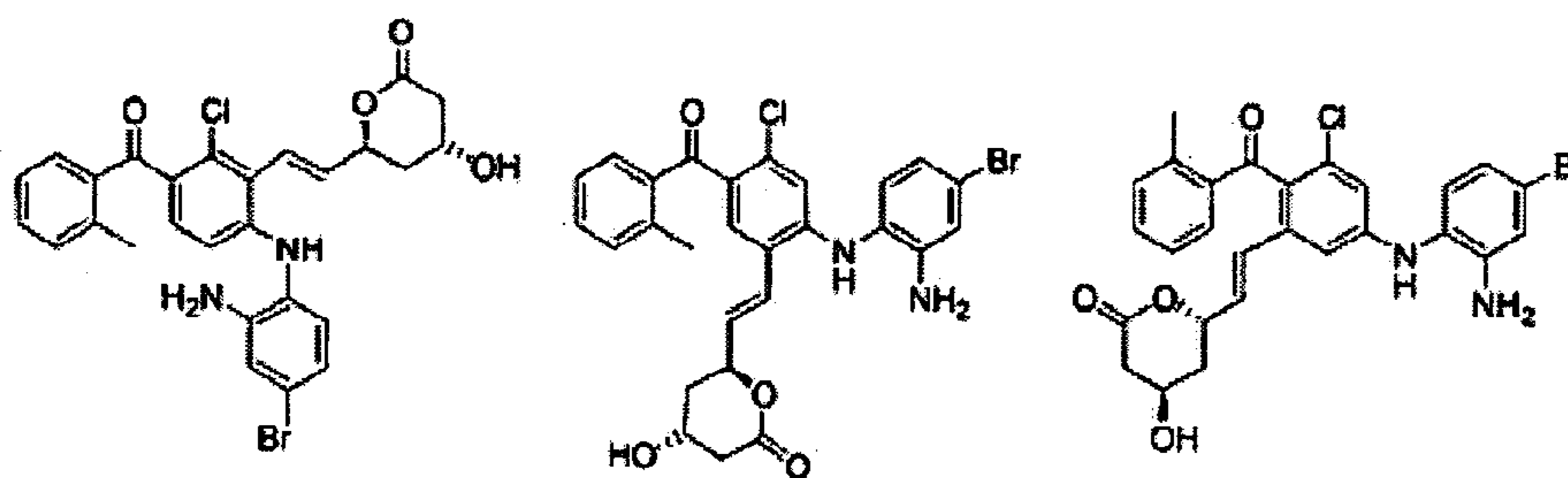
Figure 5h (4-aminobenzophenones)
