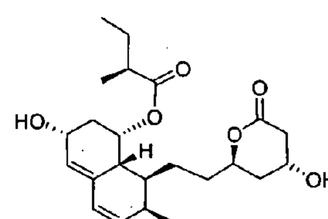
Pravastatin Lactone Figure 6i
