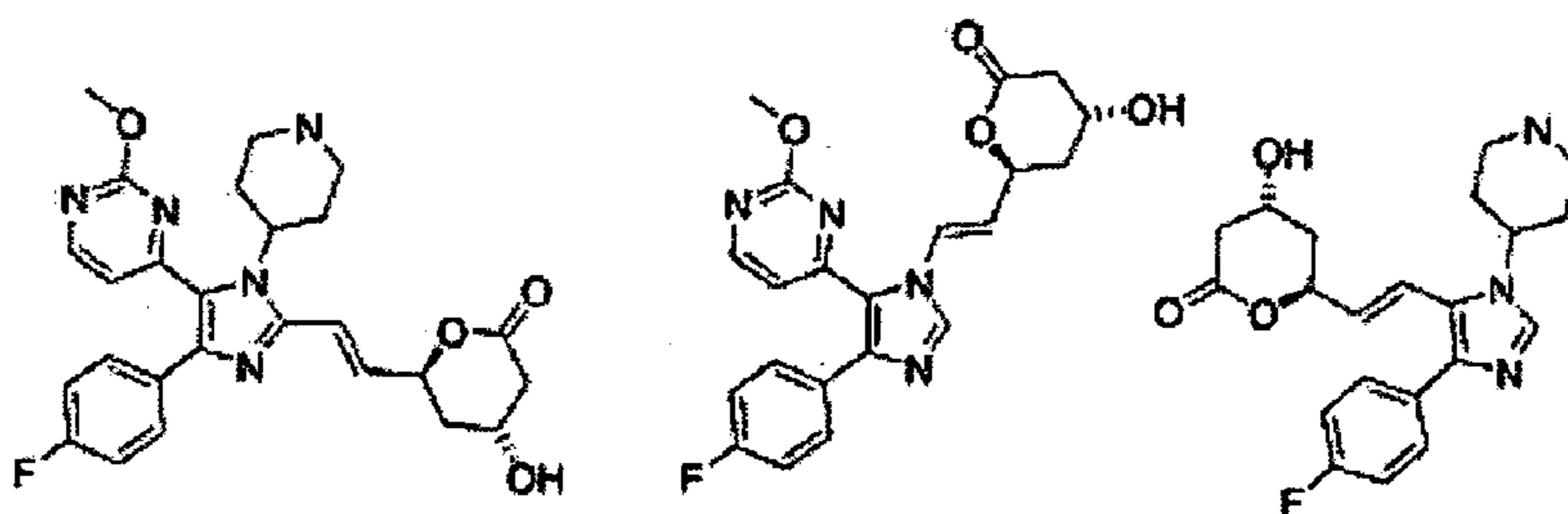
Figure 5c (imidazoles)
