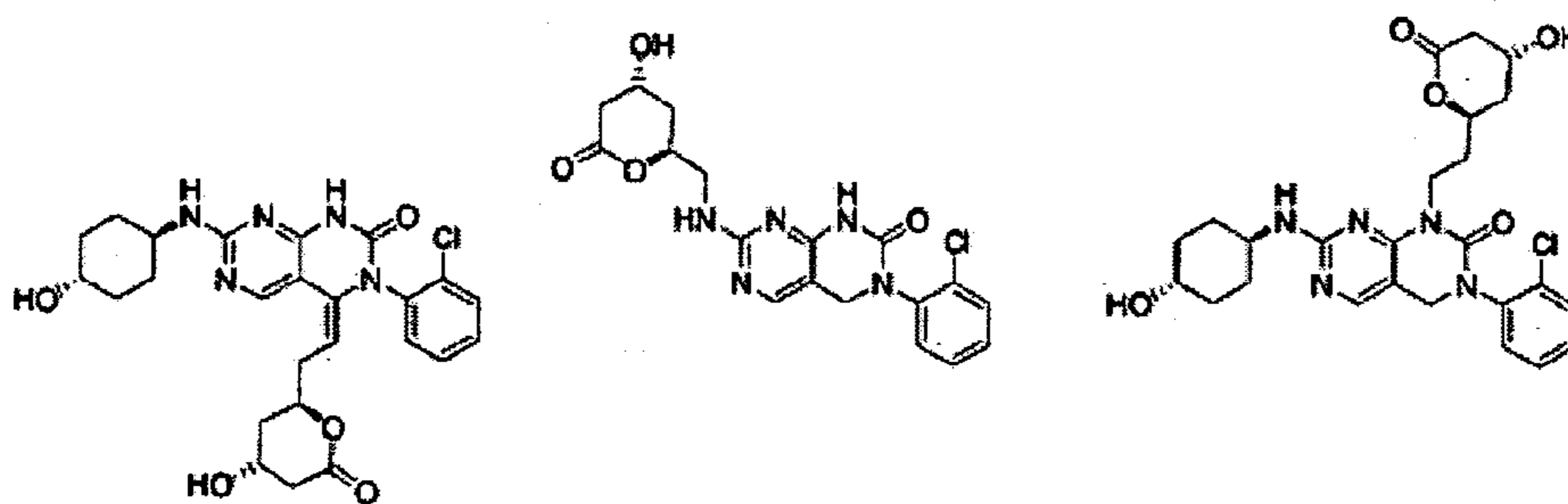
Figure 5k (pyrimidino[4,5-d]pyrimidinones)
