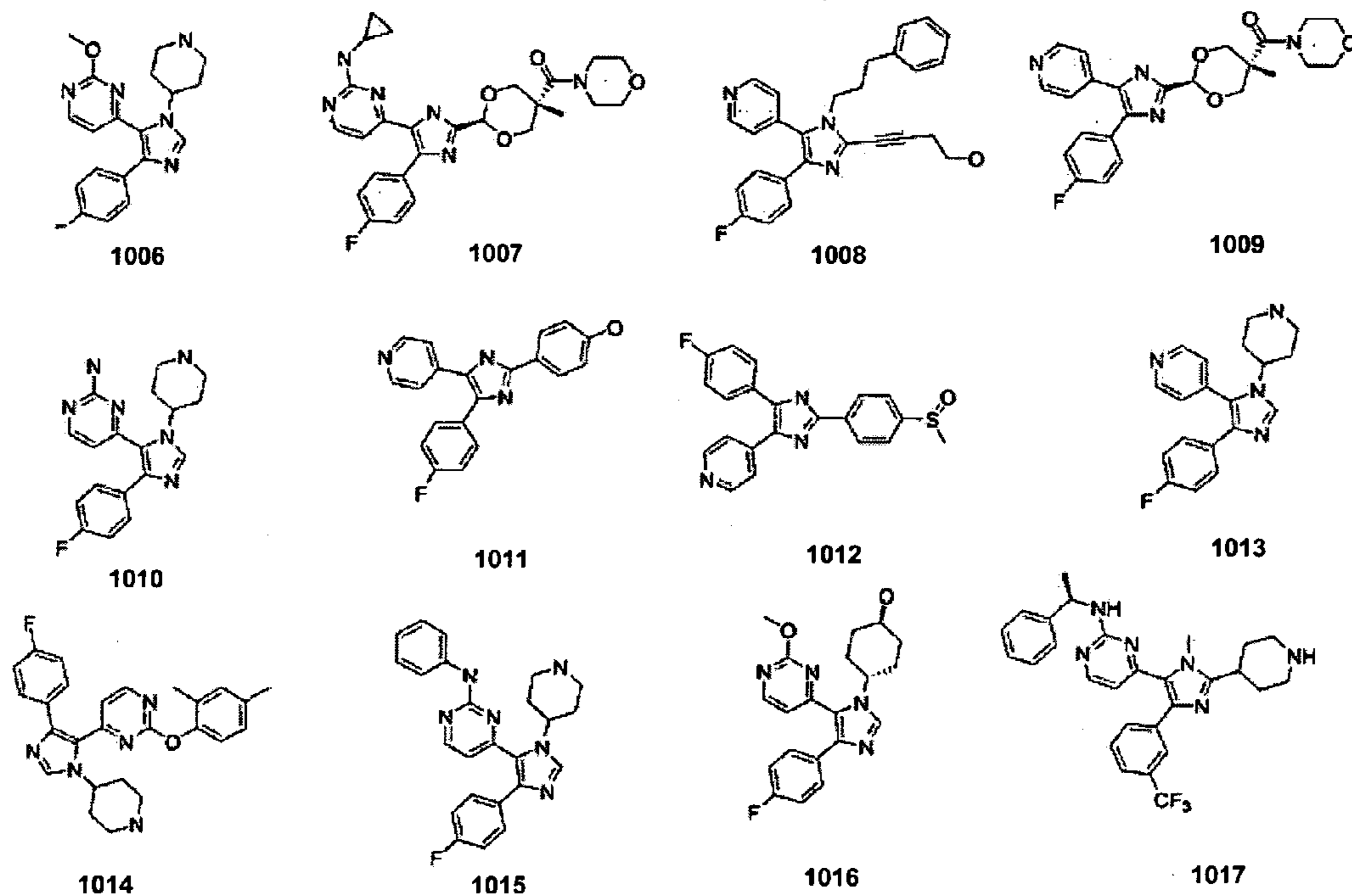
Figure 4c (imidazoles)
