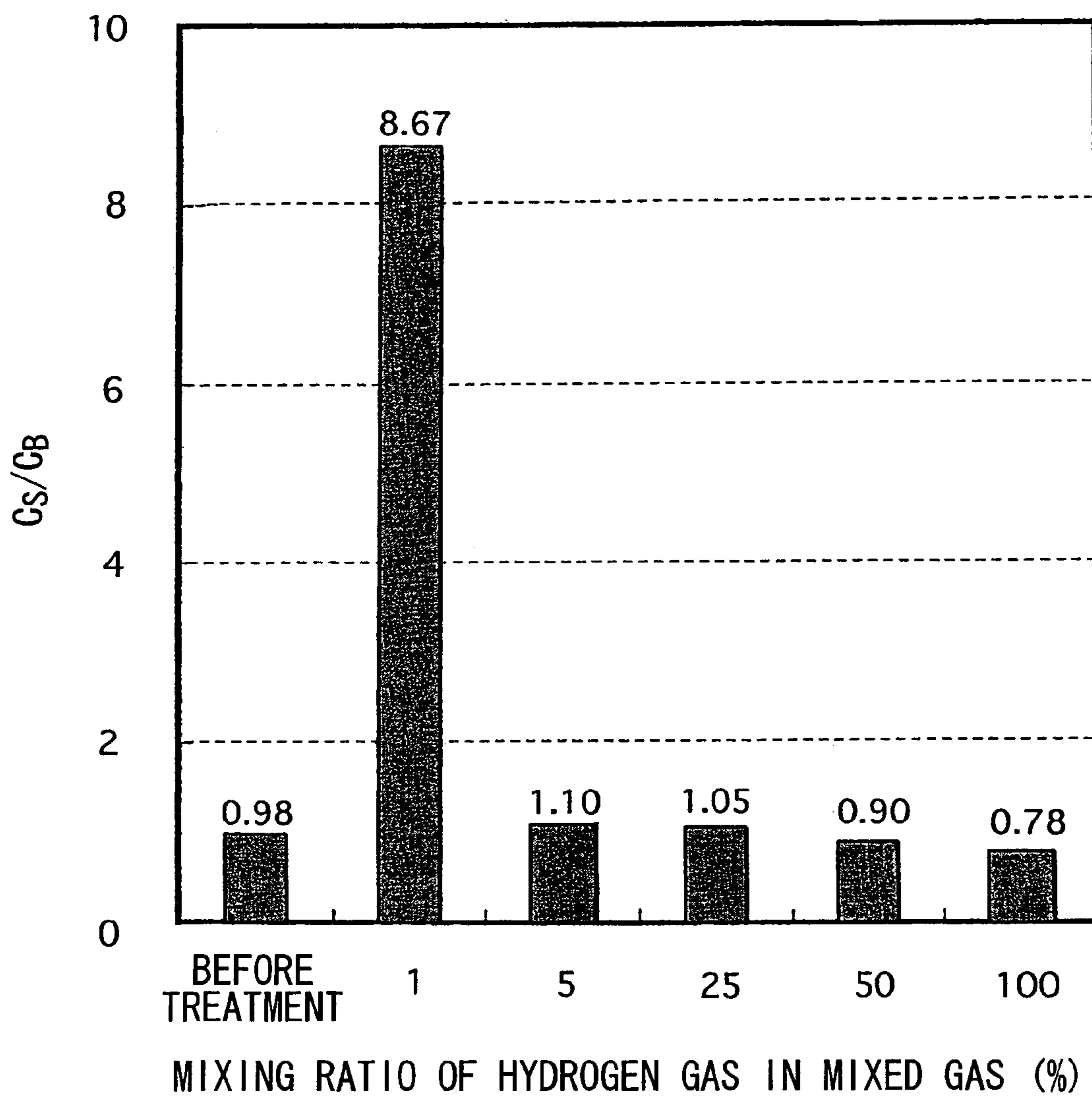
RELATION BETWEEN MIXING RATIO OF HYDROGEN GAS AND C_S/C_B
