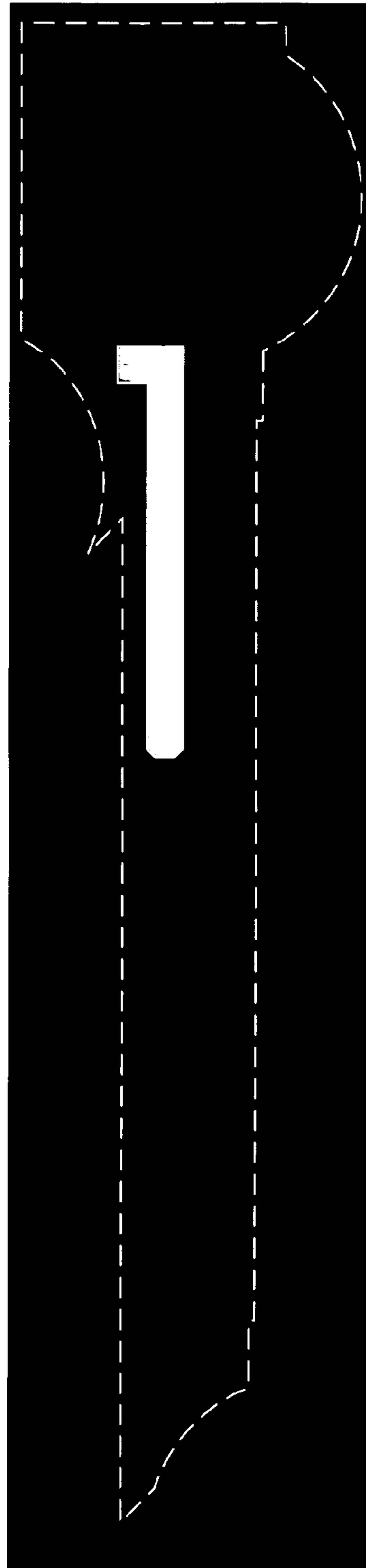
N-Well mask
