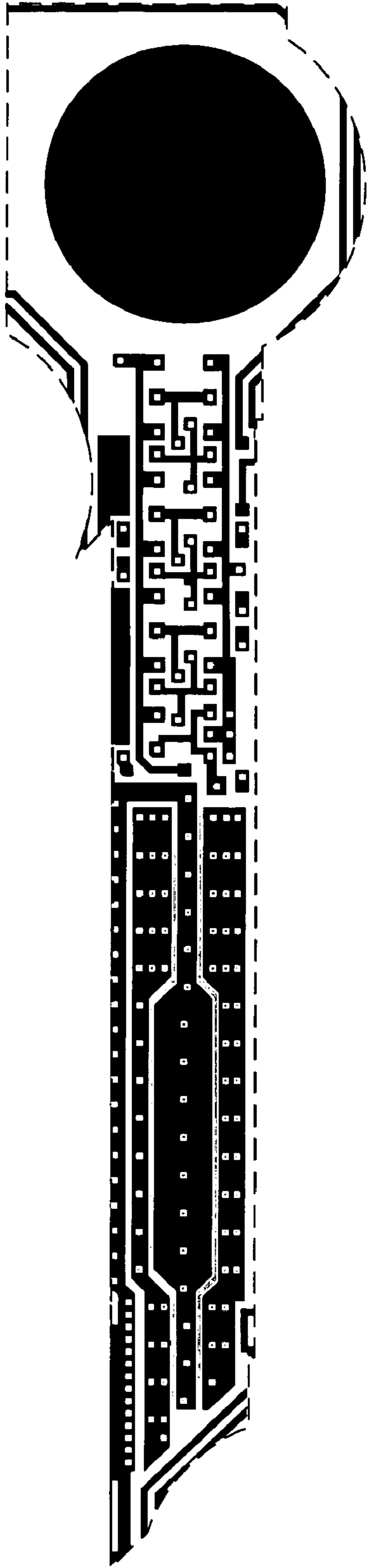
Metal 1 mask
