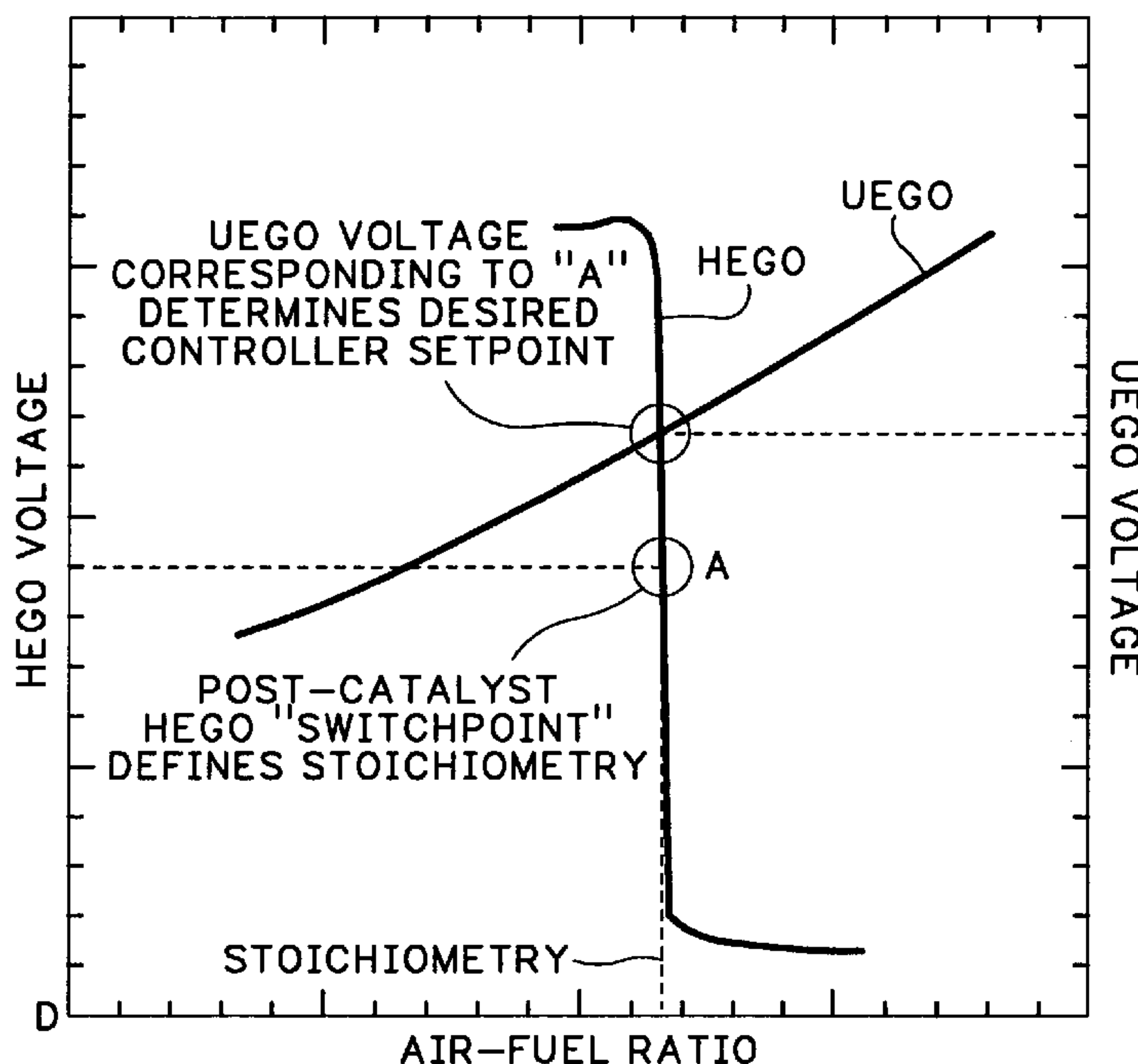
COMBINED UHEGO-HEGO SENSOR OUTPUT VOLTAGES
