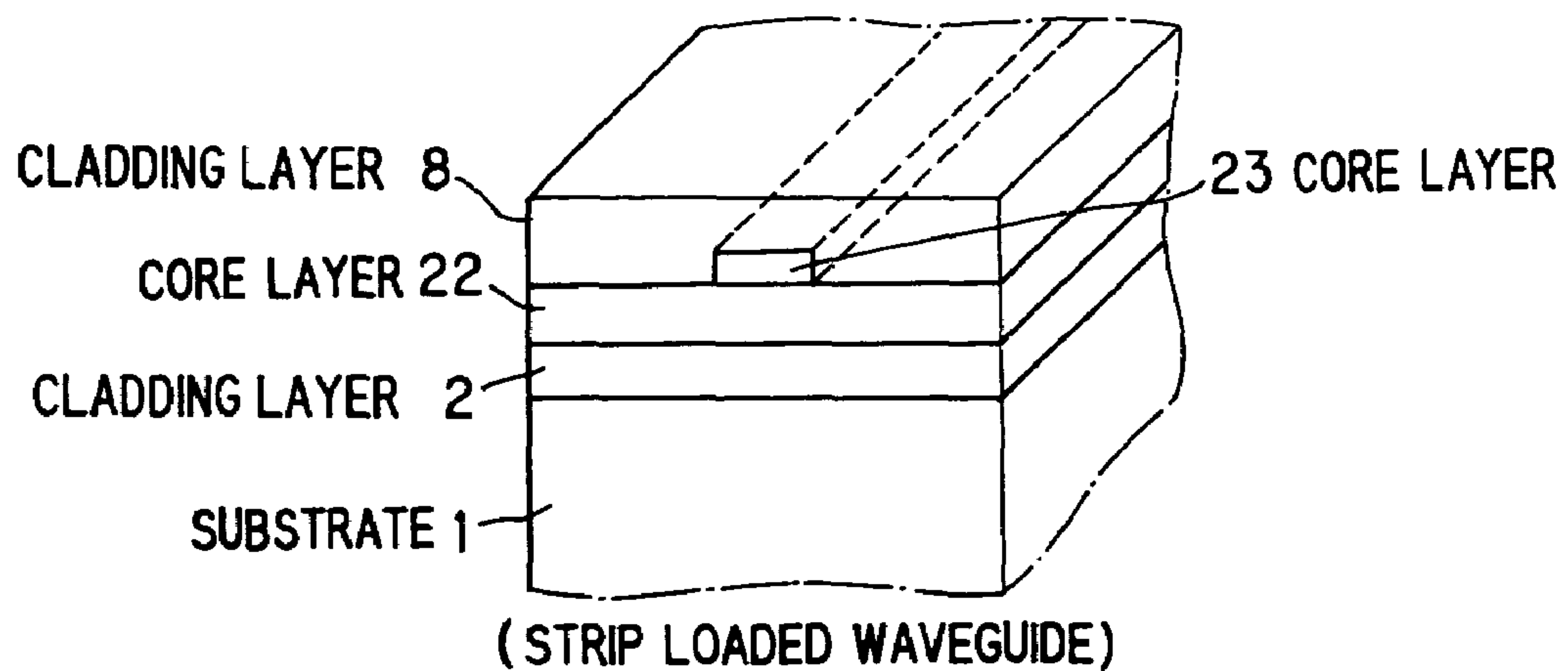
FIG. 4 (PRIOR ART)
