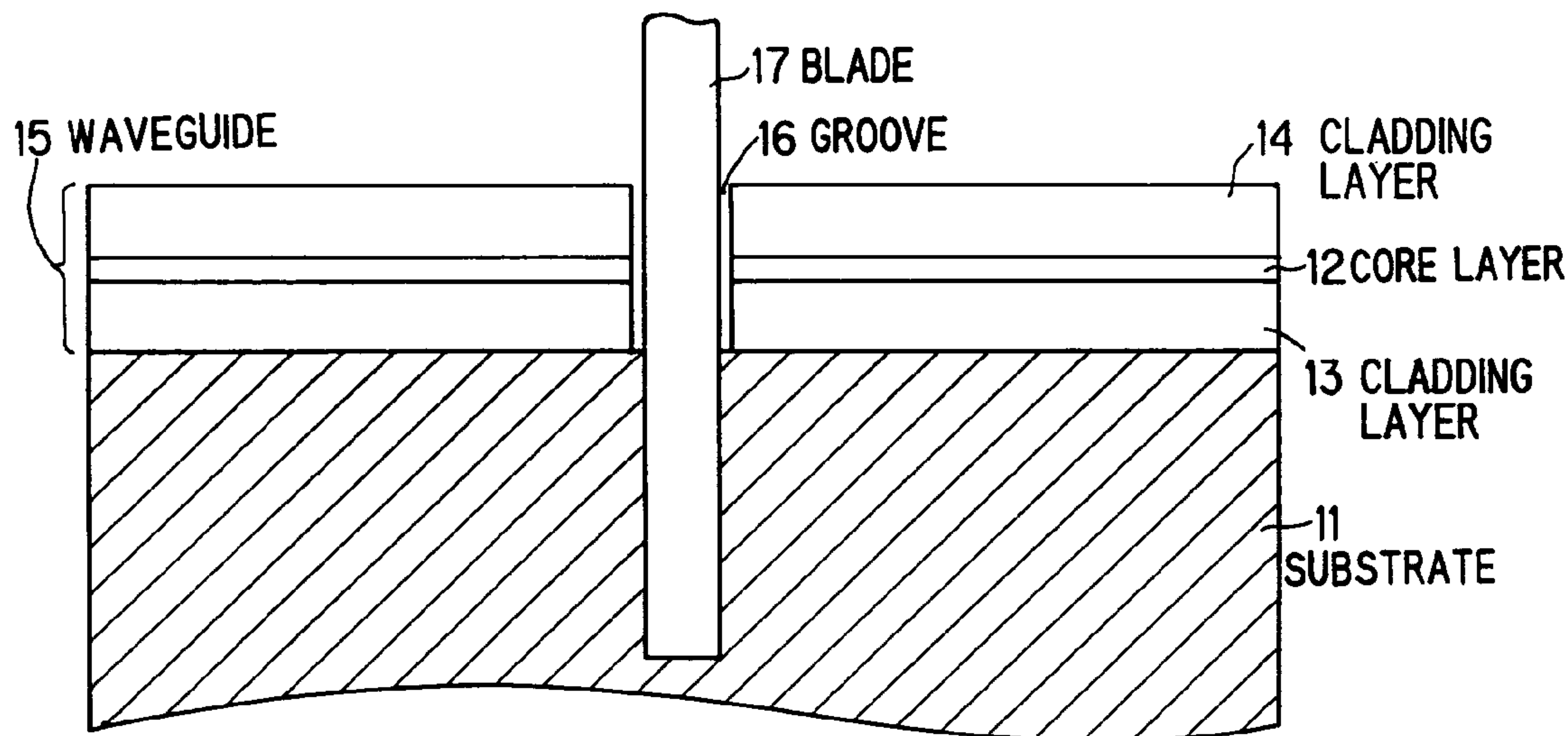
FIG. 6 (PRIOR ART)
