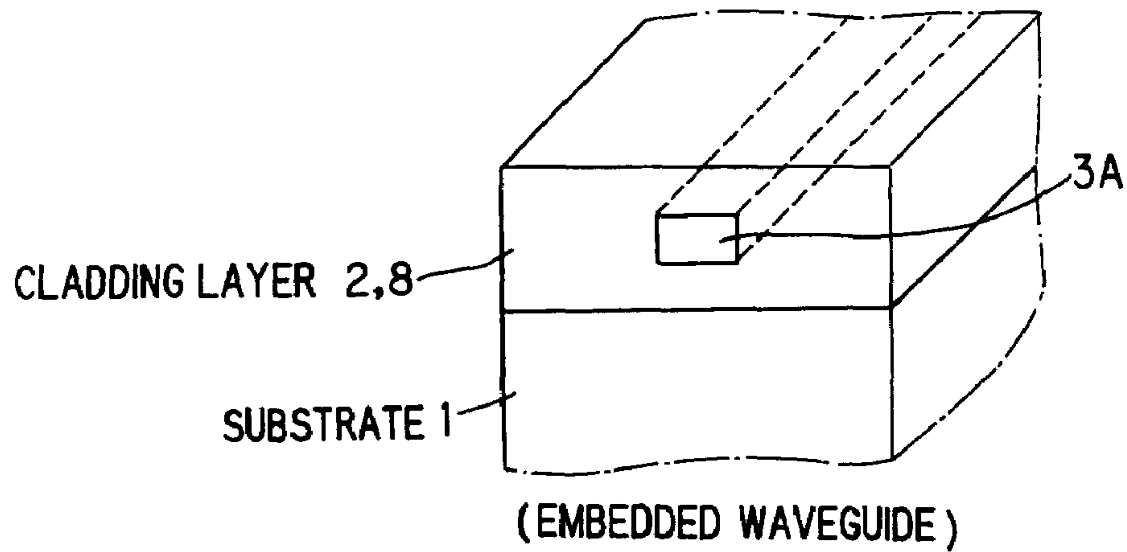
FIG. 3 (PRIOR ART)
