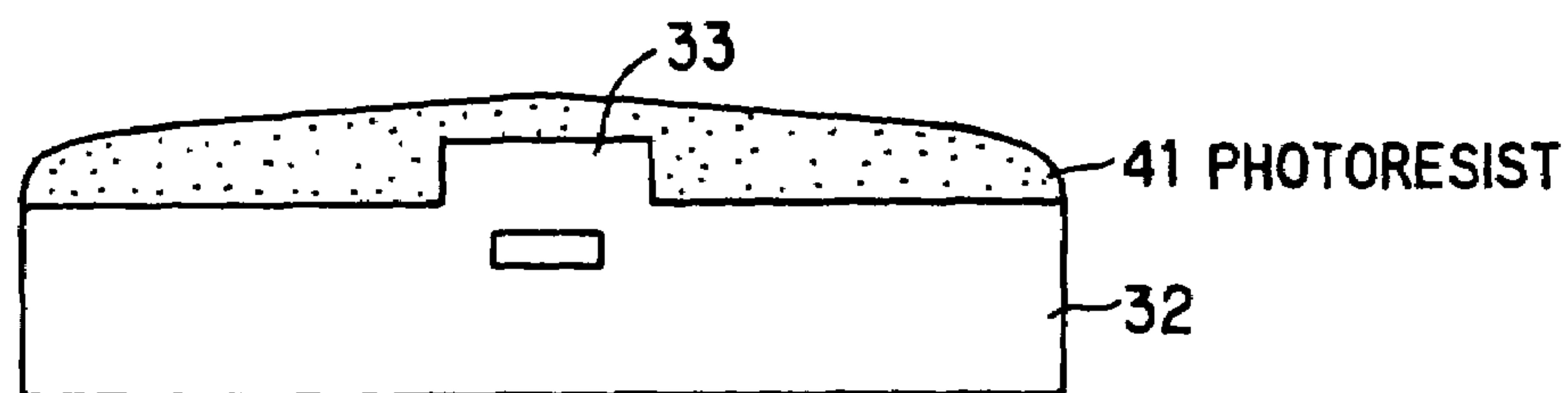
FIG. 9C (PRIOR ART)
