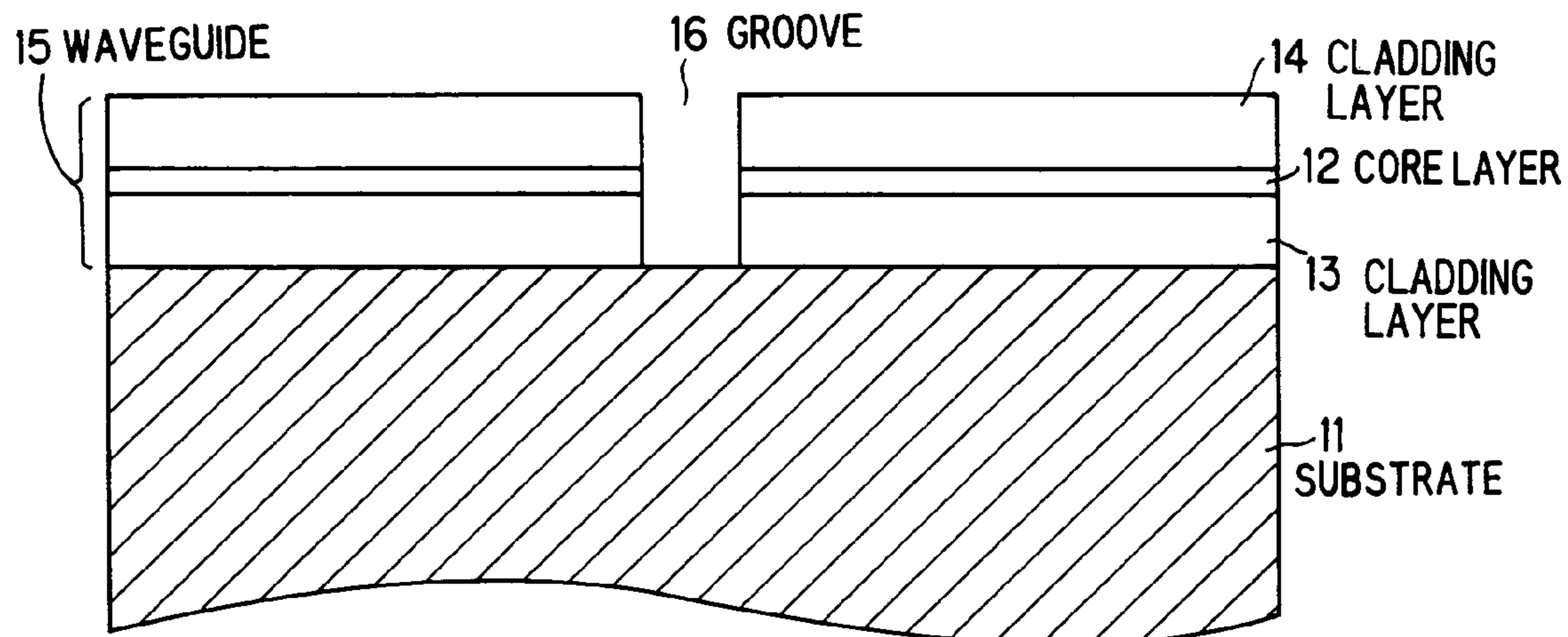
FIG. 6 (PRIOR ART)
