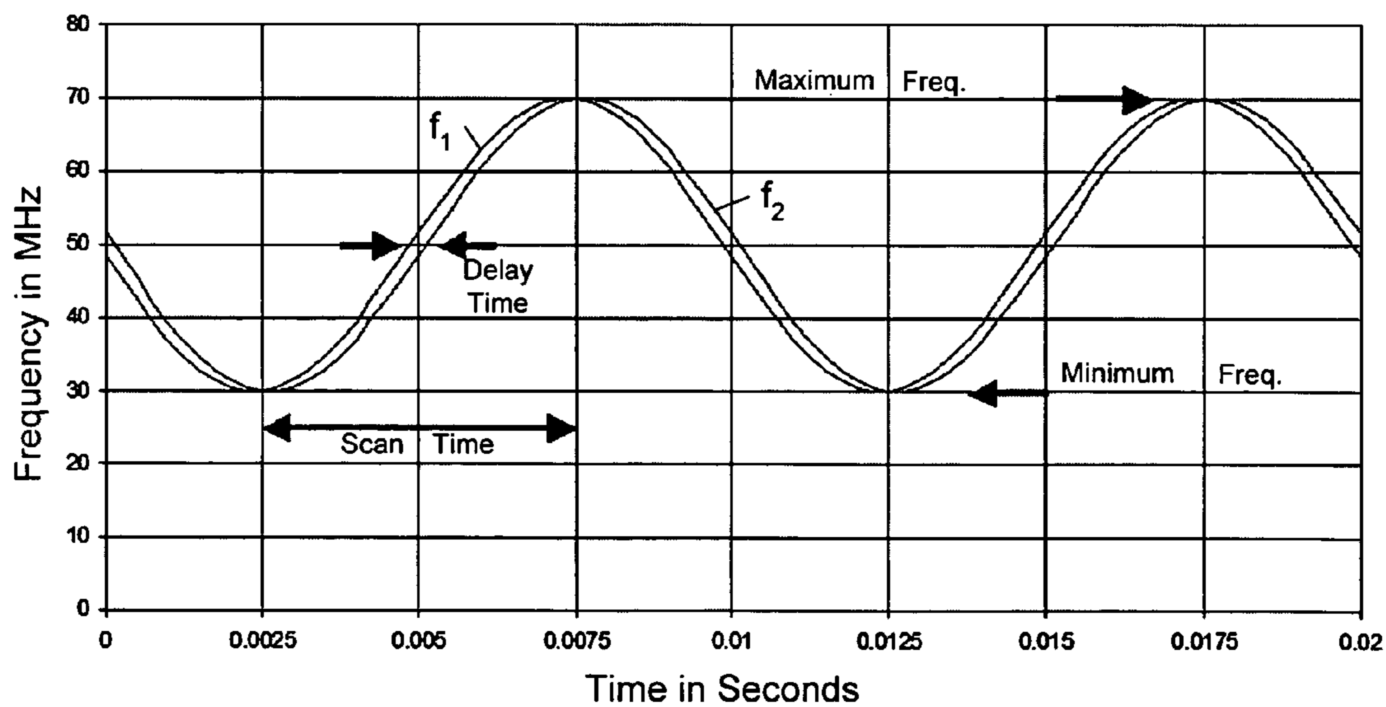
Frequencies of Drive Waveforms vs. Time: Sinusoidal Ramp
