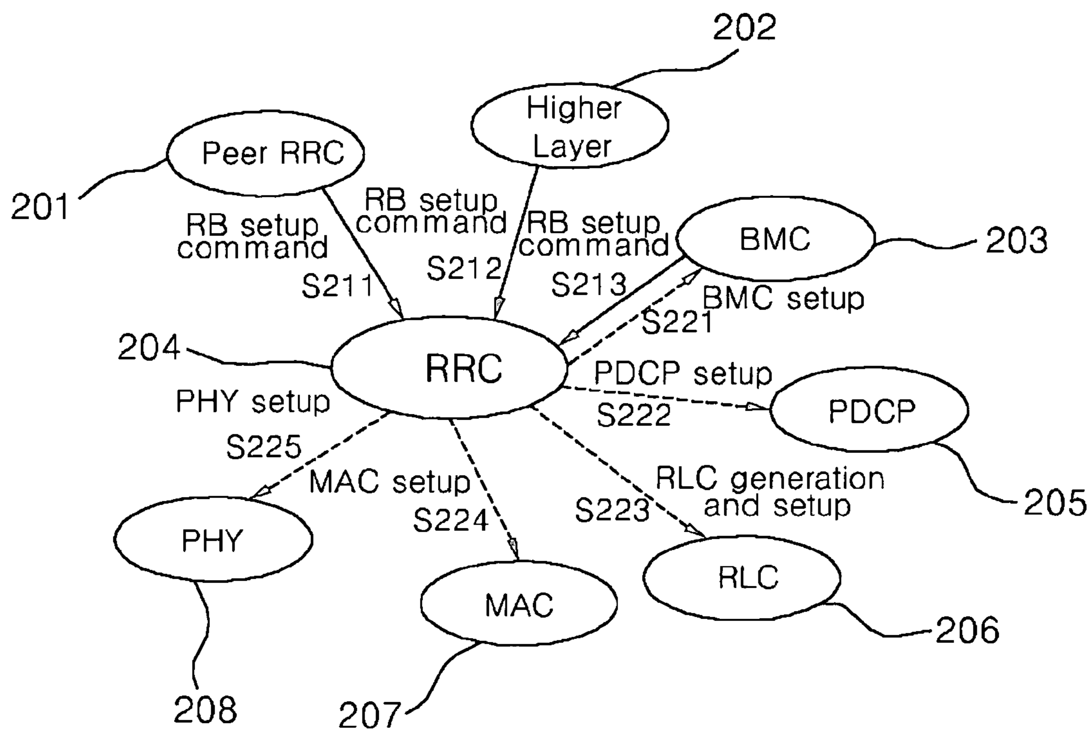
Fig. 2(Related Art)
