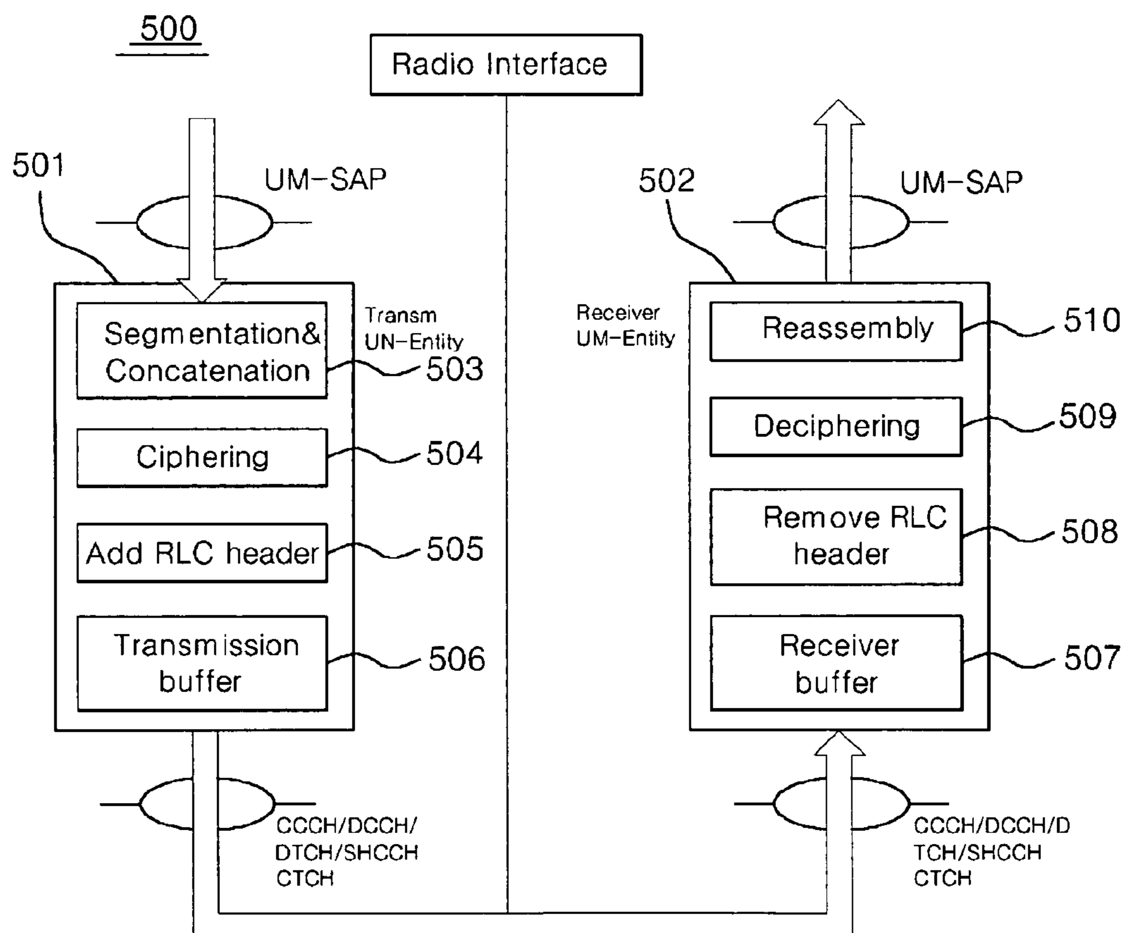
Fig. 5(Related Art)
