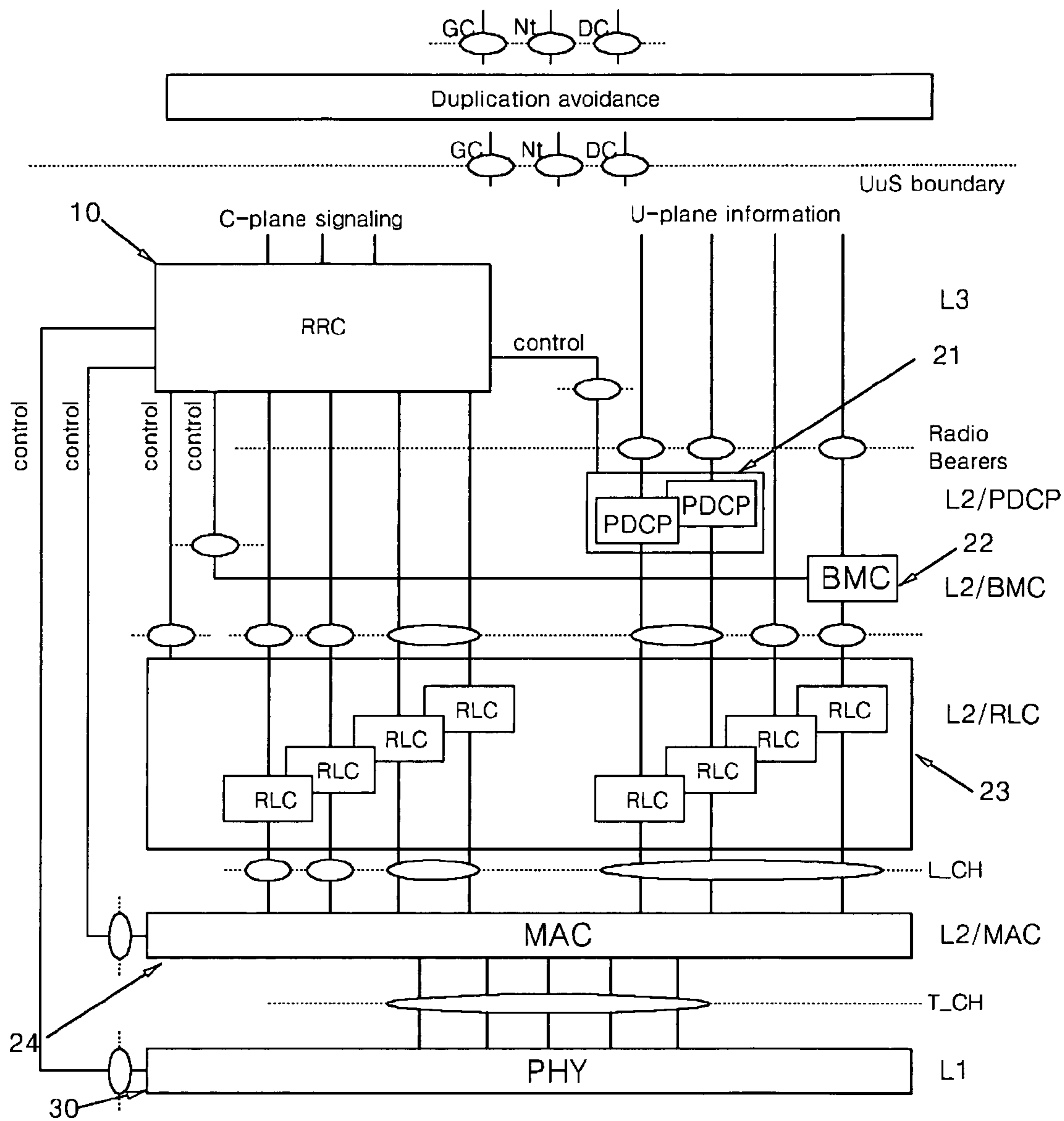
Fig. 1(Related Art)
