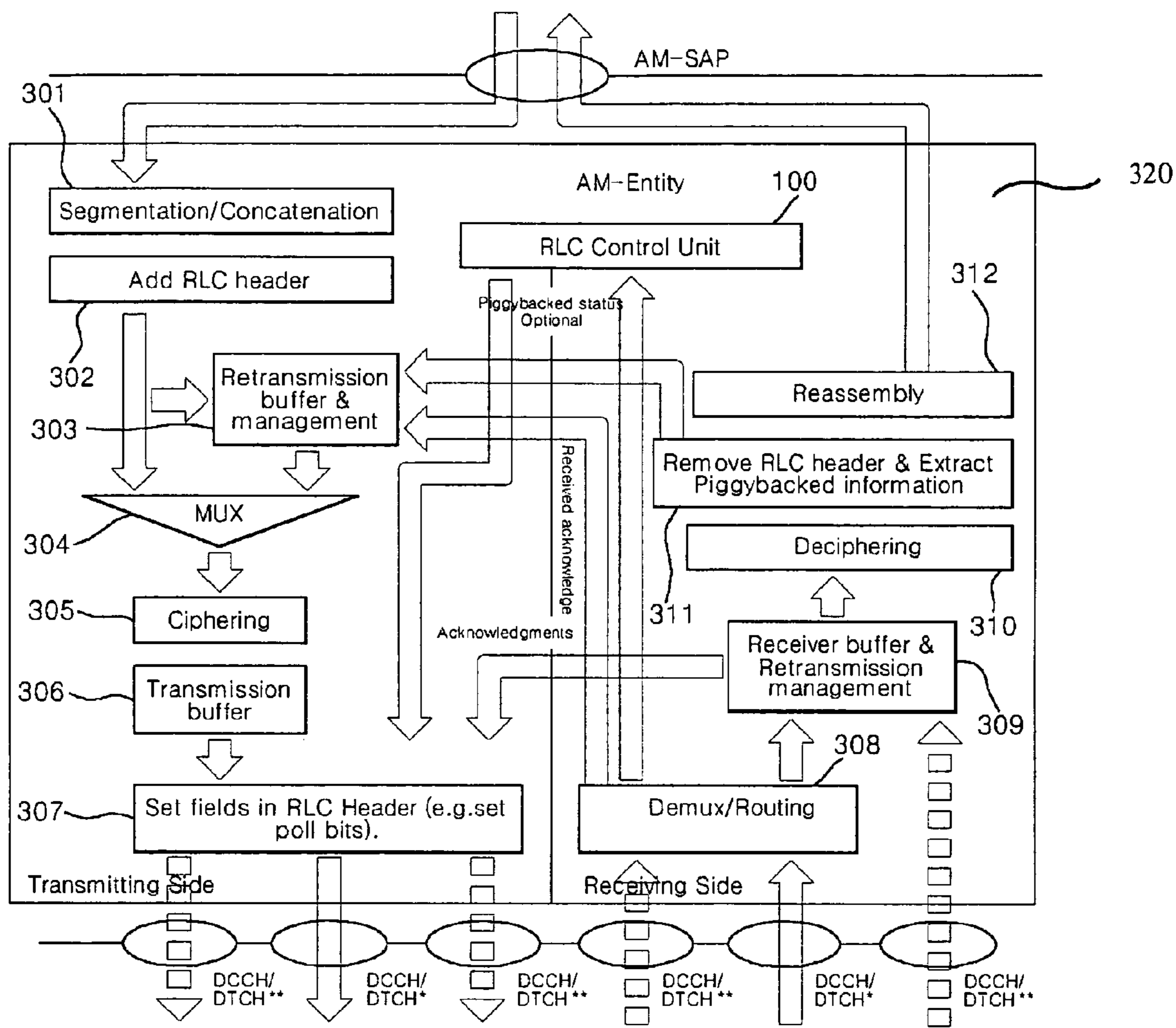
Fig. 3(Related Art)
