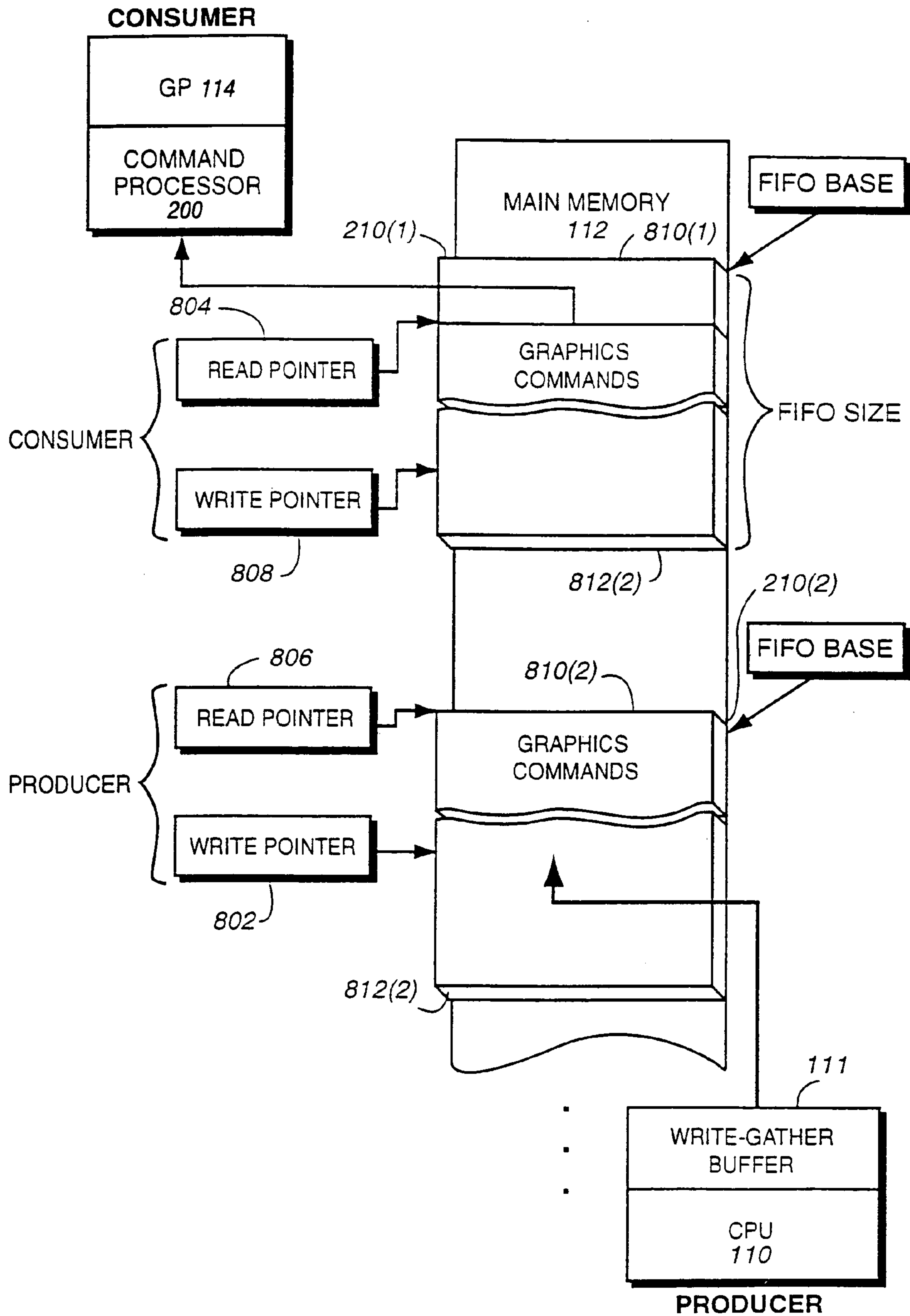
Fig. 6 EXAMPLE MULTI - BUFFERING
