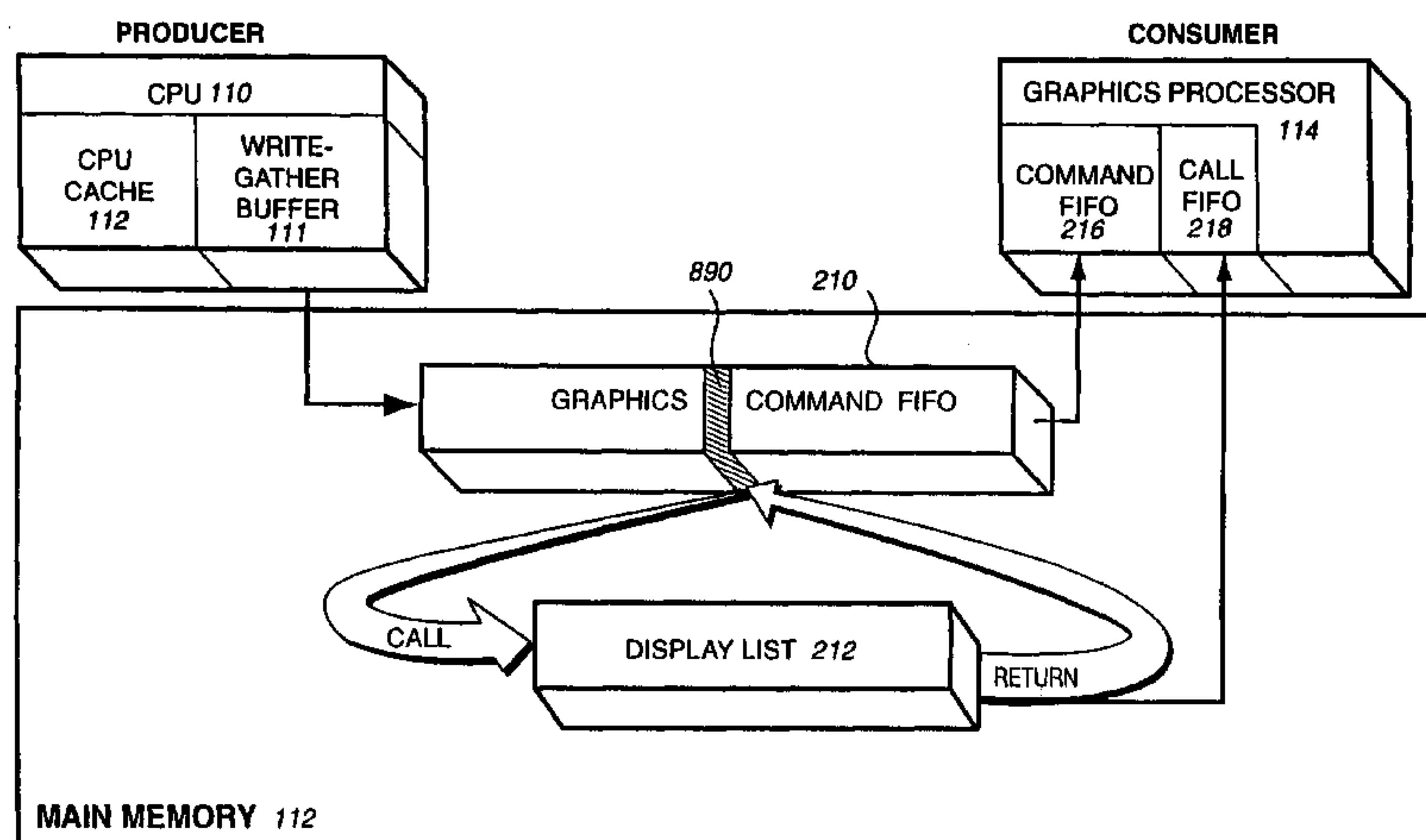
EXAMPLE DISPLAY LIST CALL FROM COMMAND FIFO
