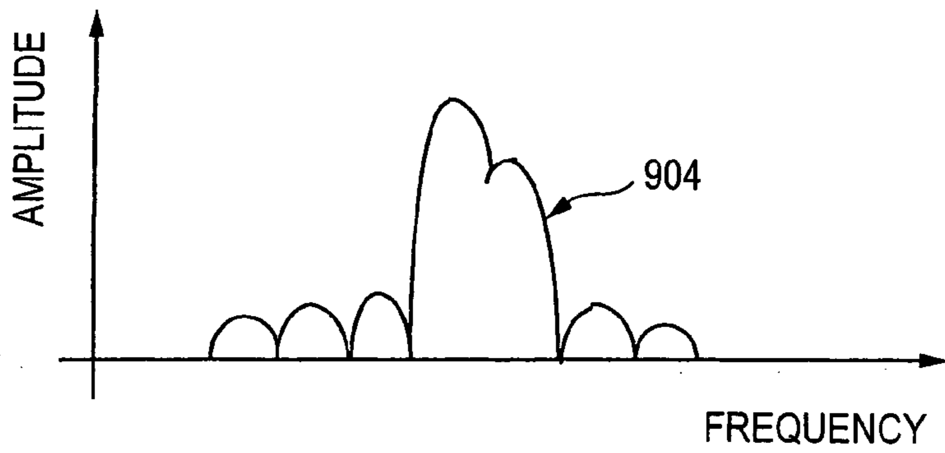
FIG. 18(b) BACKGROUND ART
