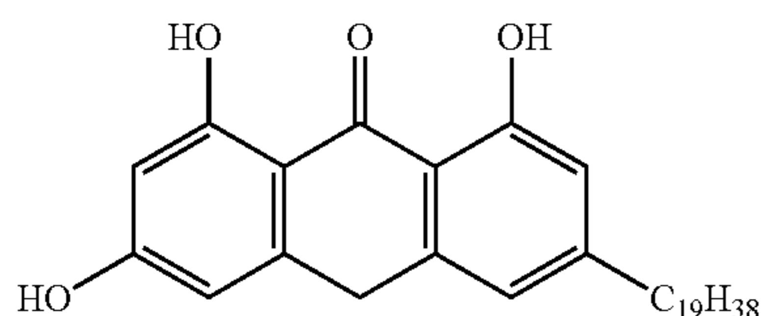
Emodin
