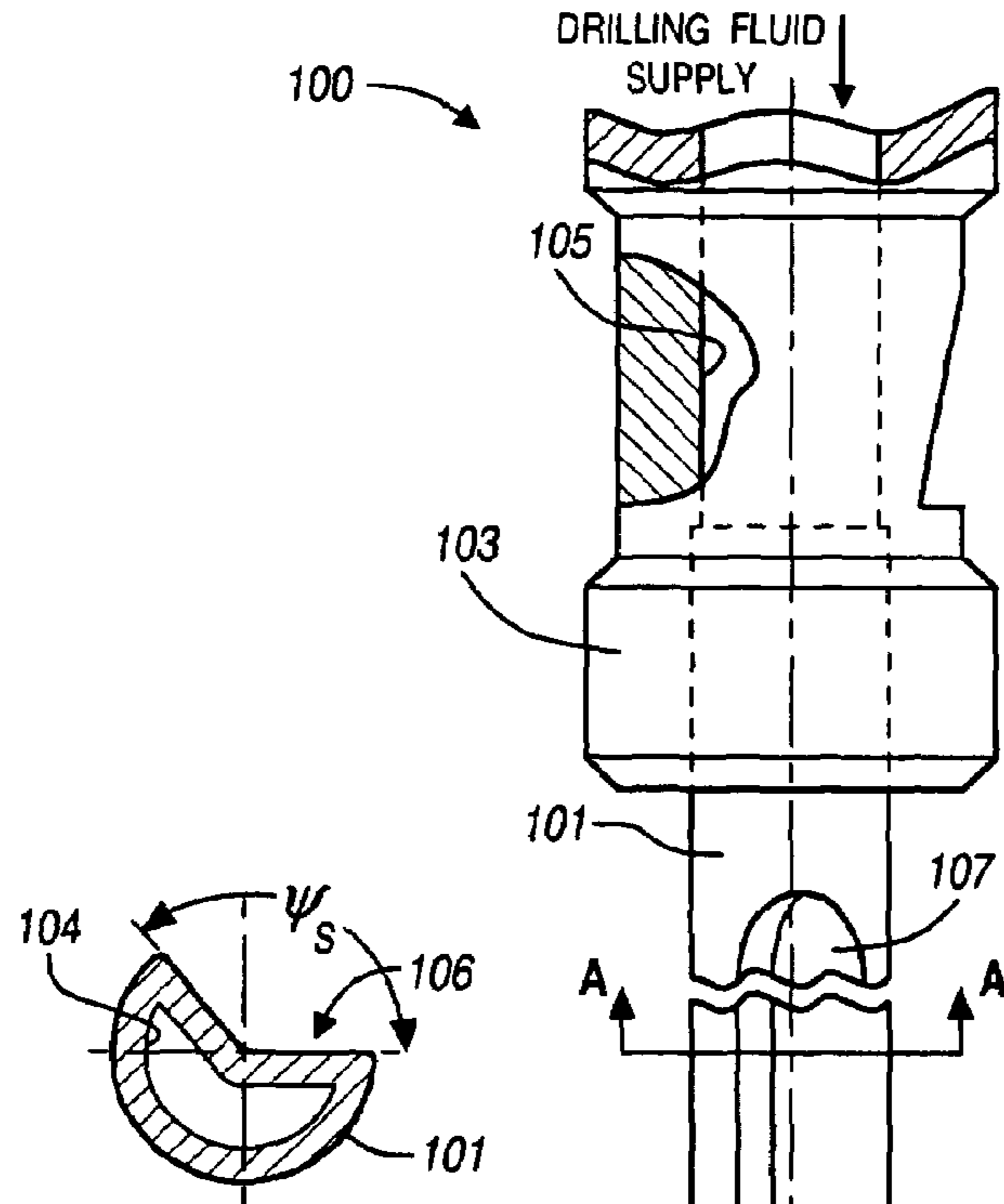
FIGURE 2 SECTION A-A PRIOR ART
