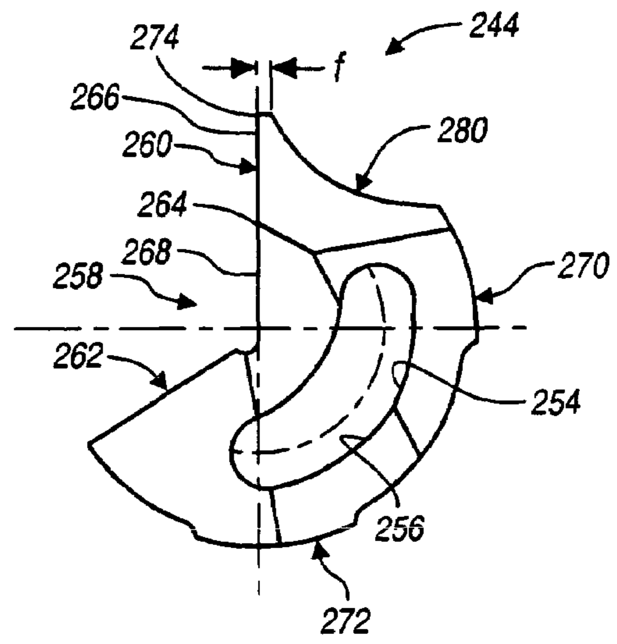
FIGURE 31 VIEW V2
