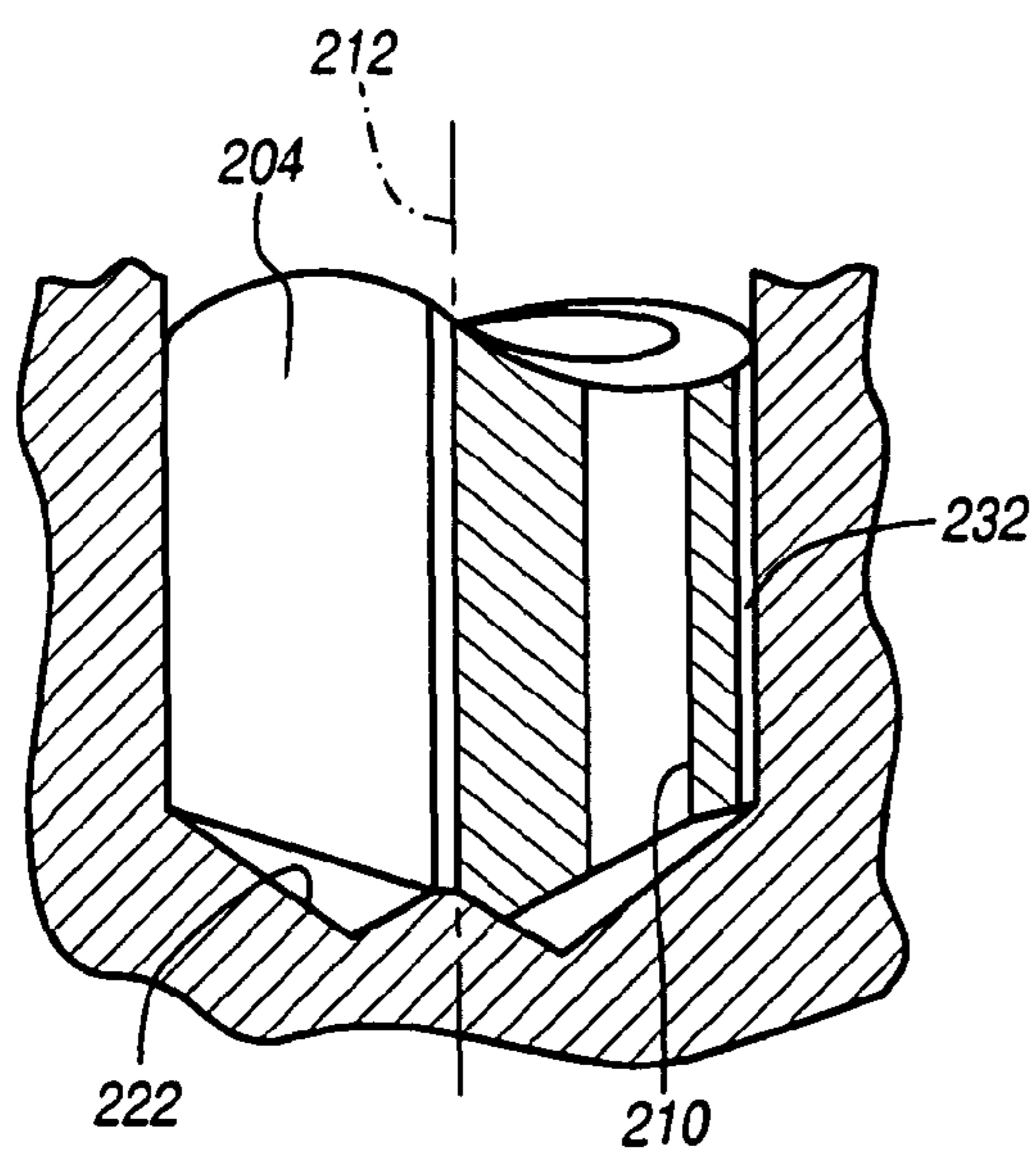
FIGURE 28 SECTION U-U
