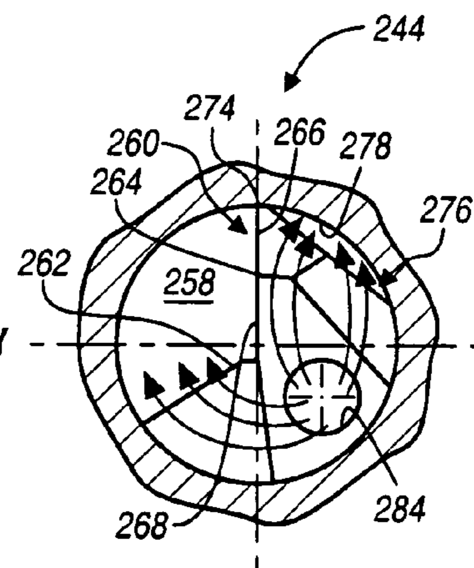
FIGURE 35 VIEW Y
