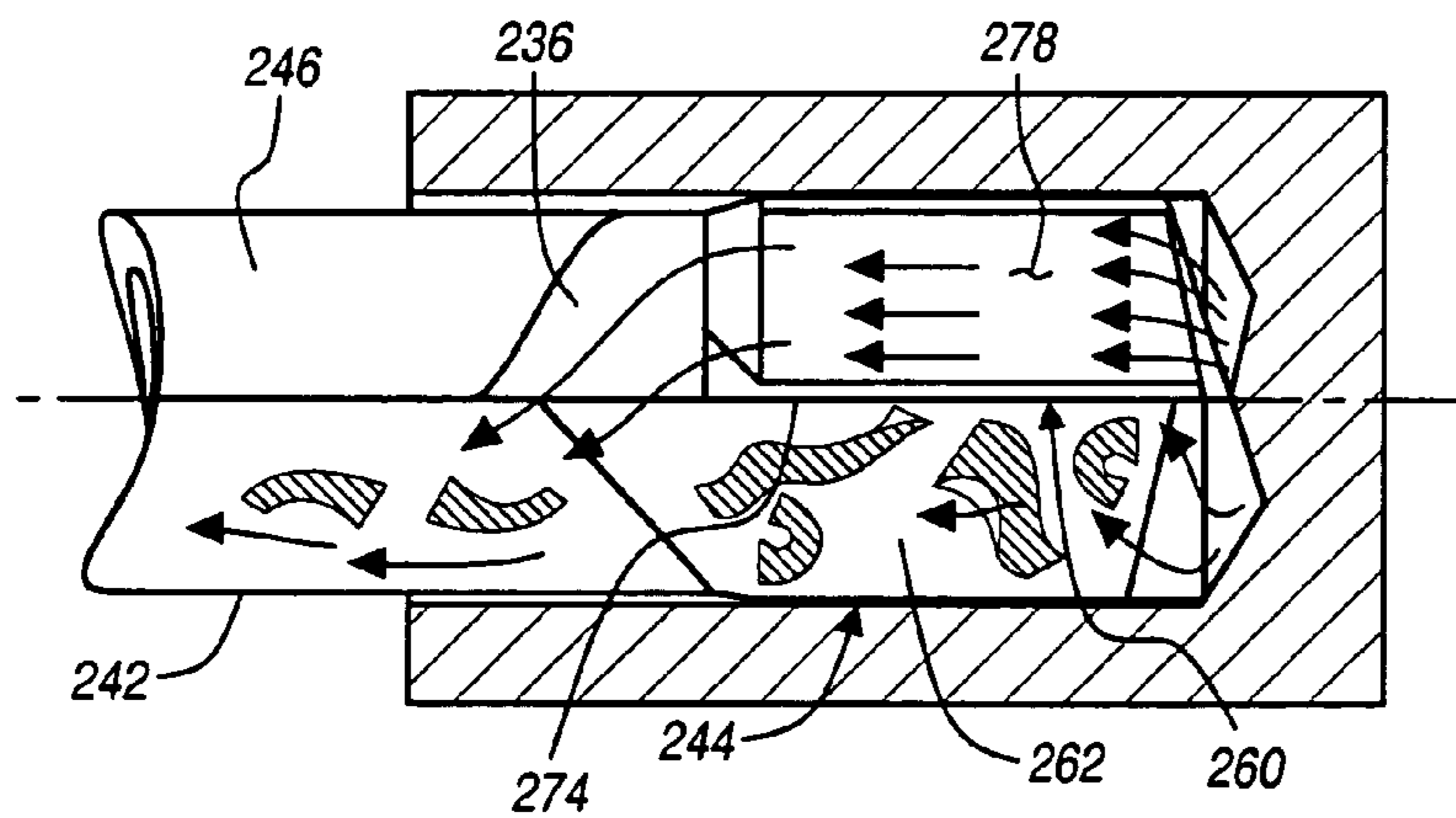
FIGURE 36 VIEW Z
