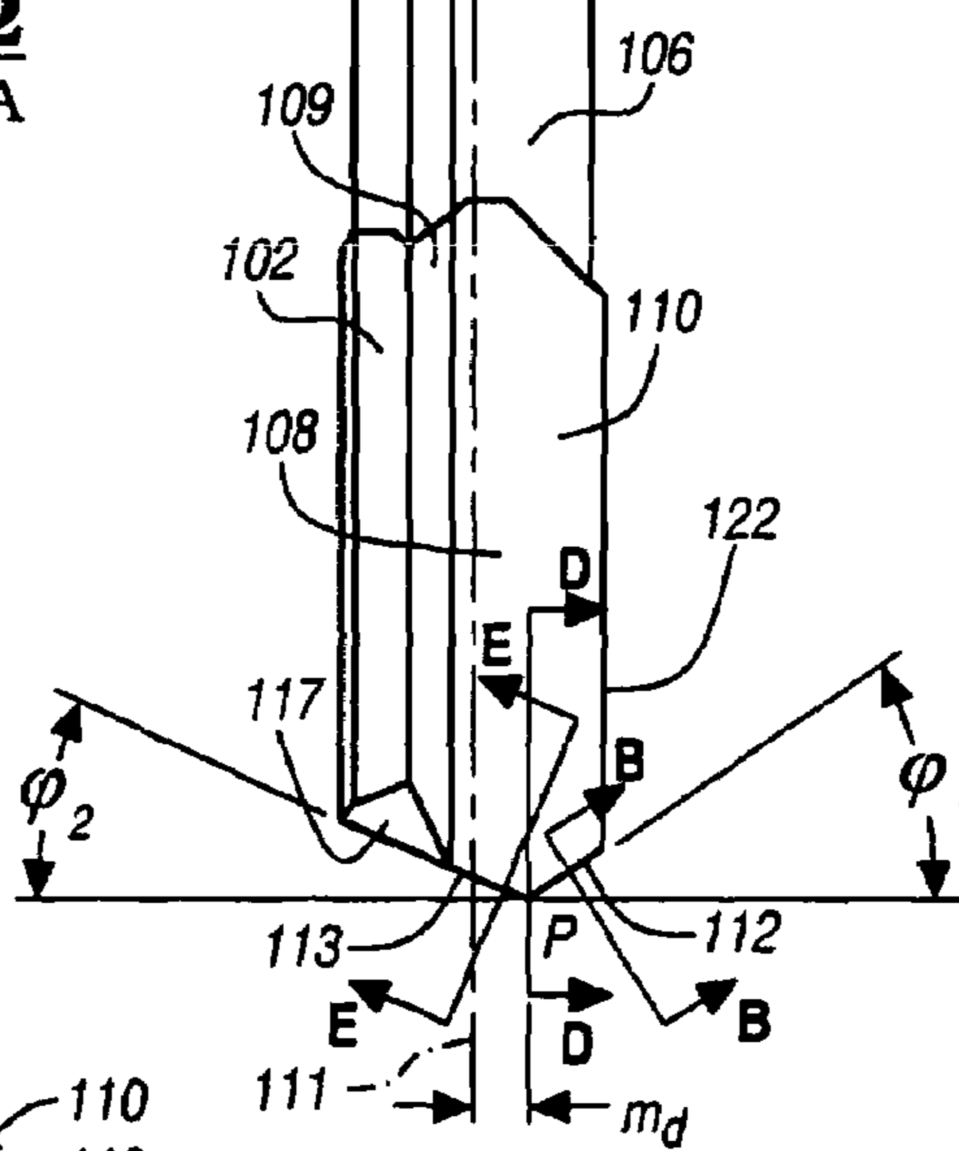
FIGURE 5 SECTION D-D PRIOR ART
