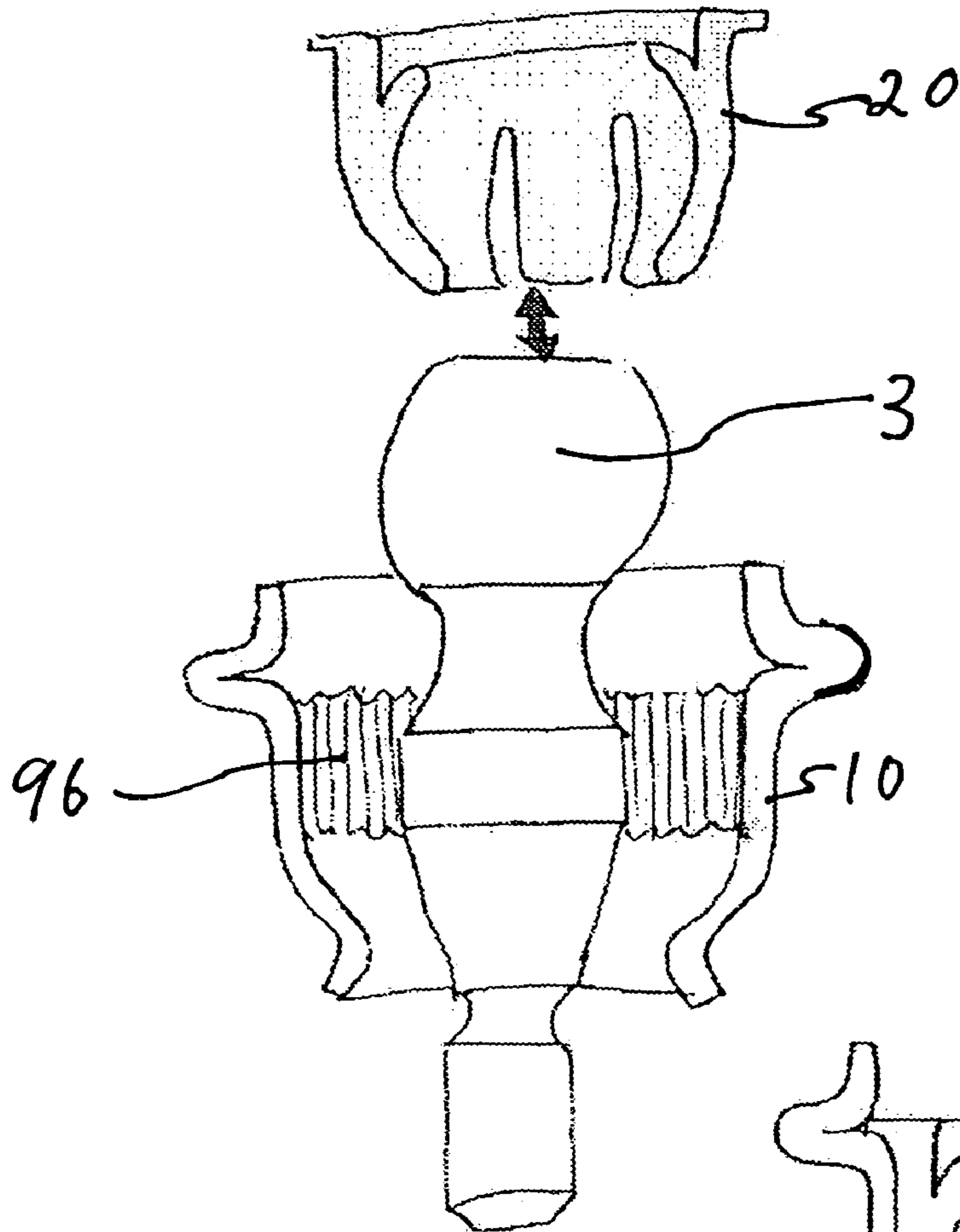
FIG 21 A
