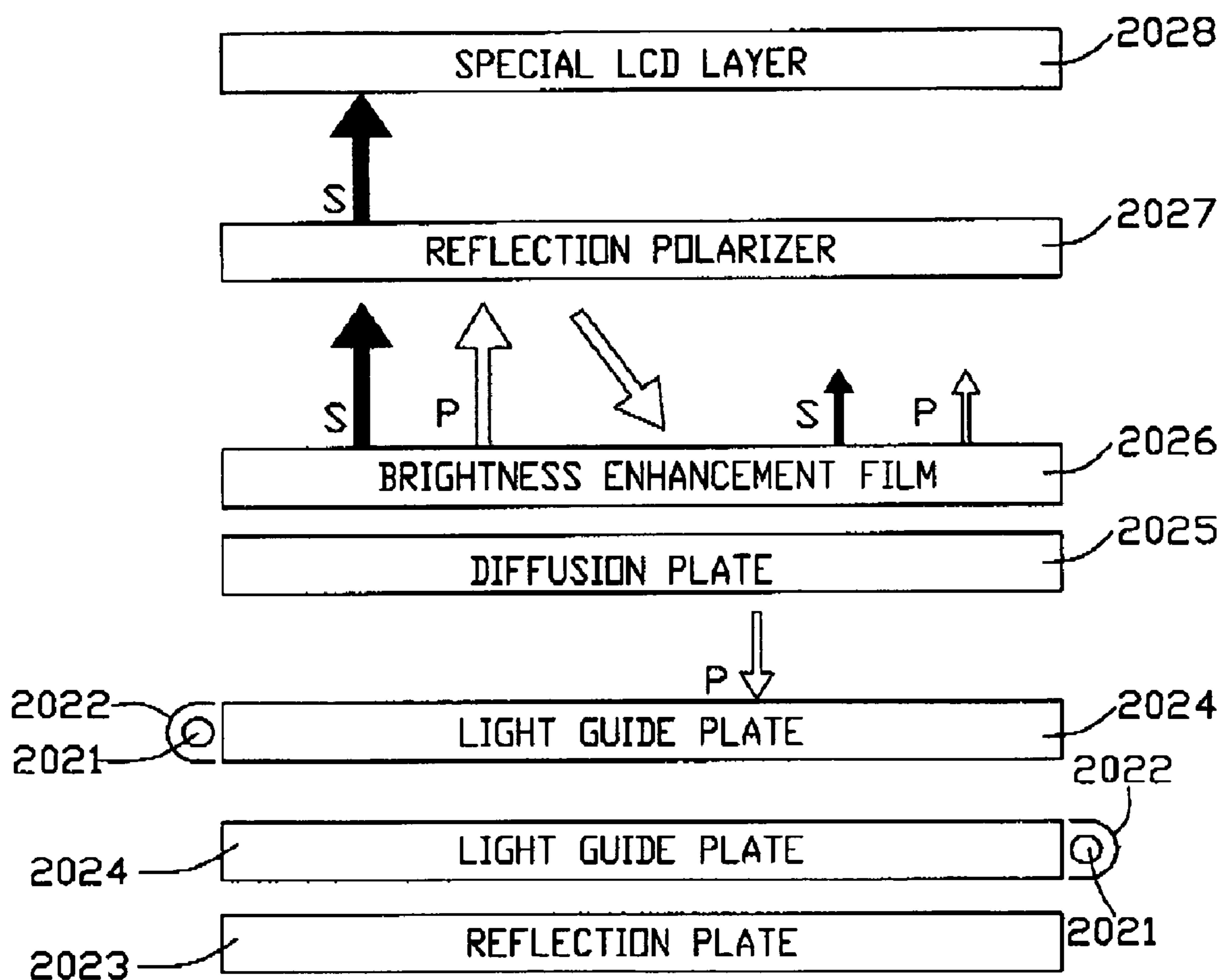
FIG. 8 (PRIOR ART)
