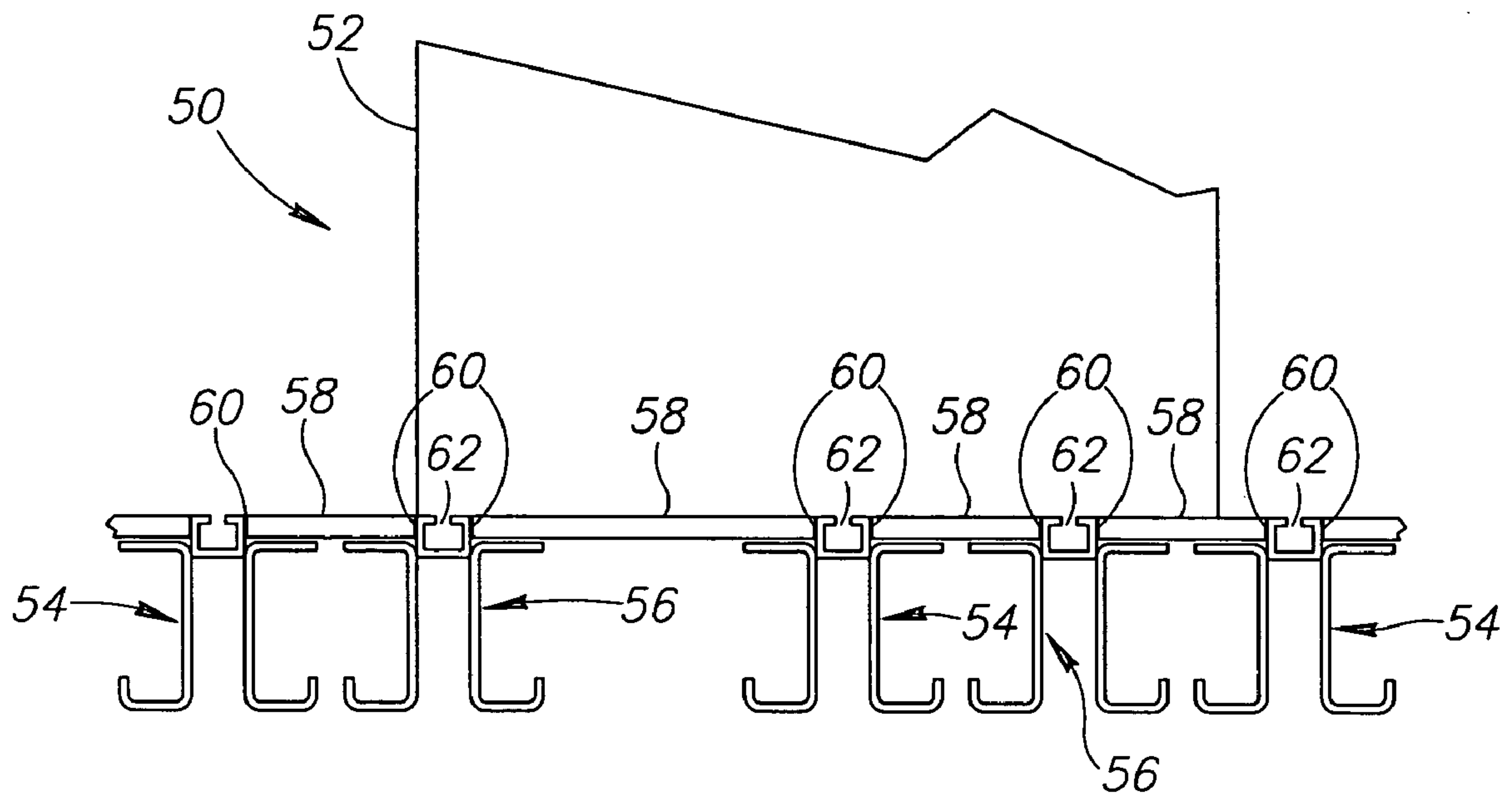
FIG. 1 (PRIOR ART)
