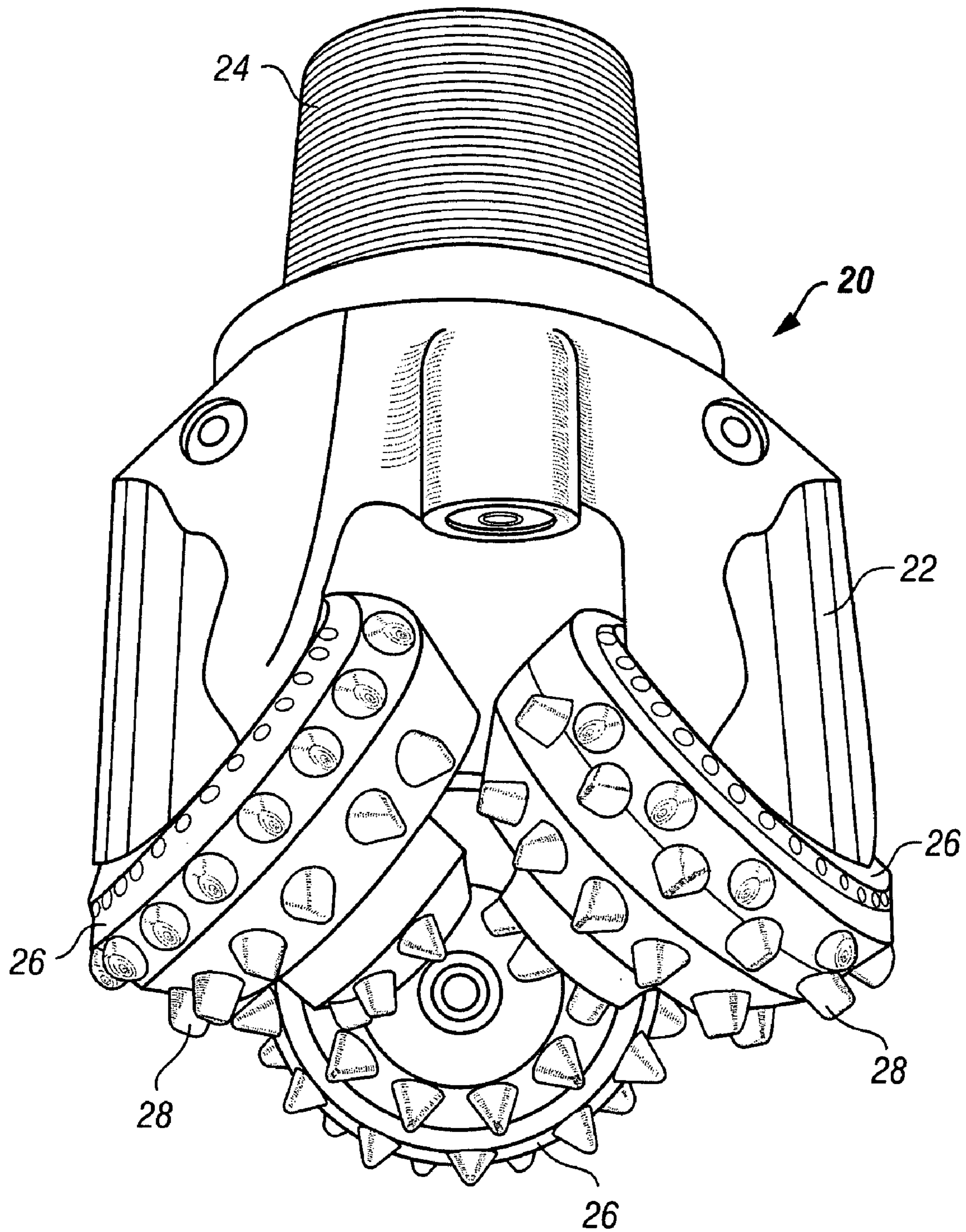
FIG. 2 (Prior Art)
