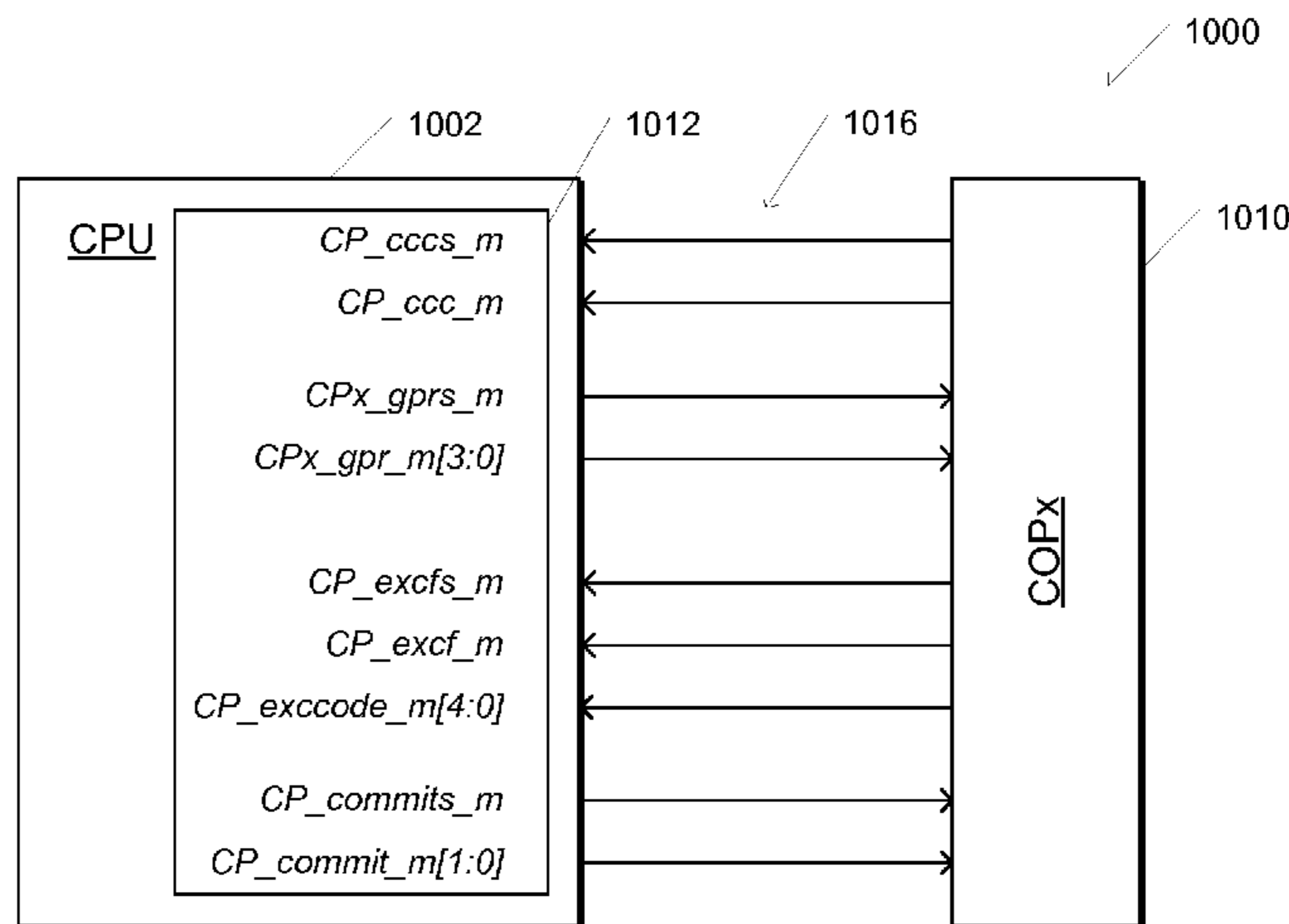
COProcessor Condition Code Check / GPR / exception Found / Instruction Commit
