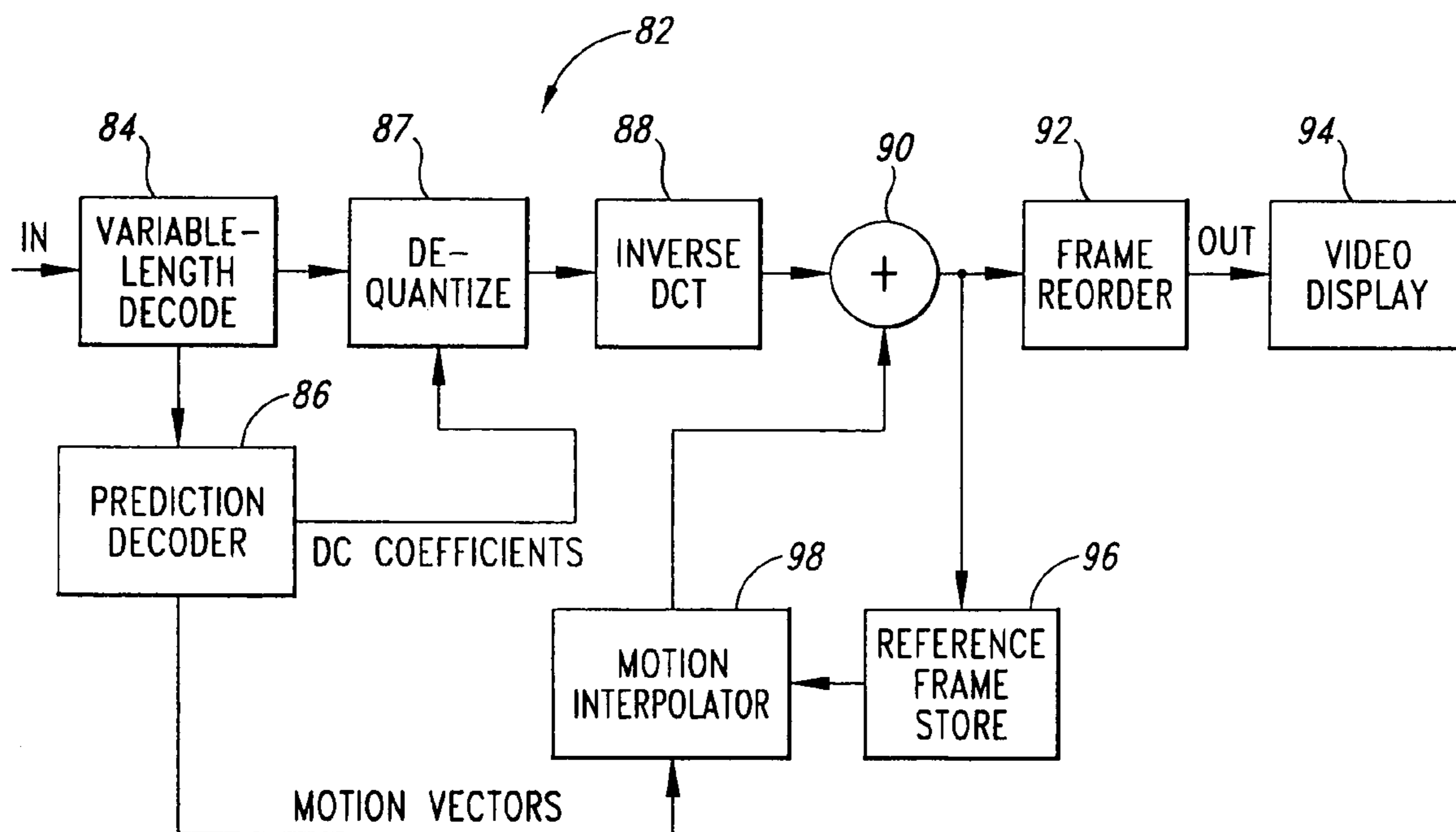
Fig. 6 (Prior Art)
