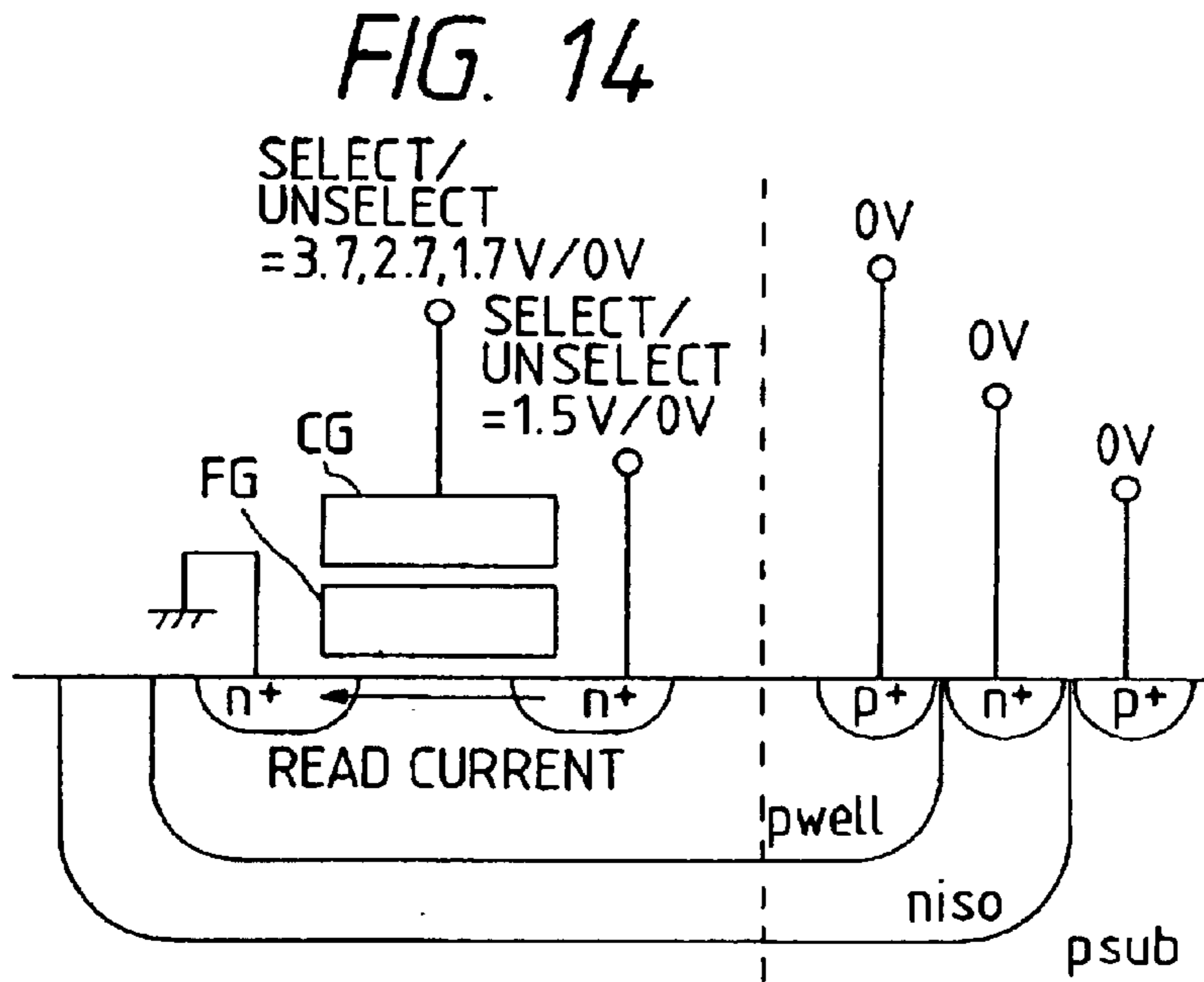
EXAMPLE OF APPLIED VOLTAGES AT READING TIME
