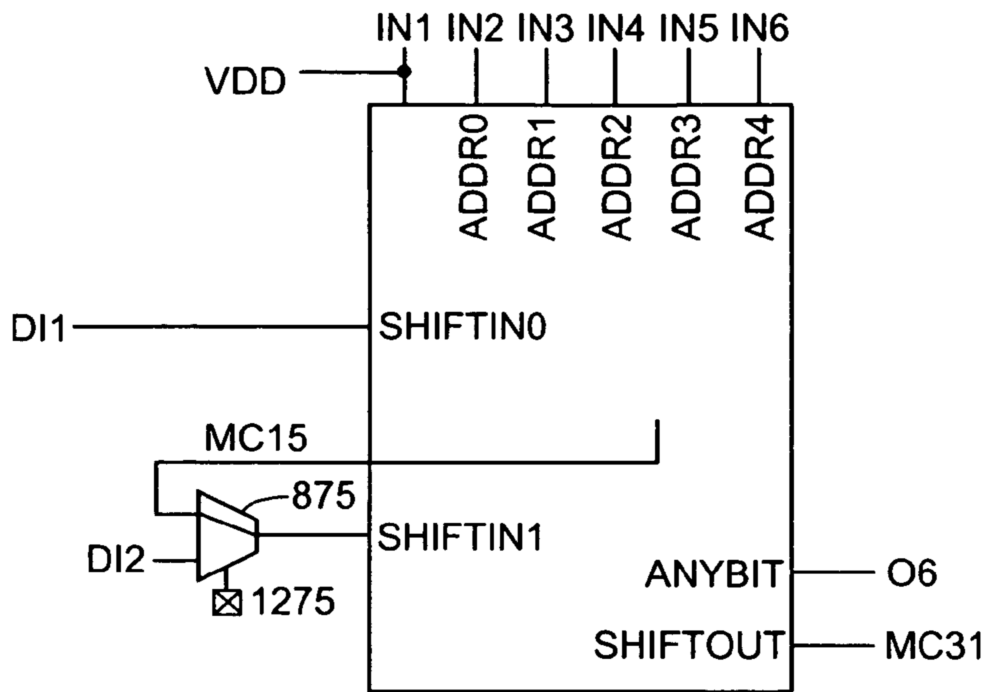
FIG. 12 (32x1 SRL)
