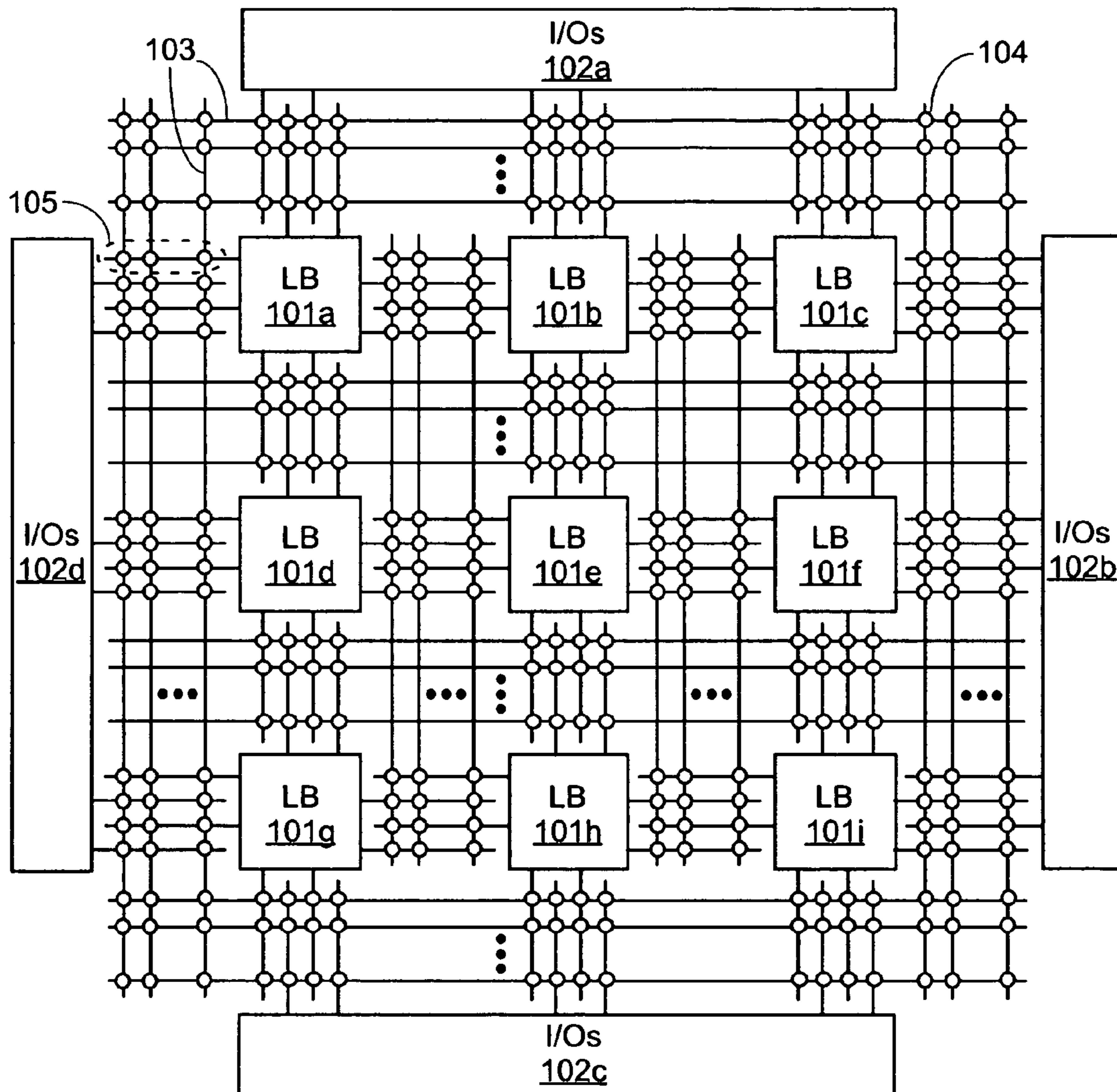
FIG. 1 (Prior Art)
