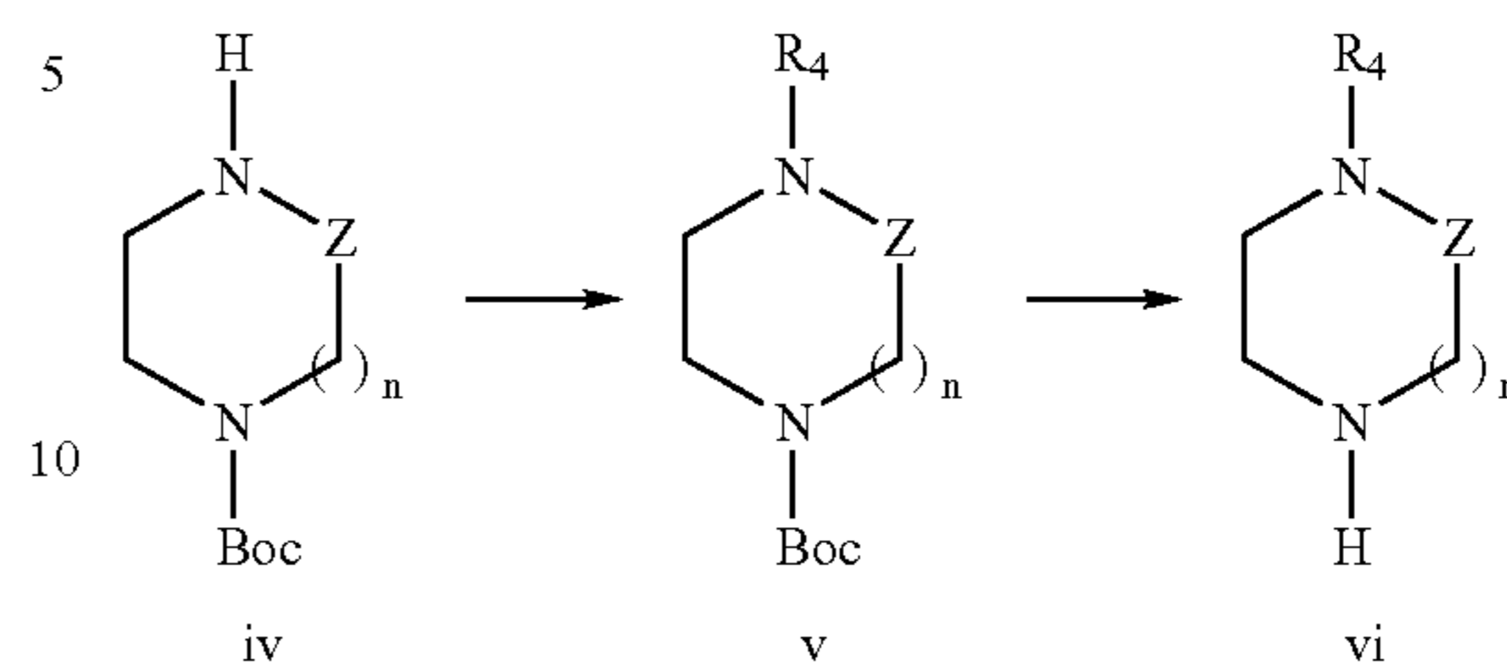
Reaction Scheme 2
