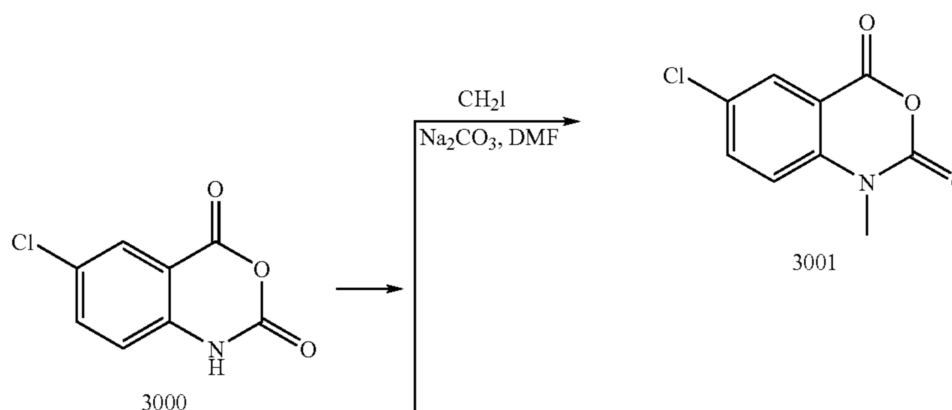
Reaction Scheme 26
