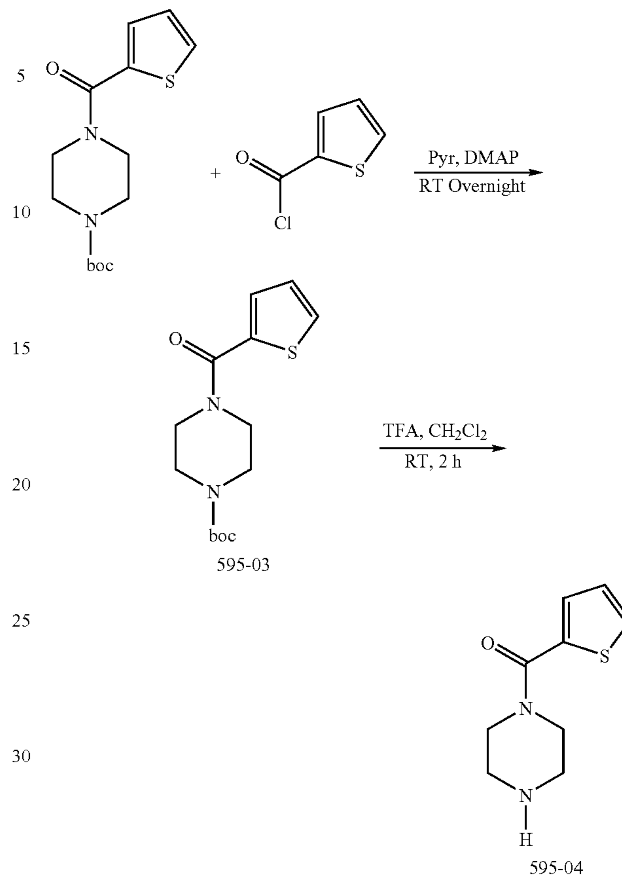
Piperazine-1-yl-thiophen-2-yl-methanone (Referred to as 595-04)
