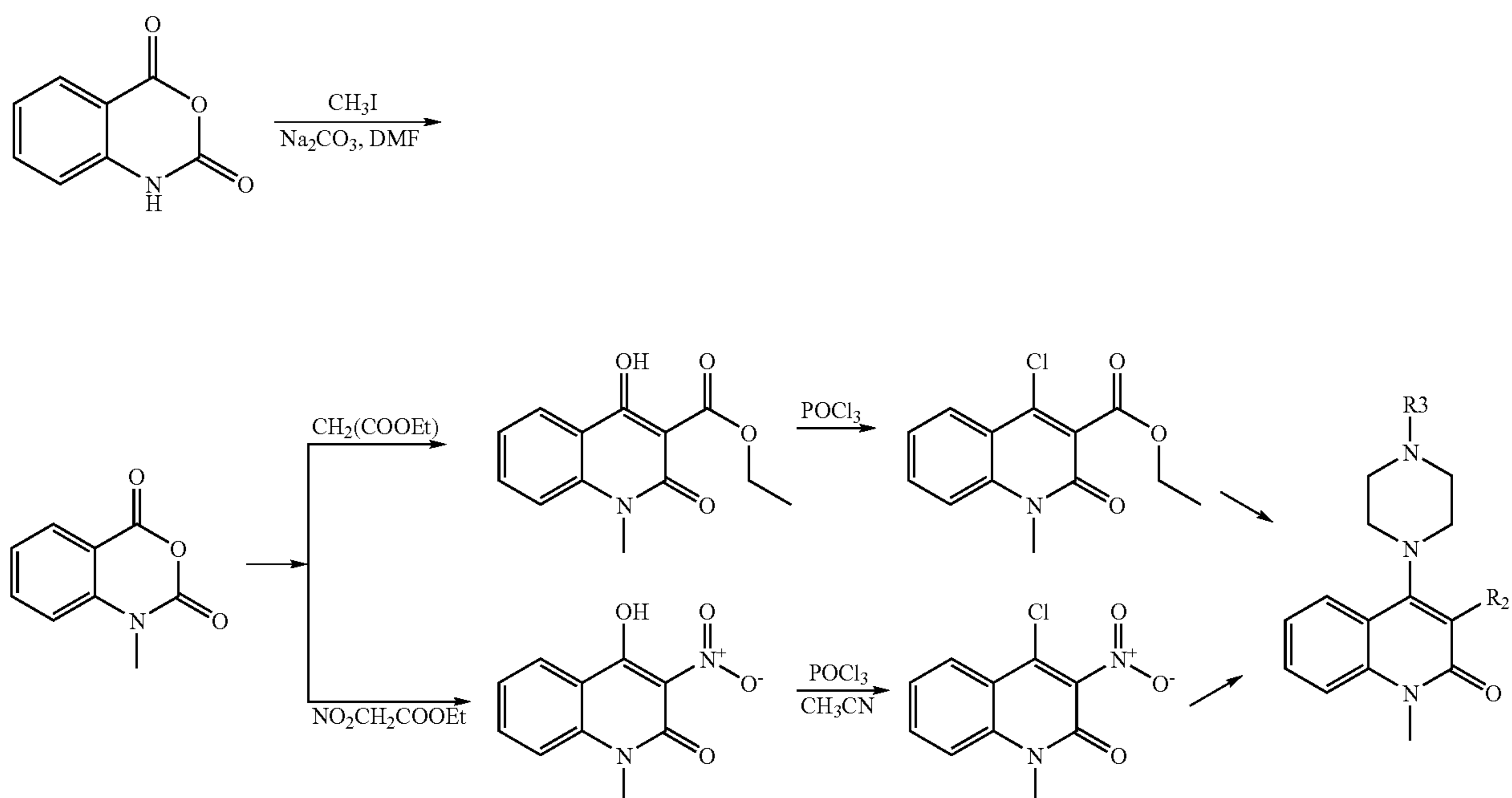
Reaction Scheme 9
