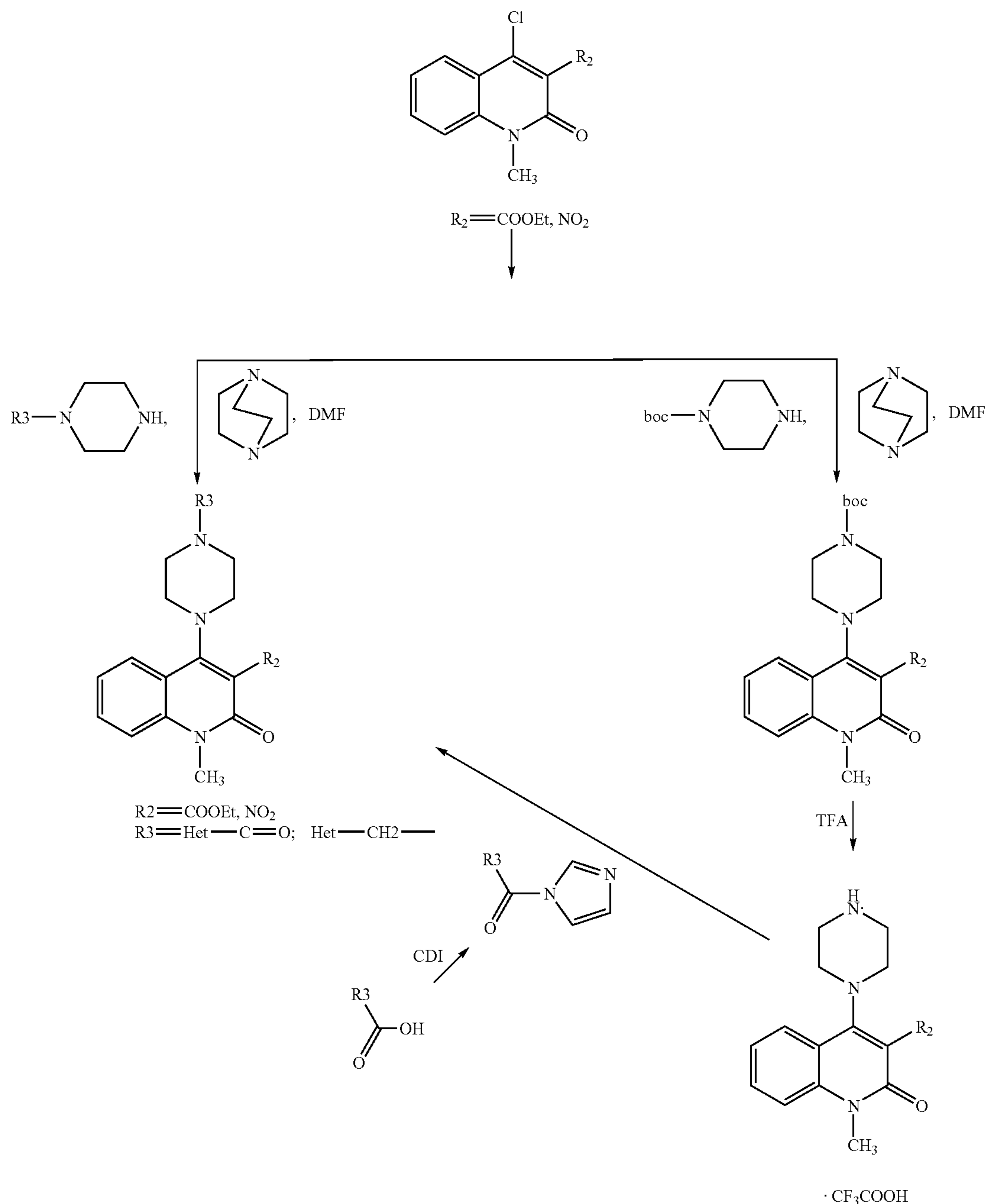
Reaction Scheme 10
