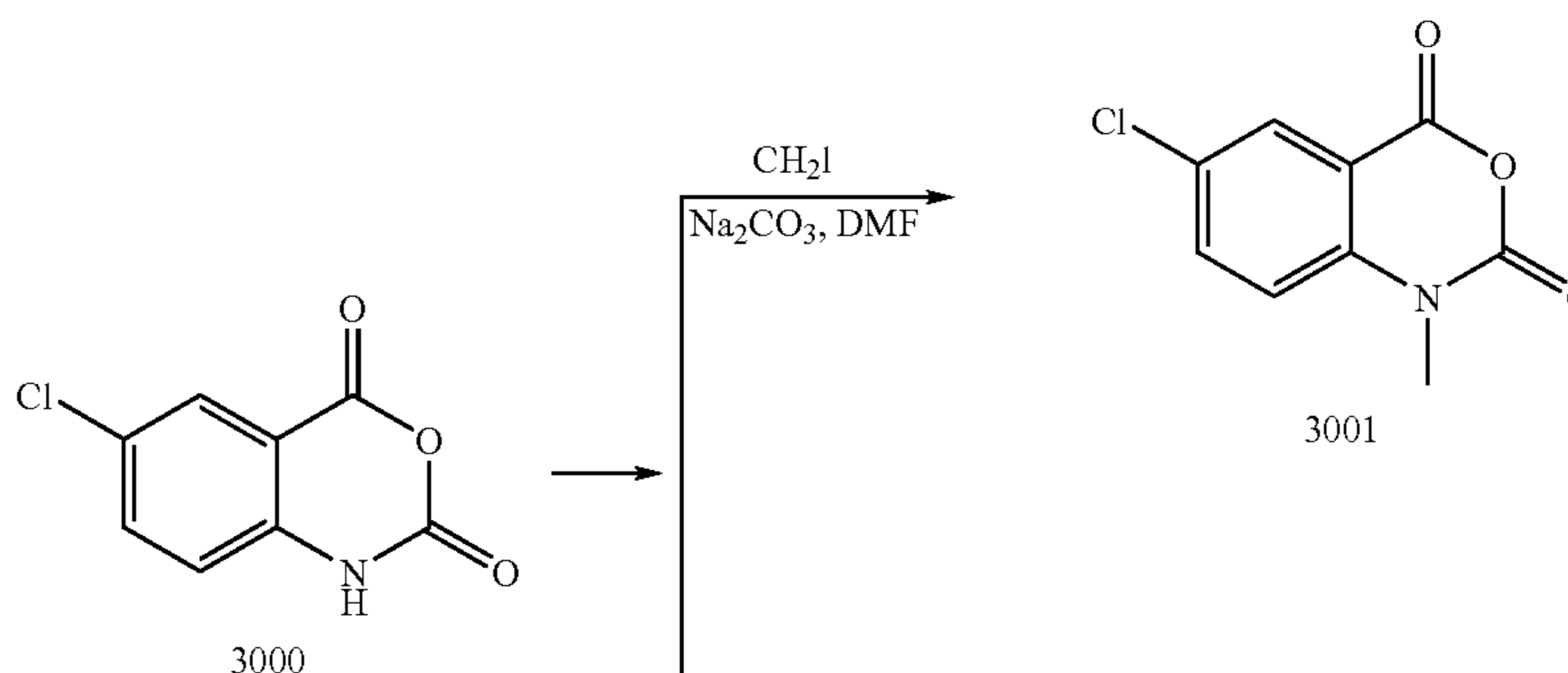
Reaction Scheme 26
