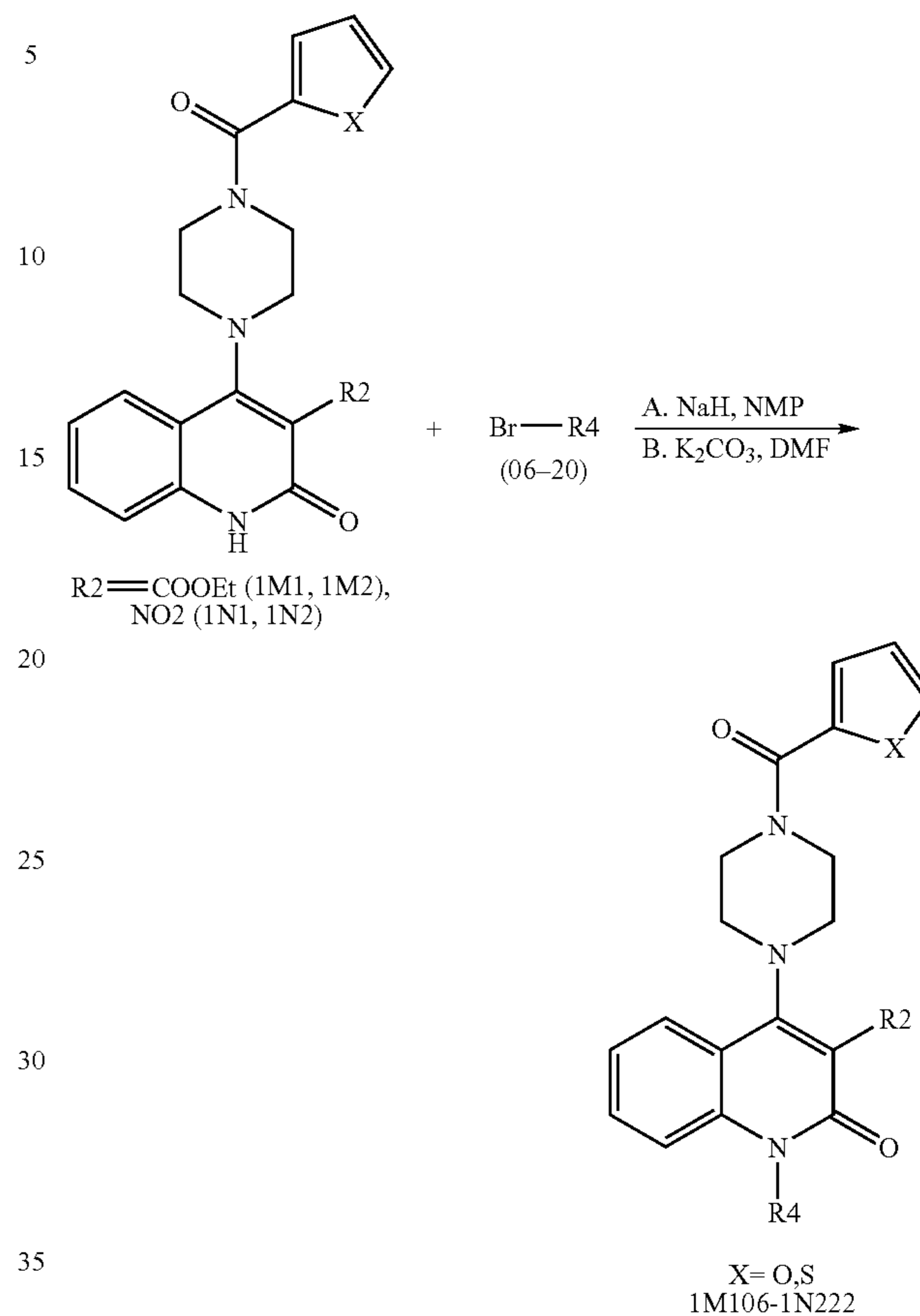
Reaction Scheme 13
