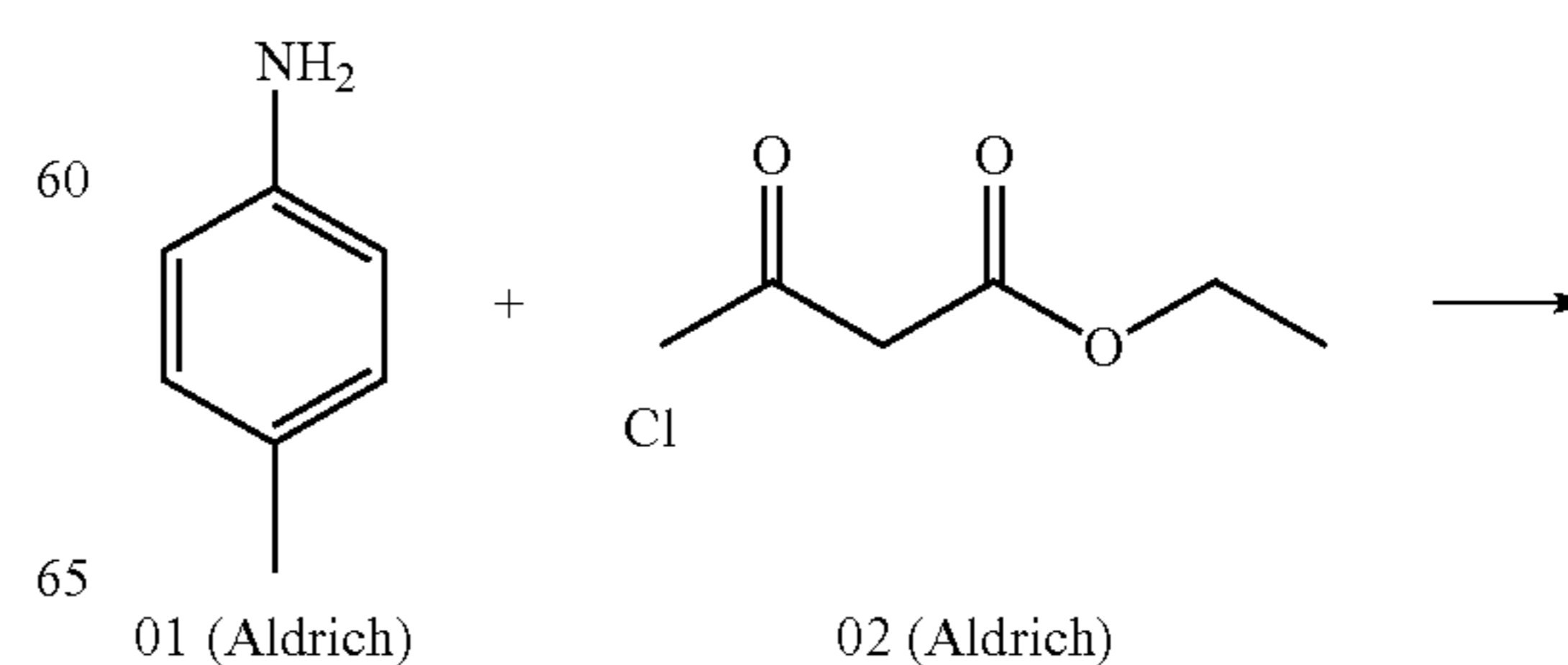
Reaction Scheme 25
