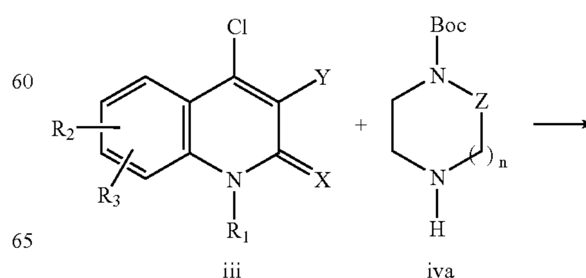
Reaction Scheme 4
