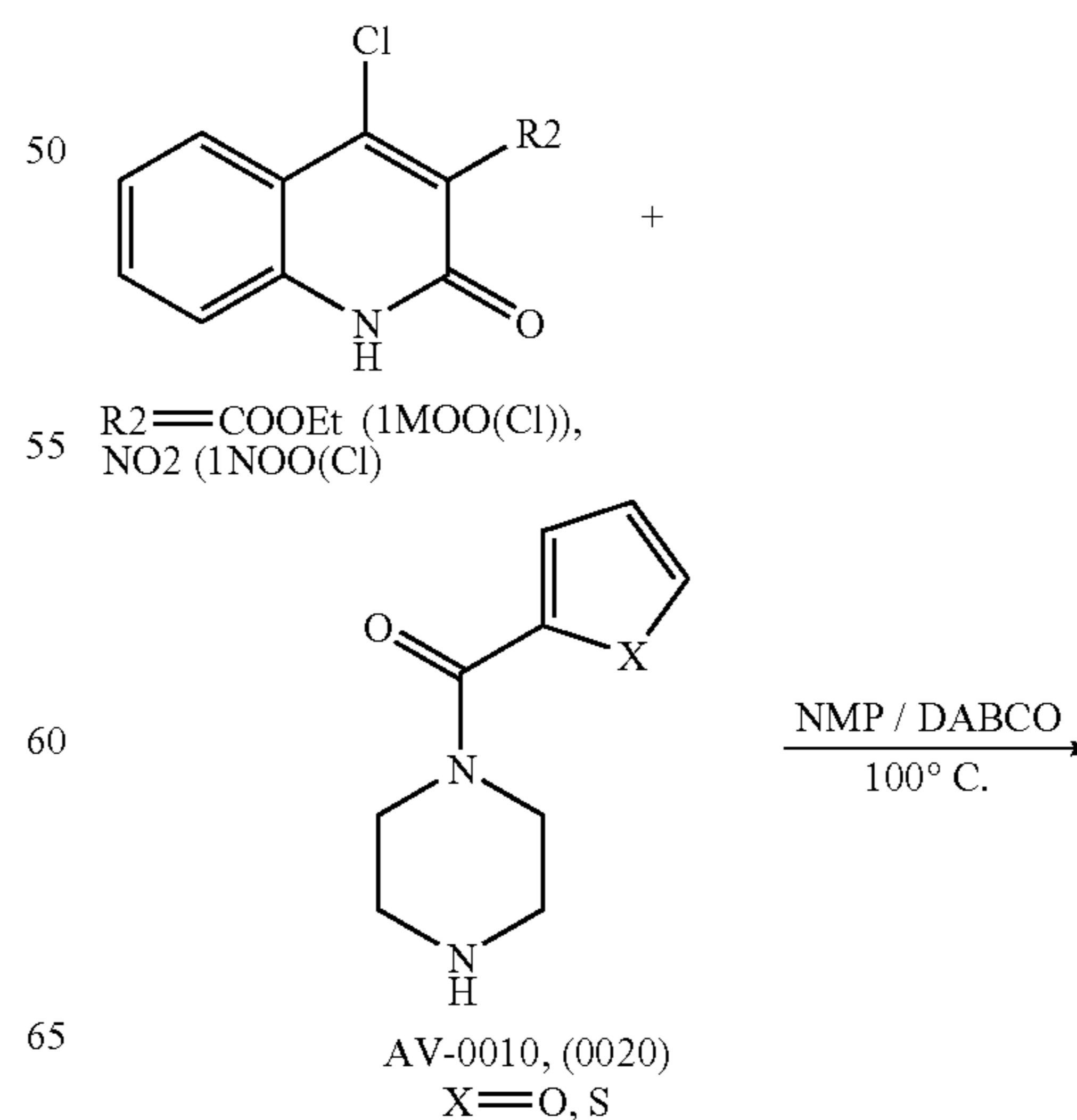
Reaction Scheme 12
