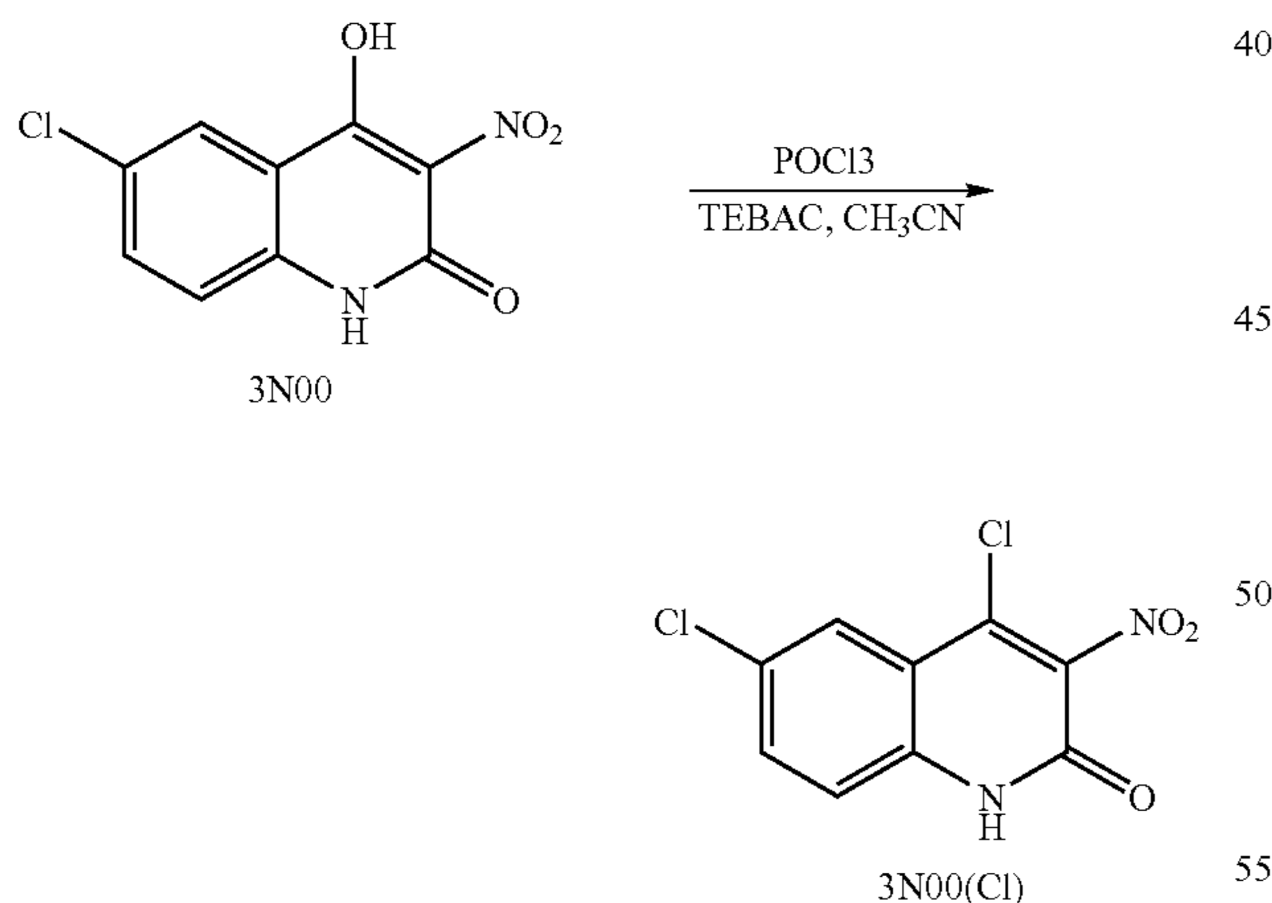
Reaction Scheme 27
