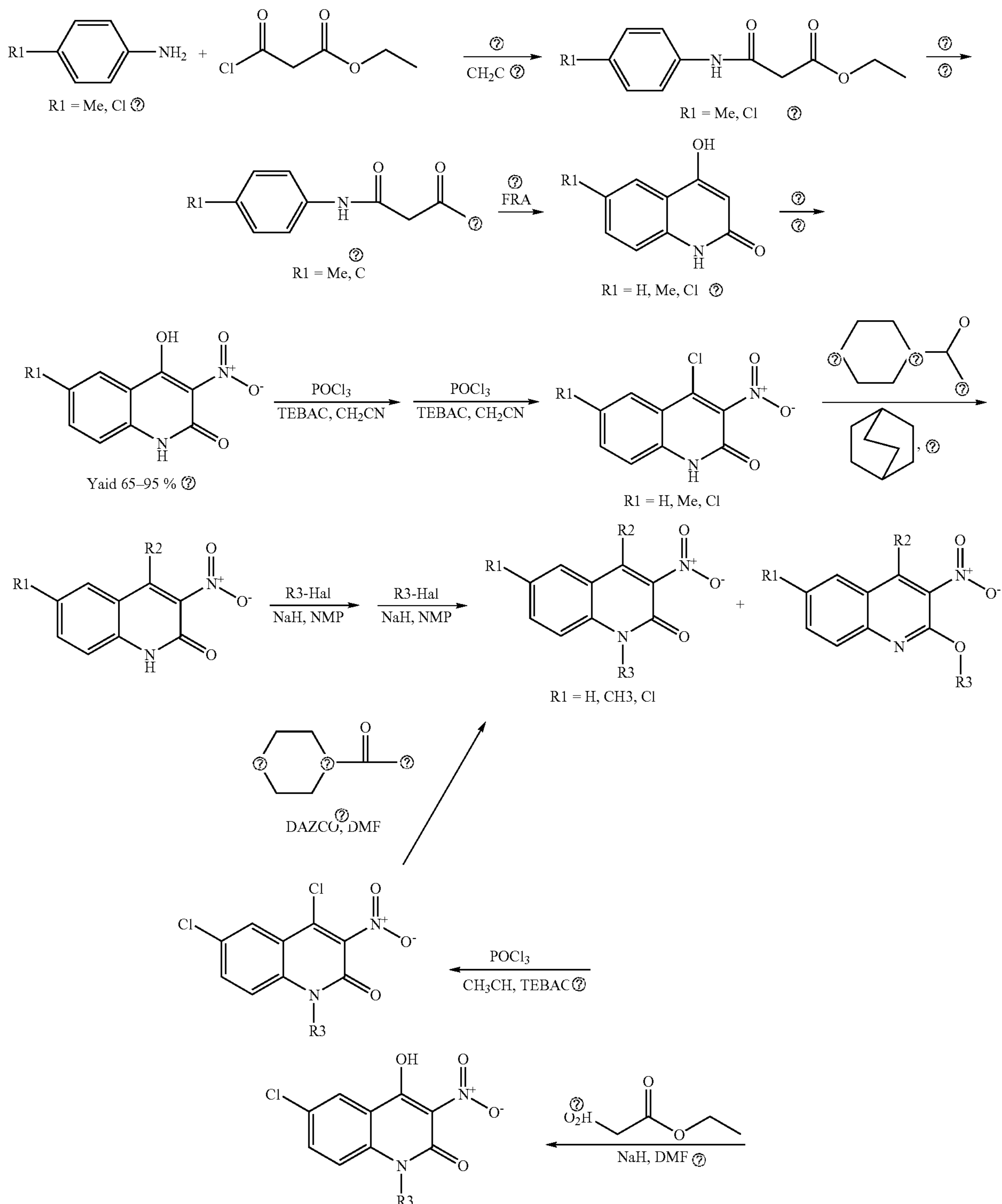
Reaction Scheme 22
