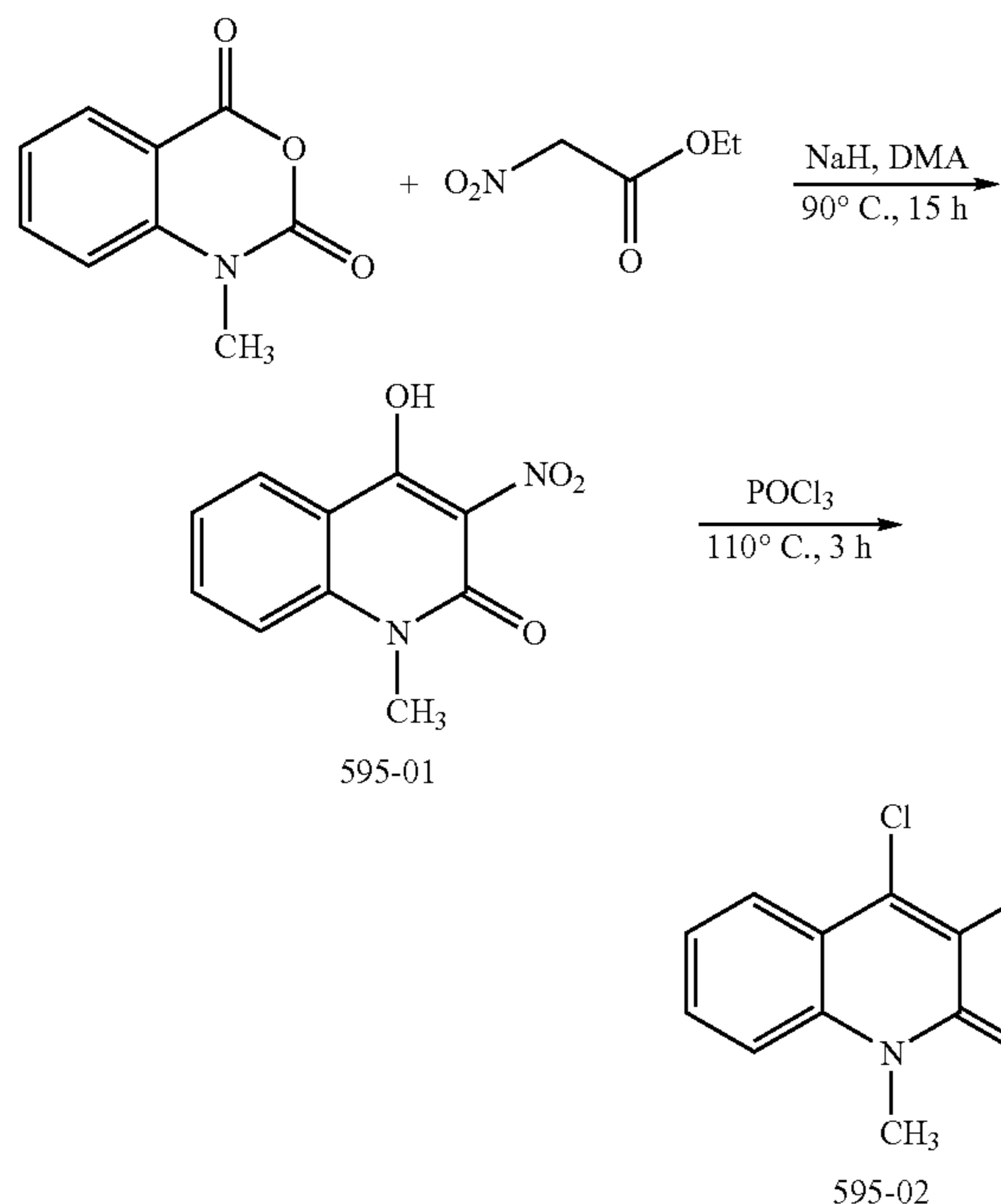
4-Chloro-1-methyl-3-nitro-1H-quinolin-2-one (Referred to as 595-02)
