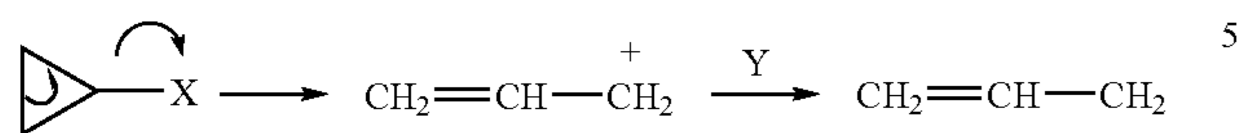
Reaction Scheme 7
