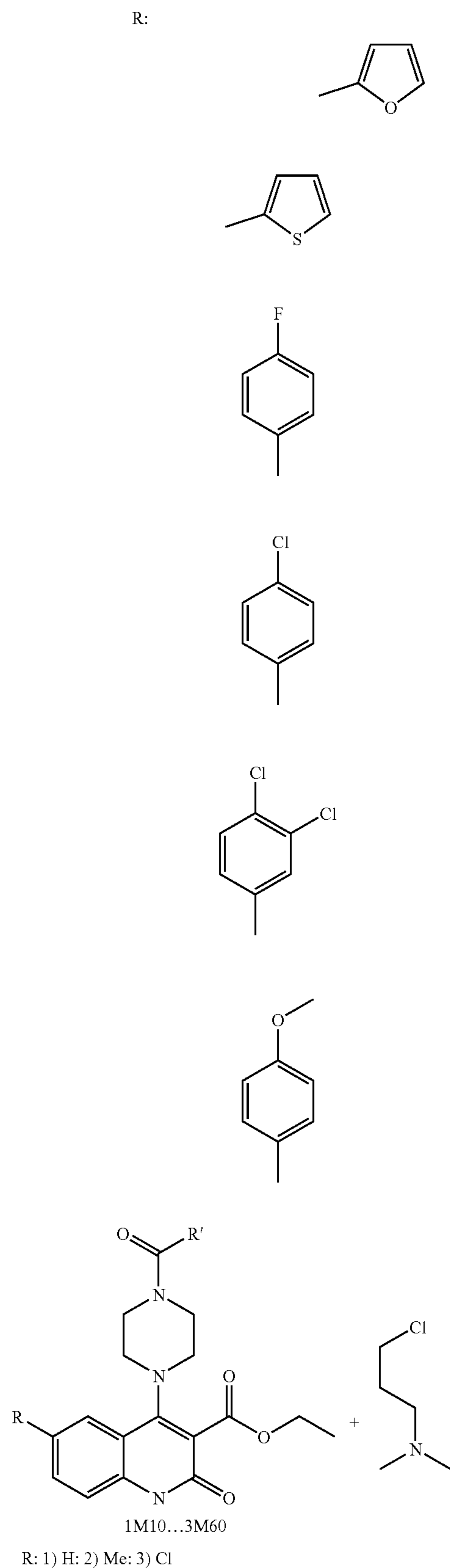
Reaction Scheme 24
