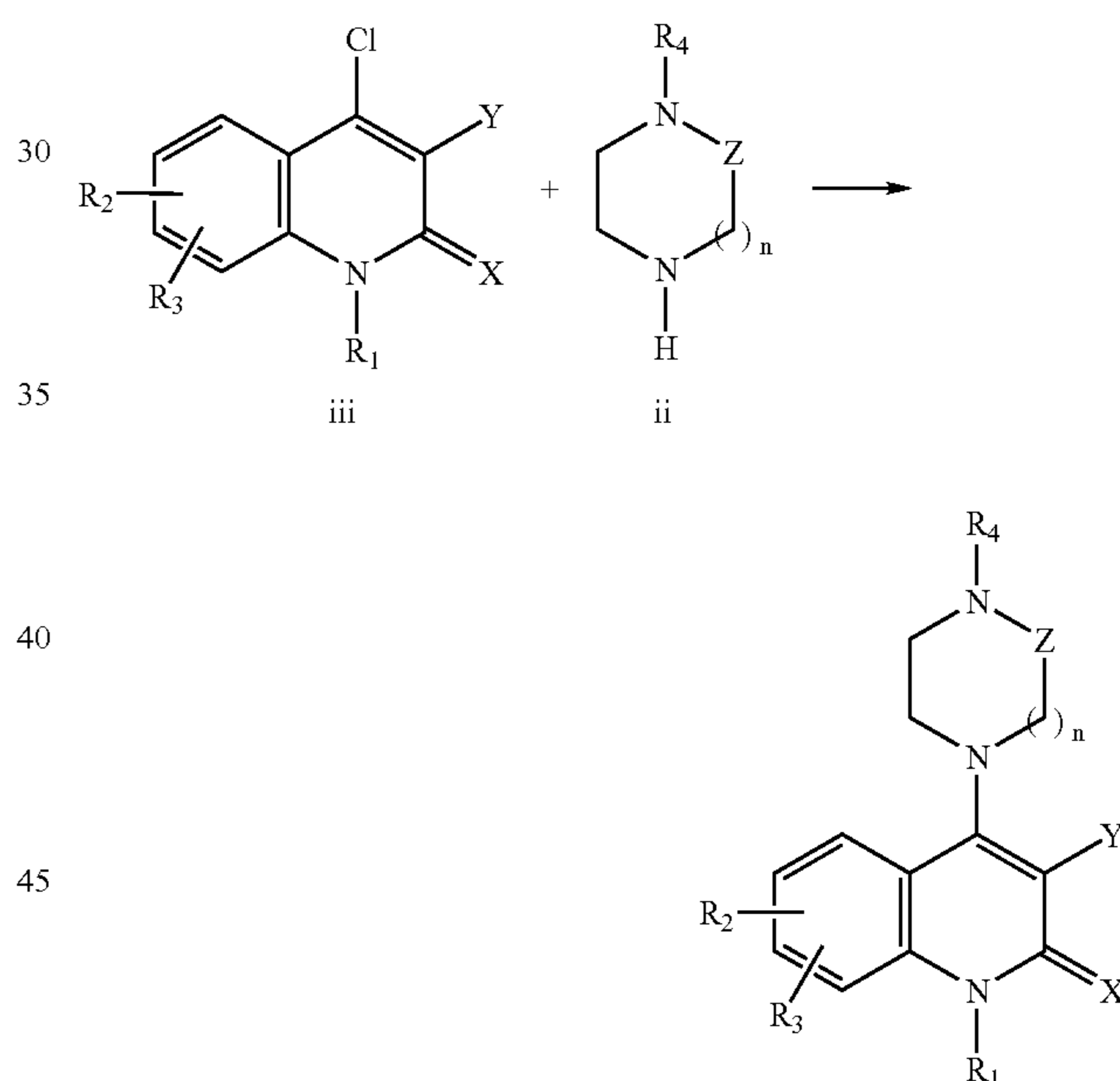
Reaction Scheme 3
