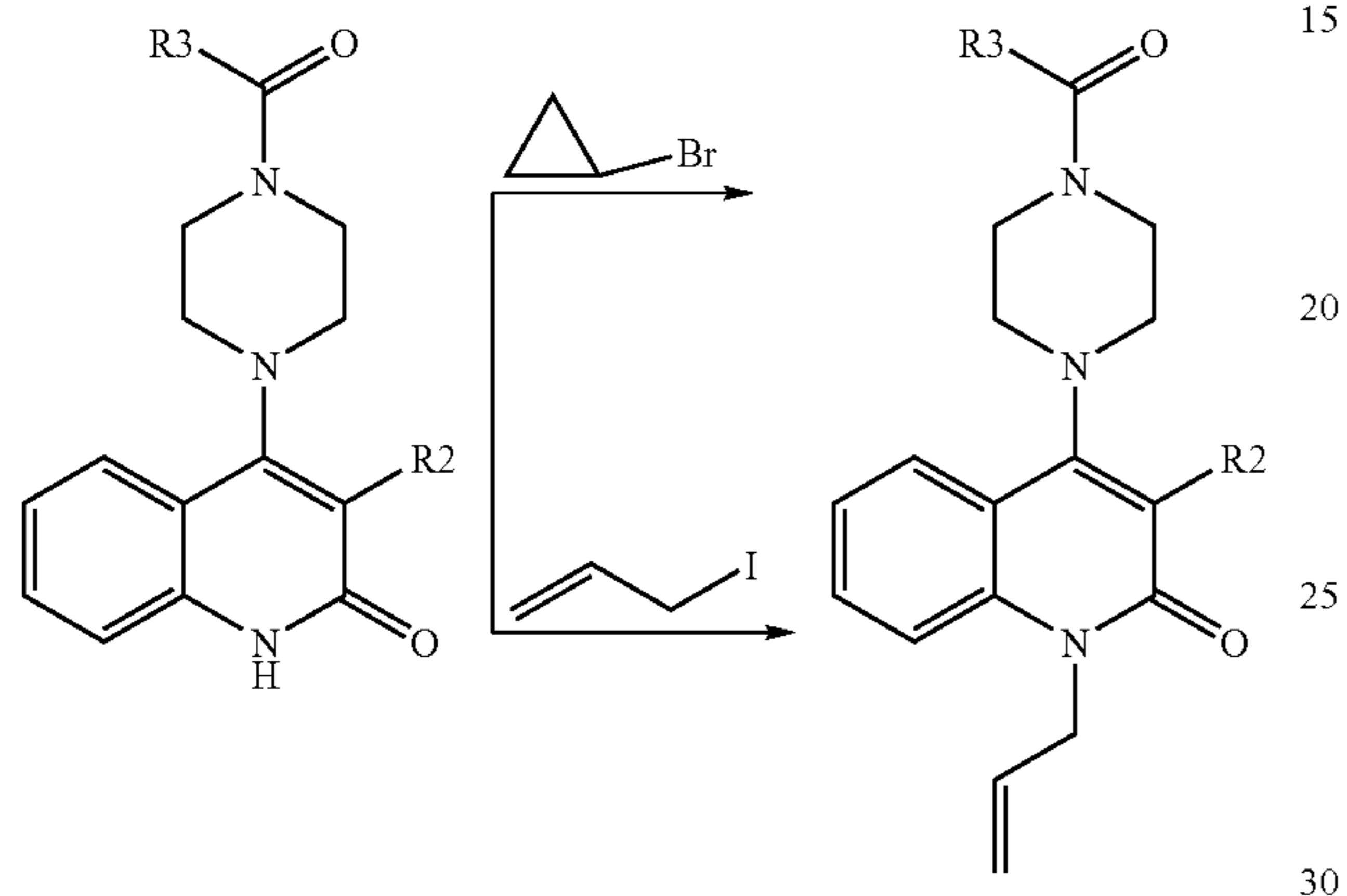
Reaction Scheme 8
