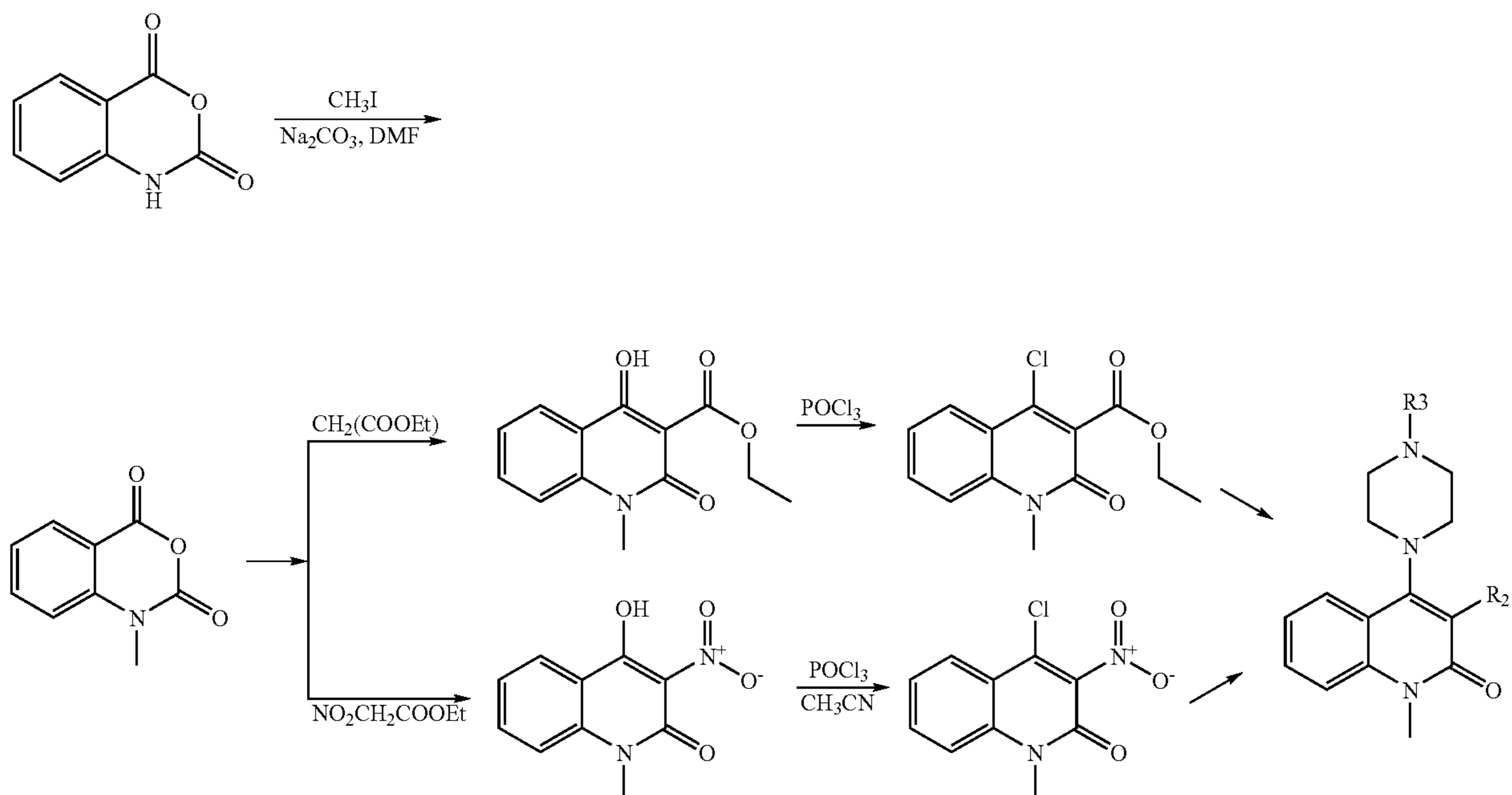
Reaction Scheme 9
