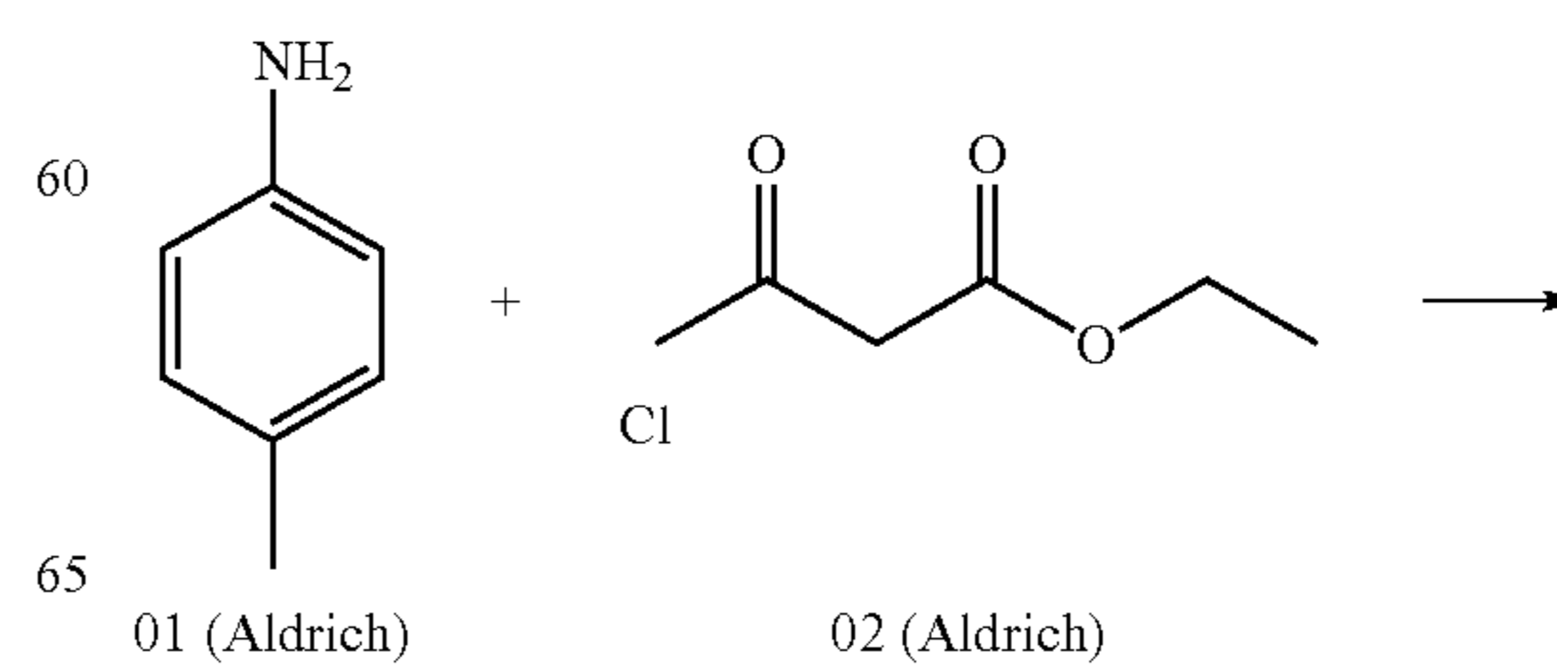
Reaction Scheme 25
