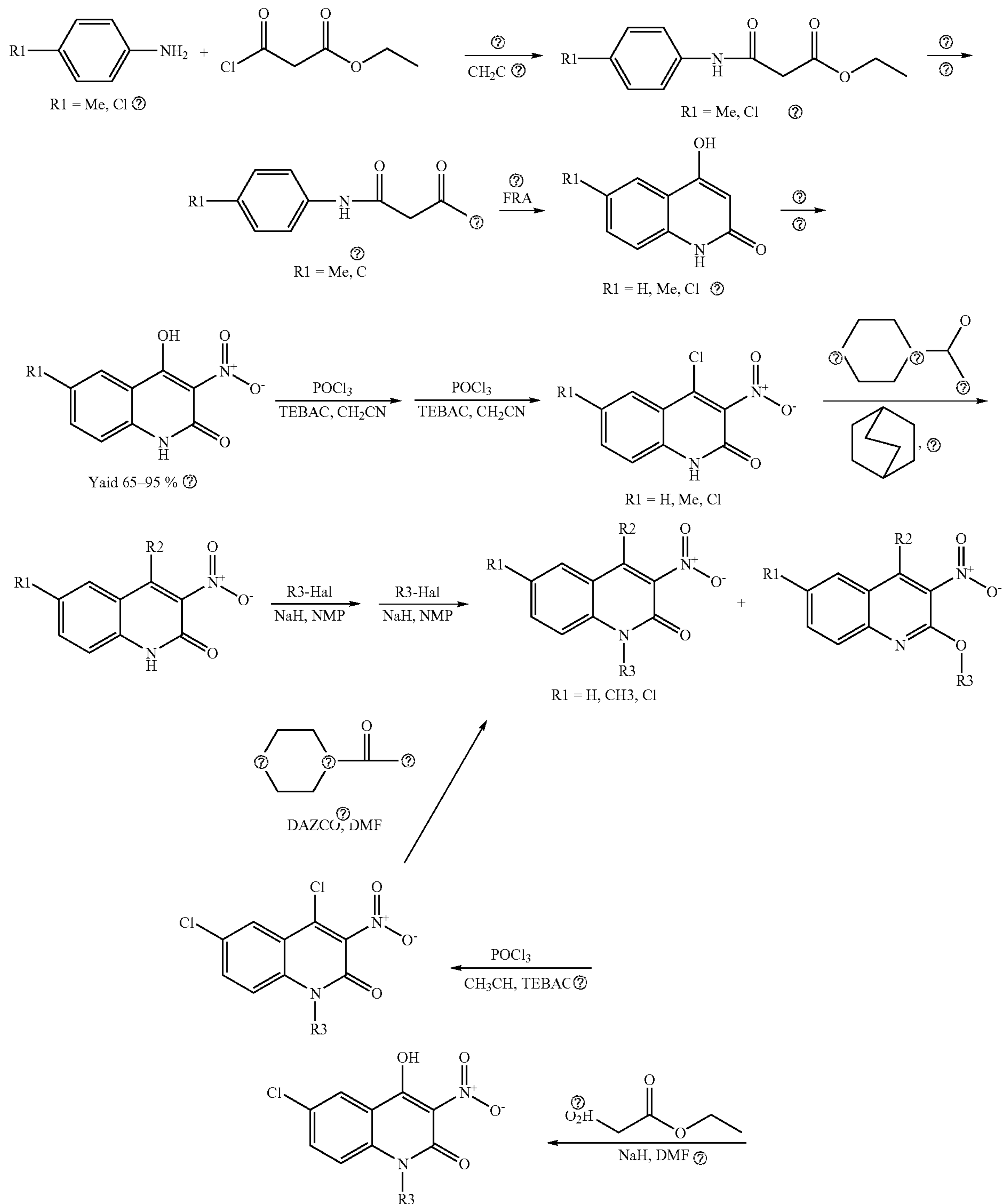
Reaction Scheme 22
