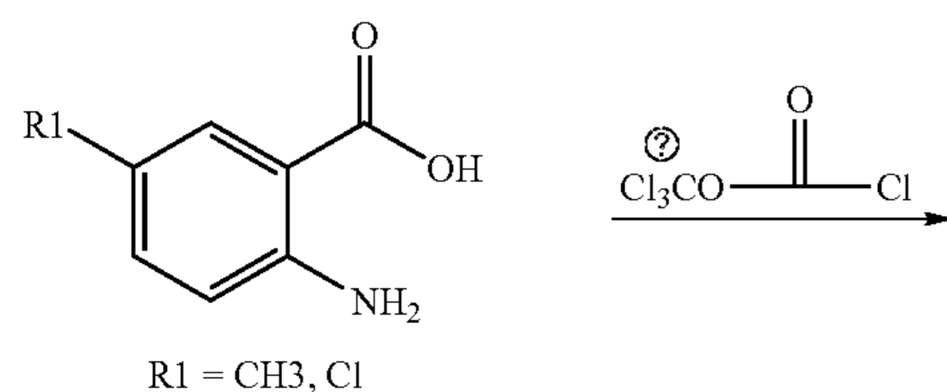
Reaction Scheme 21
