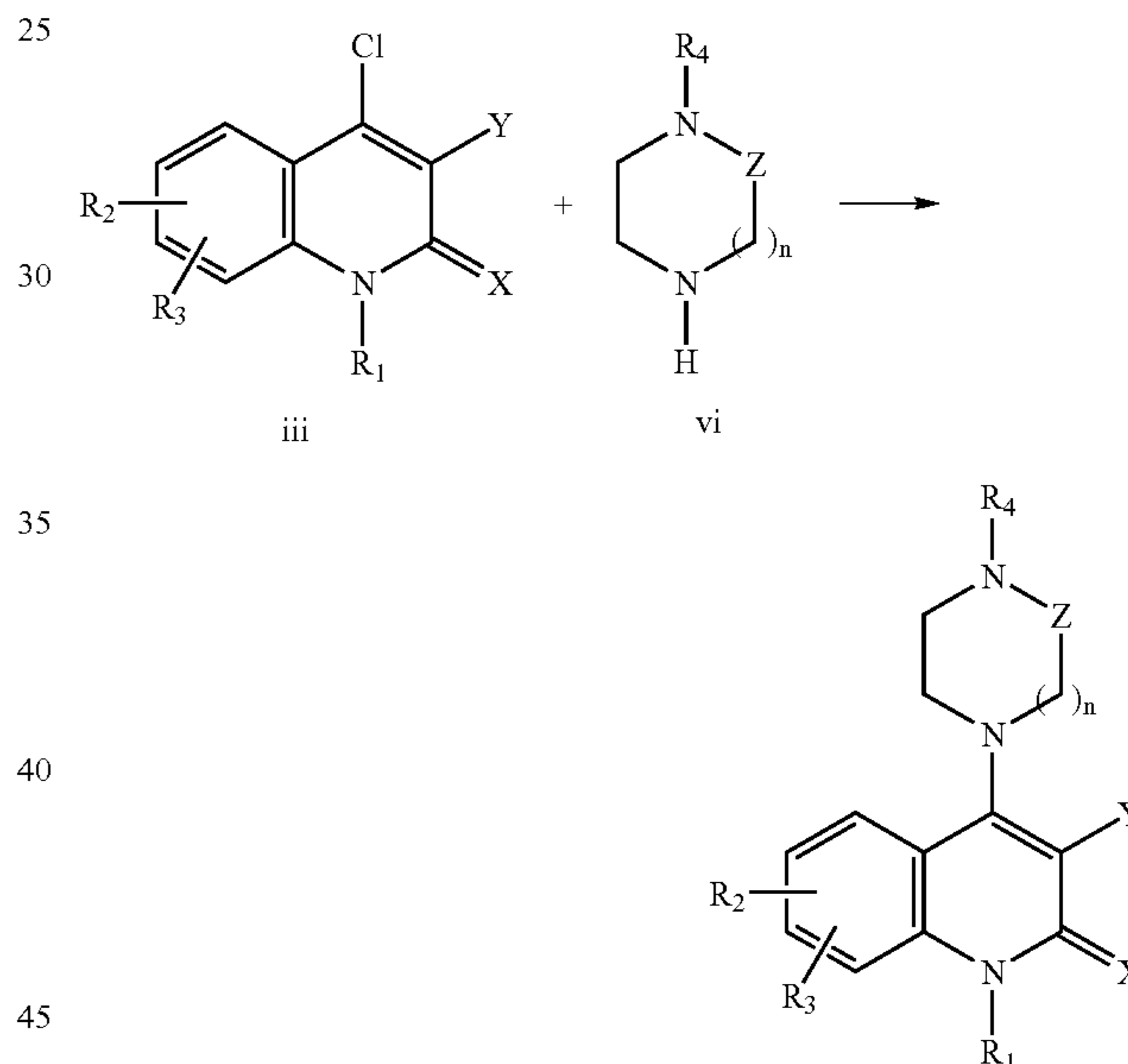
Reaction Scheme 3
