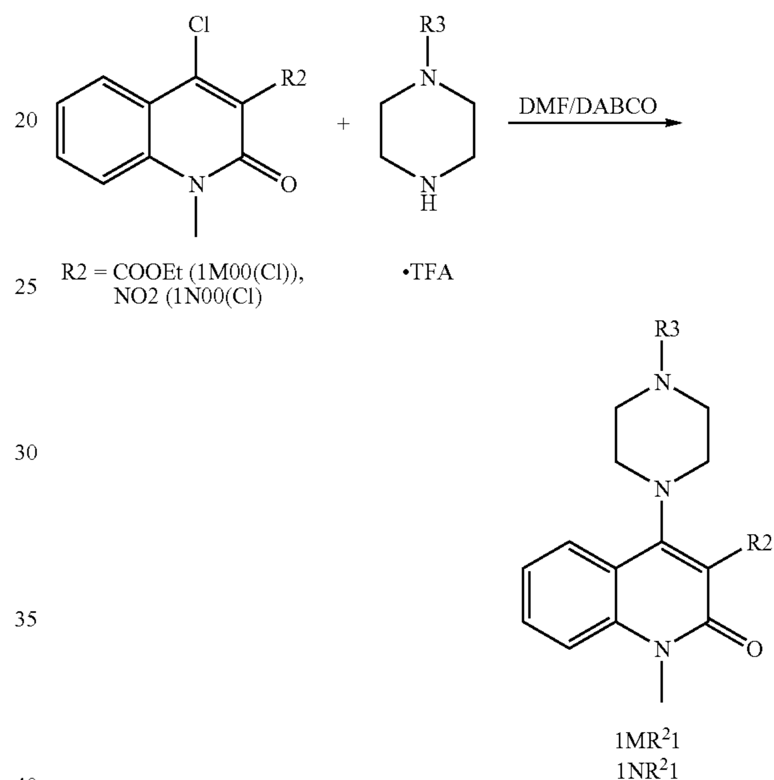
Reaction Scheme 16
