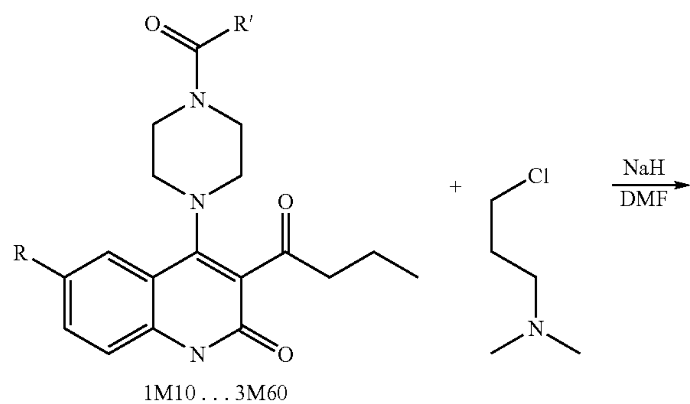
Reaction Scheme 24
