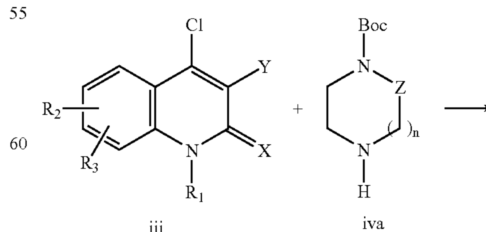
Reaction Scheme 4
