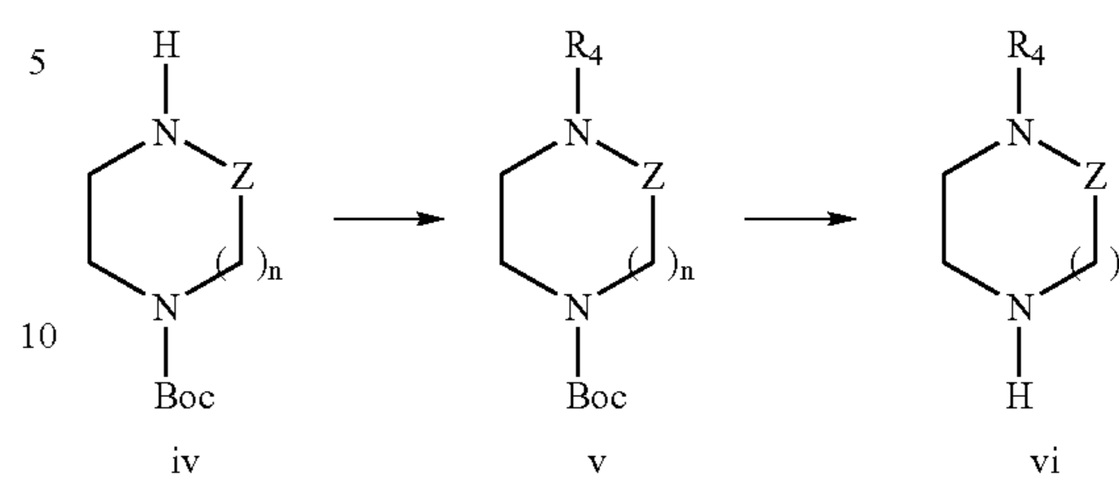
Reaction Scheme 2
