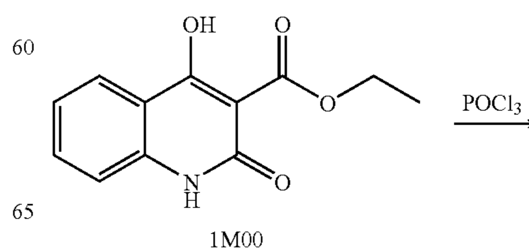
Reaction Scheme 11
