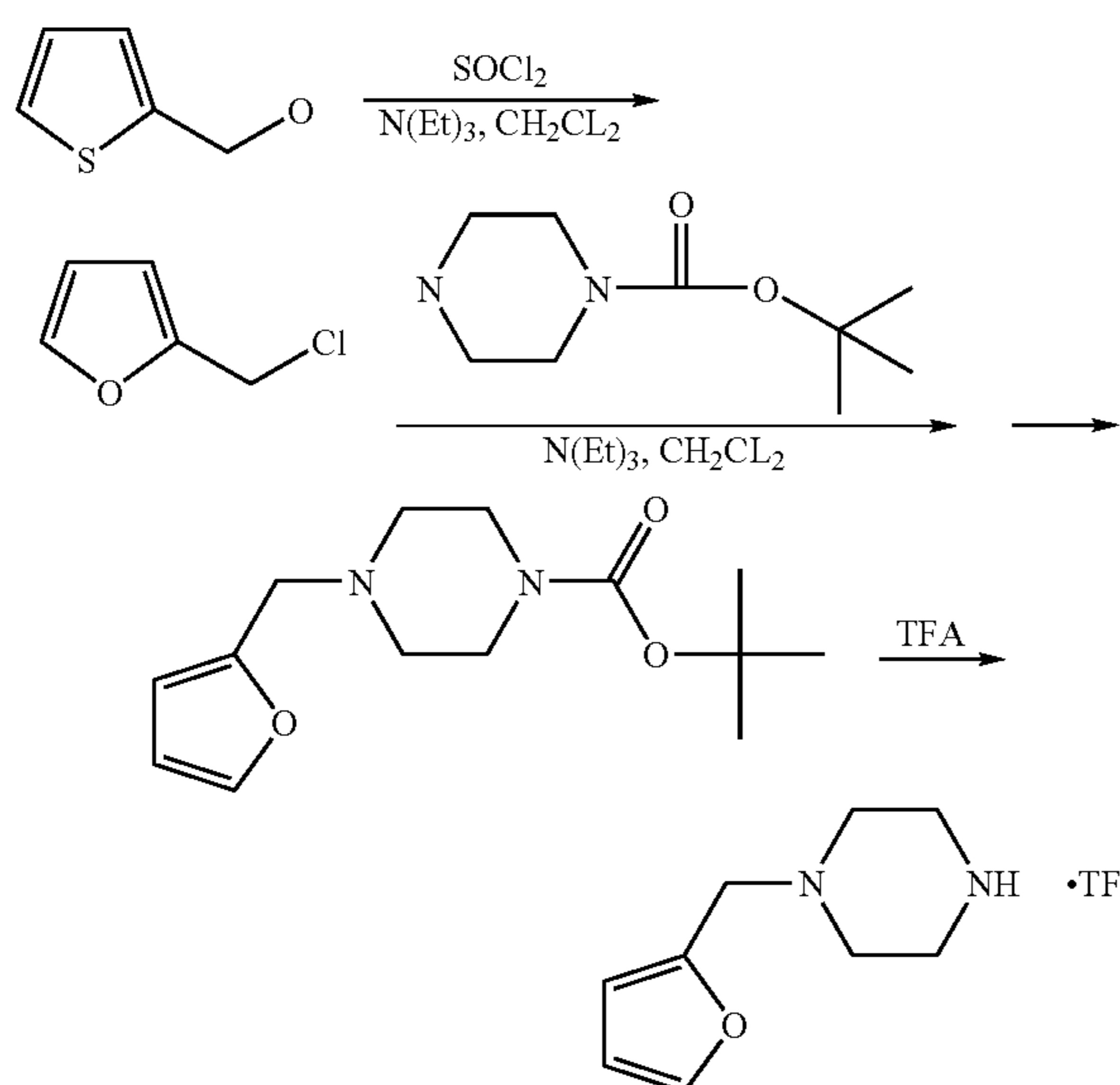
Reaction Scheme 22
