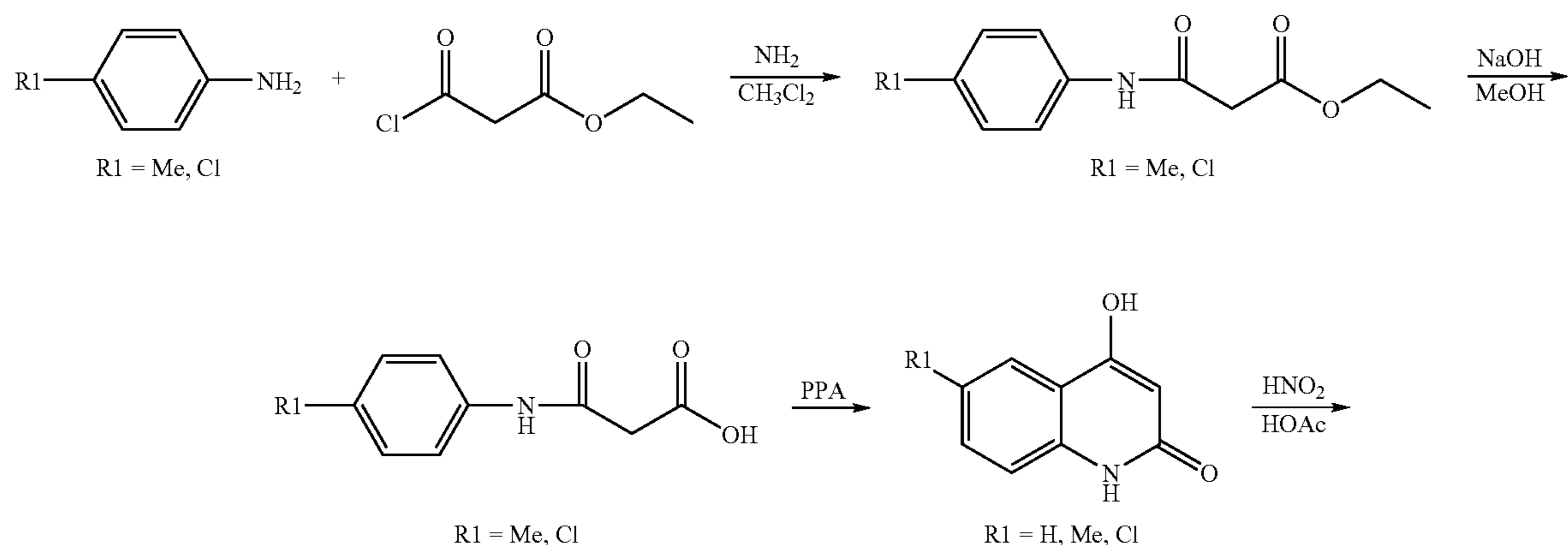
Reaction Scheme 22
