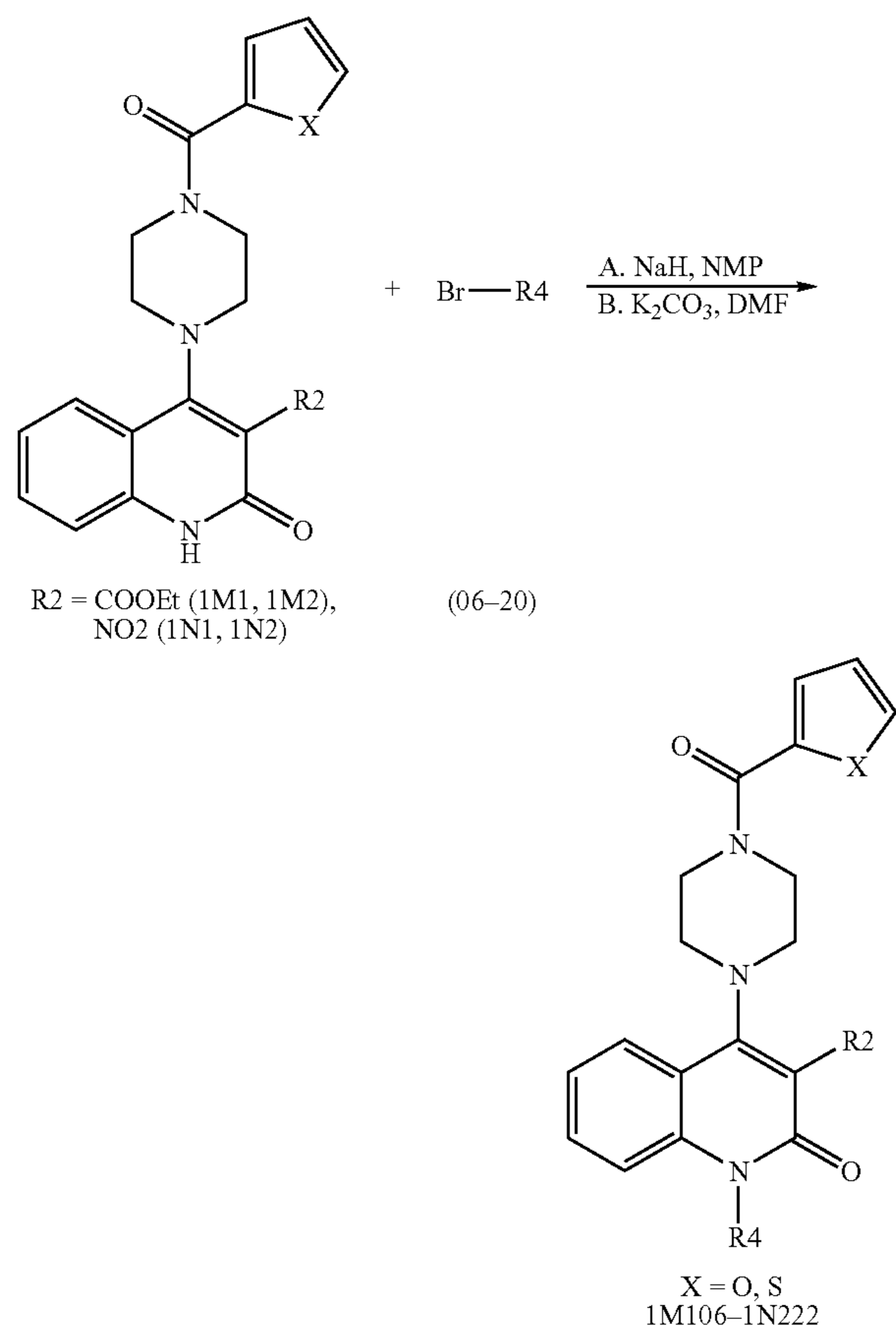
Reaction Scheme 13
