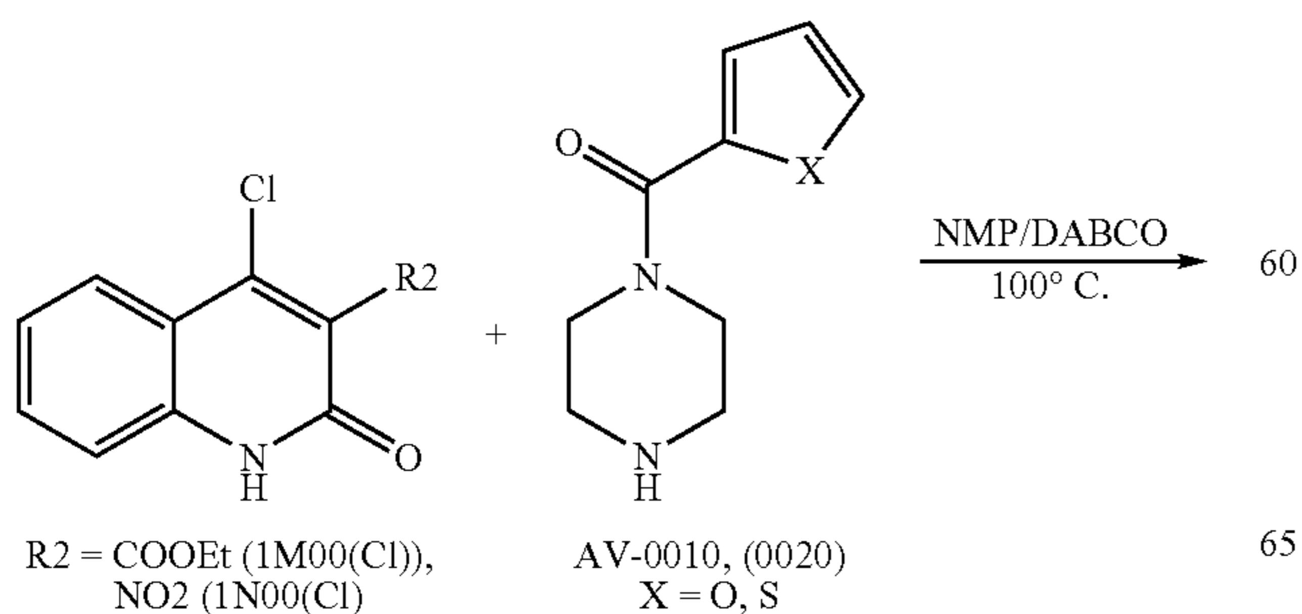
Reaction Scheme 12
