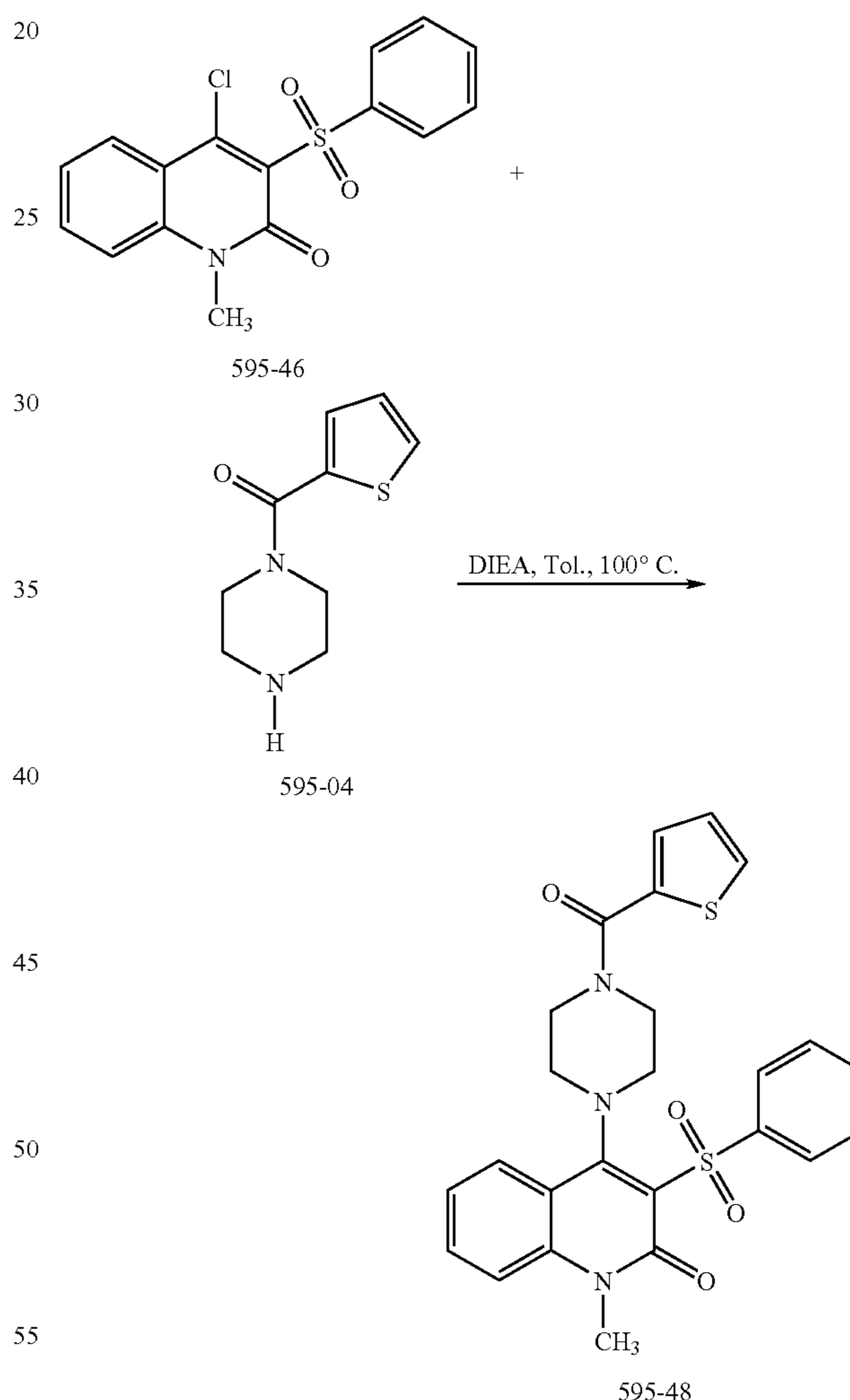
4-Hydroxy-3-methanesulfonyl-1-methyl-1H-quinolin-2-one (Referred to as 595-05)
