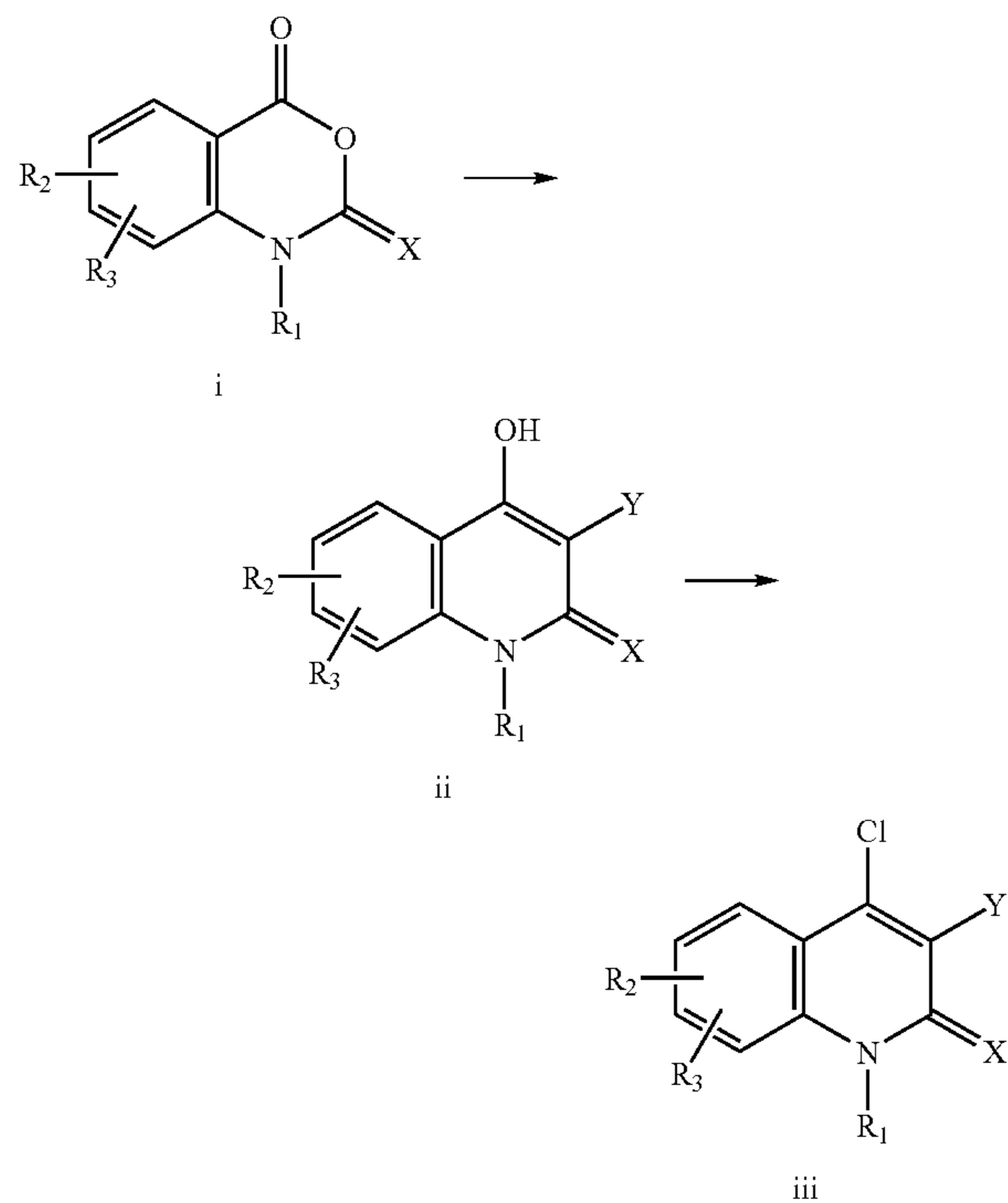
Reaction Scheme 1
