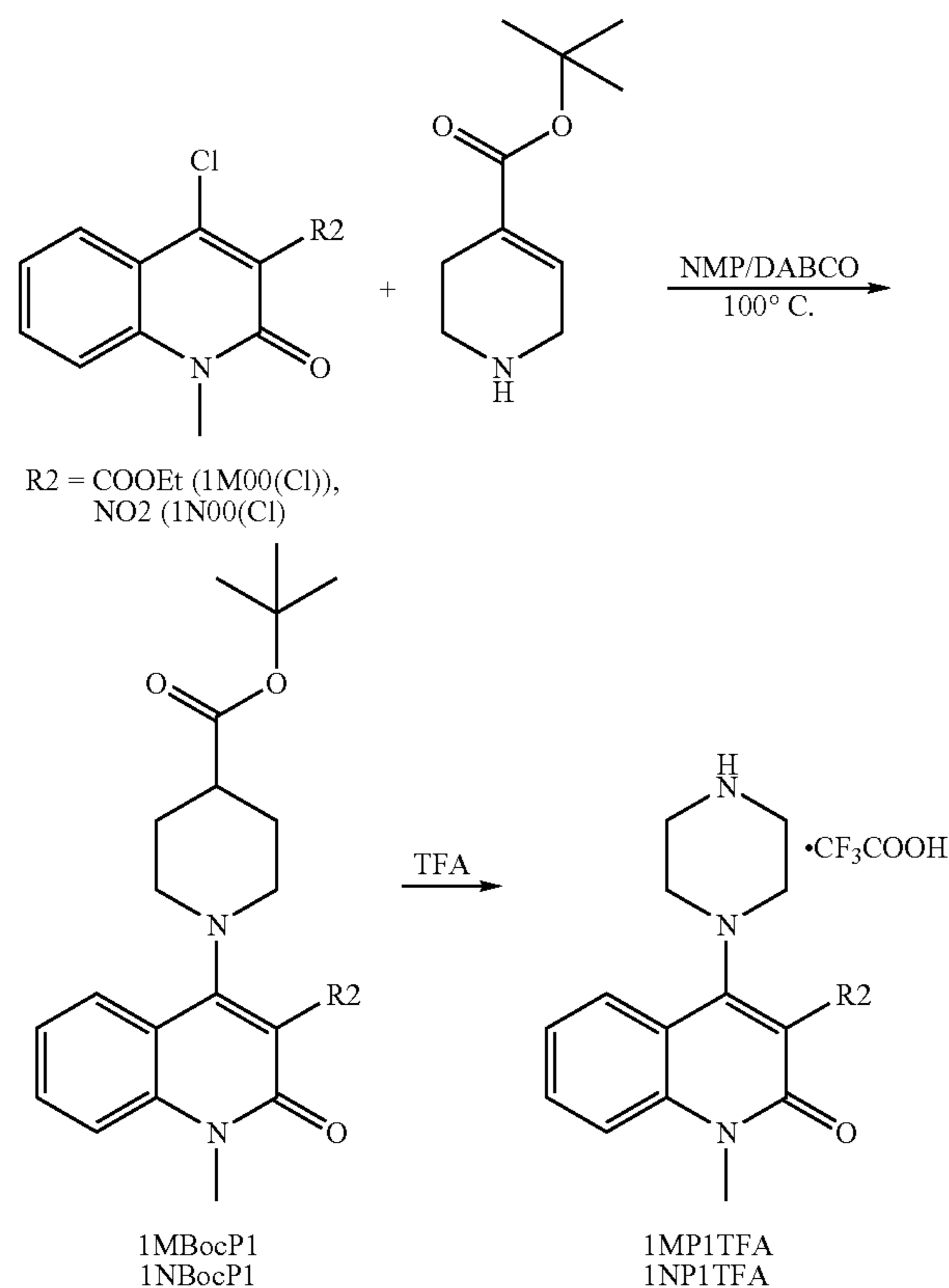
Reaction Scheme 15
