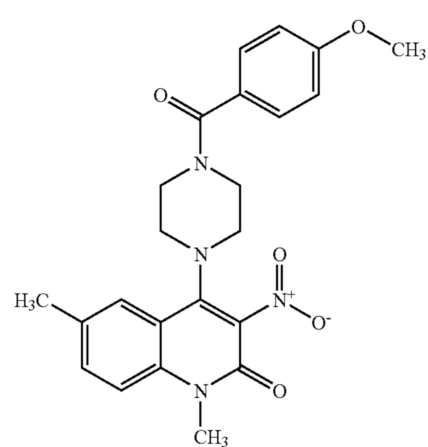
Compound 193
