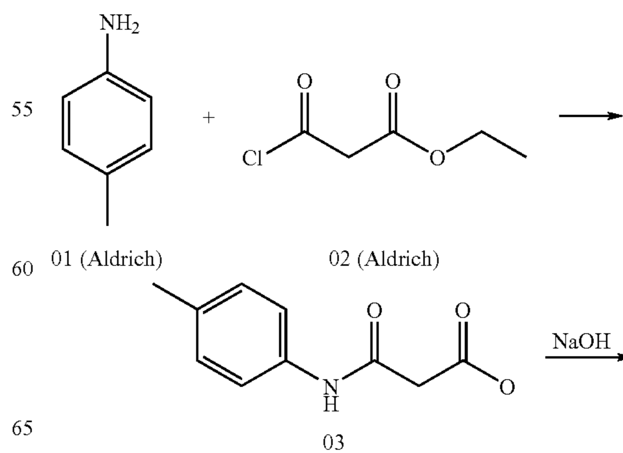
Reaction Scheme 25
