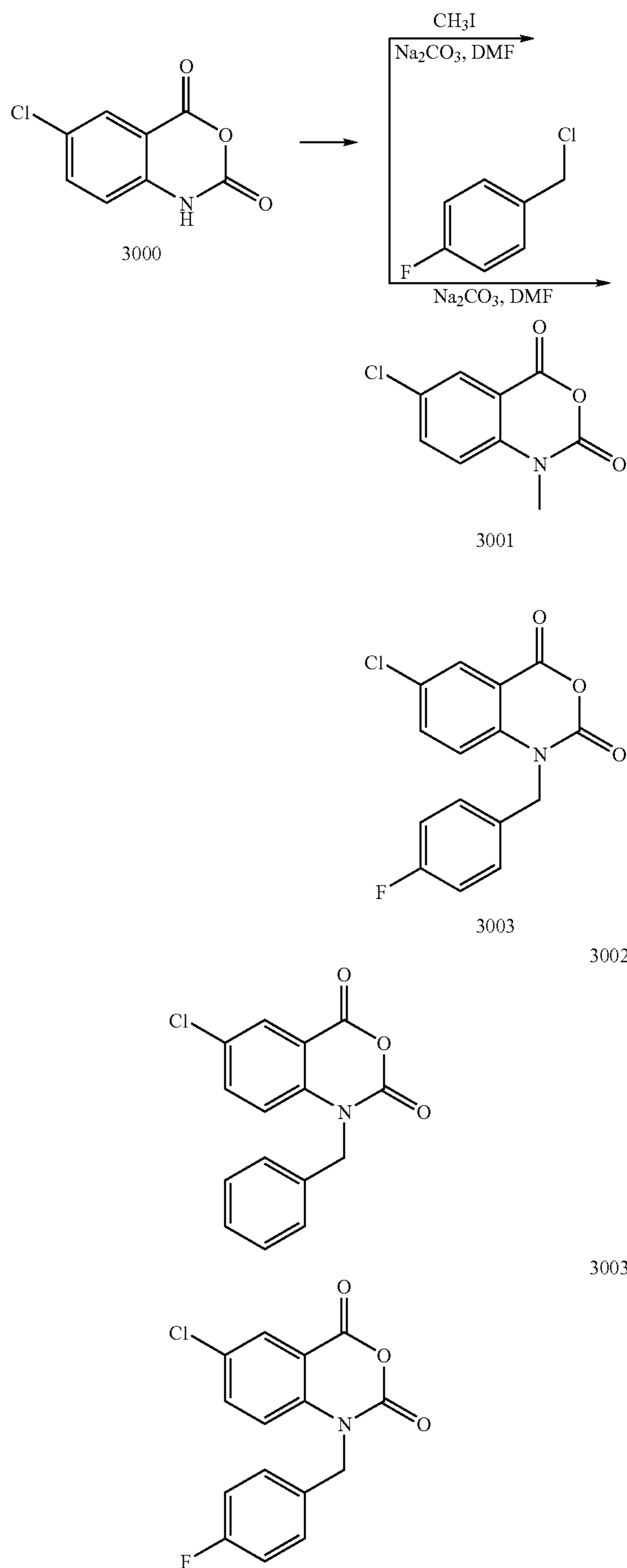
Reaction Scheme 26
