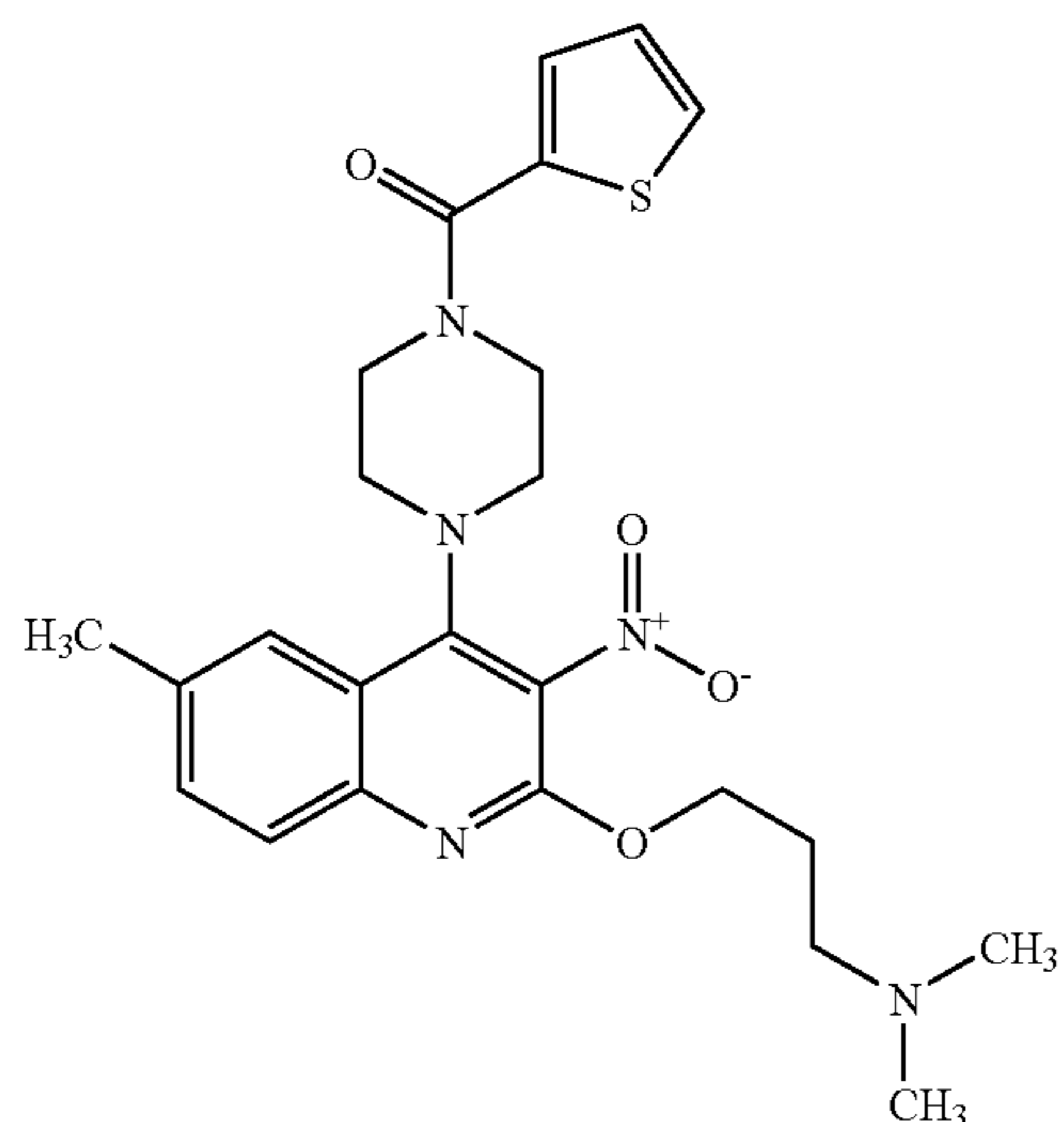
Compound 344
