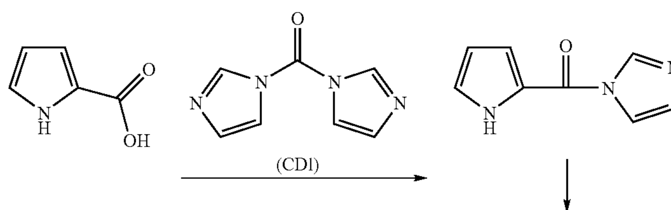
Reaction Scheme 17
