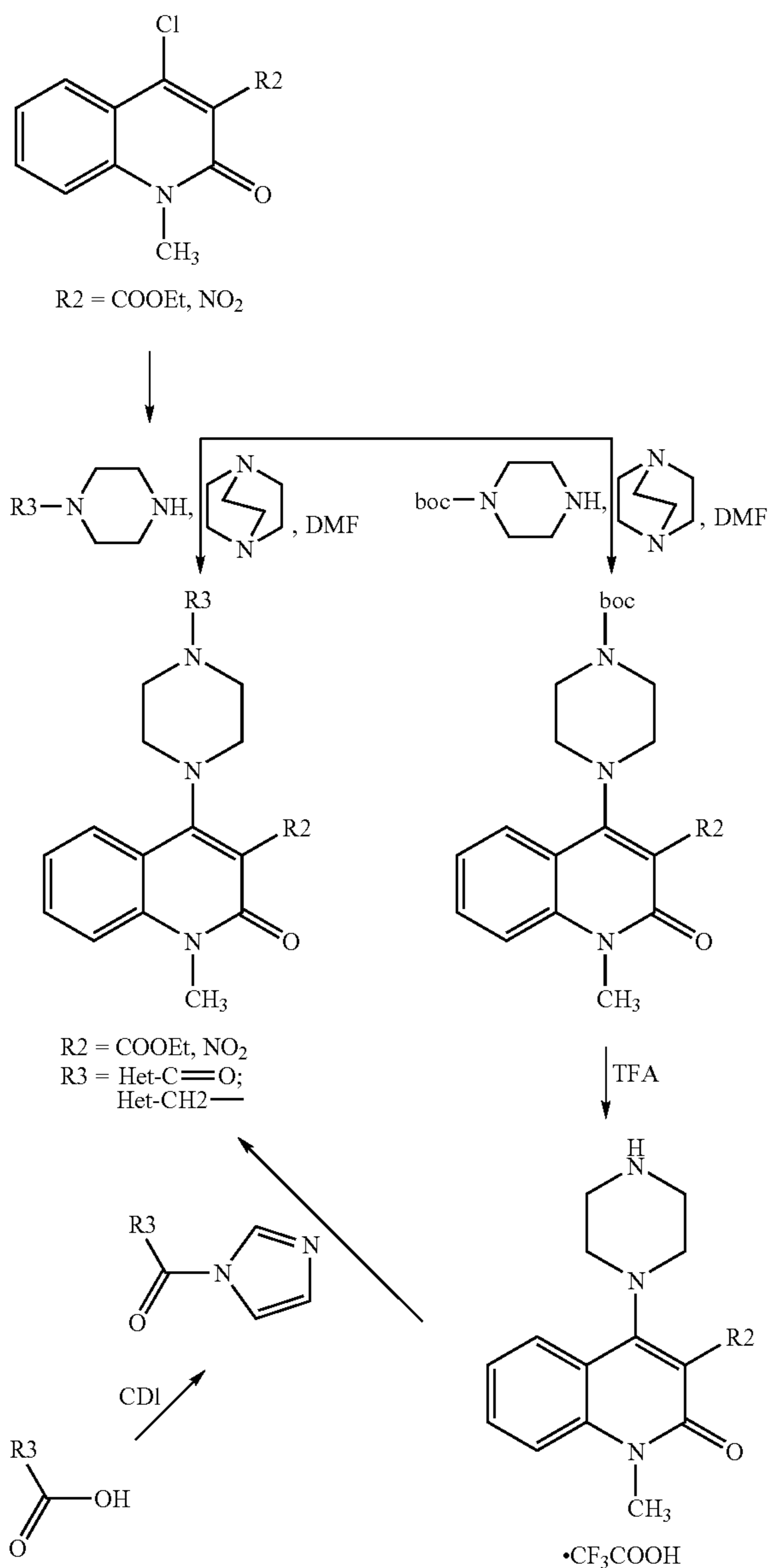
Reaction Scheme 10
