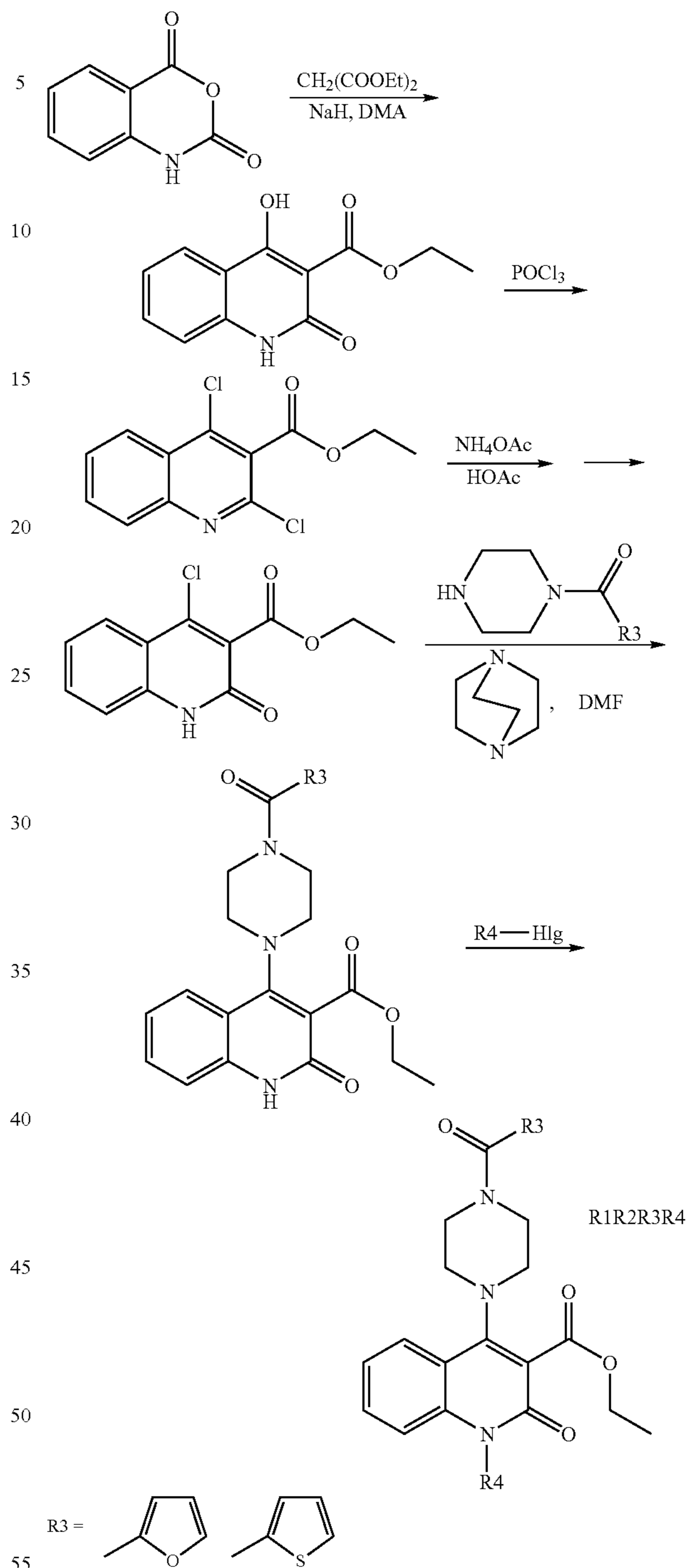
Compound 343
