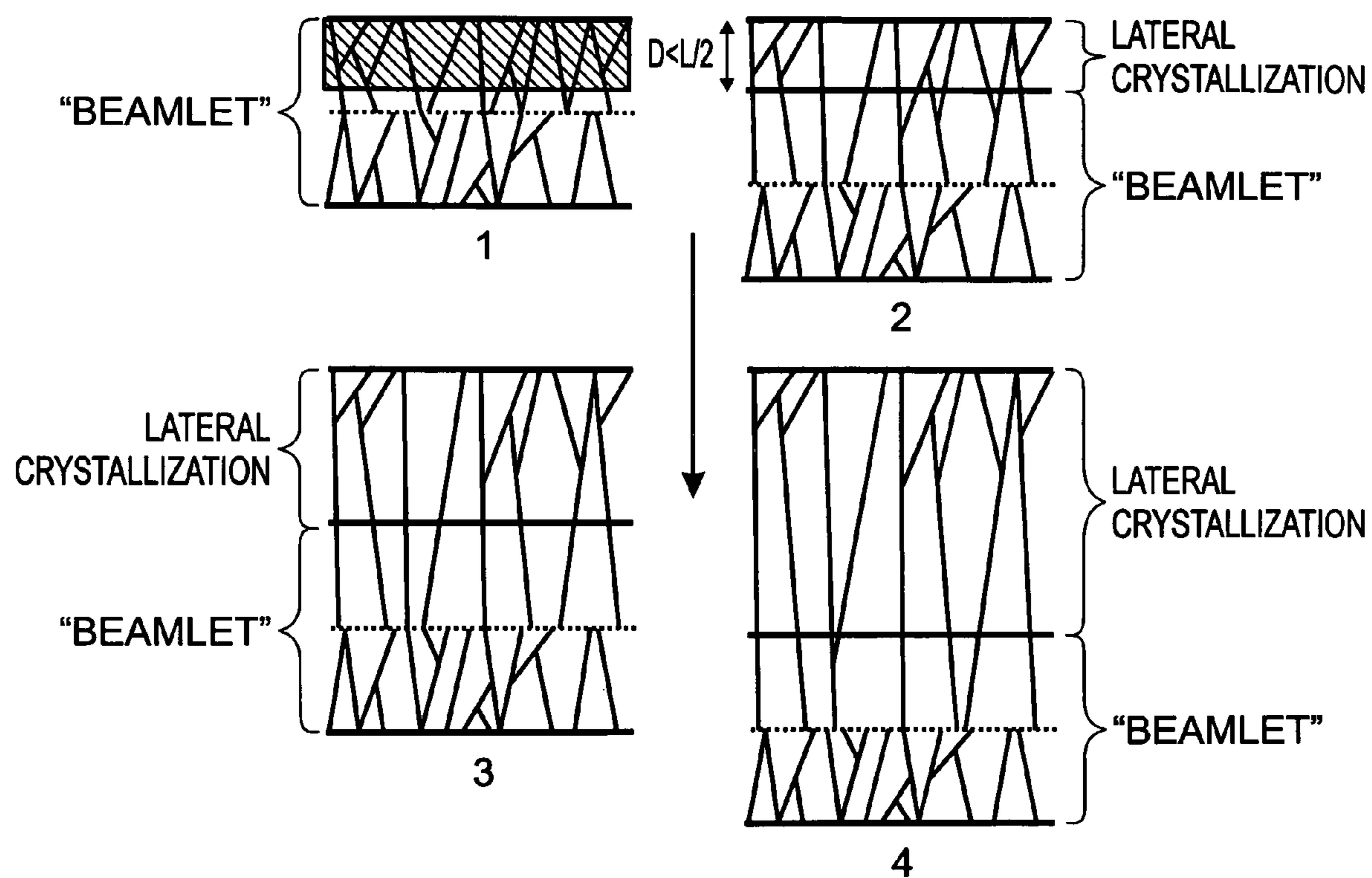
Fig. 2 (PRIOR ART)
