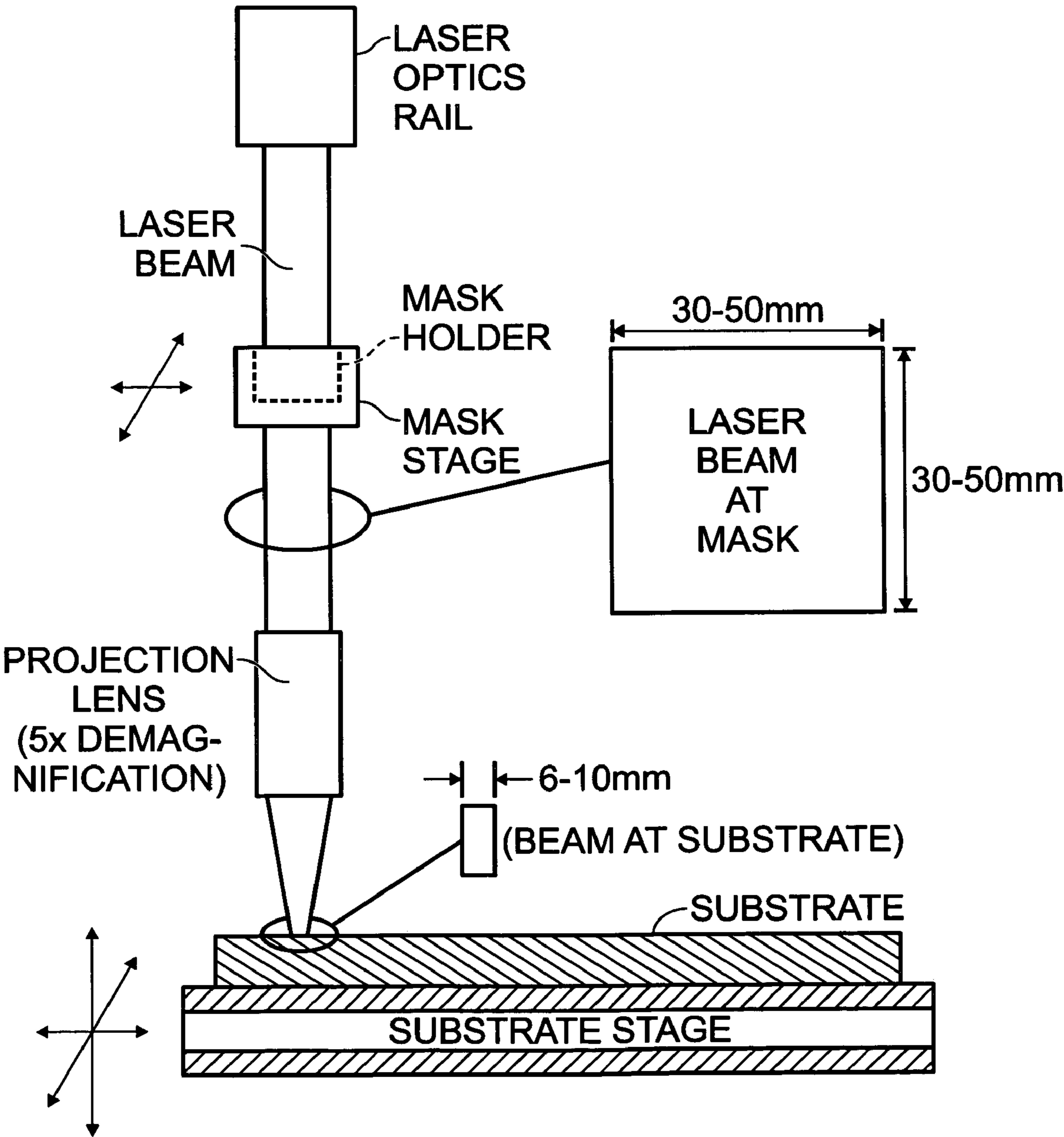
Fig. 3 (PRIOR ART)
