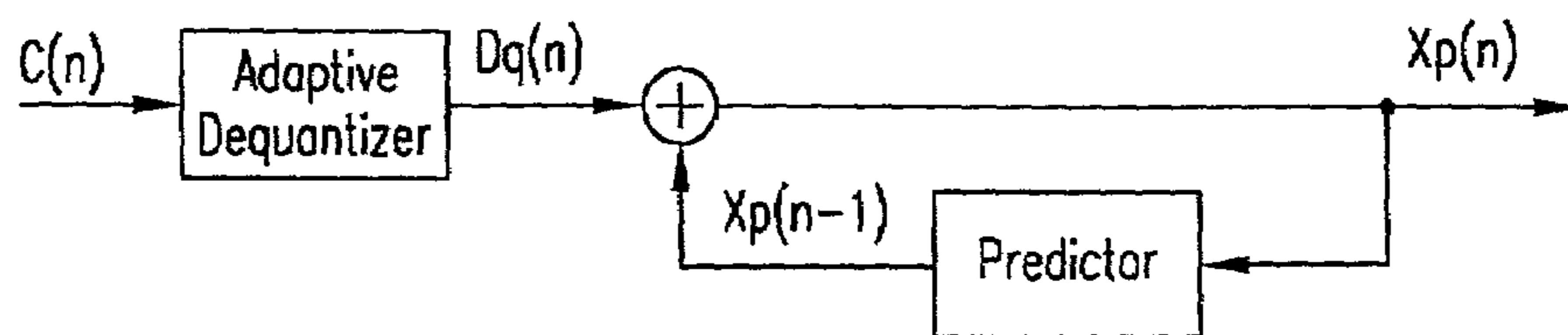
FIG. 1 (PRIOR ART)
