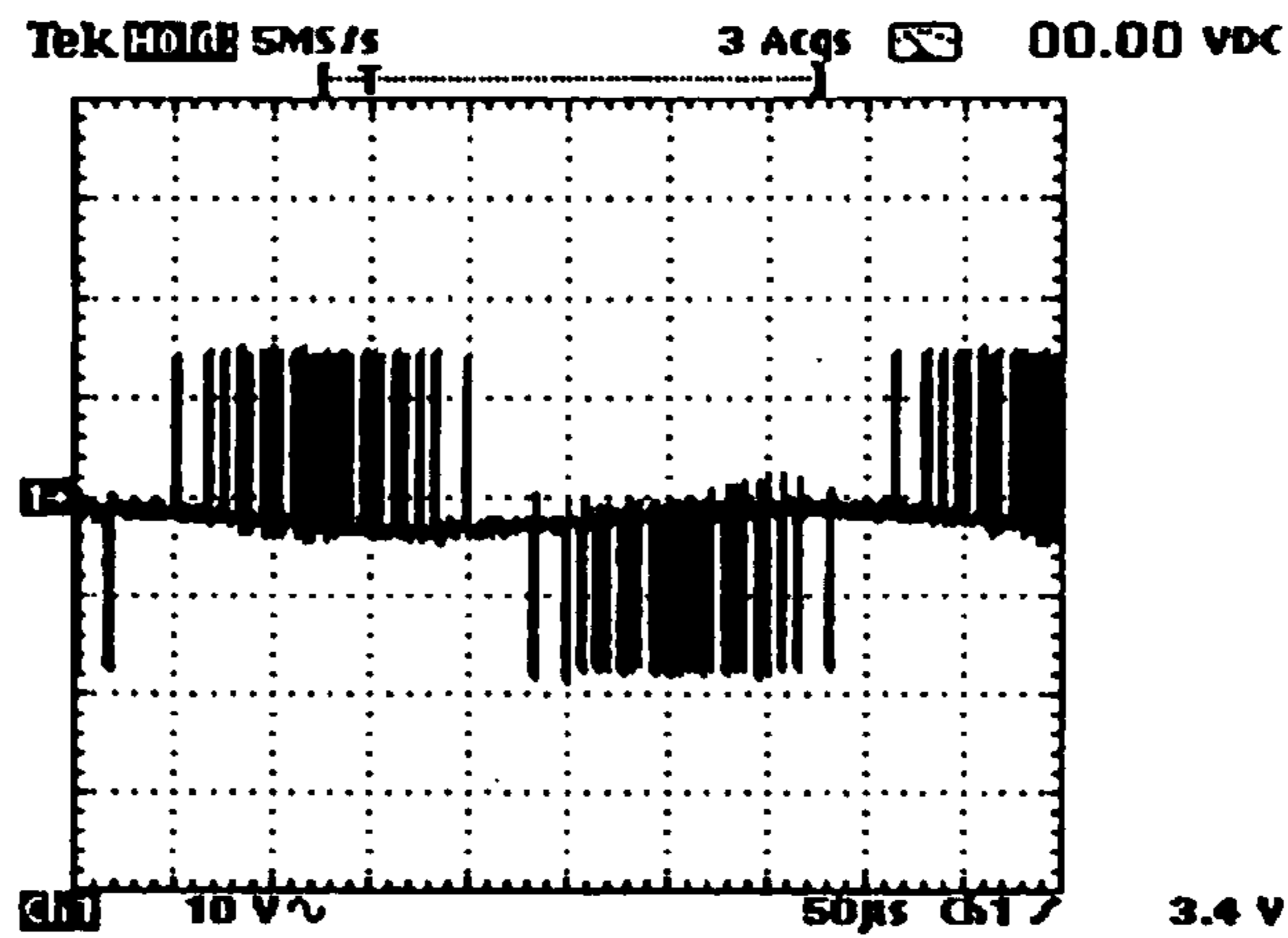
FIG. 3 Waveform in the case where the apparatus is connected to a 500 Ω resistor.
