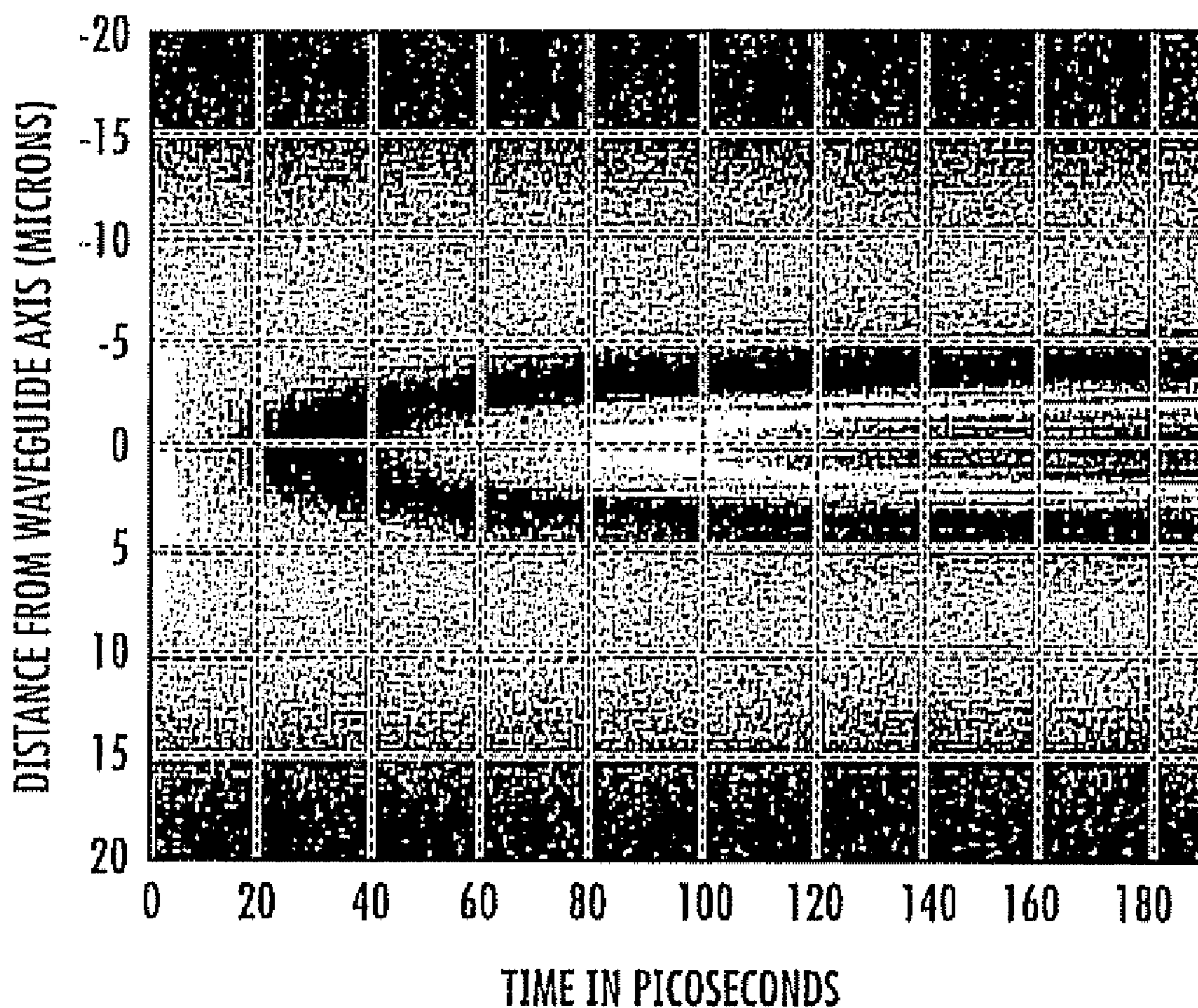
TRANSIENT FIELD PATTERNS IN SOURCE GUIDE
