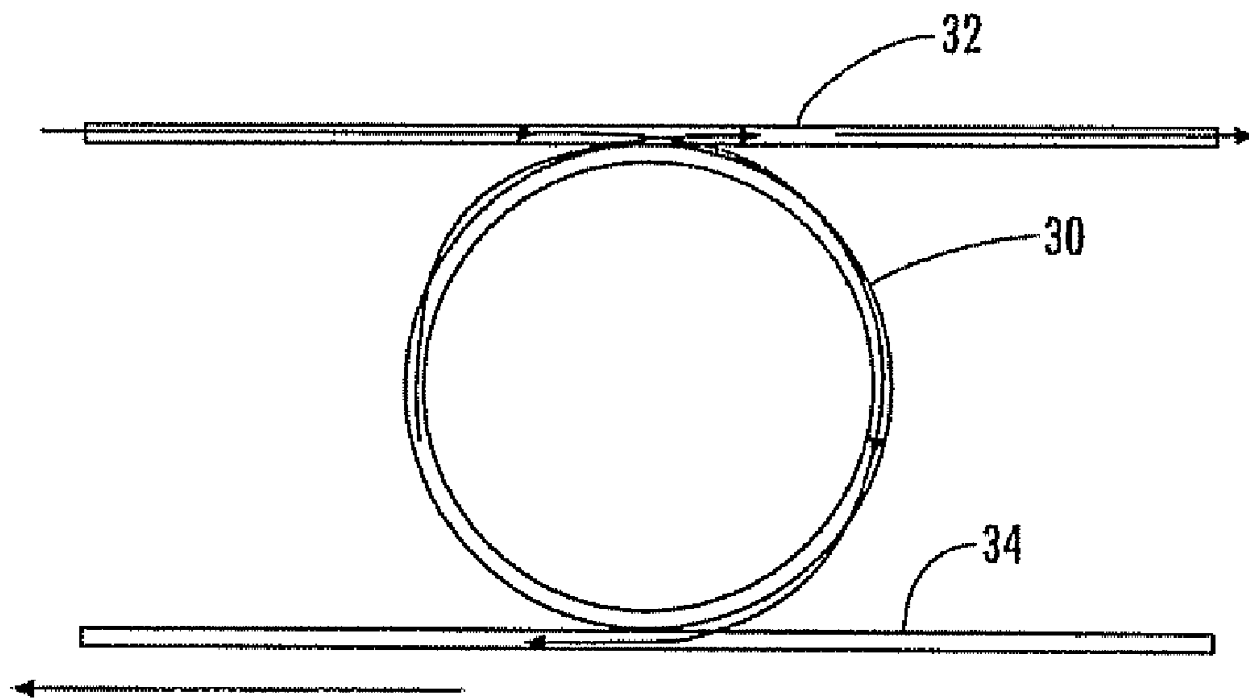
FOUR-PORT RESONANT STRUCTURE
