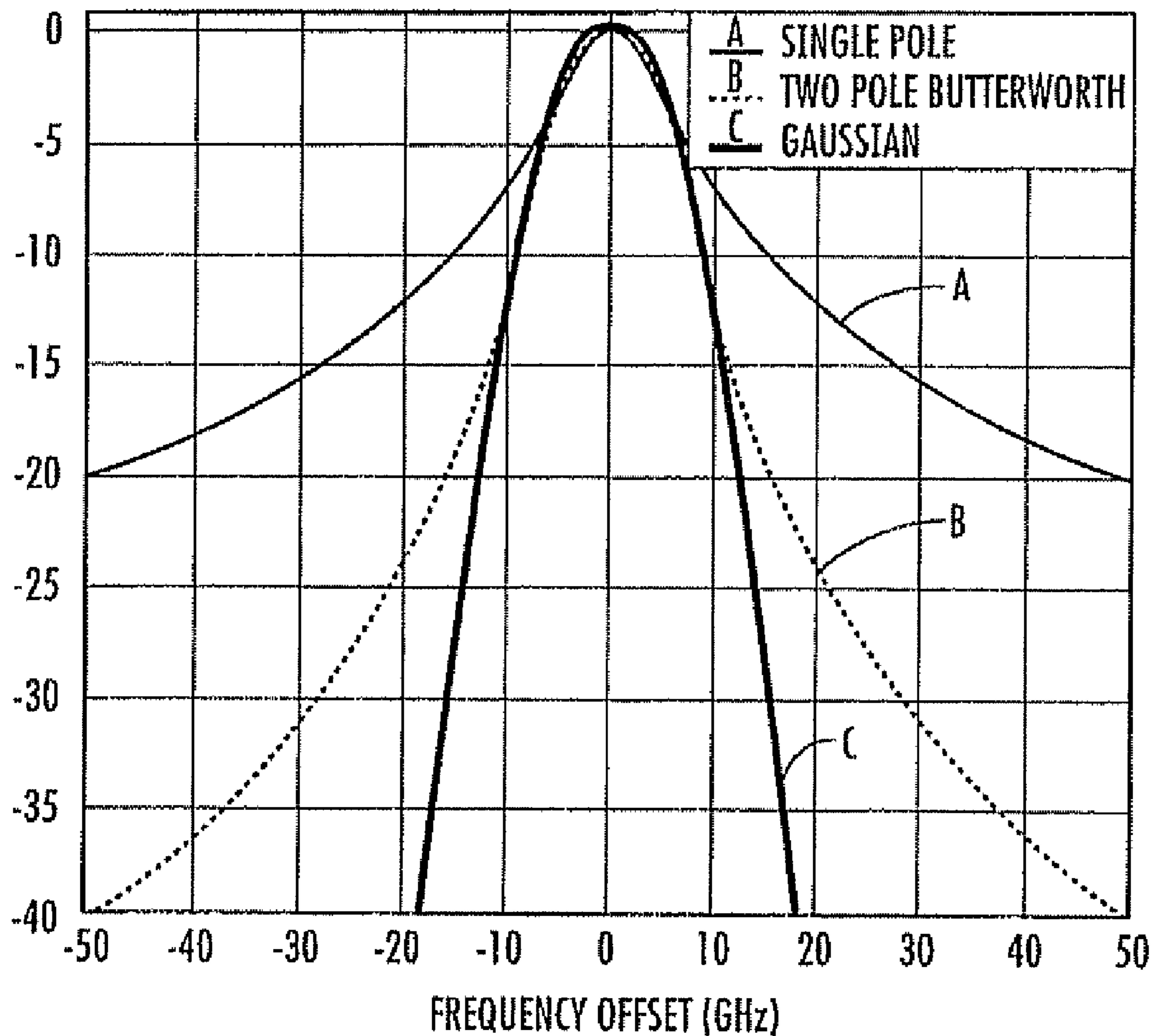
BANDSHAPE FOR GAUSSIAN AND BUTTERWORTH FILTERS
