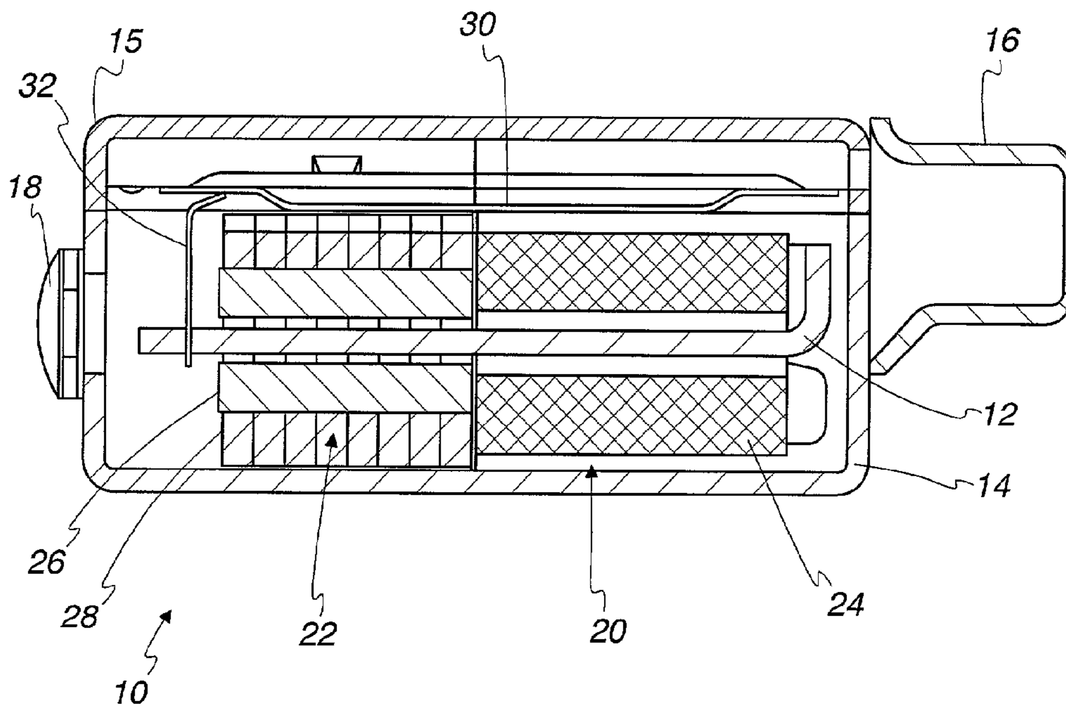
Fig. 1 (Prior Art)
