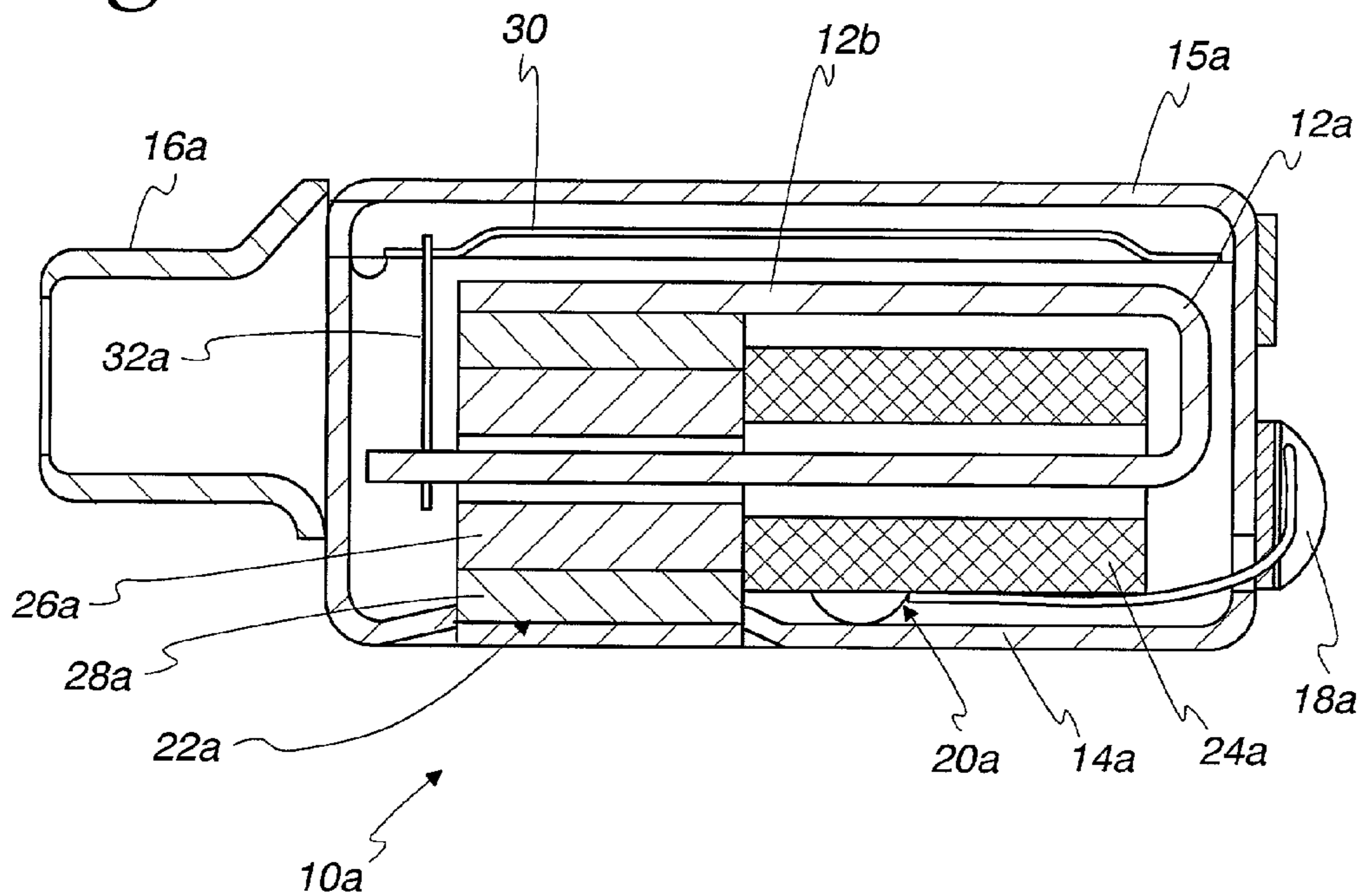
Fig. 2 (Prior Art)
