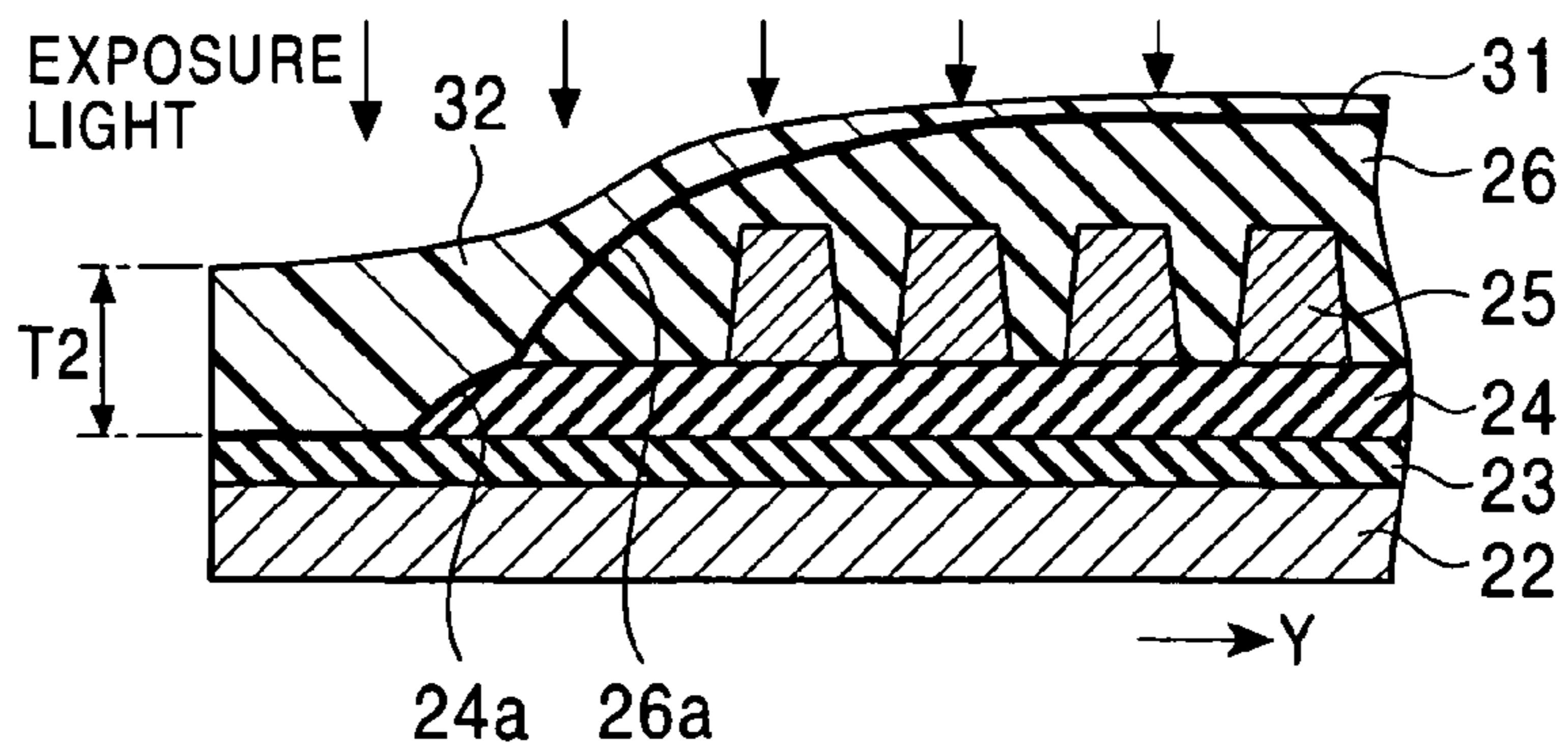
FIG. 10D PRIOR ART
