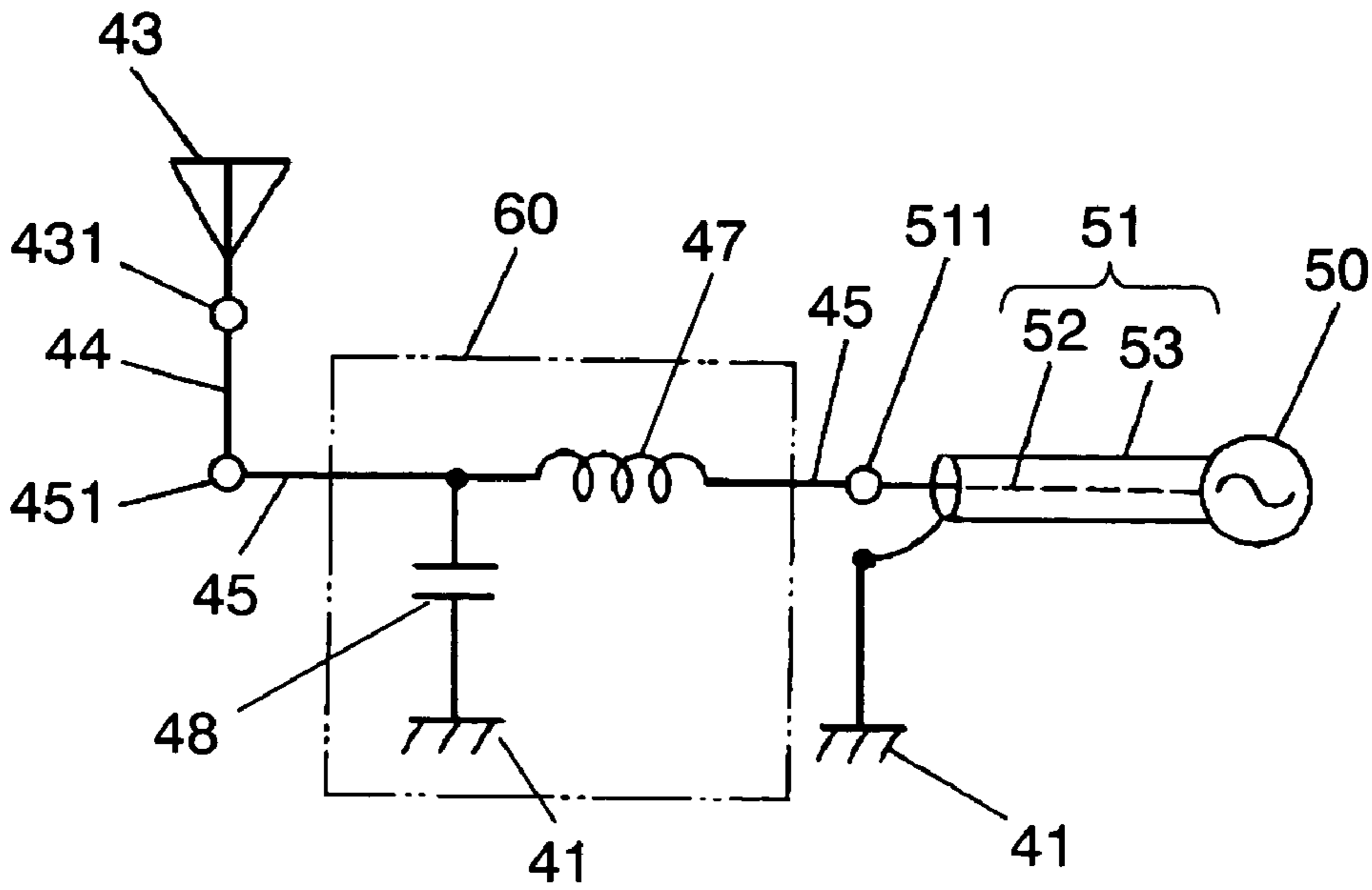
FIG. 6 PRIOR ART
