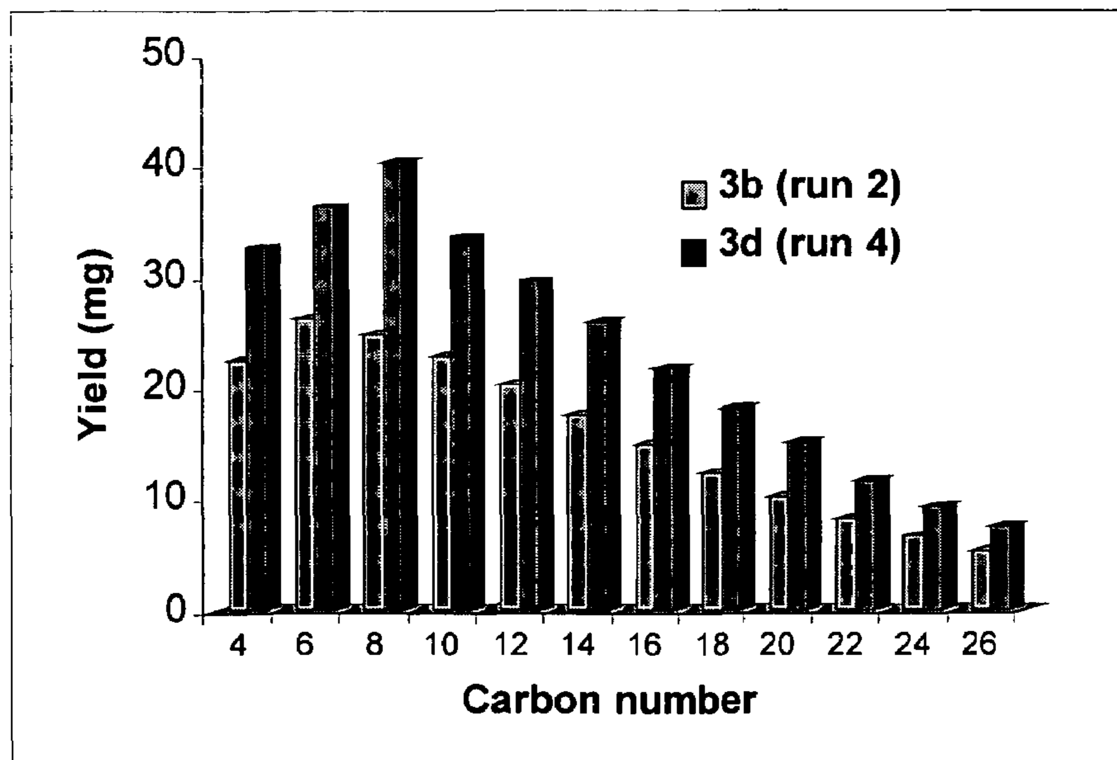
Figure 6 Oligomer distribution of oligomer fractions versus carbon number for runs 2 and 4 using pre-catalysts 3b and 3d , respectively.
