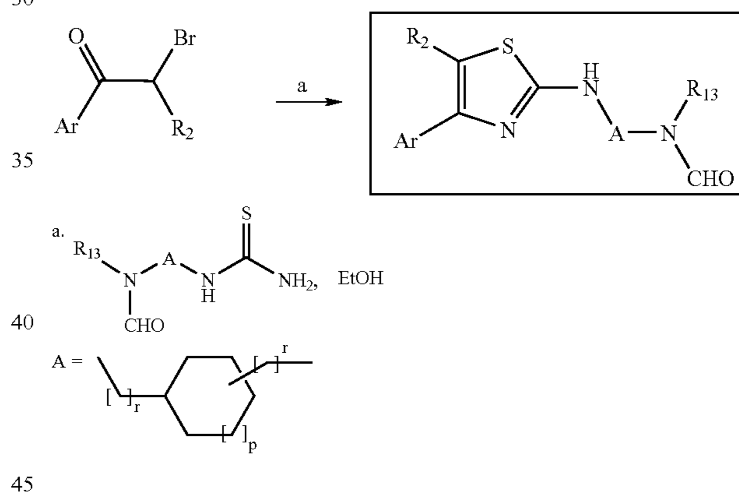
Scheme 8C. Synthesis of Bicycles
