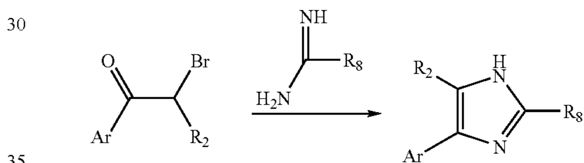
Scheme 9B. Synthesis of Bicycles
