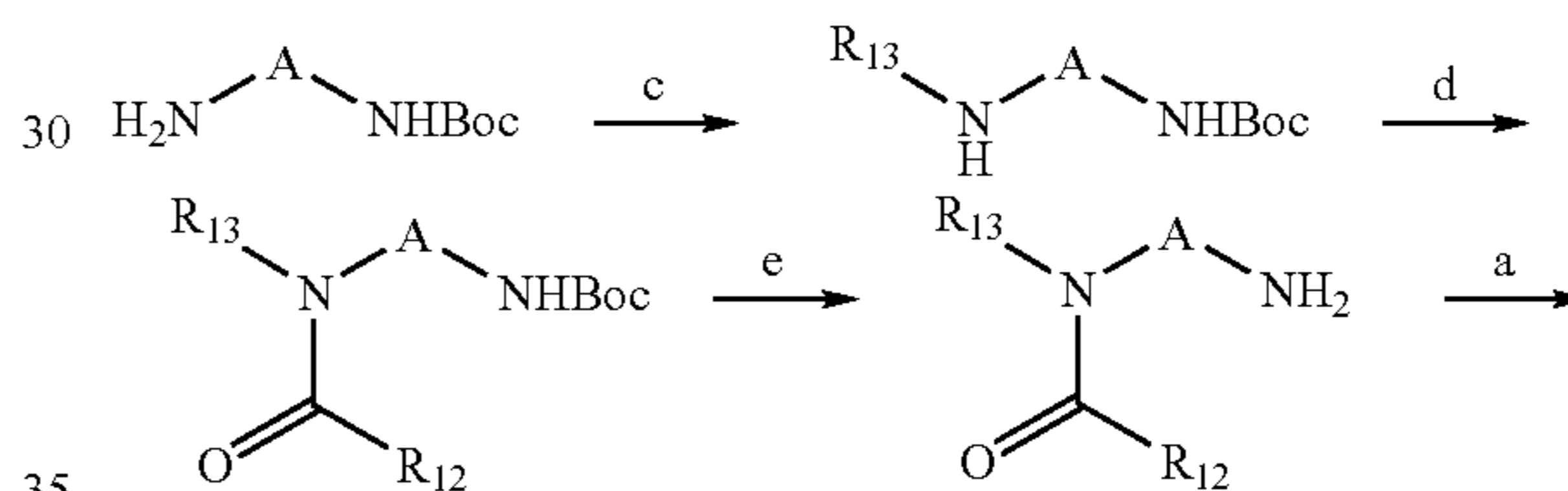
Scheme 6B. Synthesis of Thioureas
