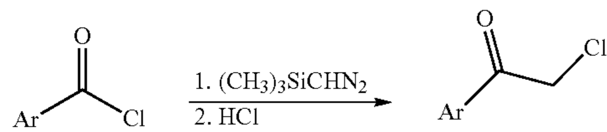
Scheme 7B. Synthesis of Chloroketones
