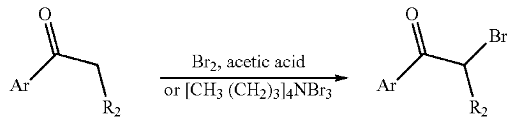
Scheme 7A. Synthesis of Bromoketones
