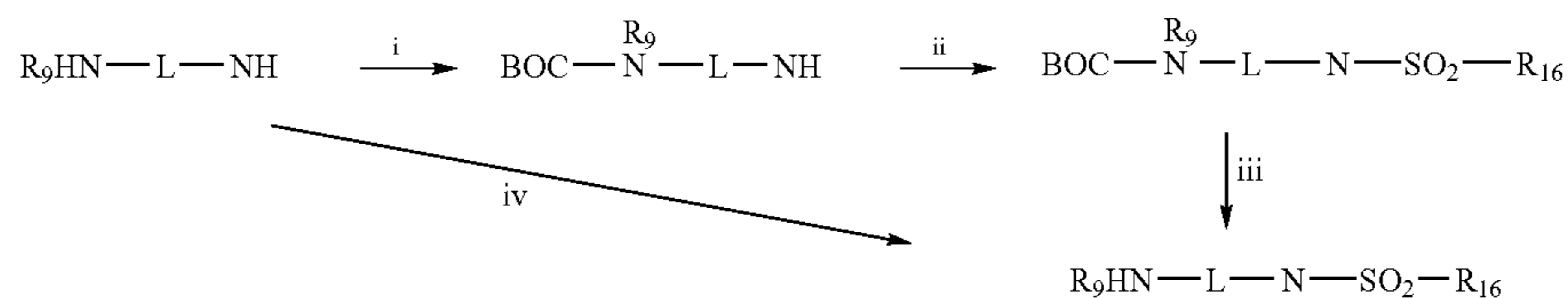
Scheme 1D. Synthesis of Side Chains
