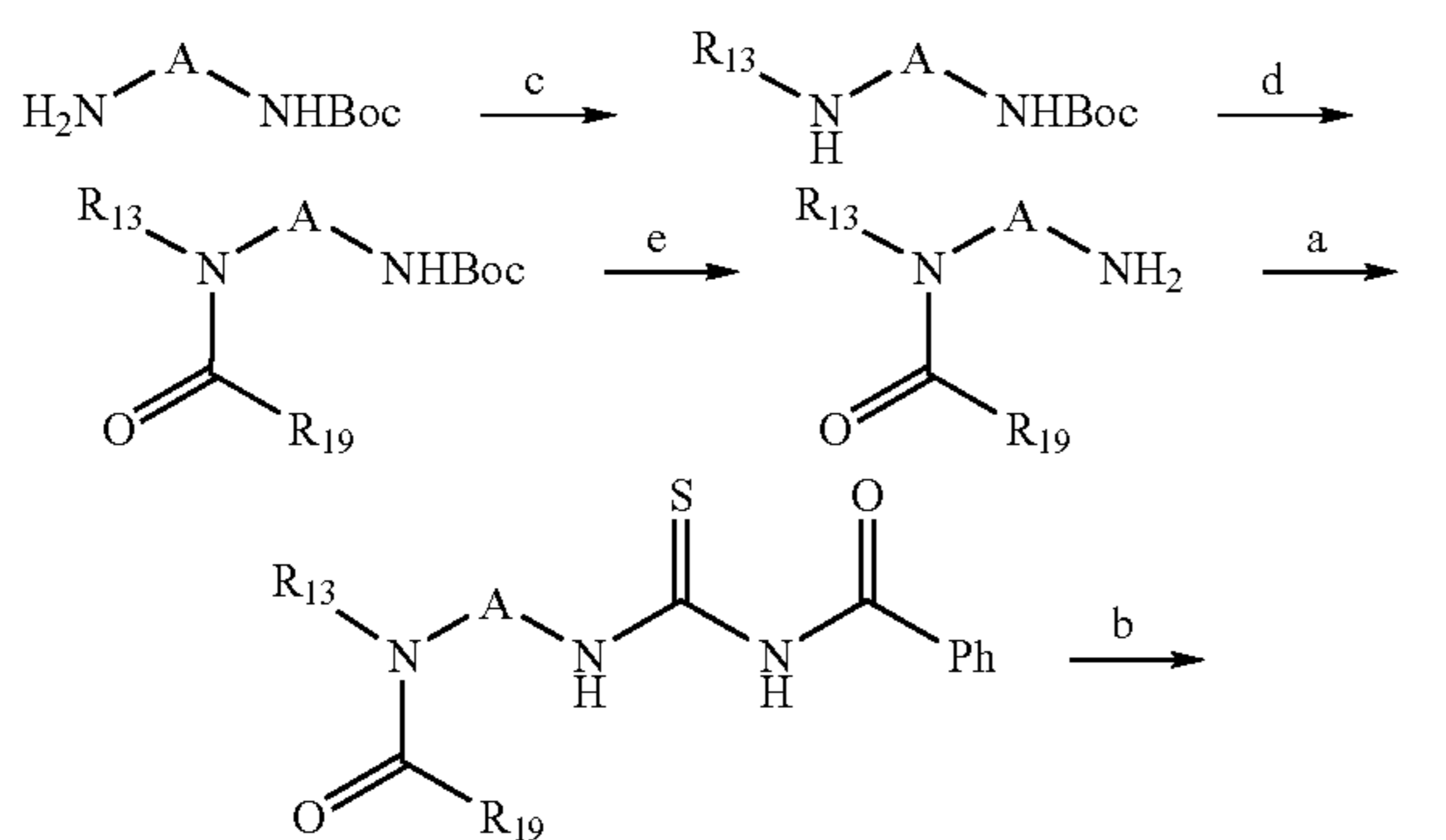
Scheme 11C. Synthesis of Thioureas
