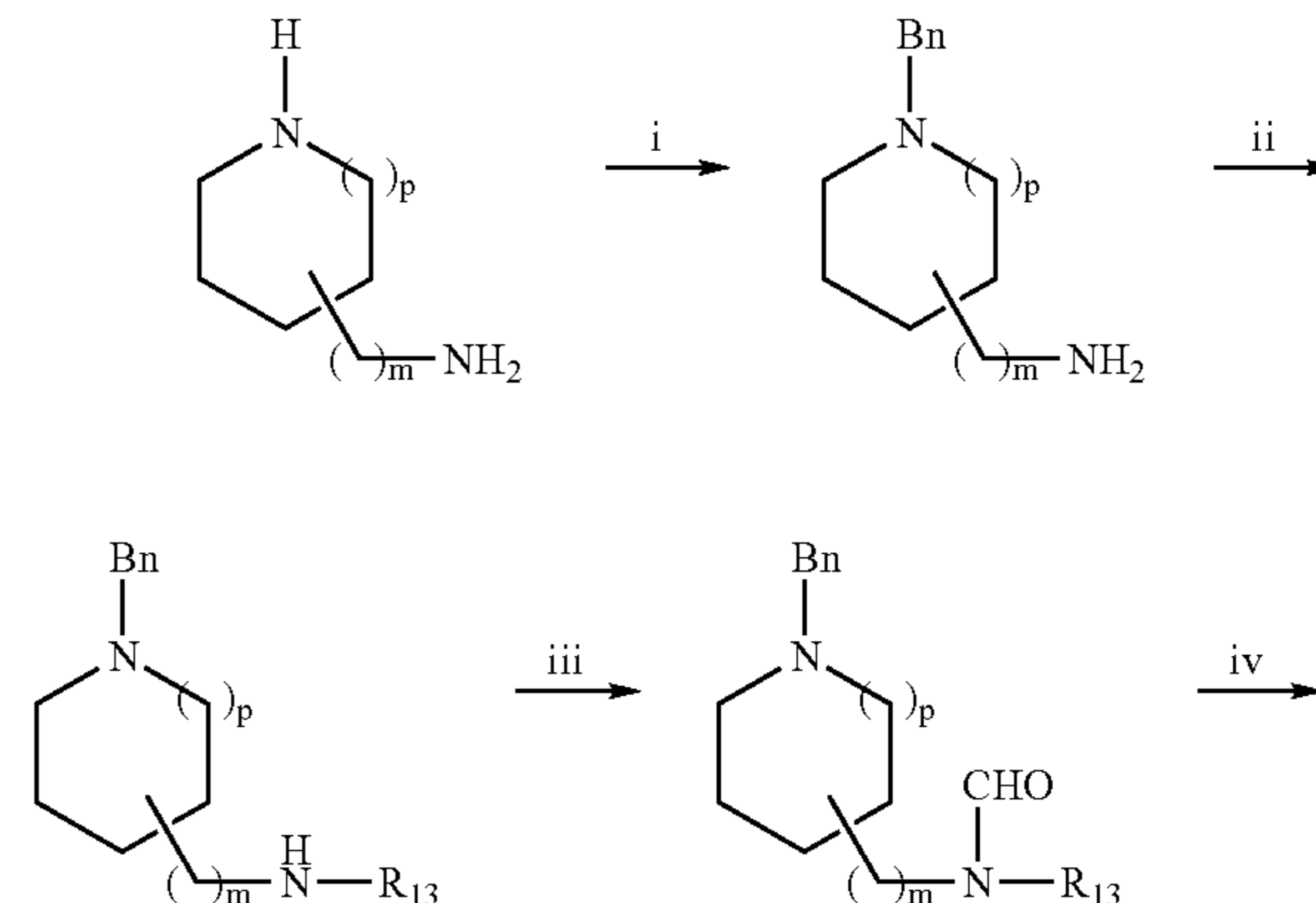
Scheme 1E. Synthesis of Side Chains
