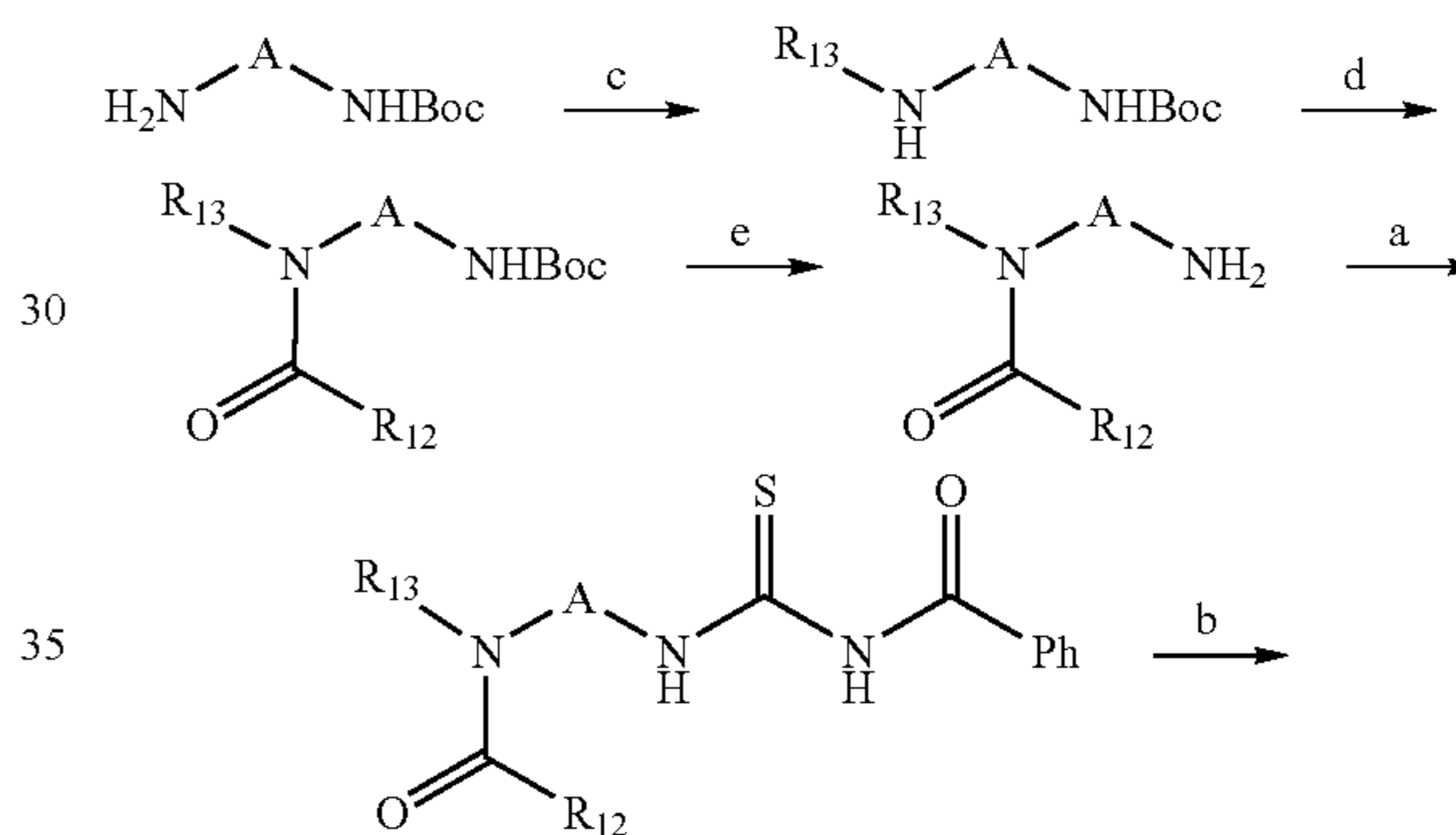
Scheme 11D. Synthesis of Thioureas
