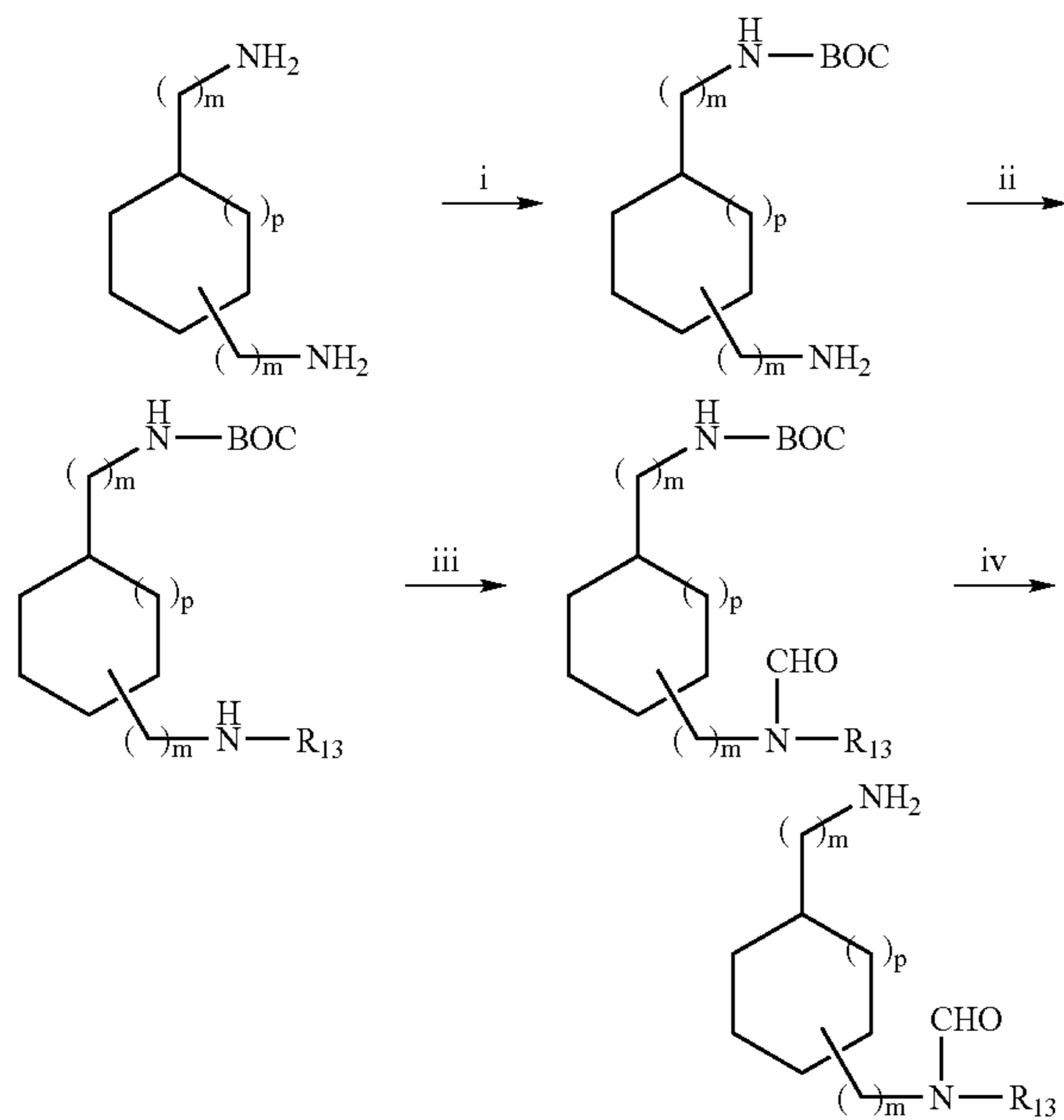
Scheme 1E. Synthesis of Side Chains
