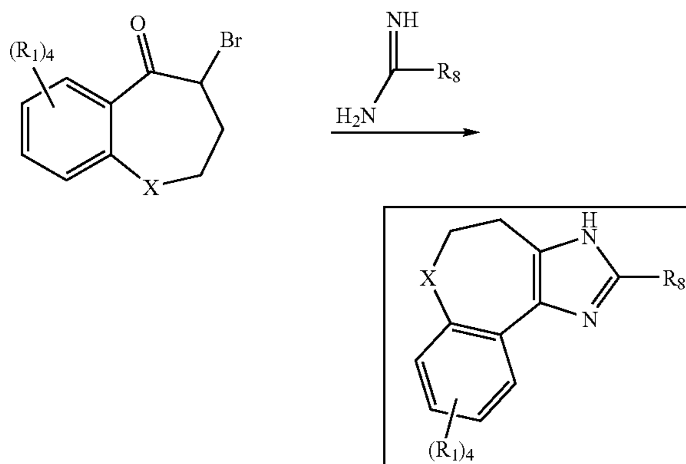
Scheme 14B. Synthesis of Tricycles
