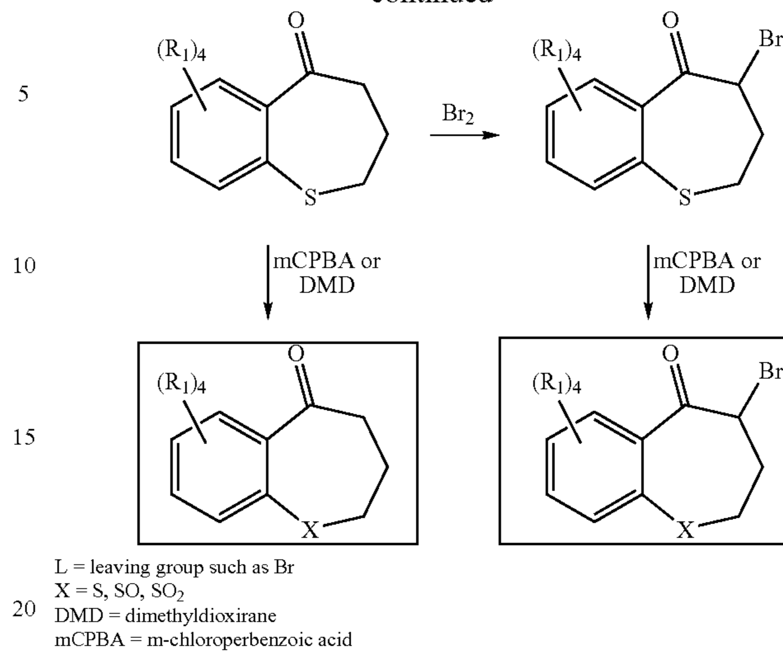
Scheme 13A. Synthesis of the Tricycles
