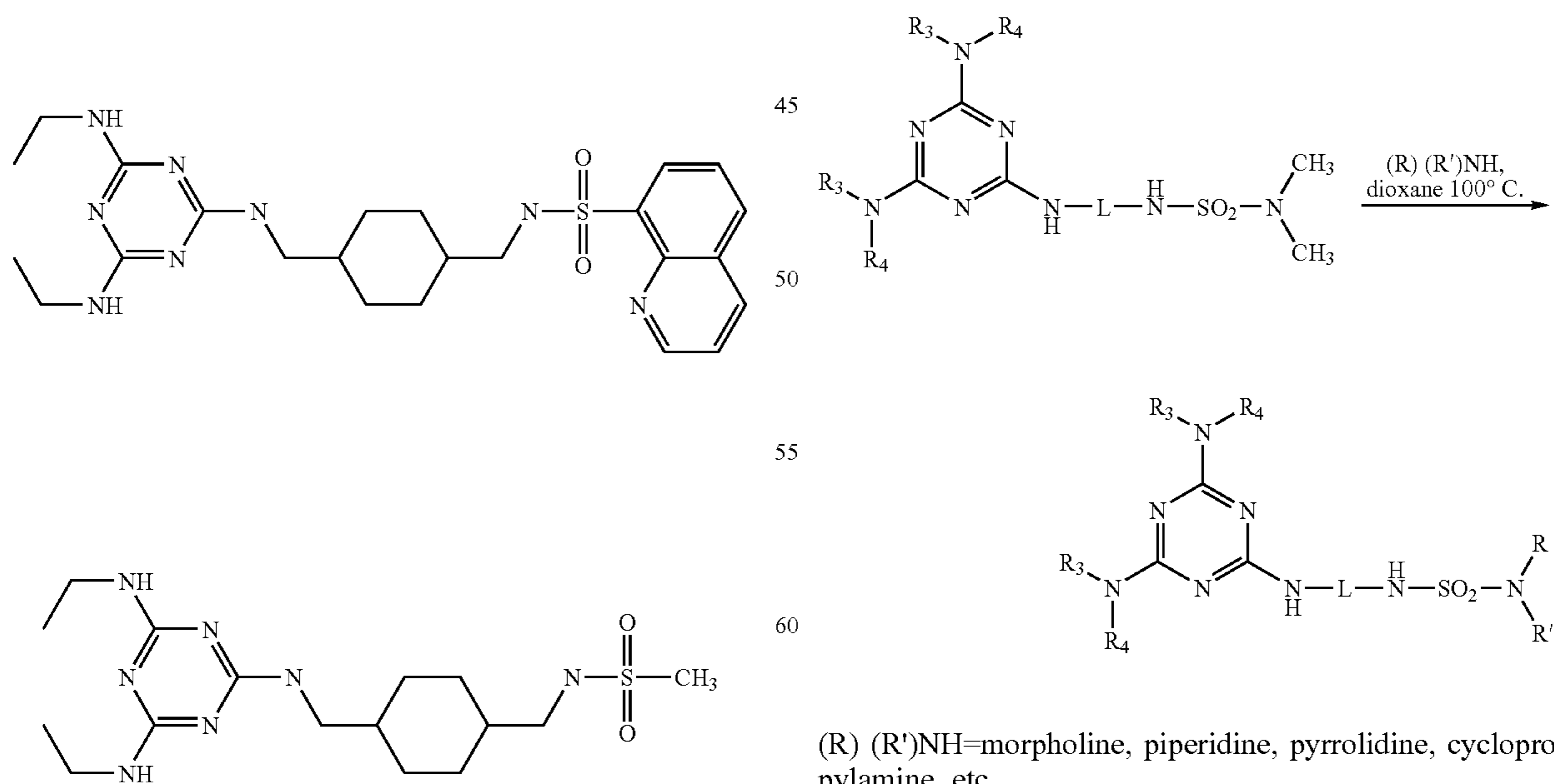
Scheme 4A. Synthesis of Triazine Derivatives
