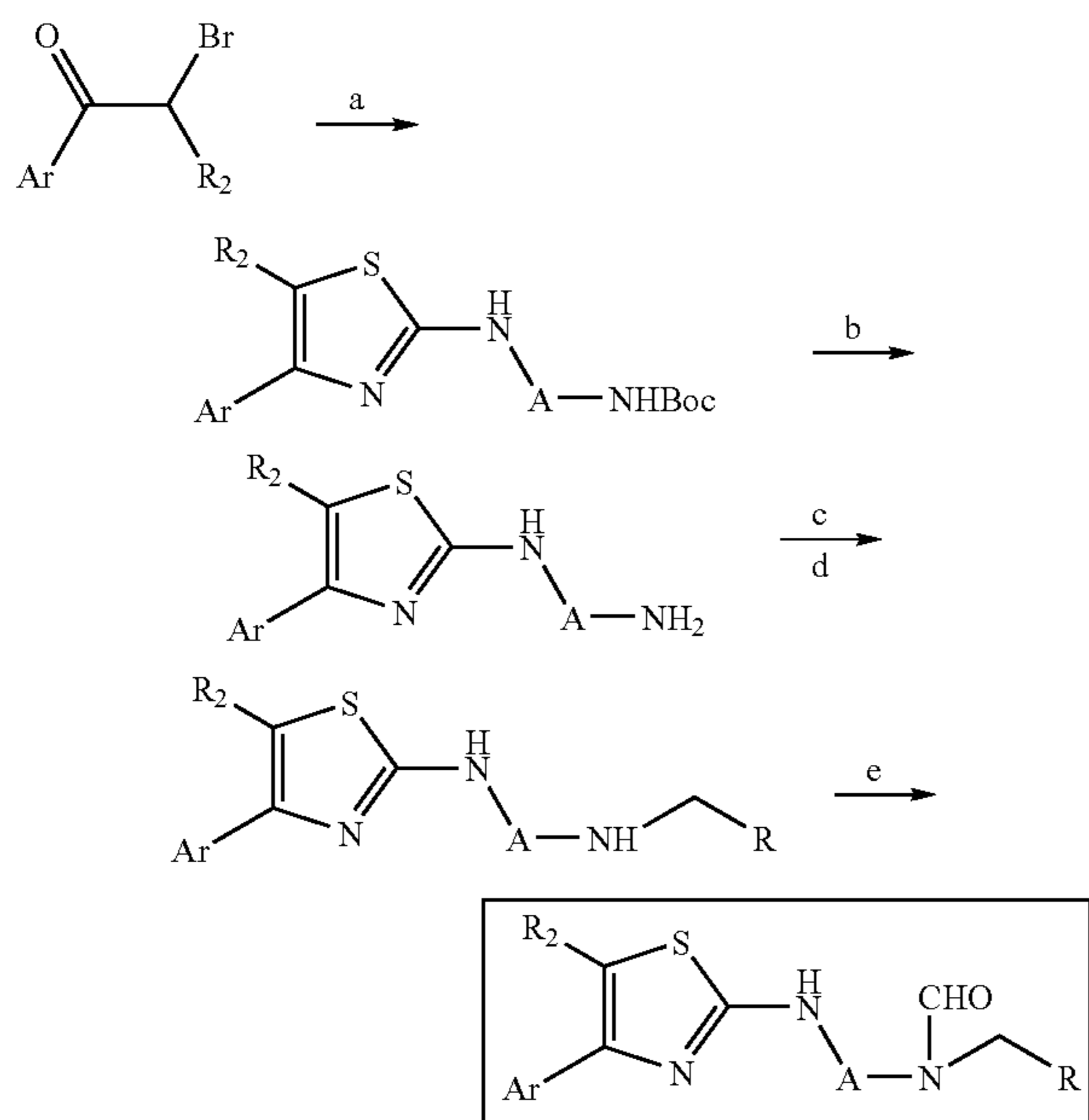
Scheme 8E. Synthesis of Bicycles
