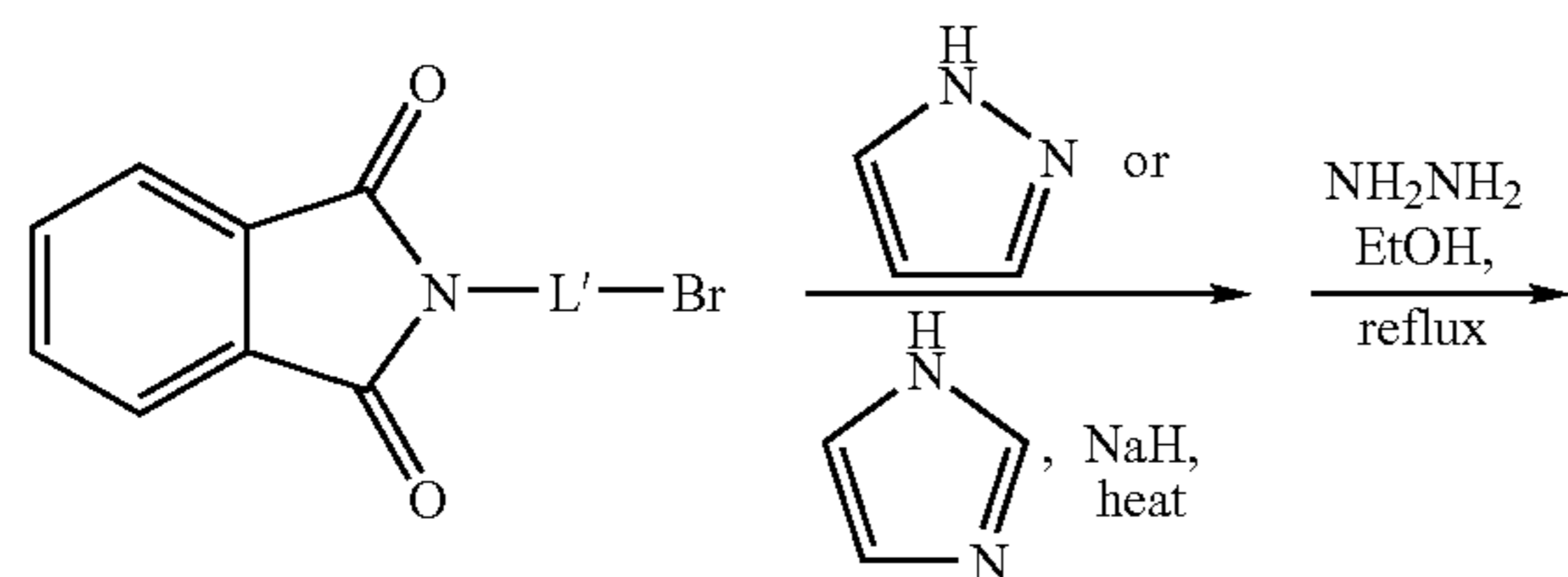
Scheme 1G. Synthesis of Side Chains
