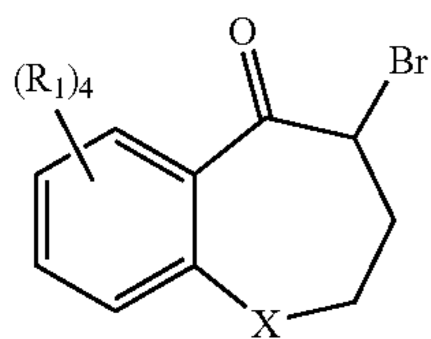
Scheme 13C. Synthesis of the Tricycles
