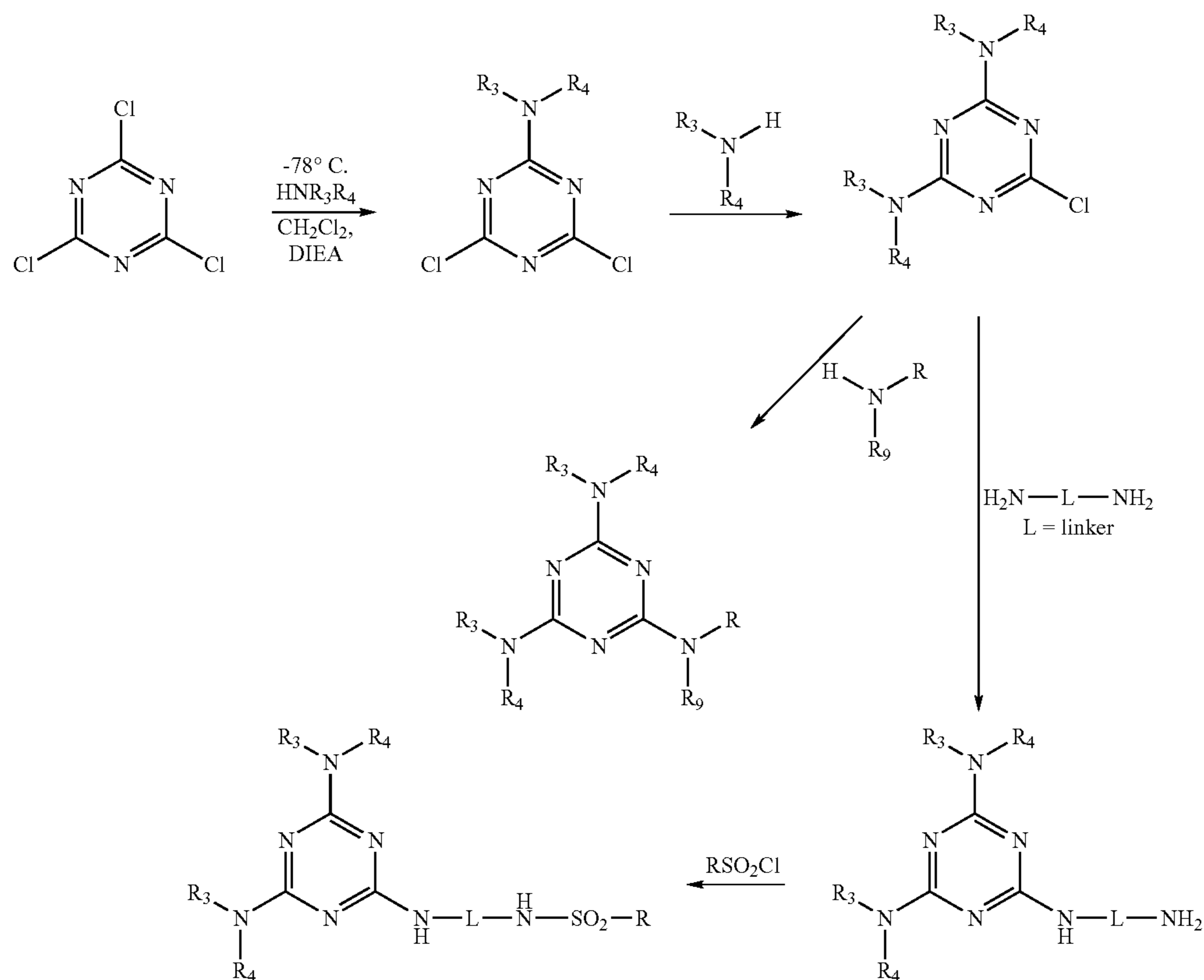
Scheme 3. Synthesis of Triaminotriazines
