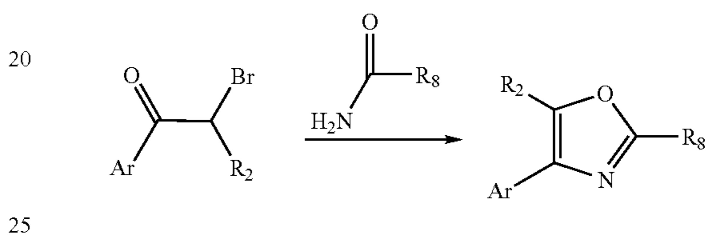
Scheme 9A. Synthesis of Bicycles
