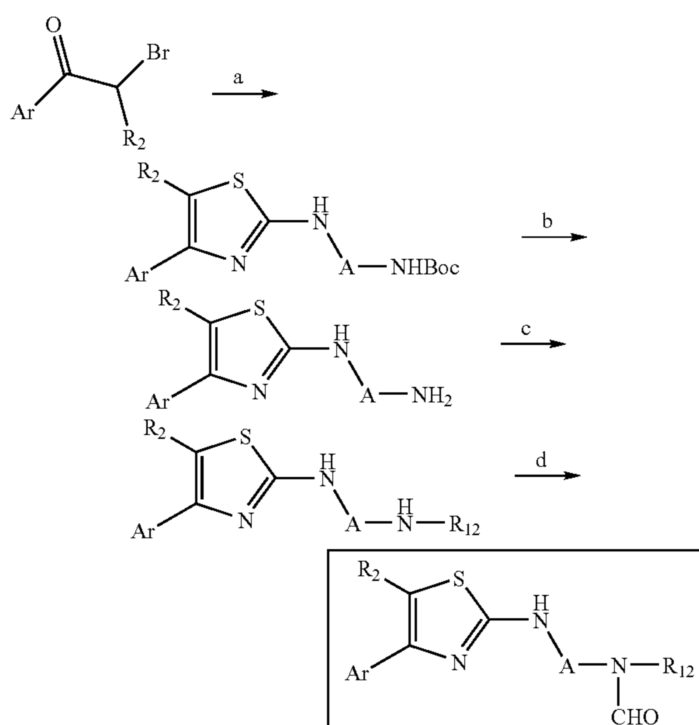
Scheme 8F. Synthesis of Bicycles
