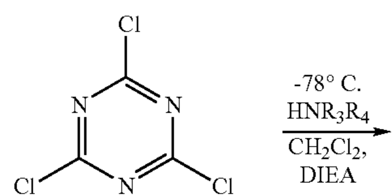
Scheme 2. Synthesis of Triaminotriazines
