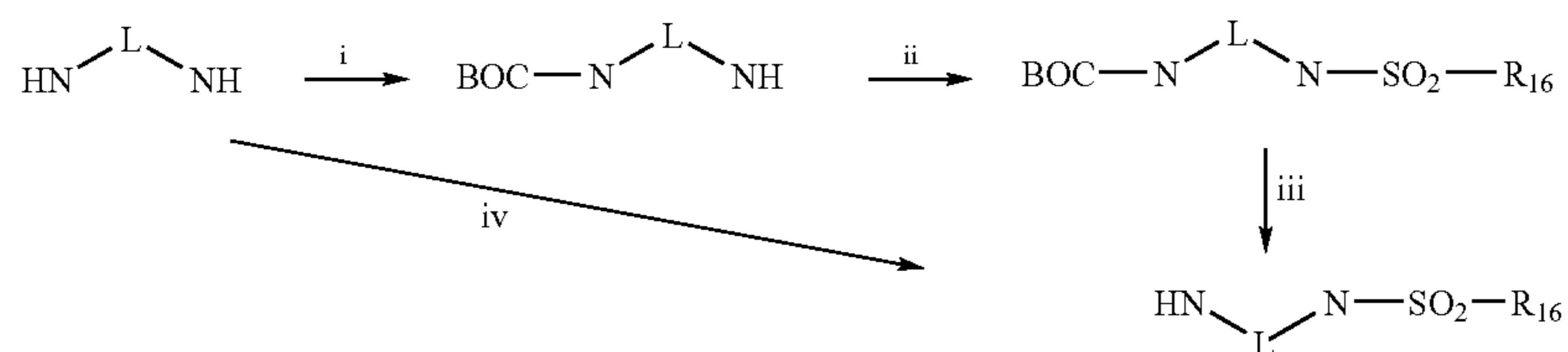
Scheme 1B. Synthesis of Side Chains
