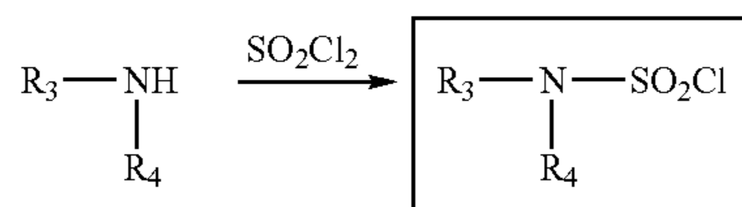
Scheme 8A. Synthesis of Bicycles
