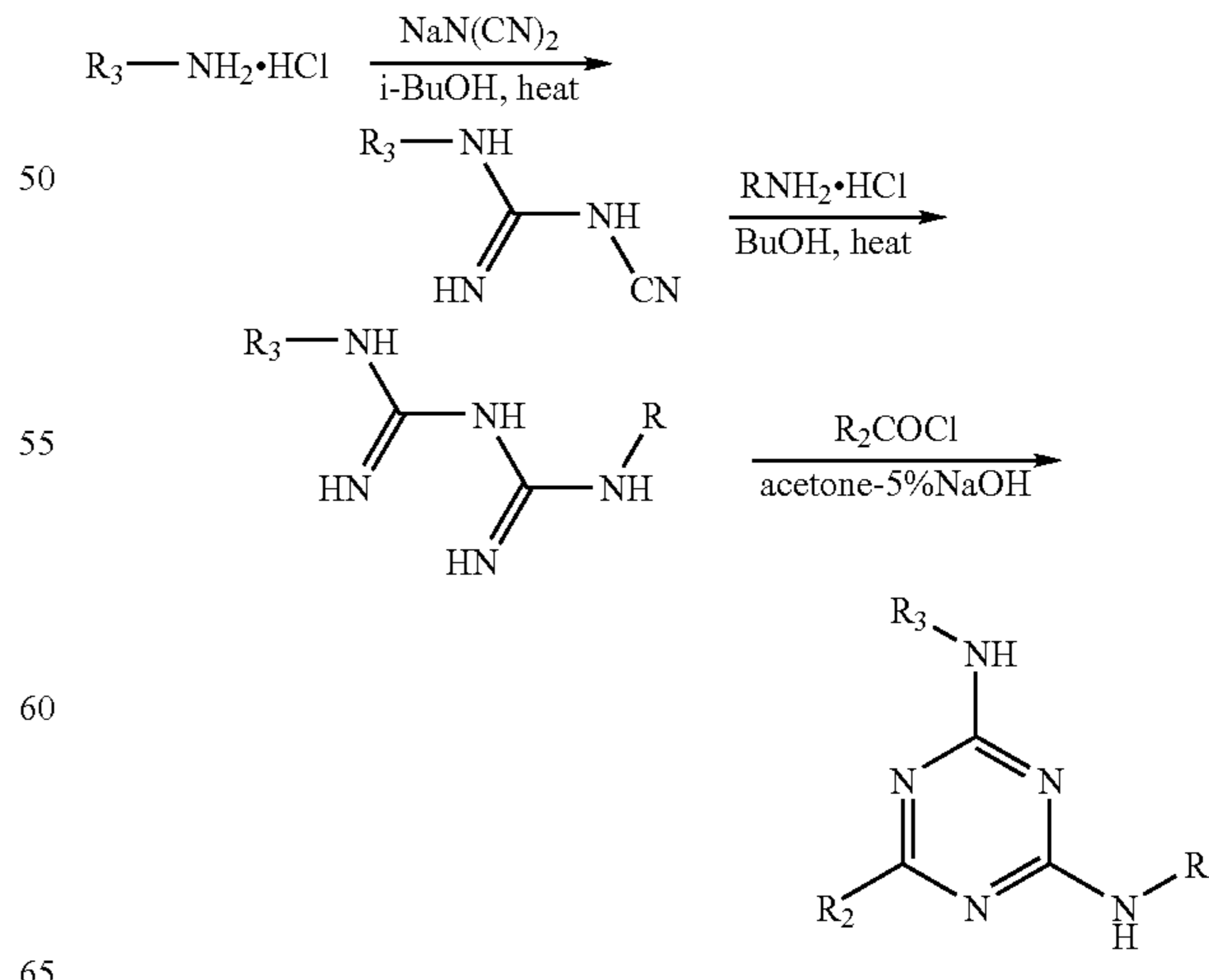
Scheme 5. Synthesis of Diamino-1,3,5-triazines
