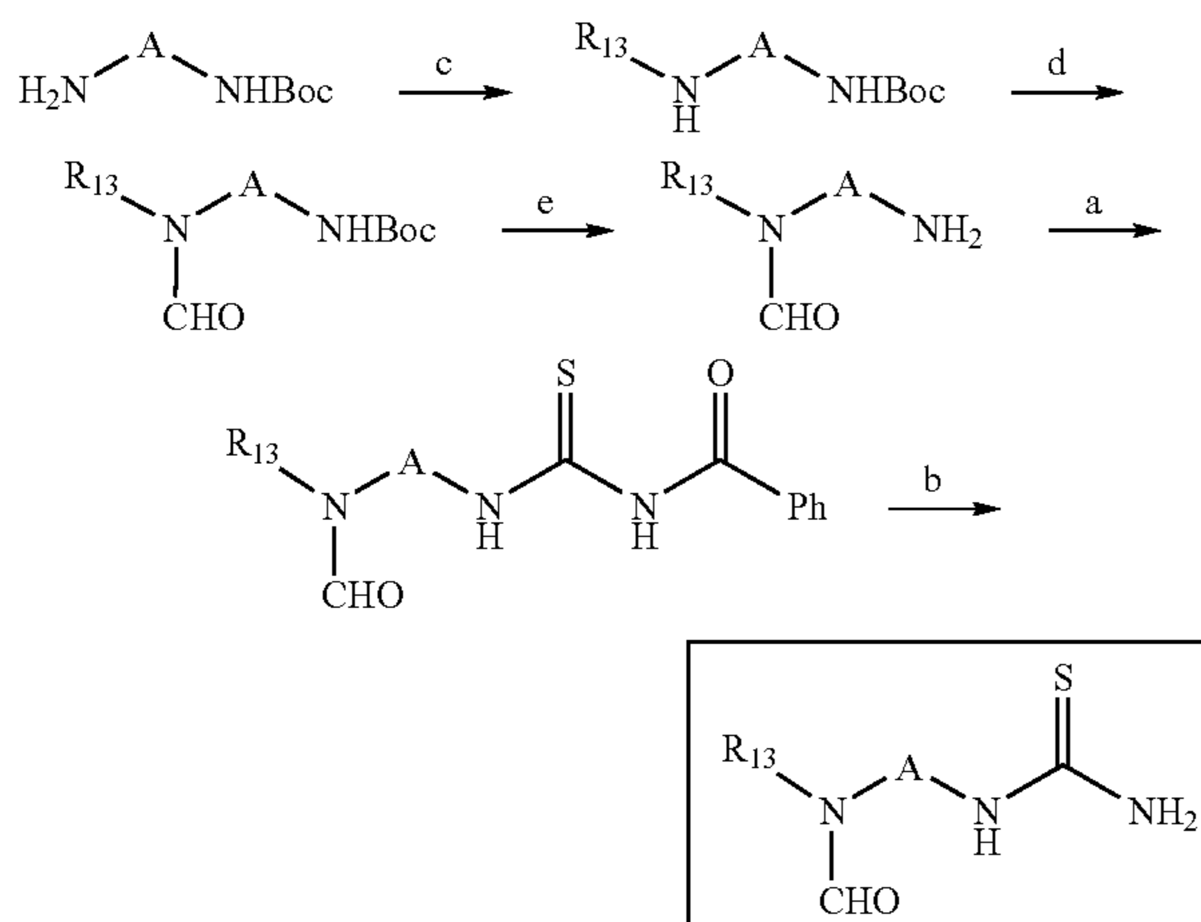
Scheme 11B. Synthesis of Thioureas
