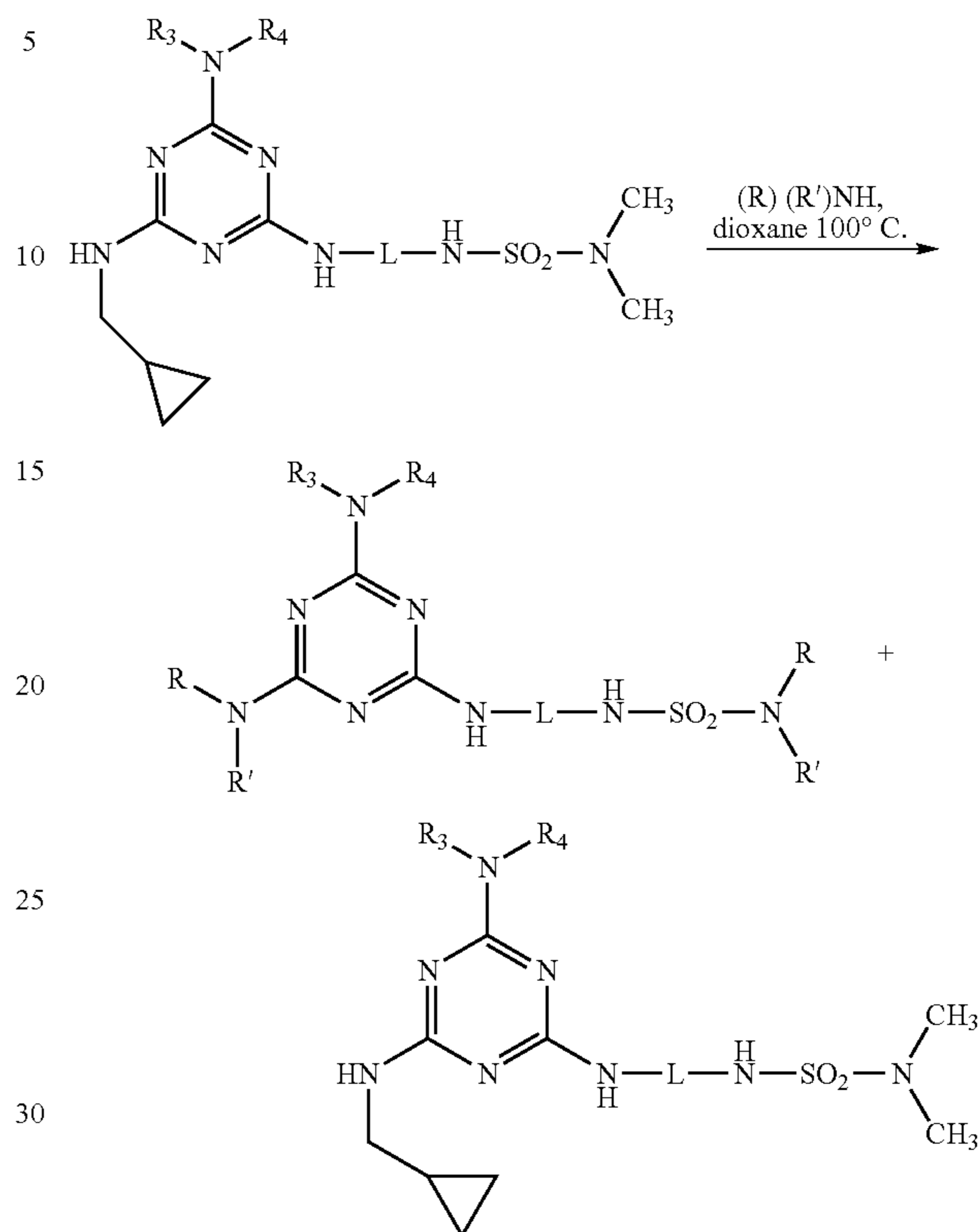
Scheme 4D. Synthesis of Triazine Derivatives
