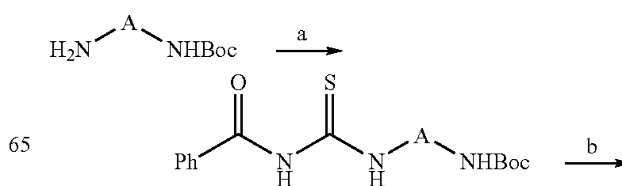
Scheme 11A. Synthesis of Thioureas
