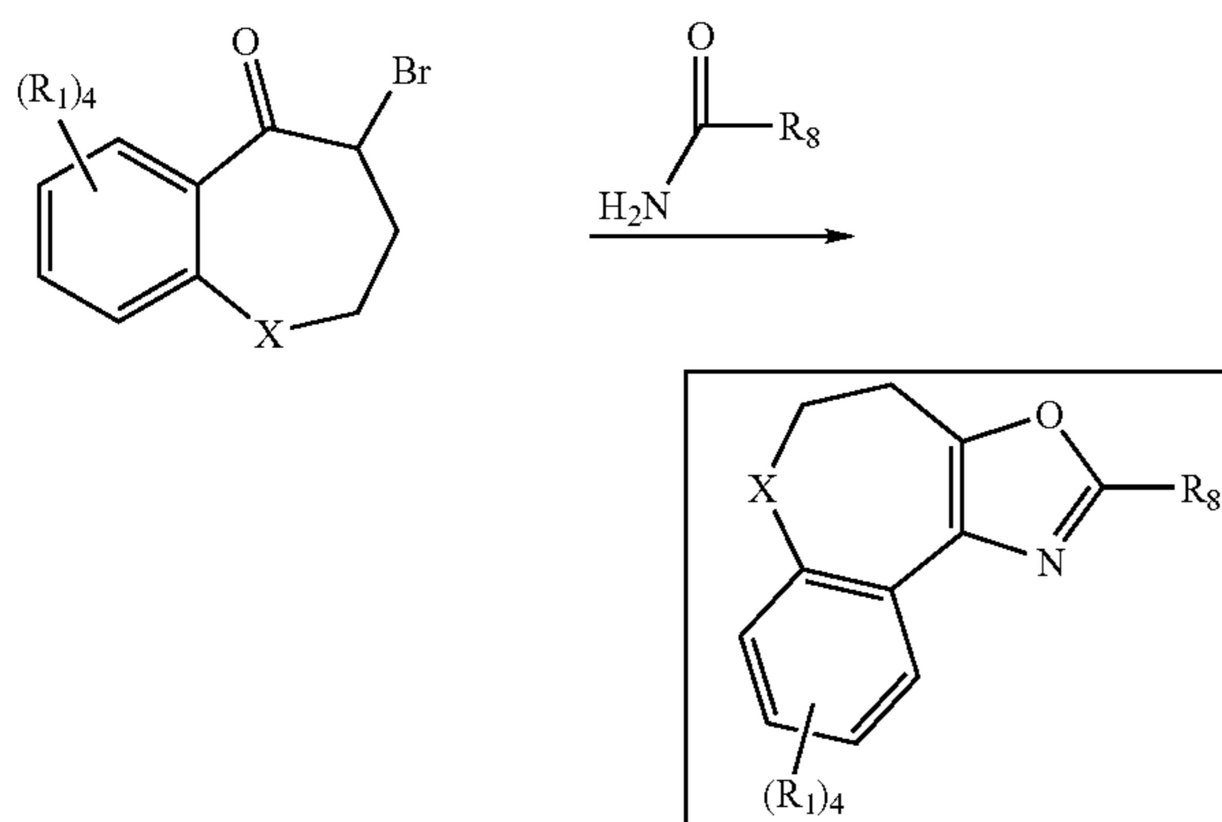
Scheme 14A. Synthesis of Tricycles
