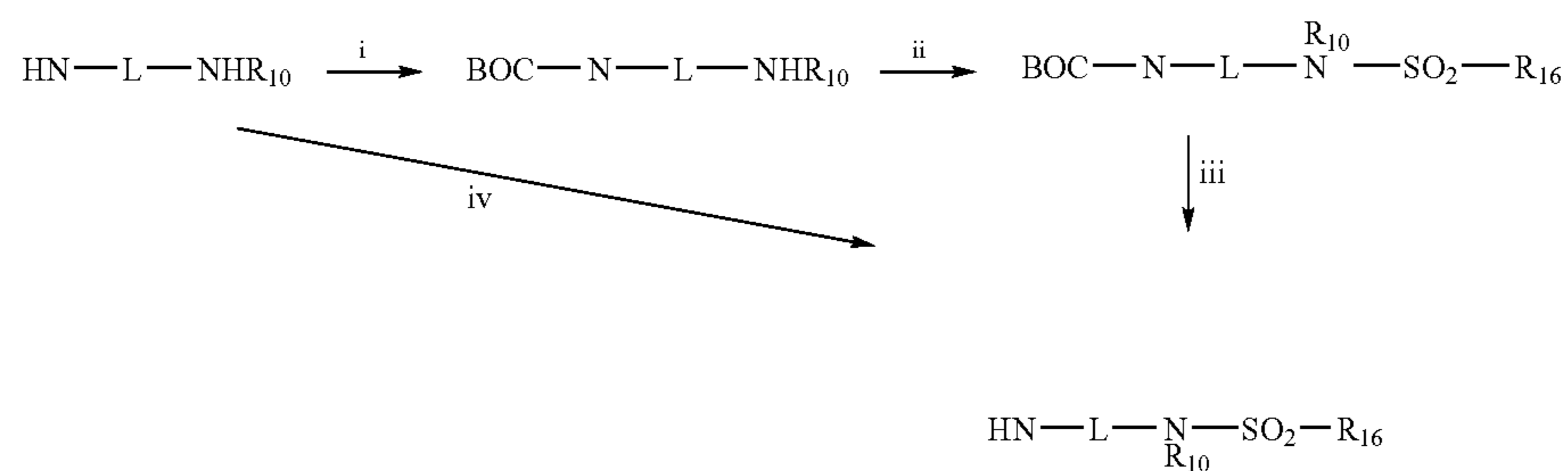
Scheme 1C. Synthesis of Side Chains
