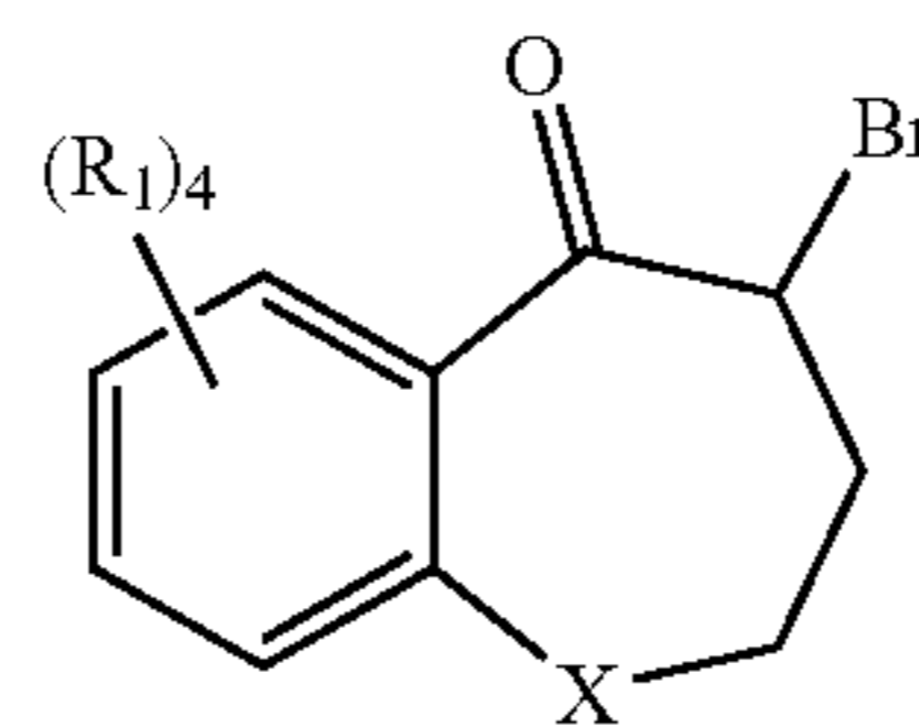
Scheme 13D. Synthesis of the Tricycles
