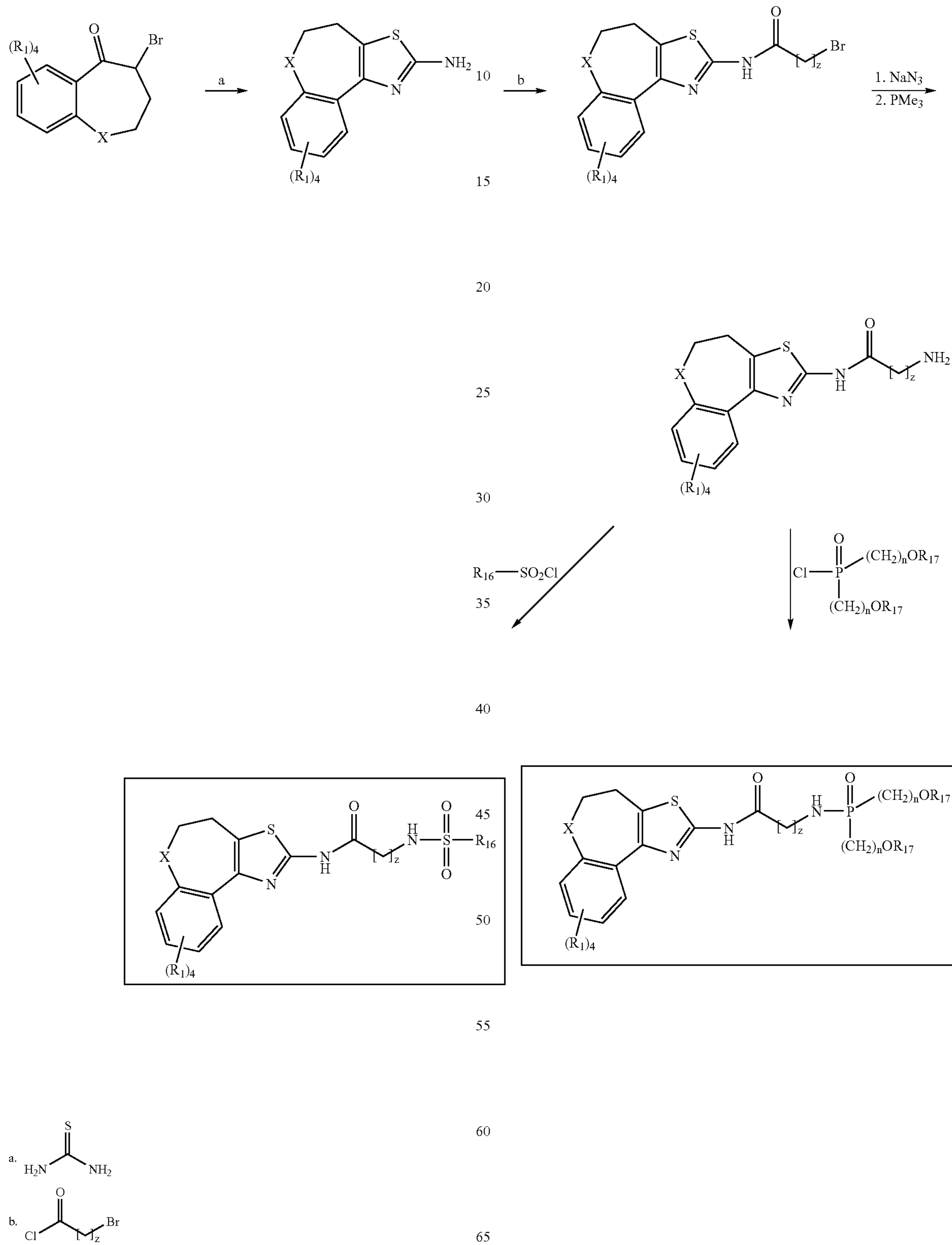
Scheme 13E. Synthesis of the Tricycles
