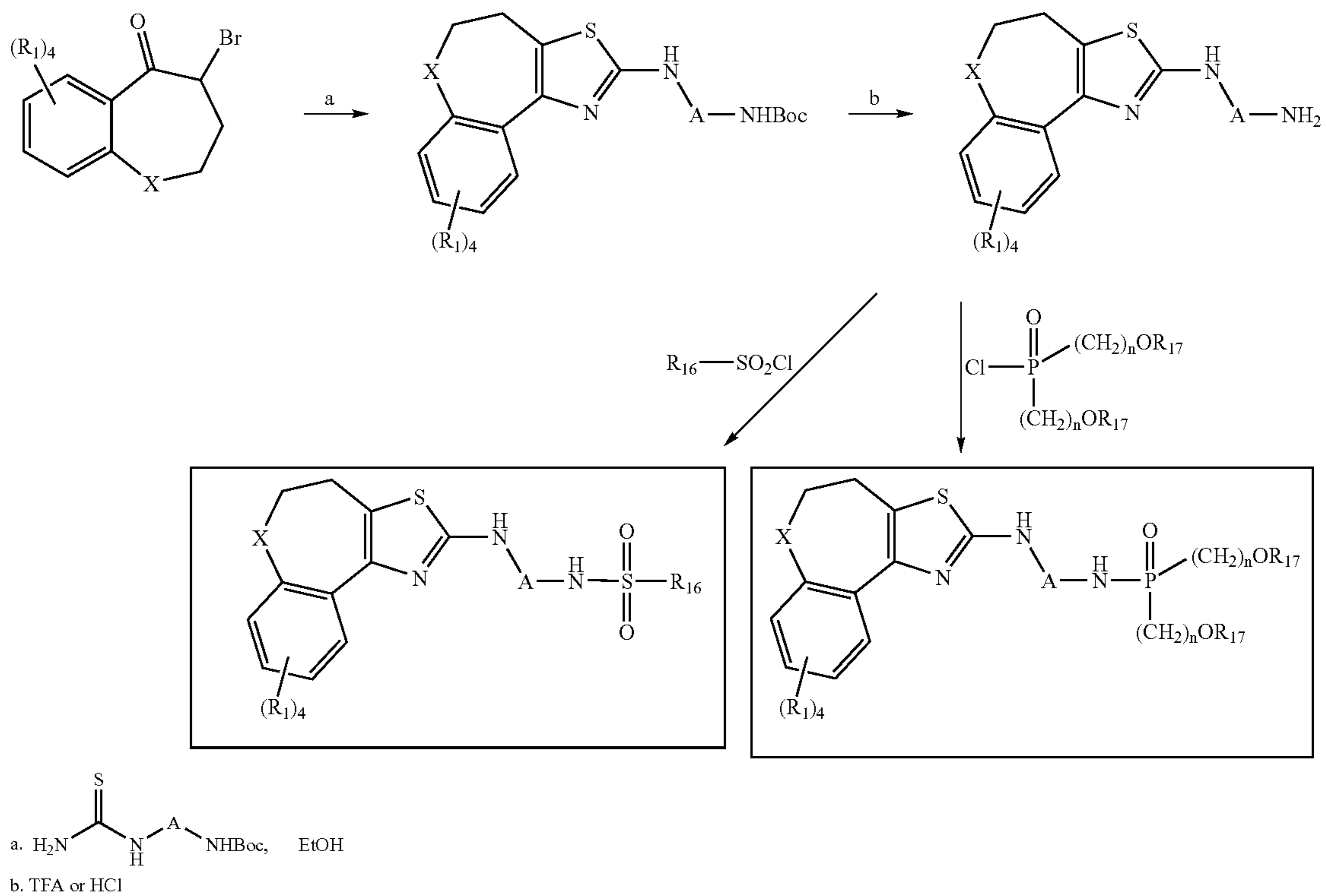
Scheme 13A. Synthesis of the Tricycles
