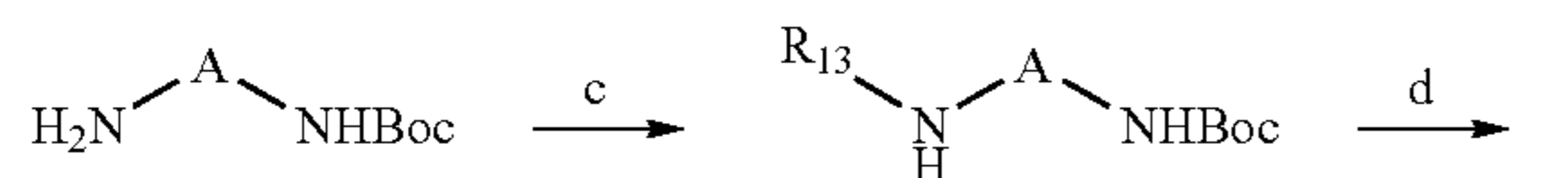
Scheme 6B. Synthesis of Thioureas
