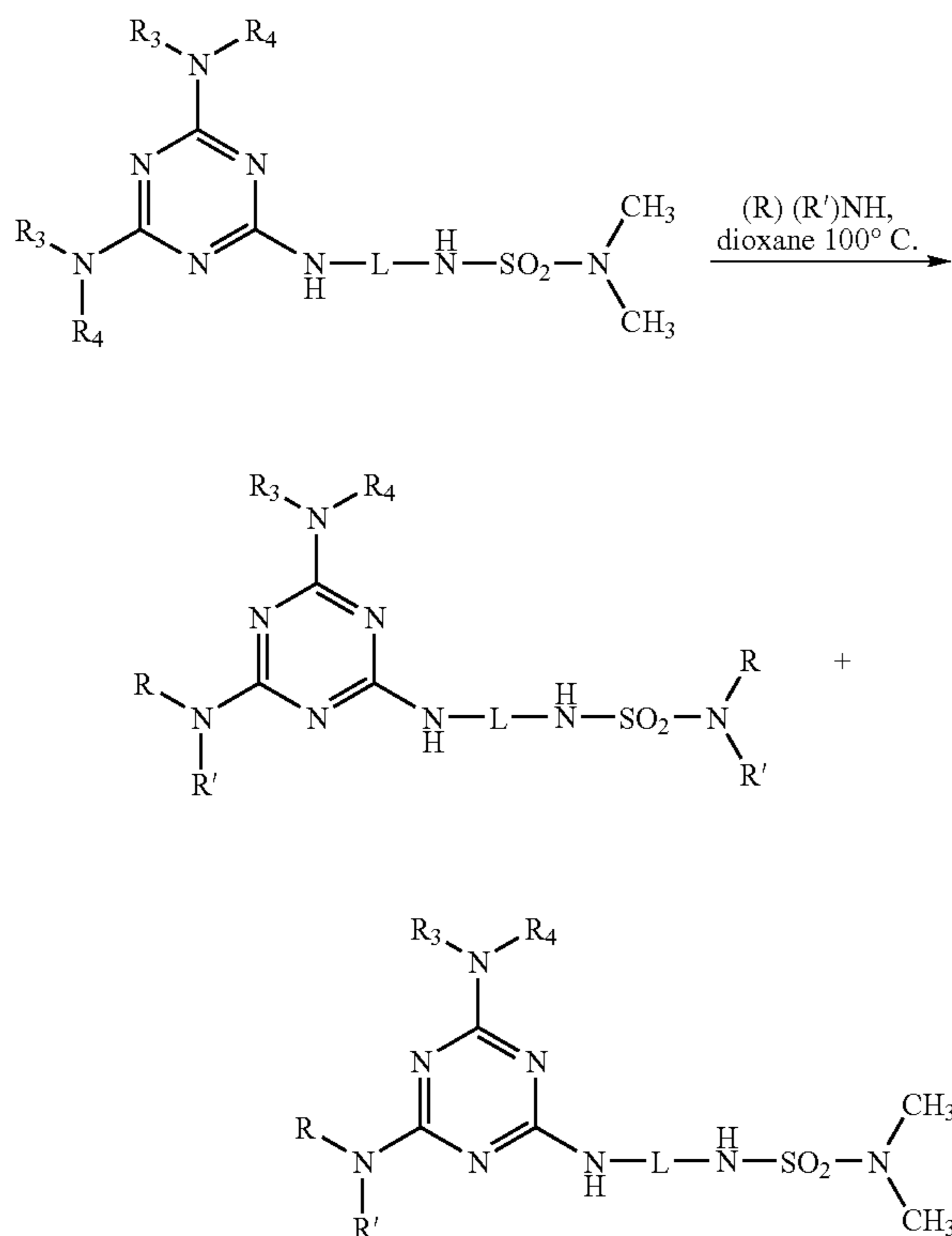
Scheme 4B. Synthesis of Triazine Derivatives
