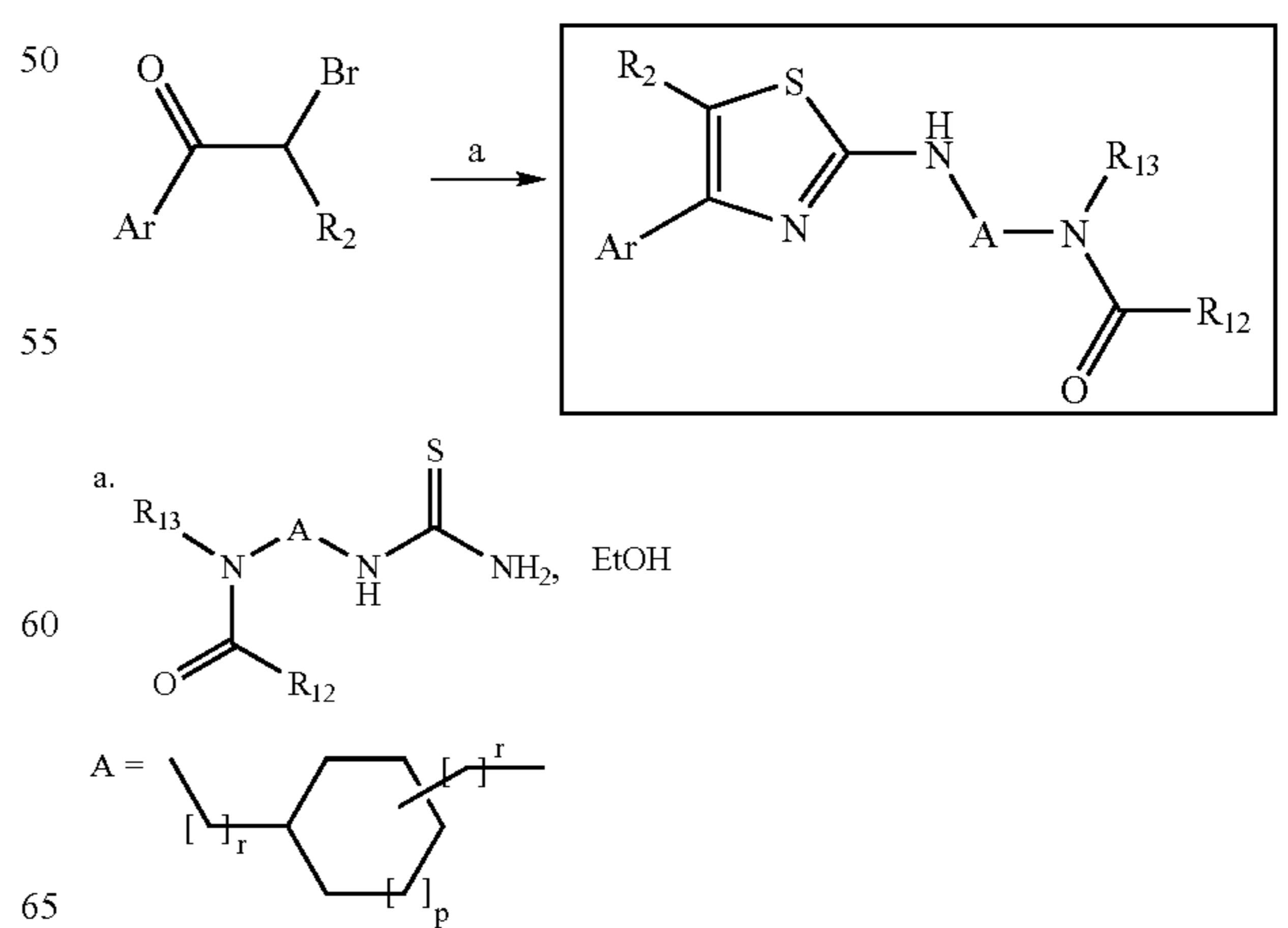
Scheme 8D. Synthesis of Bicycles
