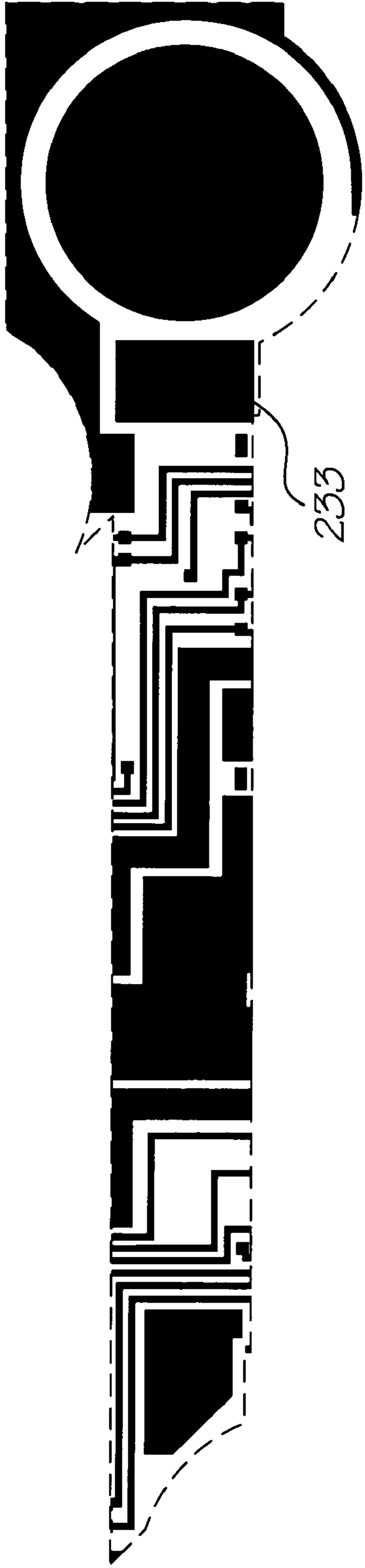
Metal 2 mask
