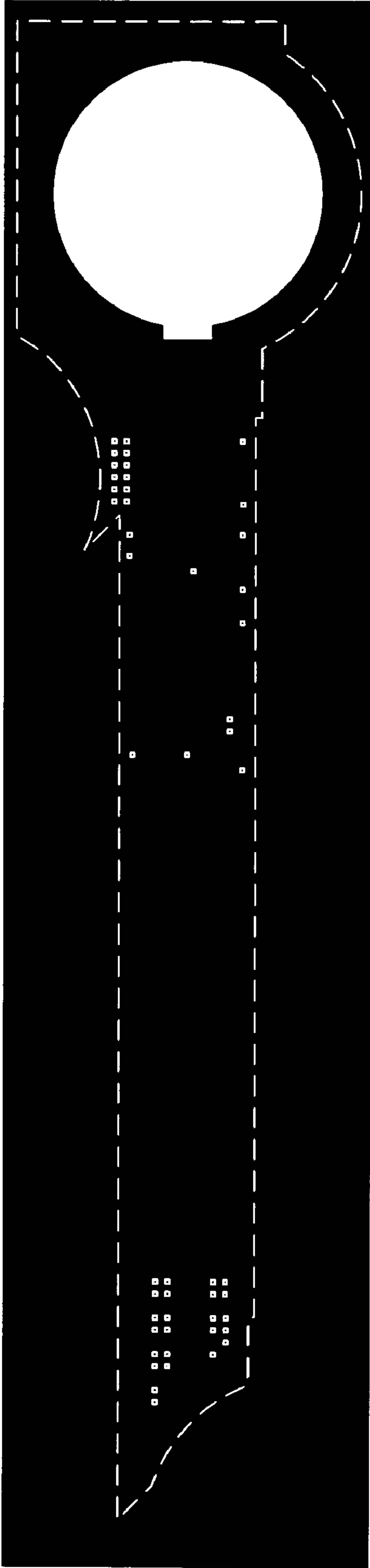
Via 1 mask
