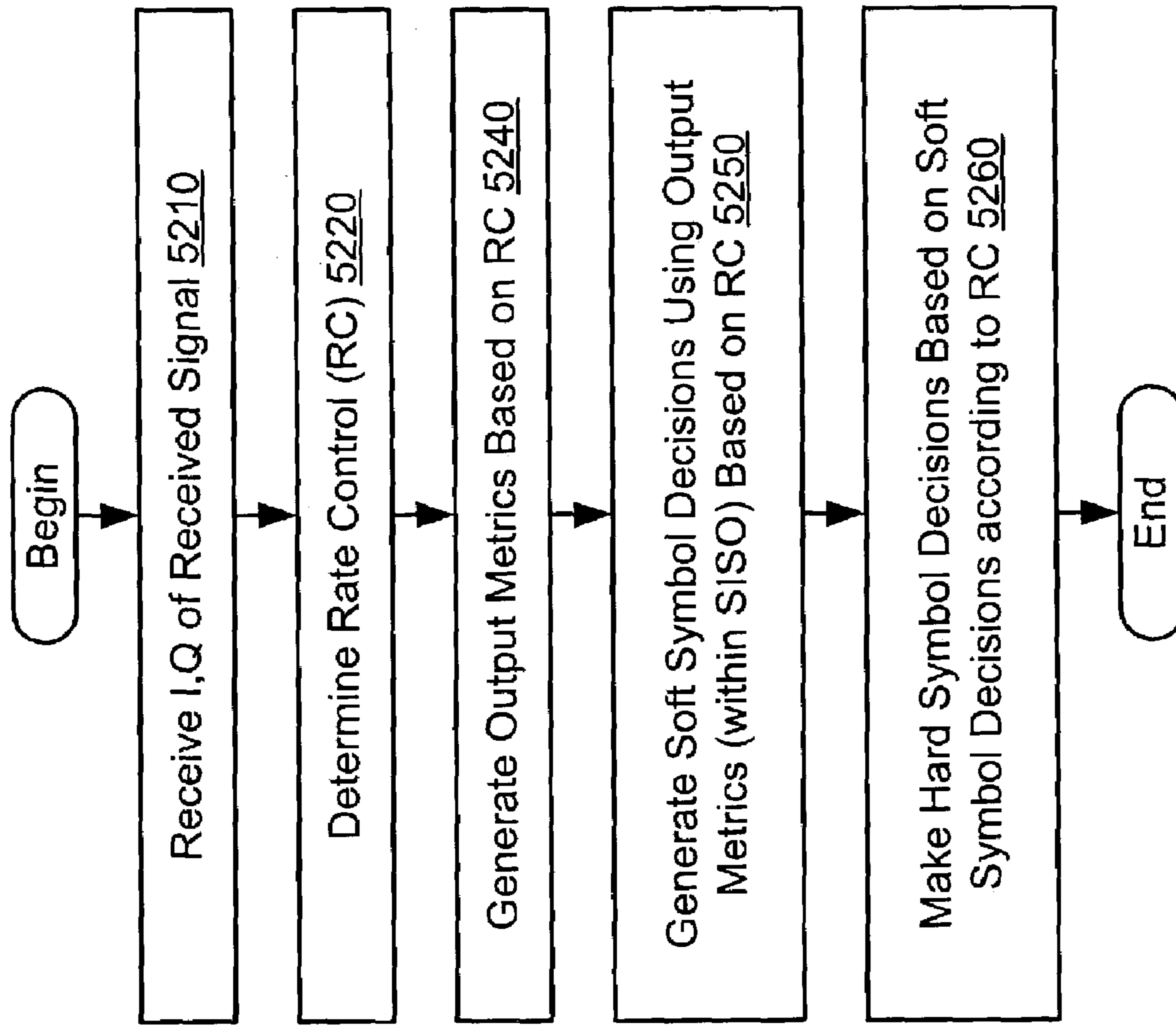
TTCCM Variable Code Rate Decoding Method 5200
