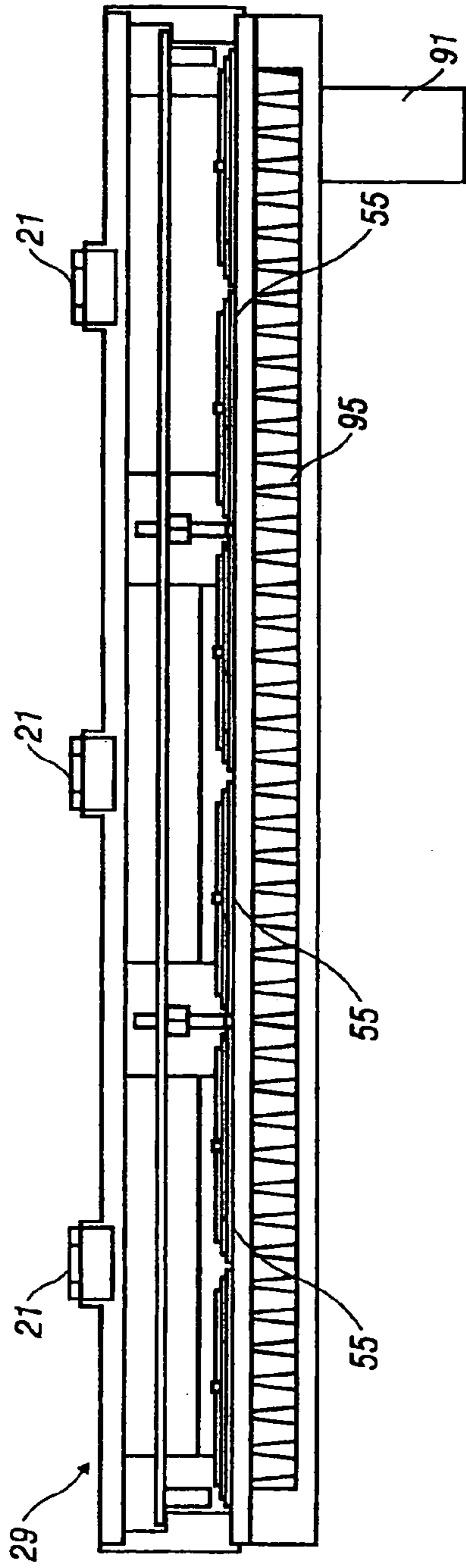
SECTION C-C
