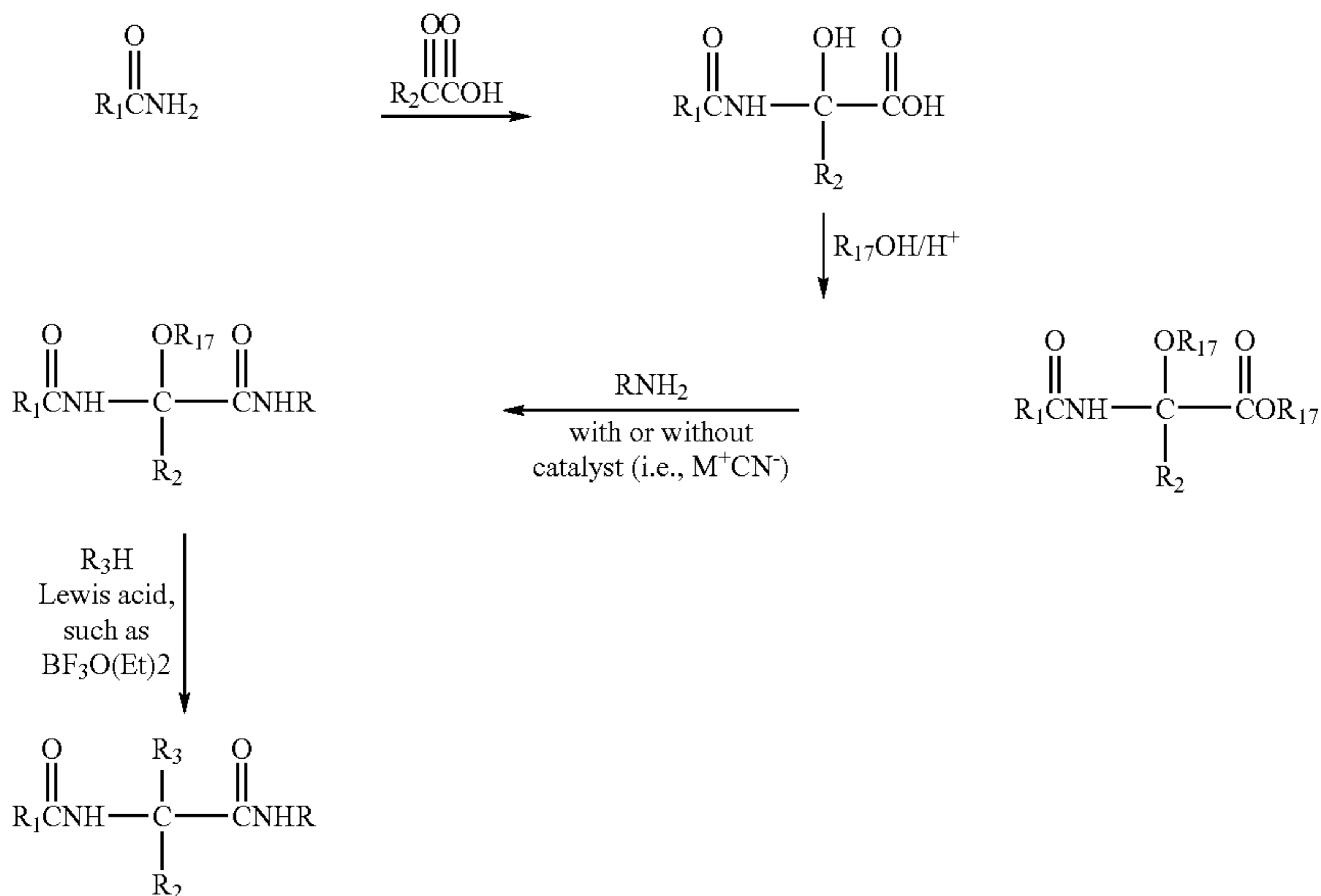
Scheme III
