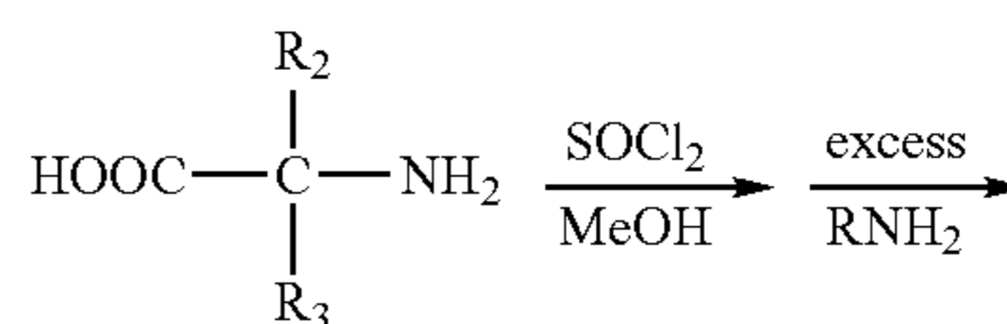
Scheme I
