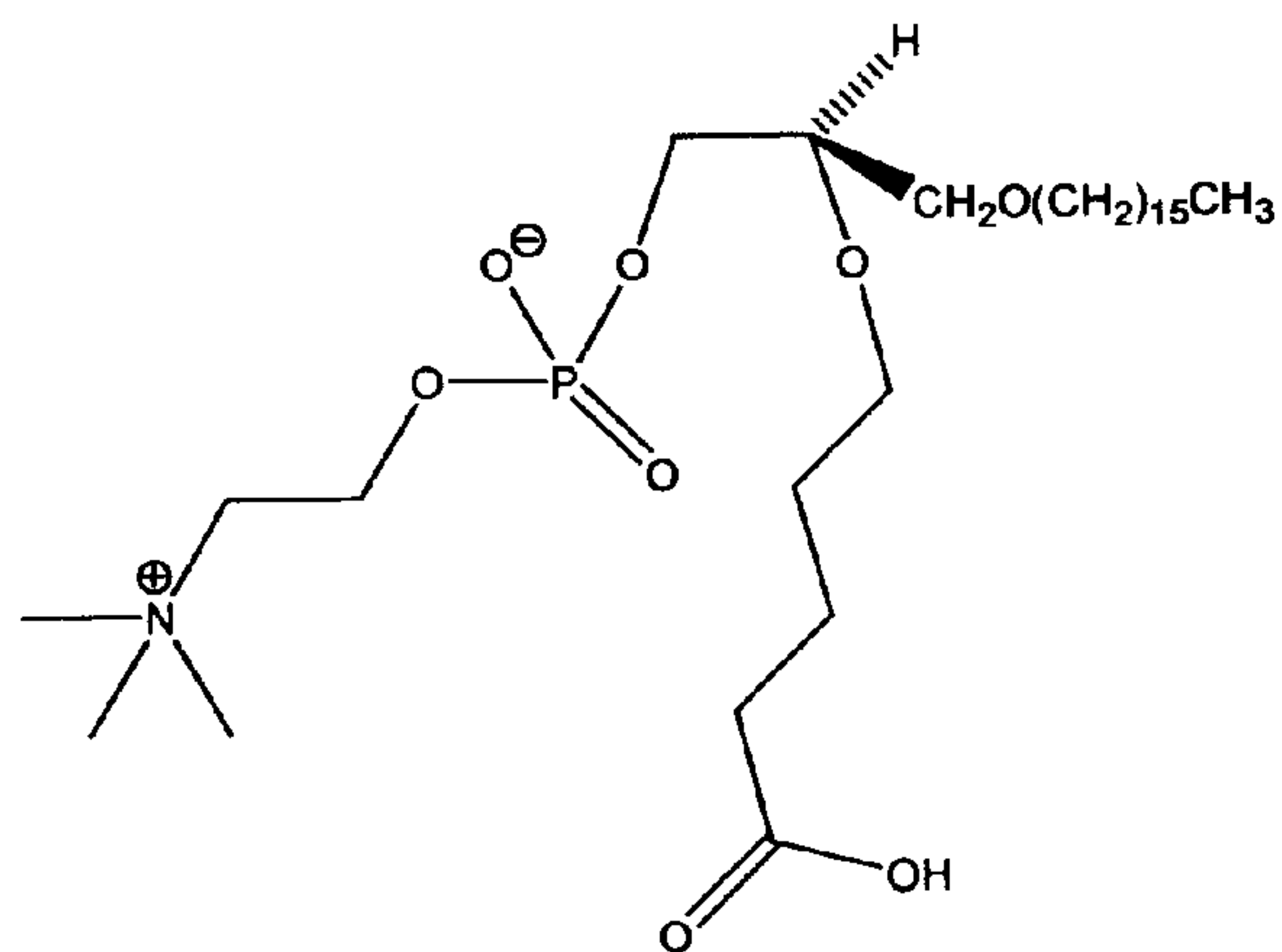
Compound I
