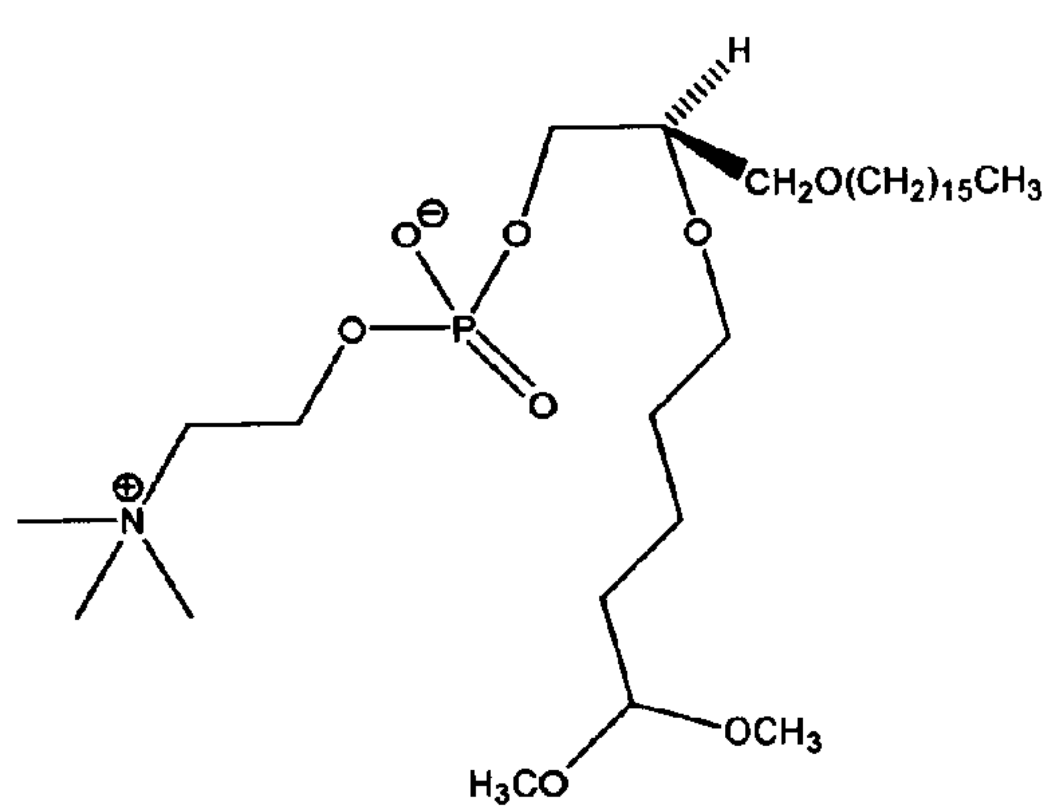
Compound IIa
