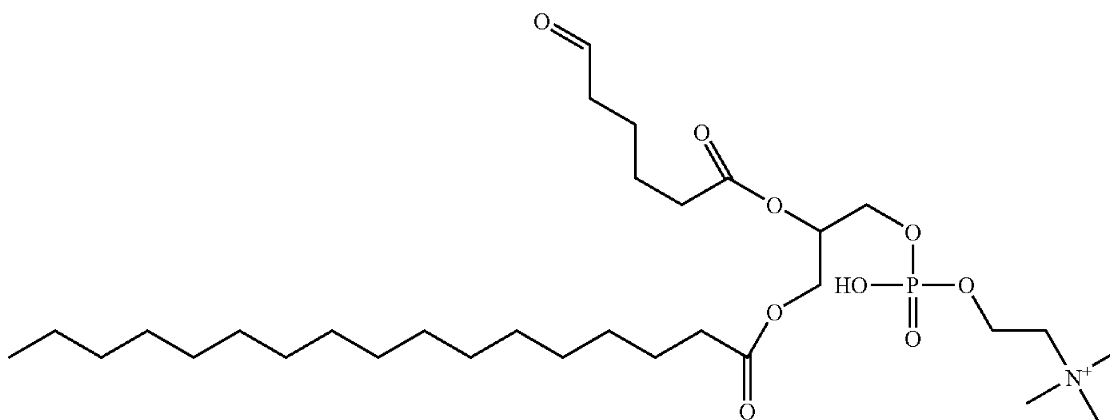
1-hexadecanoyl-2-(5'-oxo-pentanyl)-sn-3-phosphocholine
