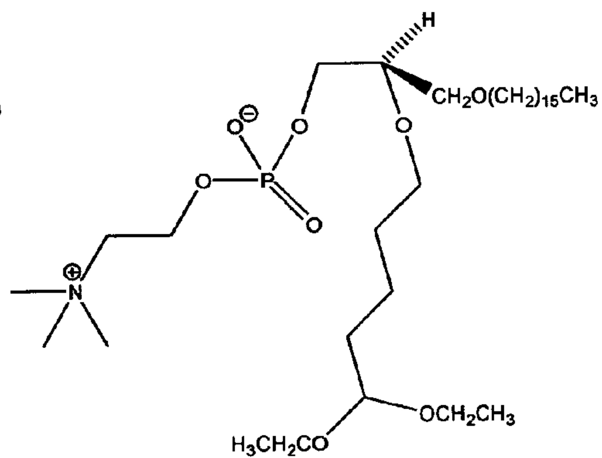
Compound IIb
